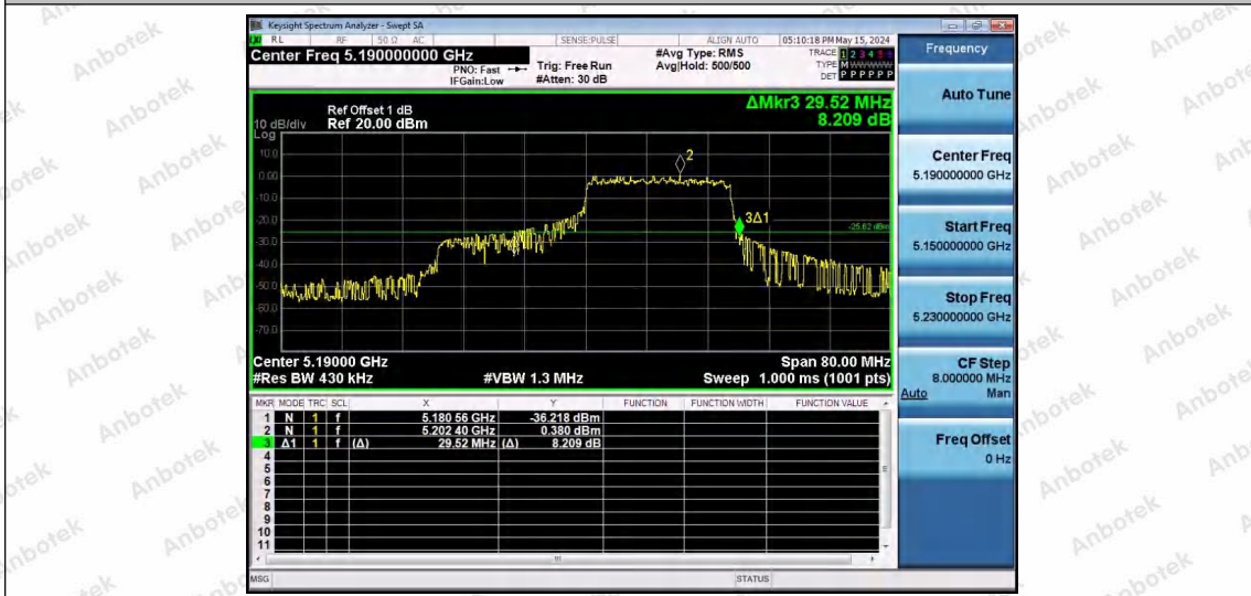
11AX40SISO-Ant1-5190-242Tone-RU62
