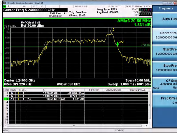
11AX20SISO-Ant1-5240-26Tone-RU8
