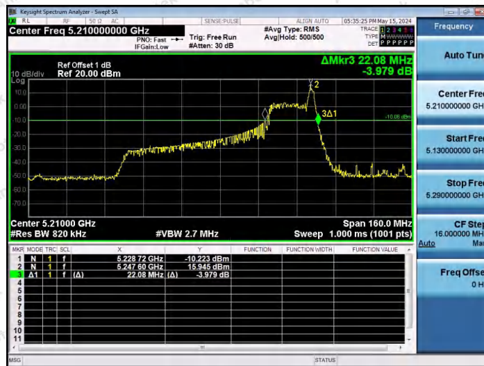
11AX80SISO-Ant1-5210-26Tone-RU36
