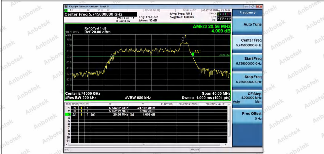
11AX20SISO-Ant1-5745-26Tone-RU8
