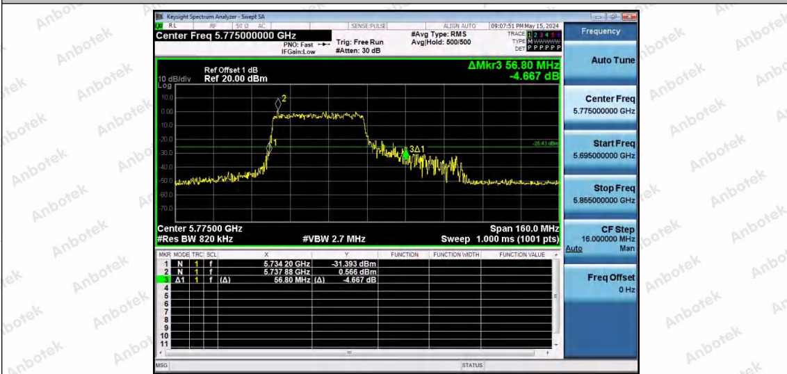
11AX80SISO-Ant1-5775-484Tone-RU65
