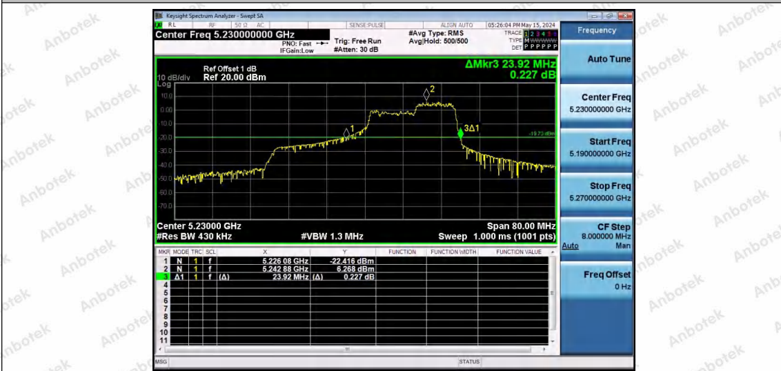
11AX40SISO-Ant1-5230-106Tone-RU56
