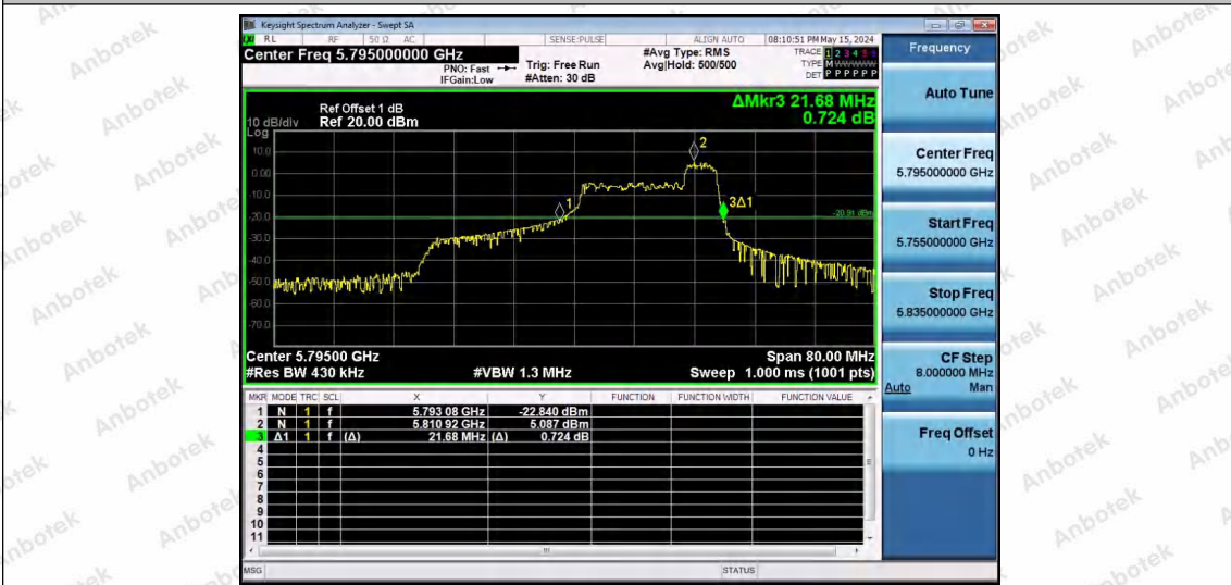
11AX40SISO-Ant1-5795-52Tone-RU44
