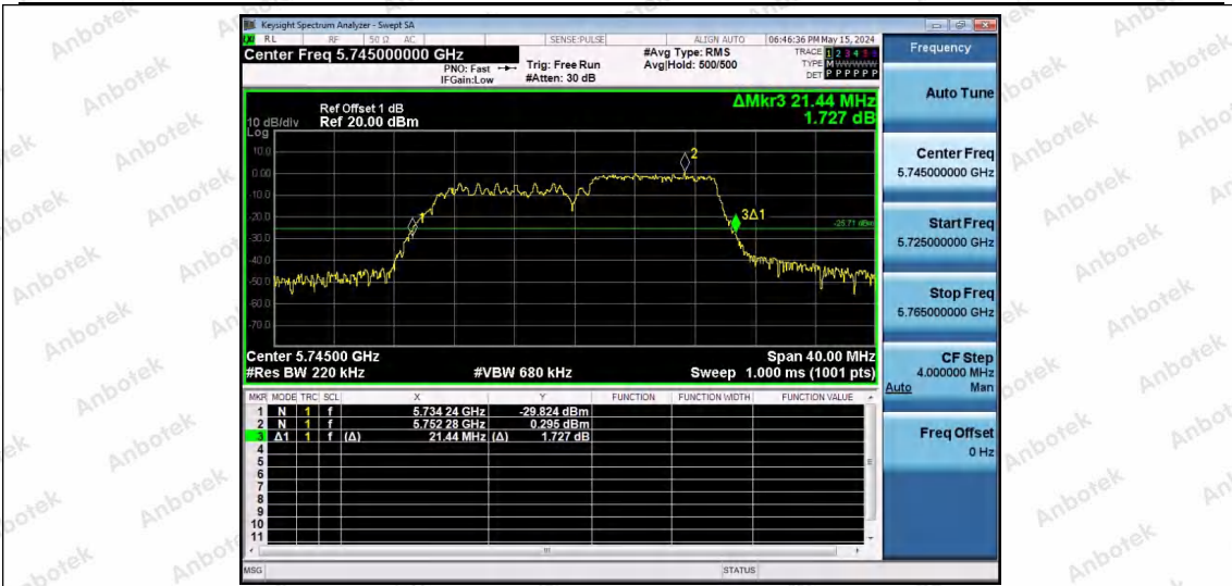
11AX20SISO-Ant1-5745-106Tone-RU54
