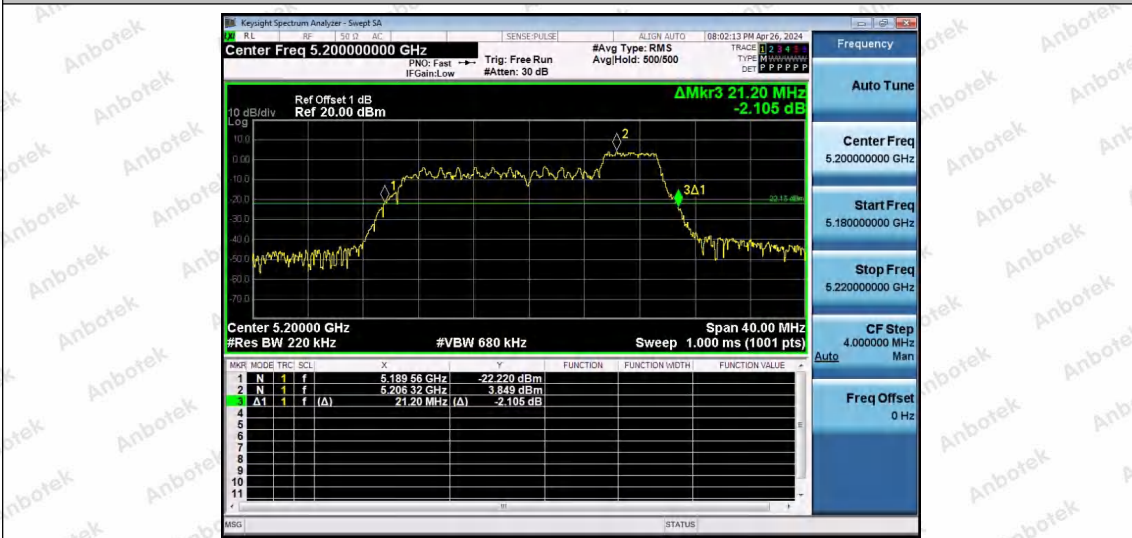
11AX20SISO-Ant1-5200-52Tone-RU40
