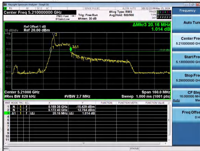
11AX80SISO-Ant1-5210-26Tone-RU0
