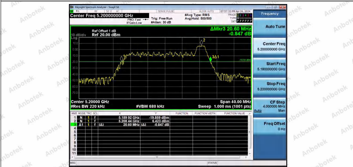
11AX20SISO-Ant1-5200-26Tone-RU8
