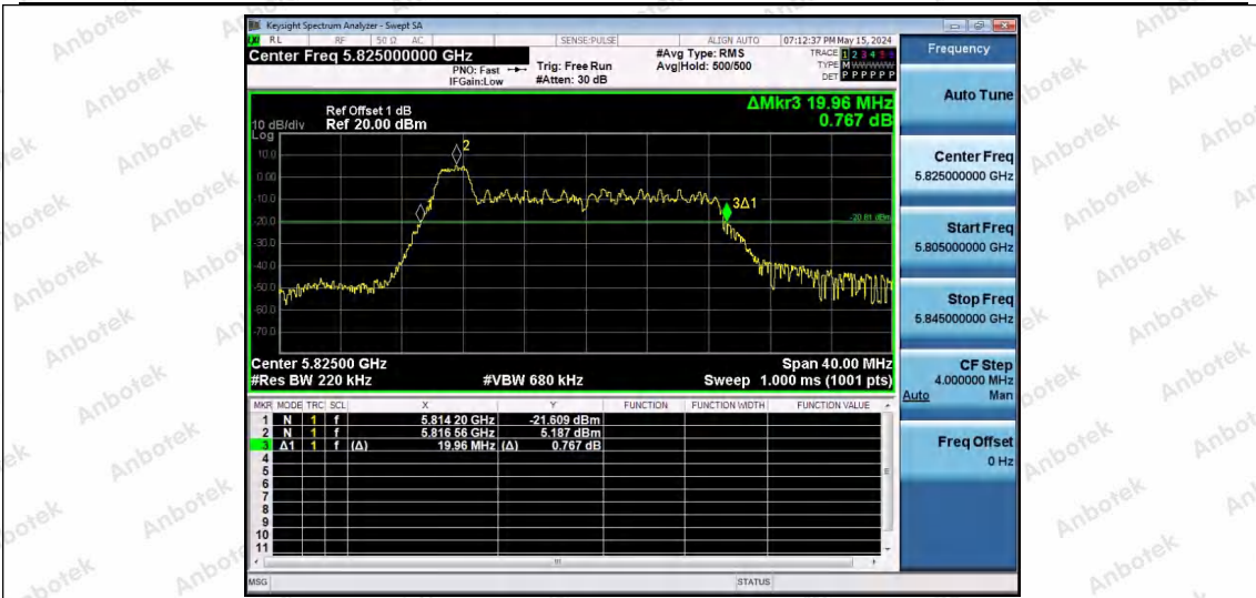
11AX20SISO-Ant1-5825-26Tone-RU0
