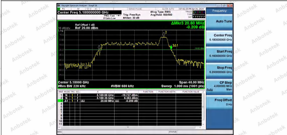
11AX20SISO-Ant1-5180-26Tone-RU8
