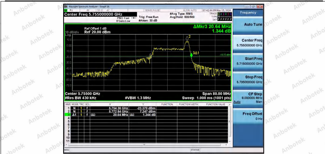
11AX40SISO-Ant1-5755-26Tone-RU17
