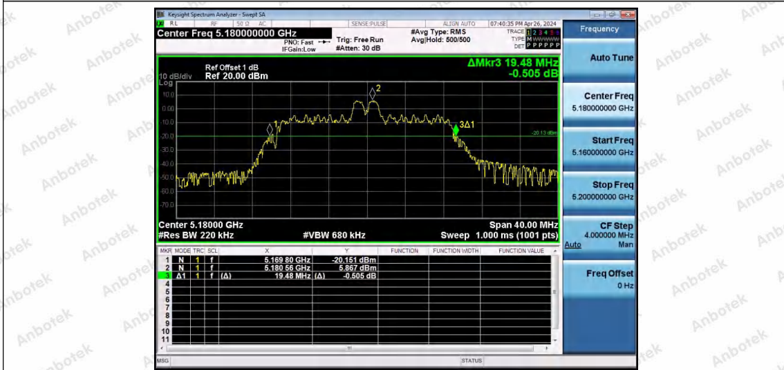
11AX20SISO-Ant1-5180-26Tone-RU4
