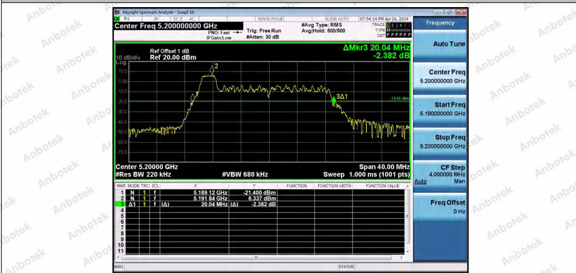
11AX20SISO-Ant1-5200-26Tone-RU0
