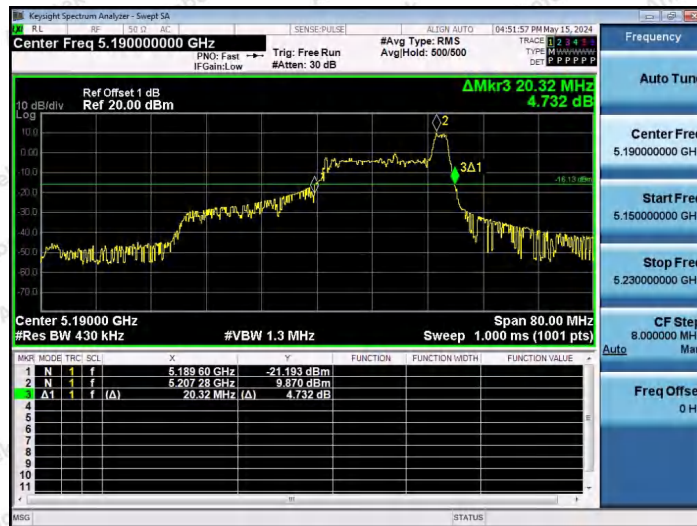
11AX40SISO-Ant1-5190-26Tone-RU17
