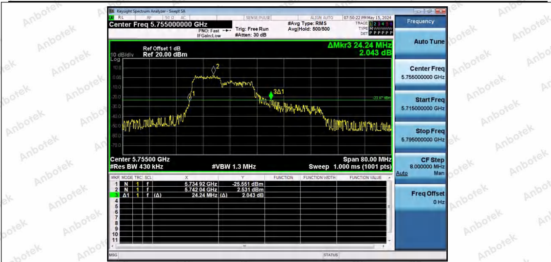
11AX40SISO-Ant1-5755-106Tone-RU53
