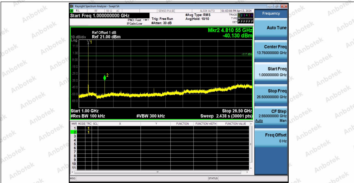
Zigbee_Ant1_2440_0~Reference
