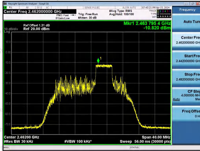
11AX20SISO-Ant1-2462-52Tone-RU39-PASS
