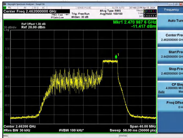
11AX20SISO-Ant1-2462-52Tone-RU40-PASS
