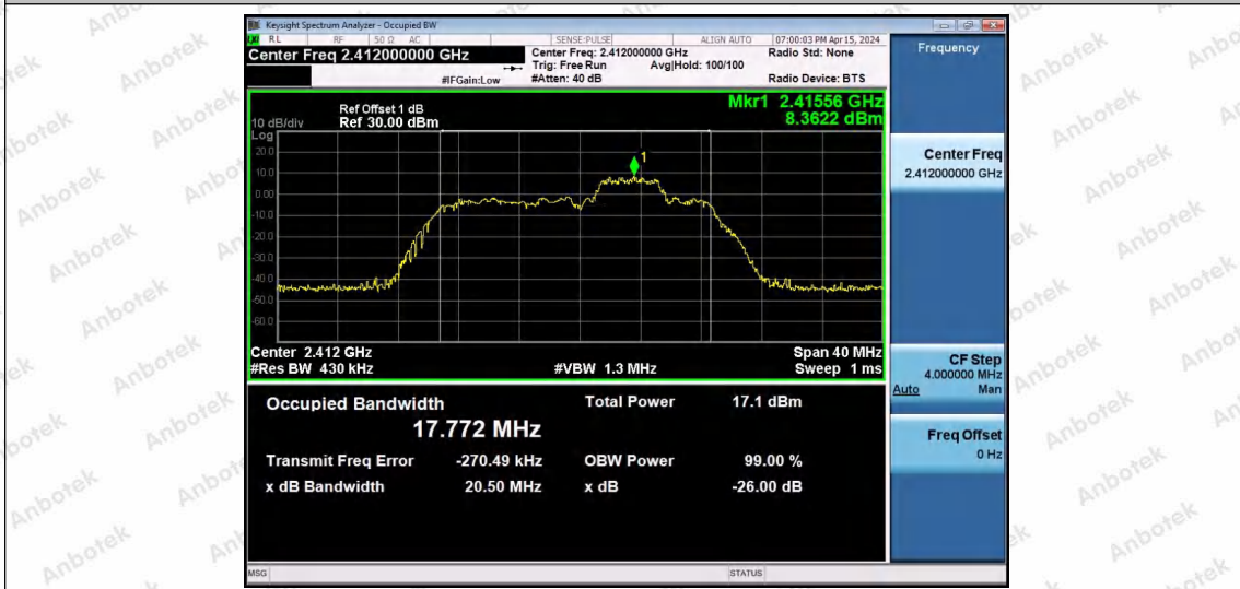
11AX20SISO-Ant1-2412-52Tone-RU37
