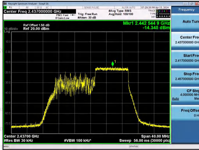
11AX20SISO-Ant1-2437-106Tone-RU54-PASS
