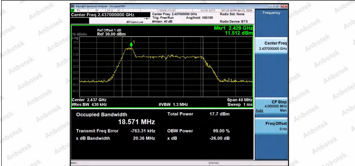
11AX20SISO-Ant1-2437-26Tone-RU0
