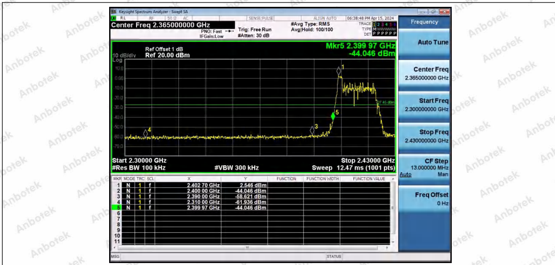
11AX20SISO-Ant1-2412-26Tone-RU0-PASS
