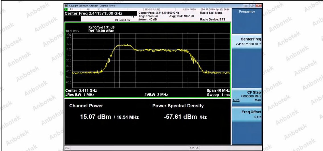
11AX20SISO-Ant1-2412-52Tone-RU37-PASS
