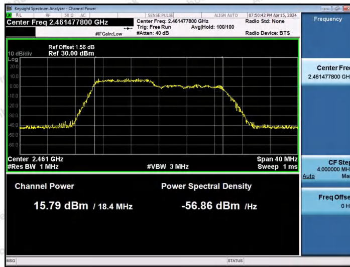
11AX20SISO-Ant1-2462-106Tone-RU53-PASS
