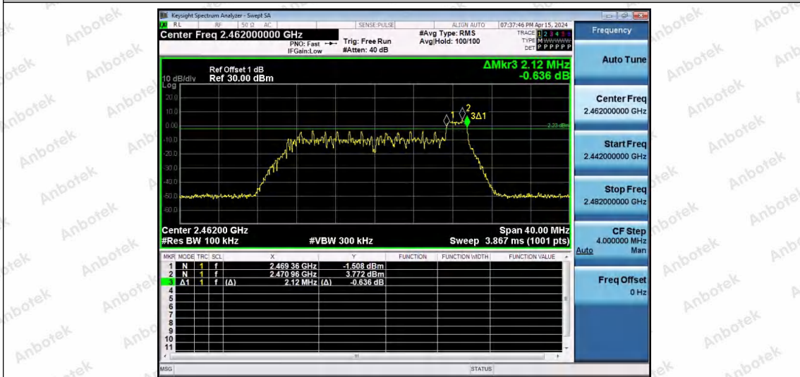
11AX20SISO-Ant1-2462-26Tone-RU8-PASS
