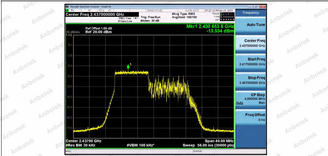
11AX20SISO-Ant1-2437-52Tone-RU40-PASS
