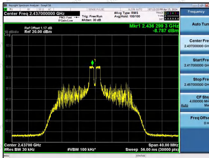
11AX20SISO-Ant1-2437-26Tone-RU0-PASS
