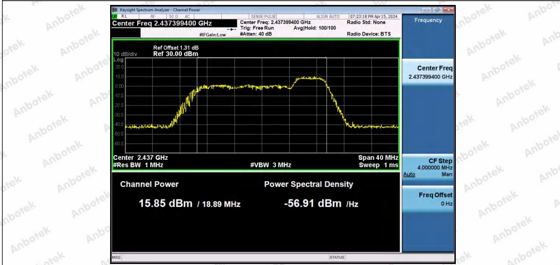
11AX20SISO-Ant1-2437-52Tone-RU40-PASS
