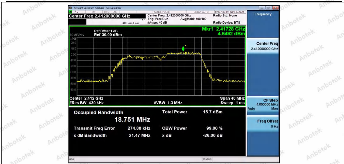
11AX20SISO-Ant1-2412-106Tone-RU54
