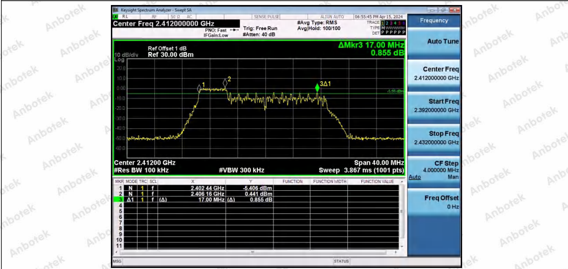
11AX20SISO-Ant1-2412-52Tone-RU37-PASS
