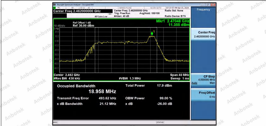
11AX20SISO-Ant1-2462-26Tone-RU8
