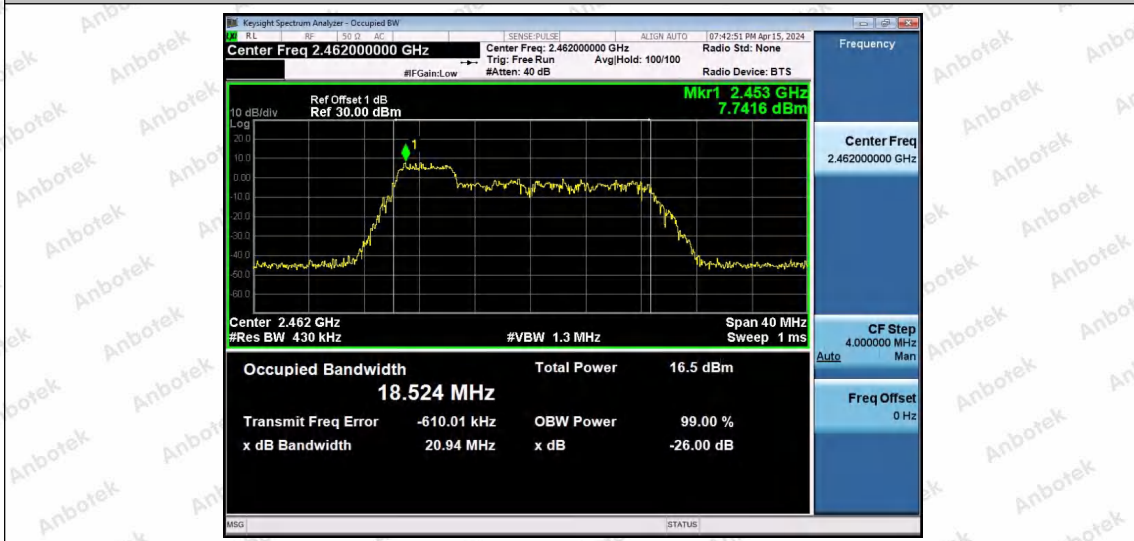
11AX20SISO-Ant1-2462-26Tone-RU8
