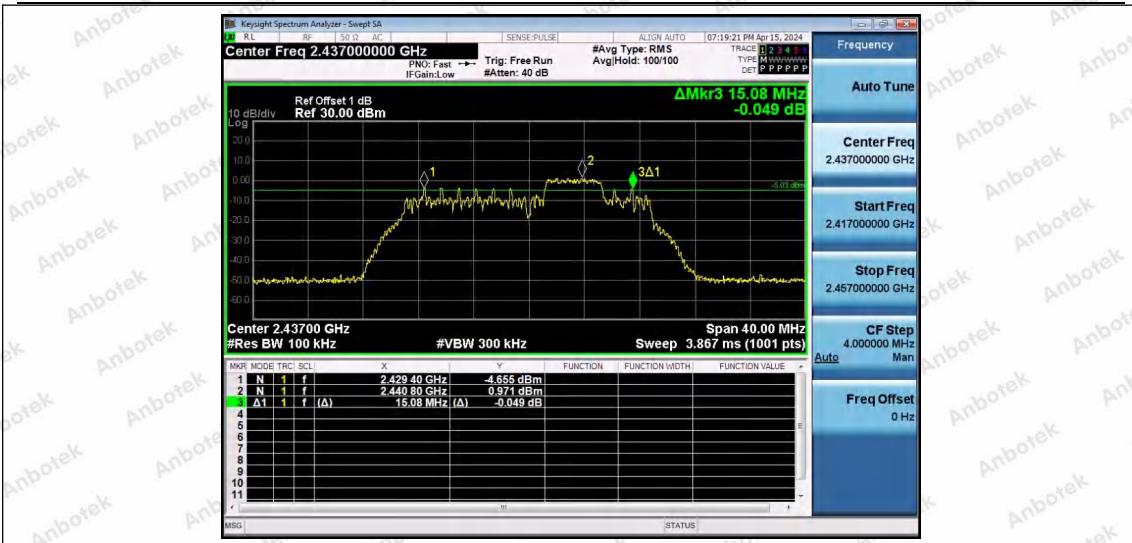
11AX20SISO-Ant1-2437-52Tone-RU39-PASS
