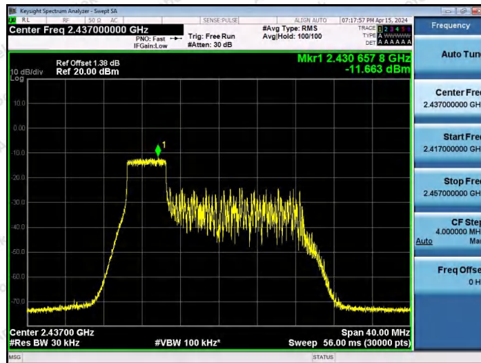
11AX20SISO-Ant1-2437-52Tone-RU37-PASS
