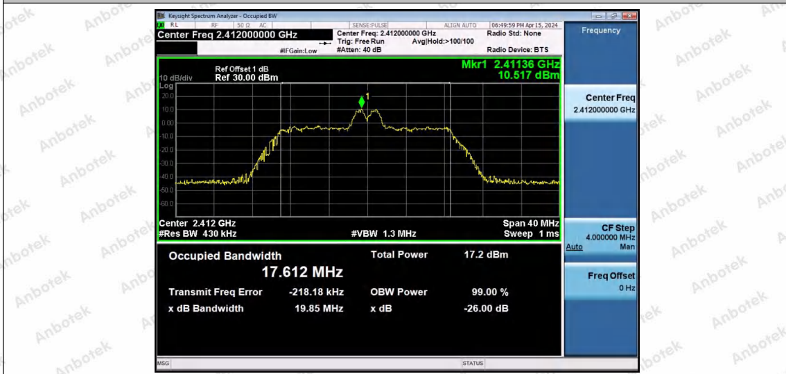
11AX20SISO-Ant1-2412-26Tone-RU4
