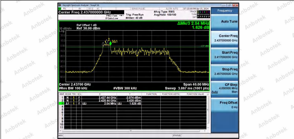
11AX20SISO-Ant1-2437-26Tone-RU0-PASS
