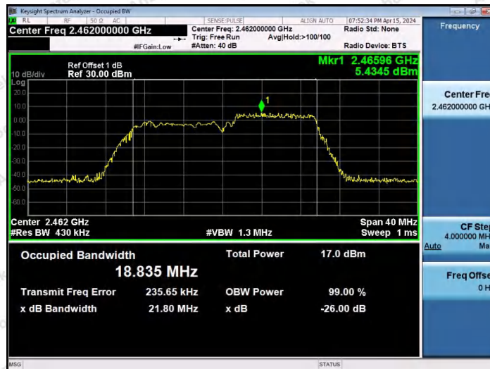
11AX20SISO-Ant1-2462-106Tone-RU54
