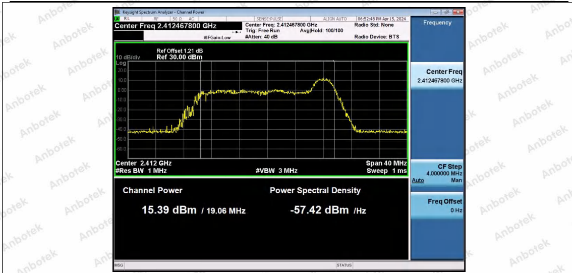
11AX20SISO-Ant1-2412-26Tone-RU8-PASS
