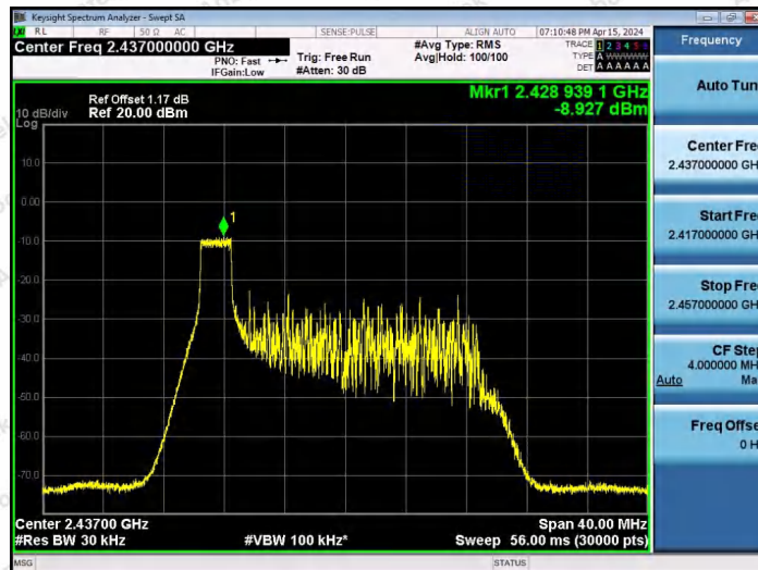
11AX20SISO-Ant1-2437-26Tone-RU0-PASS
