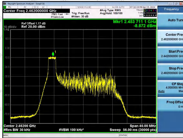
11AX20SISO-Ant1-2462-26Tone-RU0-PASS
