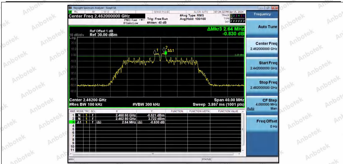
11AX20SISO-Ant1-2462-26Tone-RU4-PASS
