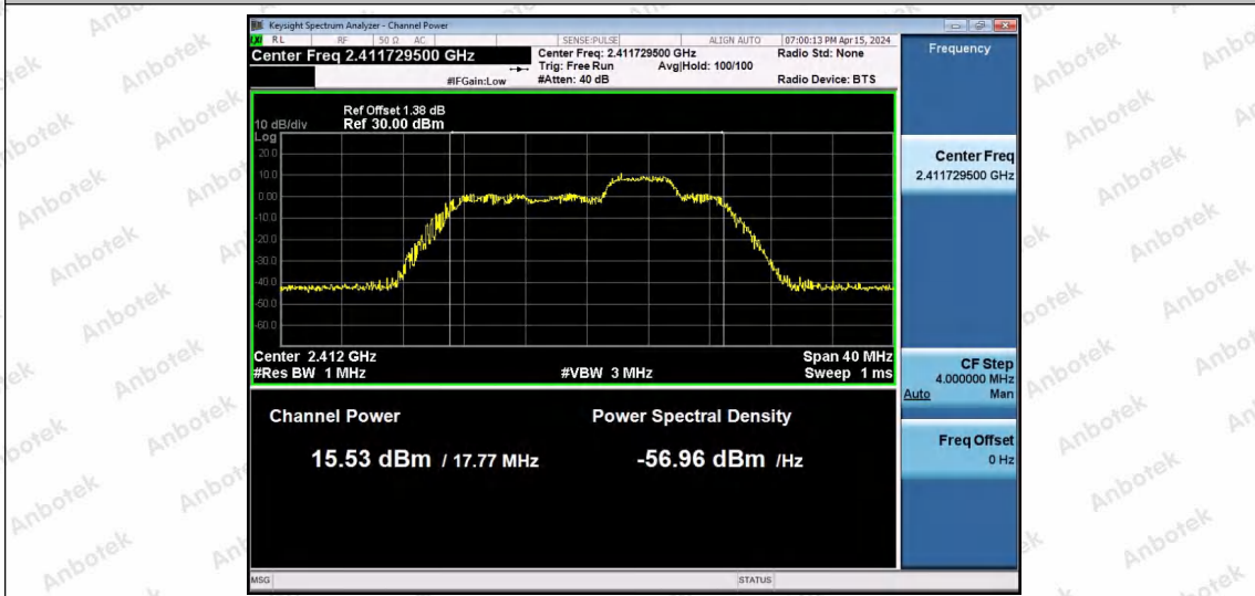
11AX20SISO-Ant1-2412-52Tone-RU37-PASS
