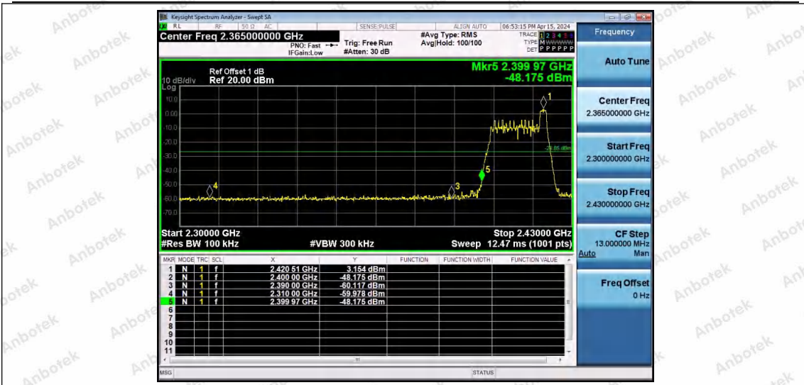
11AX20SISO-Ant1-2412-26Tone-RU8-PASS
