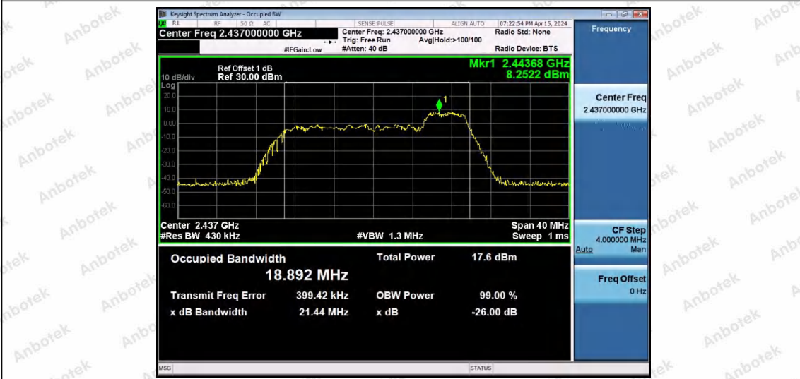
11AX20SISO-Ant1-2437-52Tone-RU40
