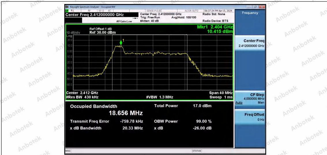
11AX20SISO-Ant1-2412-26Tone-RU0
