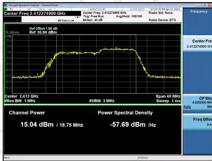
11AX20SISO-Ant1-2412-106Tone-RU54-PASS
