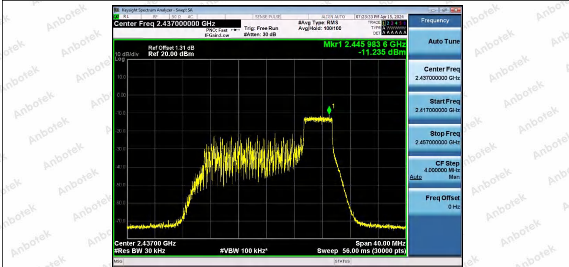
11AX20SISO-Ant1-2437-52Tone-RU40-PASS
