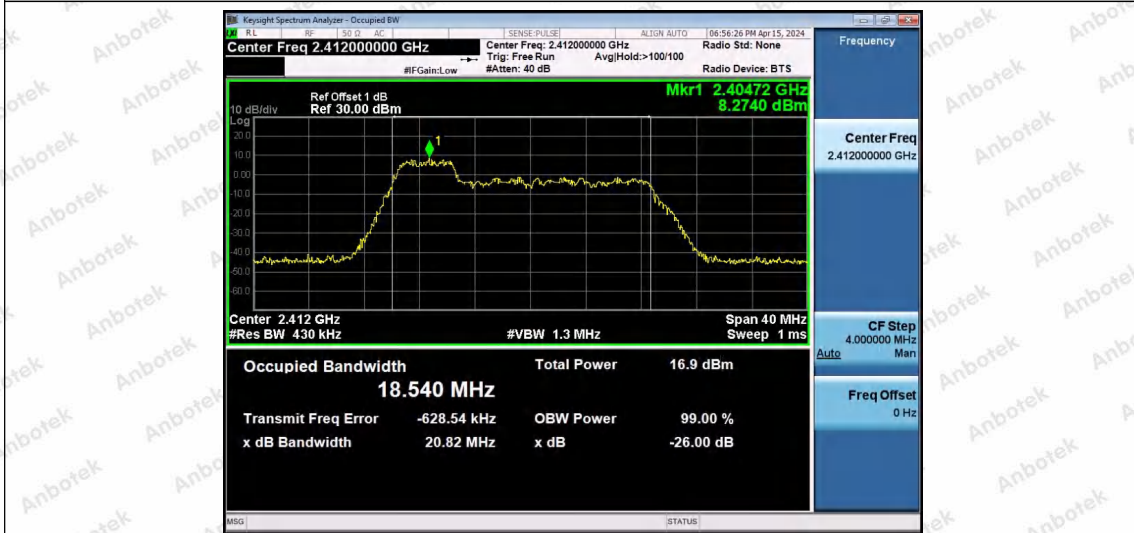
11AX20SISO-Ant1-2412-52Tone-RU37
