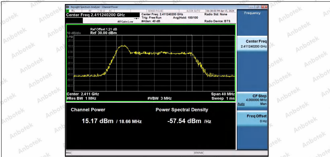
11AX20SISO-Ant1-2412-26Tone-RU0-PASS
