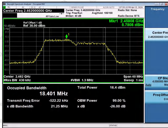
11AX20SISO-Ant1-2462-106Tone-RU53
