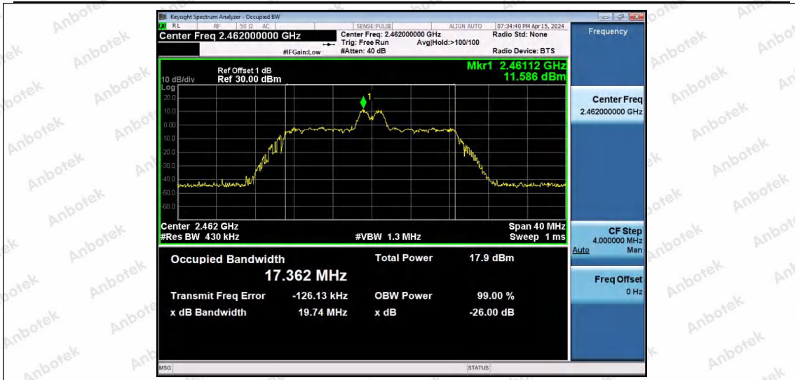
11AX20SISO-Ant1-2462-26Tone-RU4
