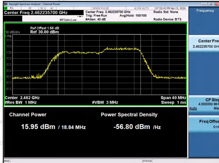
11AX20SISO-Ant1-2462-106Tone-RU54-PASS
