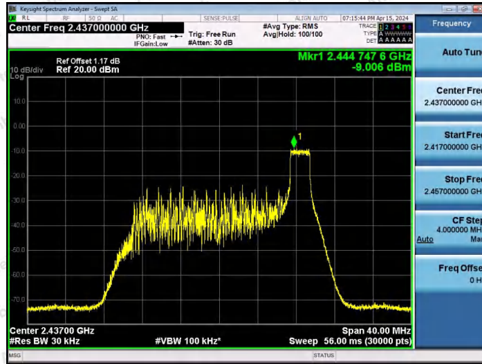
11AX20SISO-Ant1-2437-26Tone-RU8-PASS
