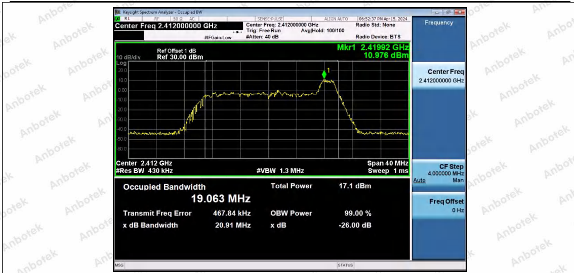
11AX20SISO-Ant1-2412-26Tone-RU8
