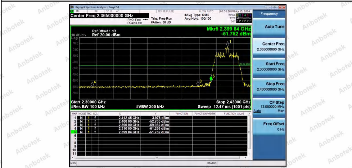
11AX20SISO-Ant1-2412-26Tone-RU4-PASS
