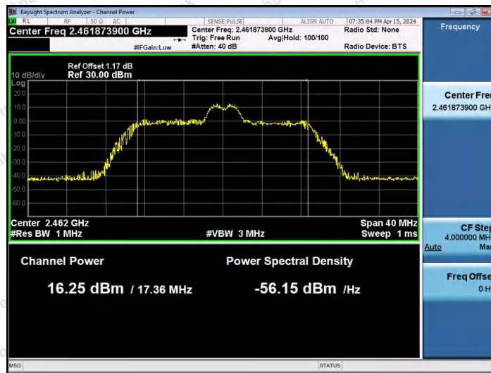
11AX20SISO-Ant1-2462-26Tone-RU4-PASS
