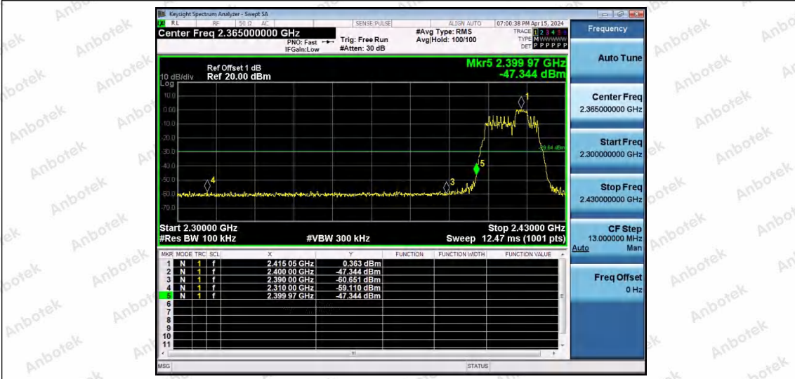
11AX20SISO-Ant1-2412-52Tone-RU37-PASS
