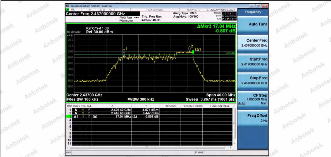
11AX20SISO-Ant1-2437-52Tone-RU40-PASS
