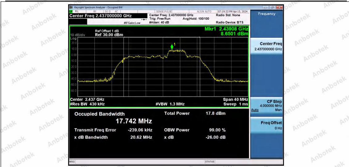
11AX20SISO-Ant1-2437-52Tone-RU39
