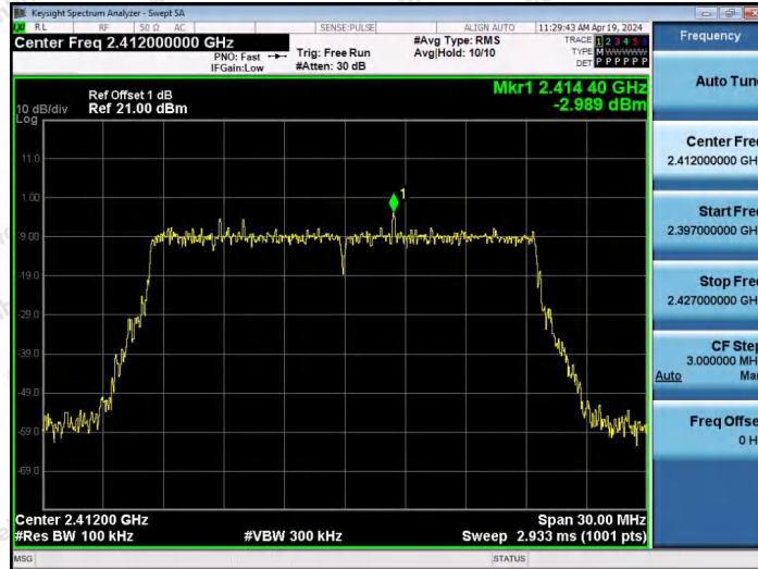
11AX20SISO-Ant1-2412-0~Reference-PASS
