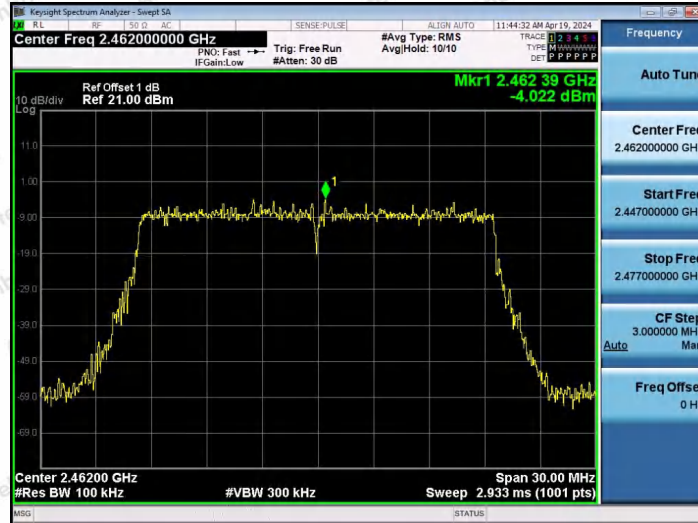
11AX20SISO-Ant1-2462-0~Reference-PASS
