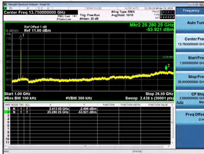
11AX20SISO-Ant1-2412-1000~26500-PASS
