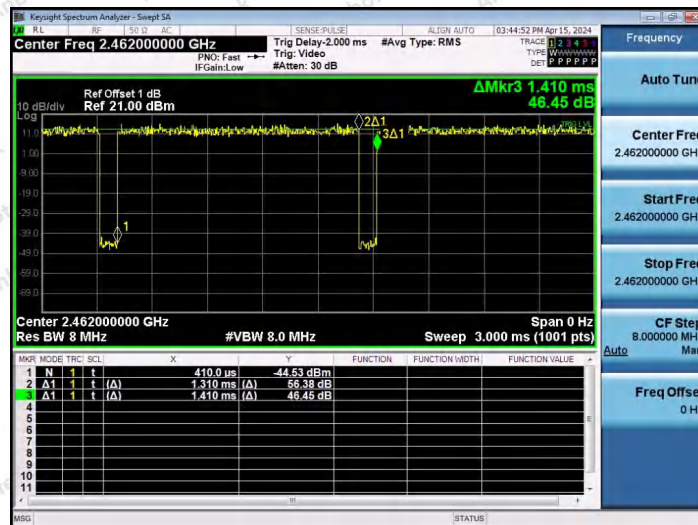
NTNV-11N20SISO-Ant1-2462
