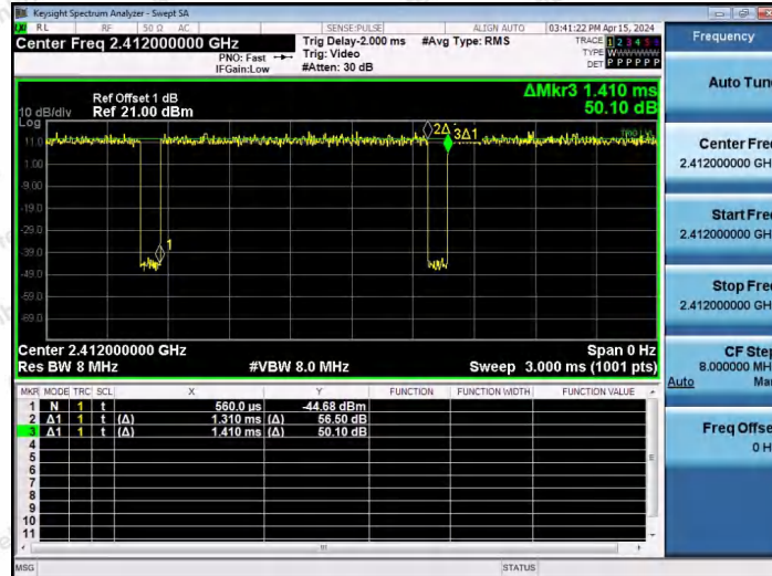
NTNV-11N20SISO-Ant1-2412
