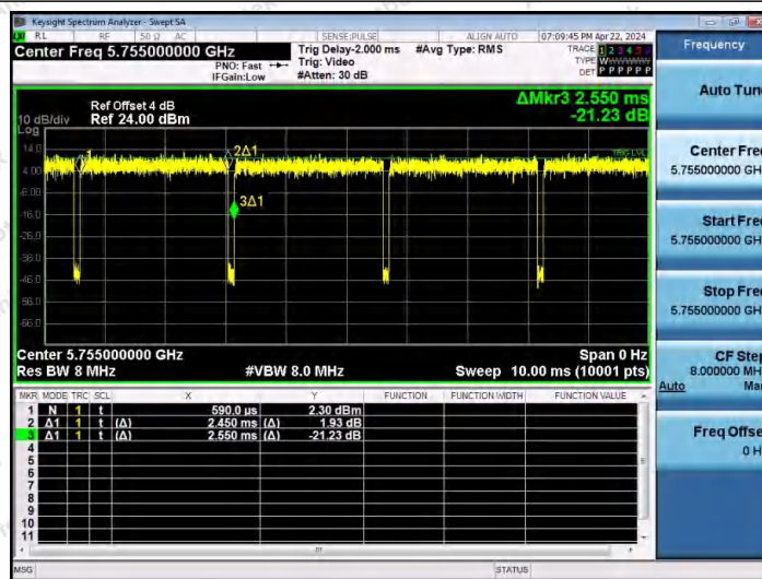
NTNV-11AX40MIMO-Ant2-5755
