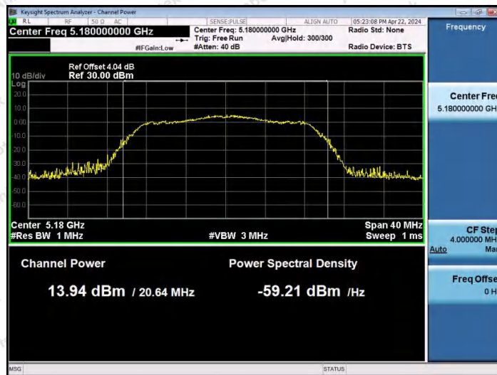
11A20MIMO-Ant1-5180-PASS
