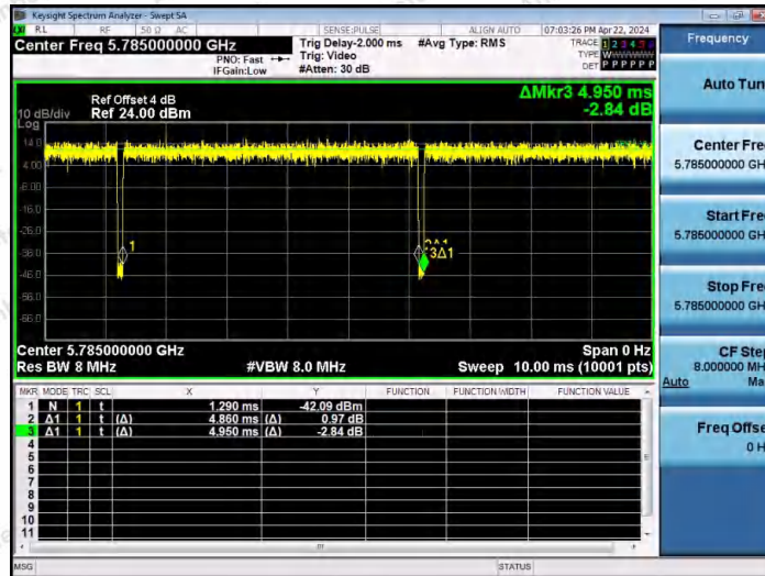
NTNV-11AX20MIMO-Ant2-5785
