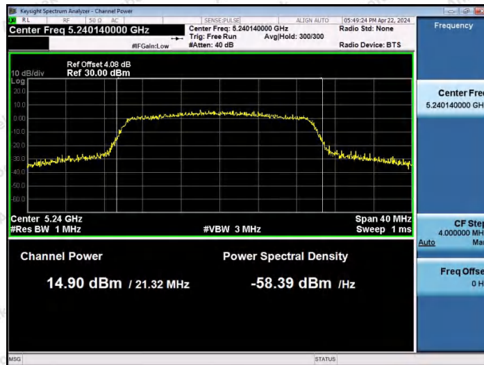
11AX20MIMO-Ant2-5240-PASS
