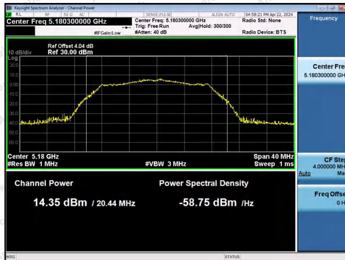
11A-Ant2-5180-PASS
