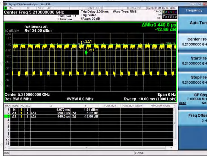
NTNV-11AX80MIMO-Ant2-5210
