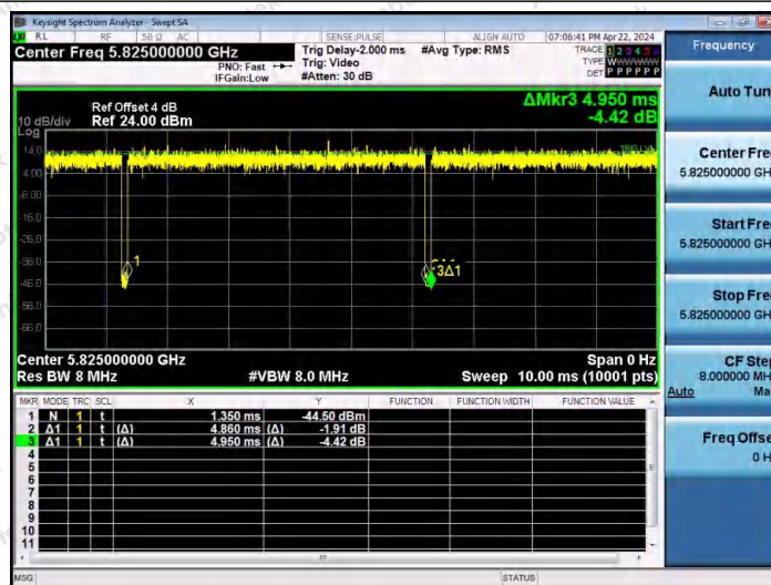
NTNV-11AX20MIMO-Ant2-5825
