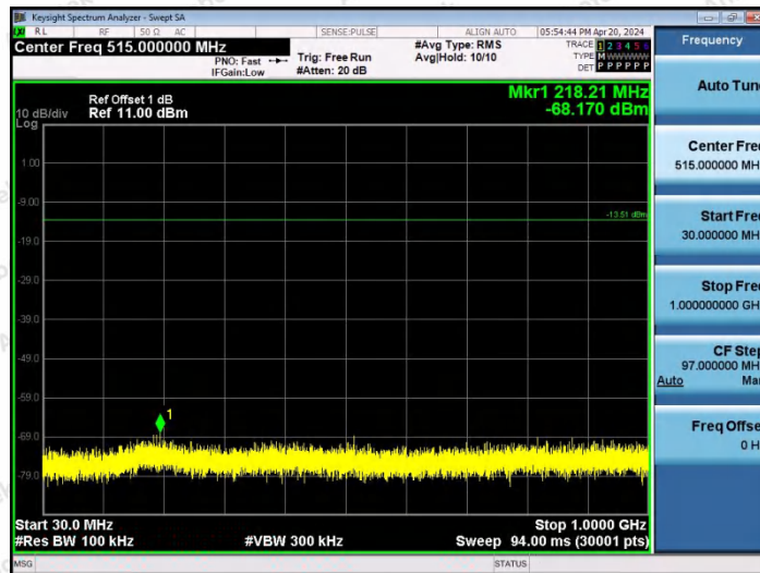
2DH5-Ant2-2441-30~1000-PASS
