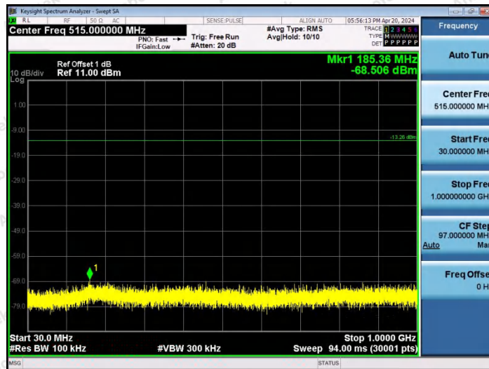
2DH5-Ant2-2480-30~1000-PASS
