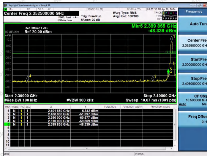
2DH5-Ant2-2402-PASS
