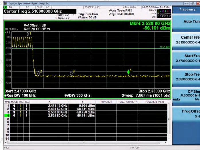
DH5-Ant2-Hop_2480-PASS
