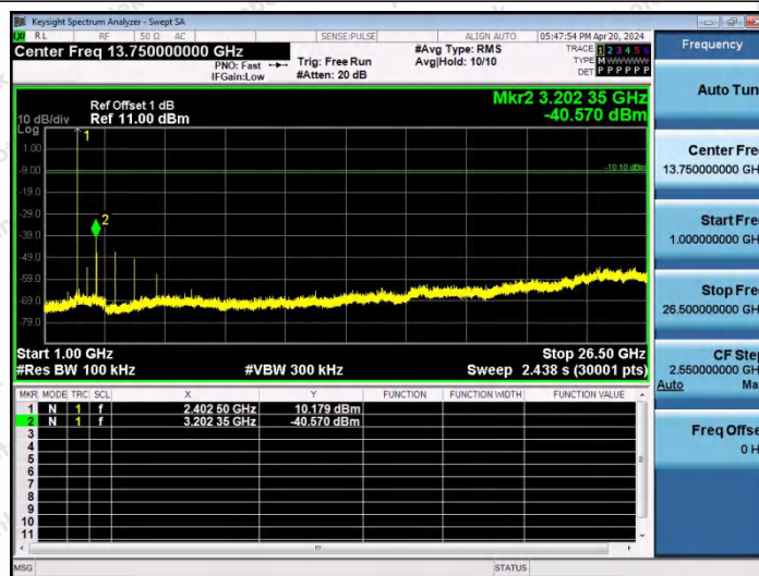
DH5-Ant2-2402-1000~26500-PASS
