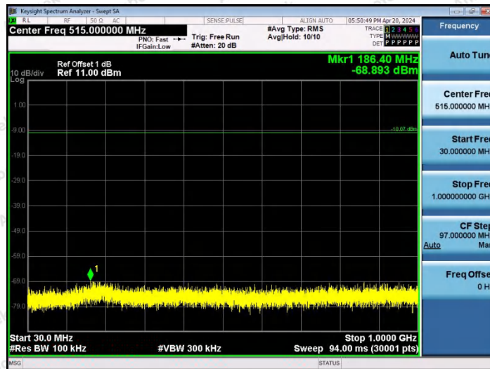
DH5-Ant2-2480-30~1000-PASS
