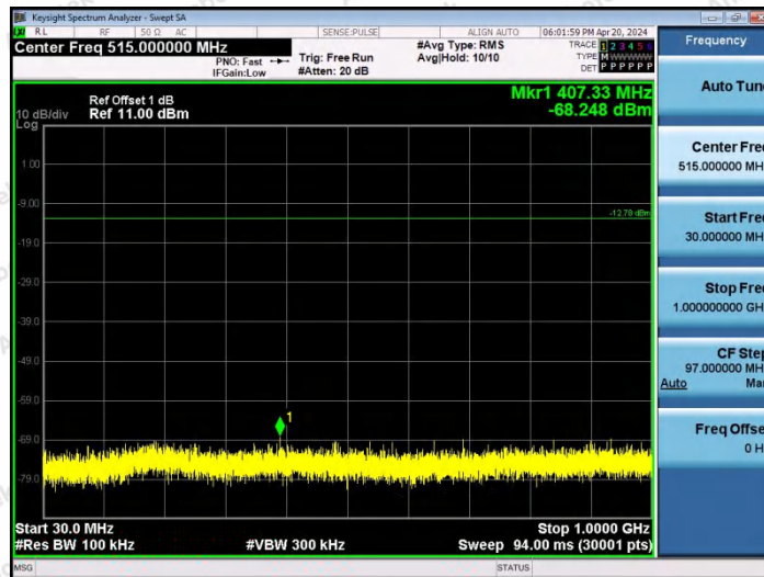
3DH5-Ant2-2480-30~1000-PASS
