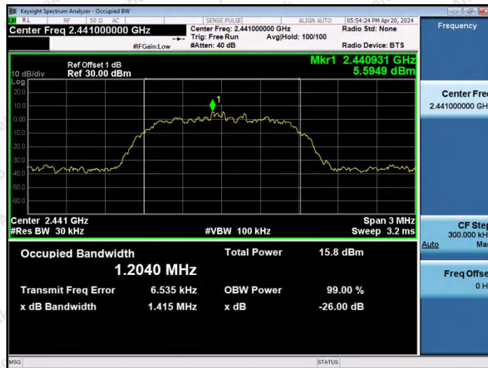
2DH5-Ant2-2441
