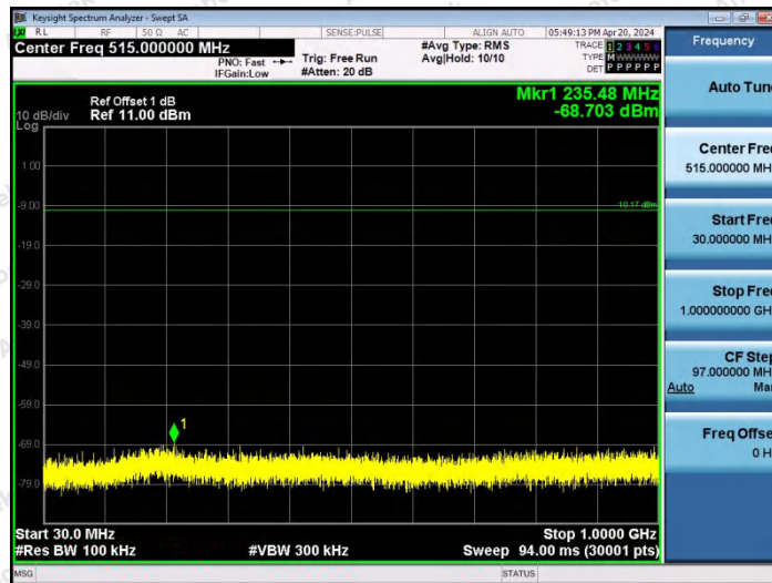
DH5-Ant2-2441-30~1000-PASS
