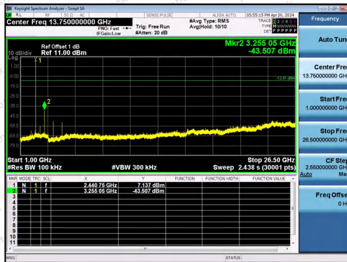
2DH5-Ant2-2441-1000~26500-PASS
