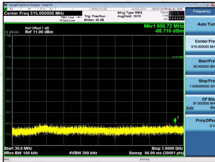
DH5-Ant2-2402-30~1000-PASS
