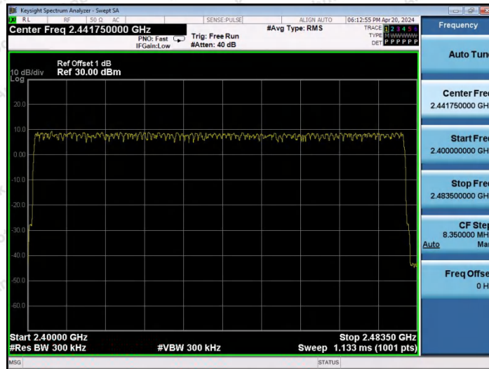
2DH5-Ant2-Hop-PASS
