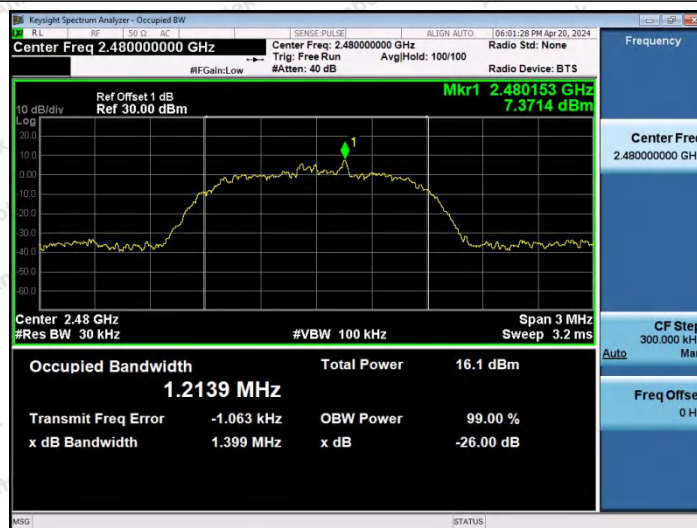
3DH5-Ant2-2480
