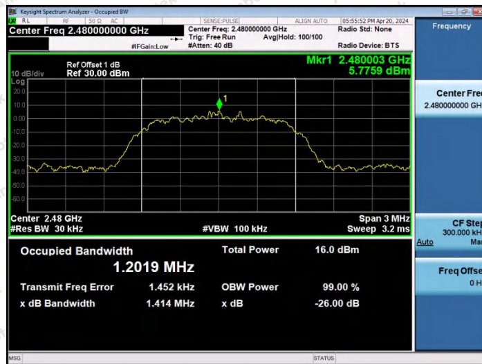
2DH5-Ant2-2480
