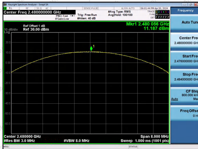
3DH5-Ant2-2480-PASS
