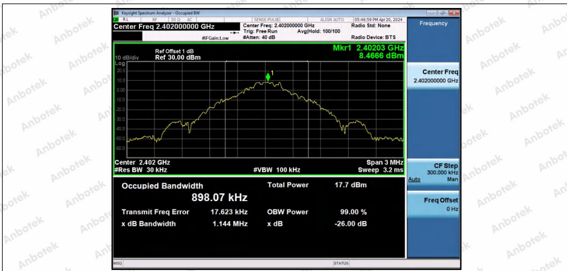
DH5-Ant2-2402
