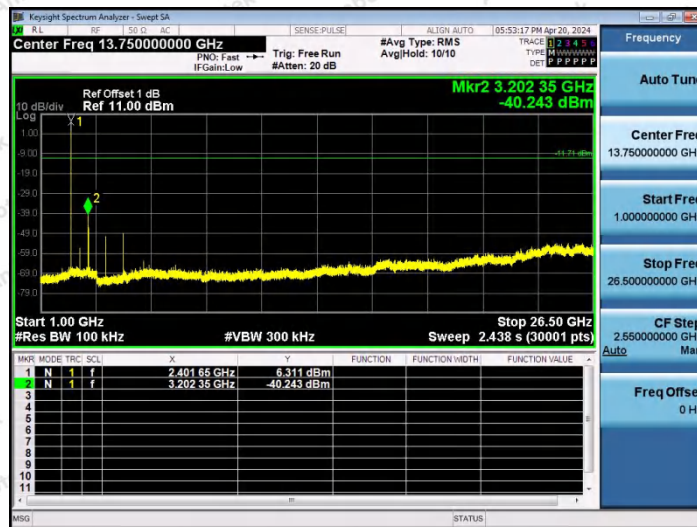
2DH5-Ant2-2402-1000~26500-PASS
