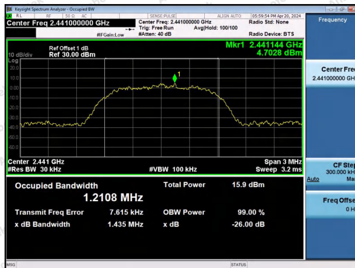
3DH5-Ant2-2441
