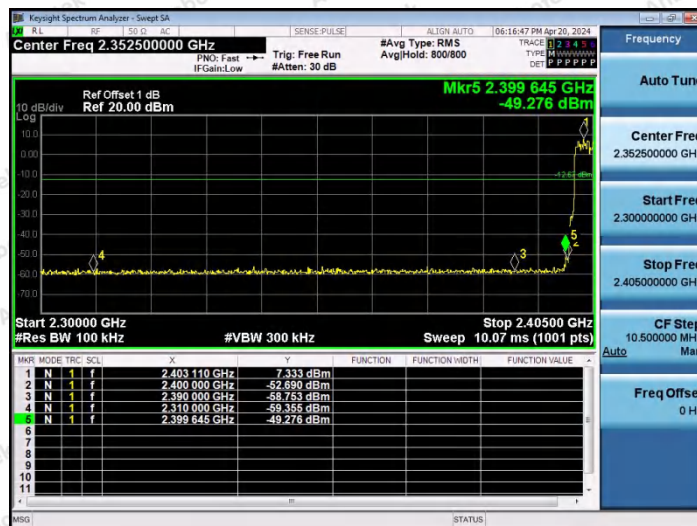
3DH5-Ant2-Hop_2402-PASS
