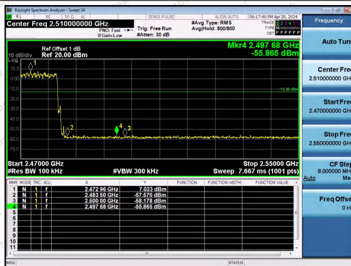
3DH5-Ant2-Hop_2480-PASS
