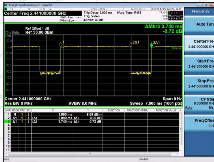
NTNV-3DH5-Ant2-2441
