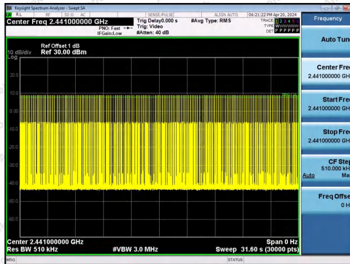
3DH3-Ant2-Hop-PASS
