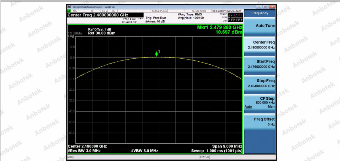
2DH5-Ant2-2480-PASS
