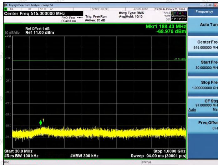
3DH5-Ant2-2402-30~1000-PASS
