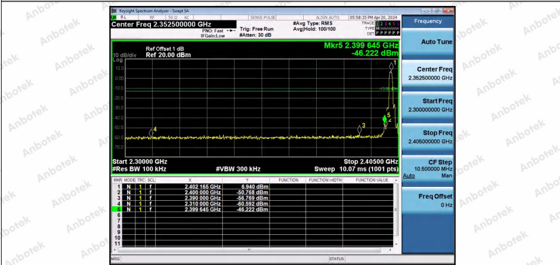
3DH5-Ant2-2402-PASS
