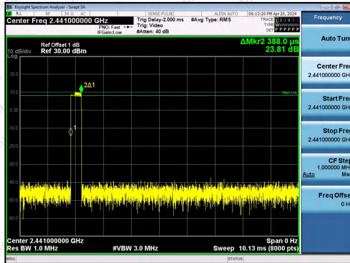
2DH1-Ant2-Hop-PASS
