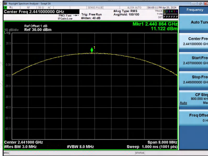
3DH5-Ant2-2441-PASS
