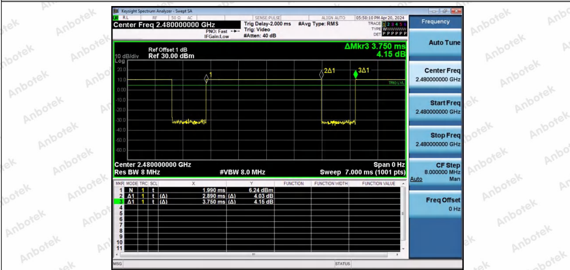
NTNV-DH5-Ant2-2480
