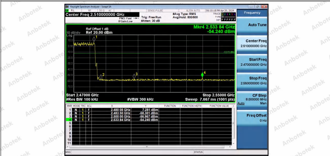
2DH5-Ant2-Hop_2480-PASS
