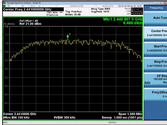
2DH5-Ant2-2441-0~Reference-PASS
