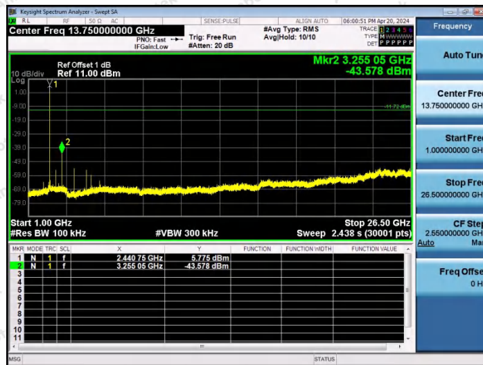
3DH5-Ant2-2441-1000~26500-PASS
