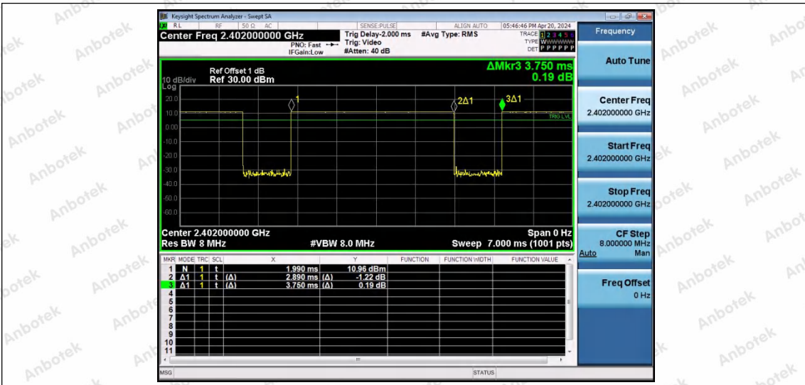
NTNV-DH5-Ant2-2402
