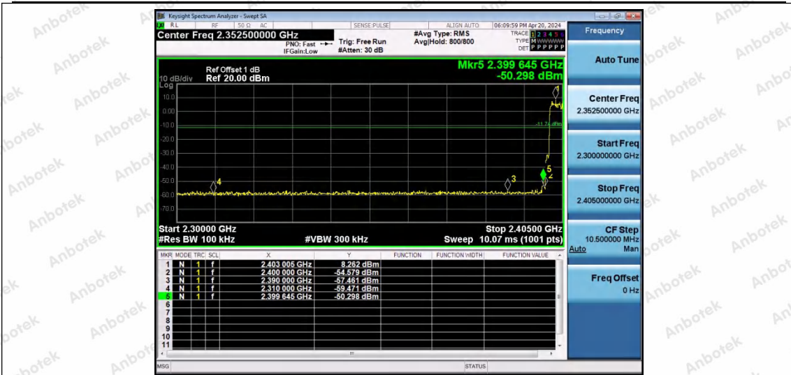
2DH5-Ant2-Hop_2402-PASS
