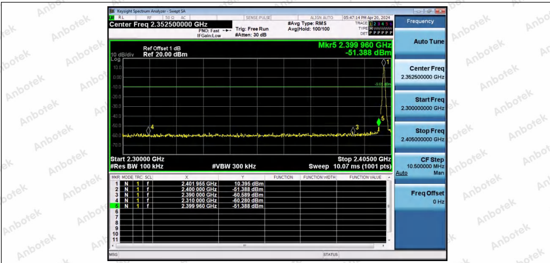
DH5-Ant2-2402-PASS
