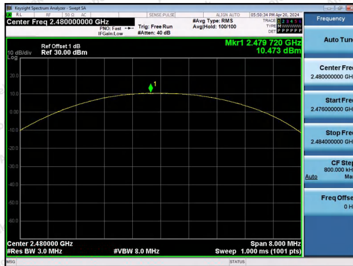
DH5-Ant2-2480-PASS
