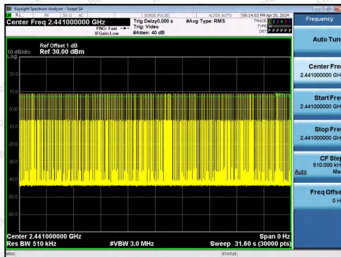
2DH1-Ant2-Hop-PASS
