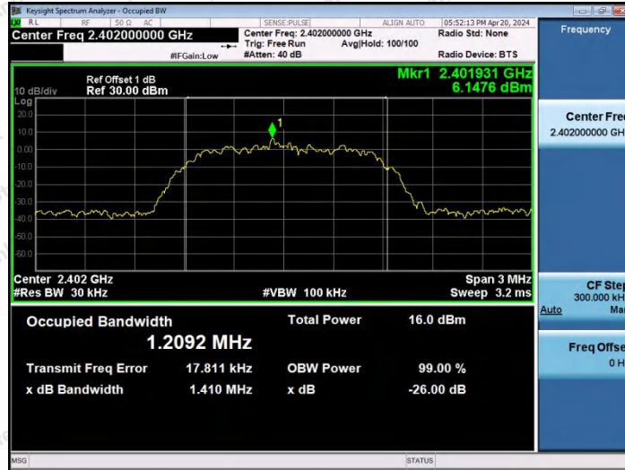
2DH5-Ant2-2402
