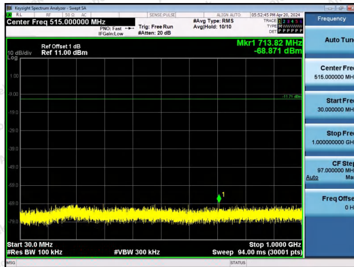
2DH5-Ant2-2402-30~1000-PASS
