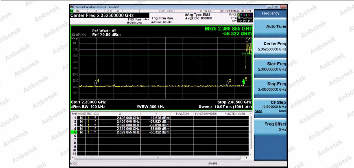
DH5-Ant2-Hop_2402-PASS
