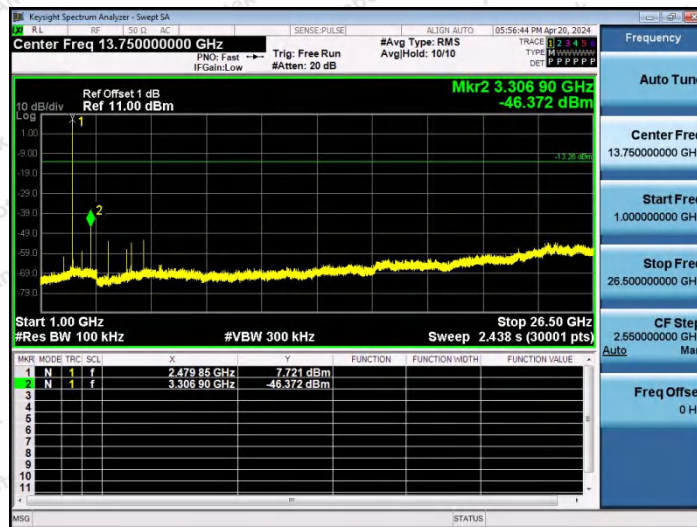
2DH5-Ant2-2480-1000~26500-PASS
