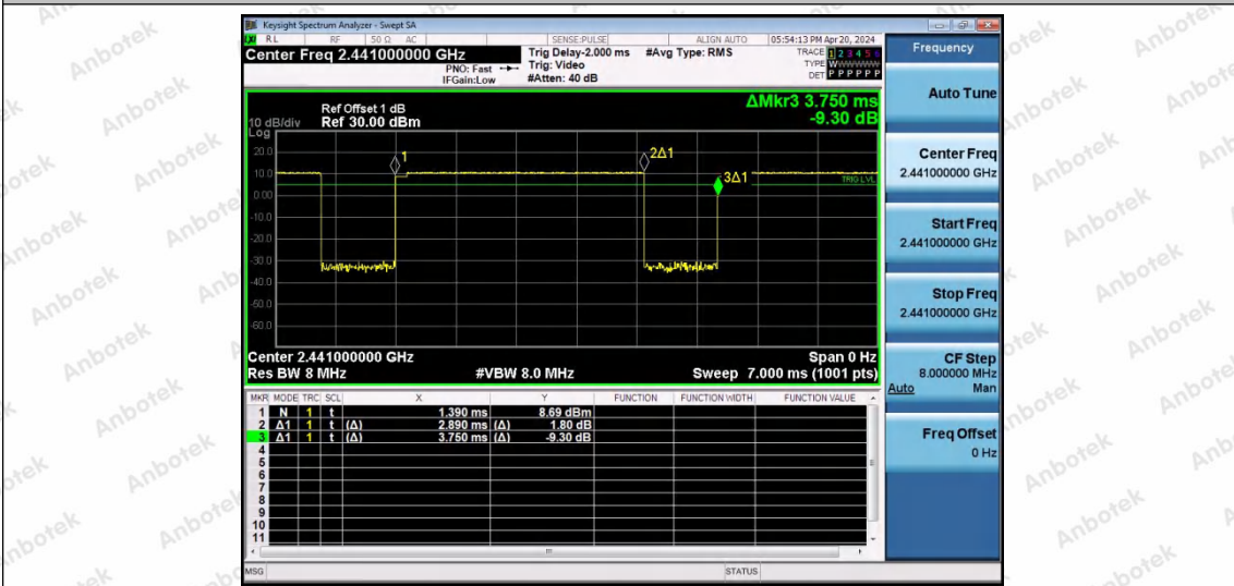
NTNV-2DH5-Ant2-2441
