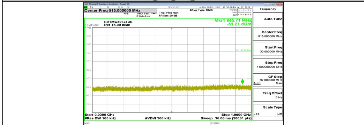
LE 1M_Ant1_2440_30~1000
