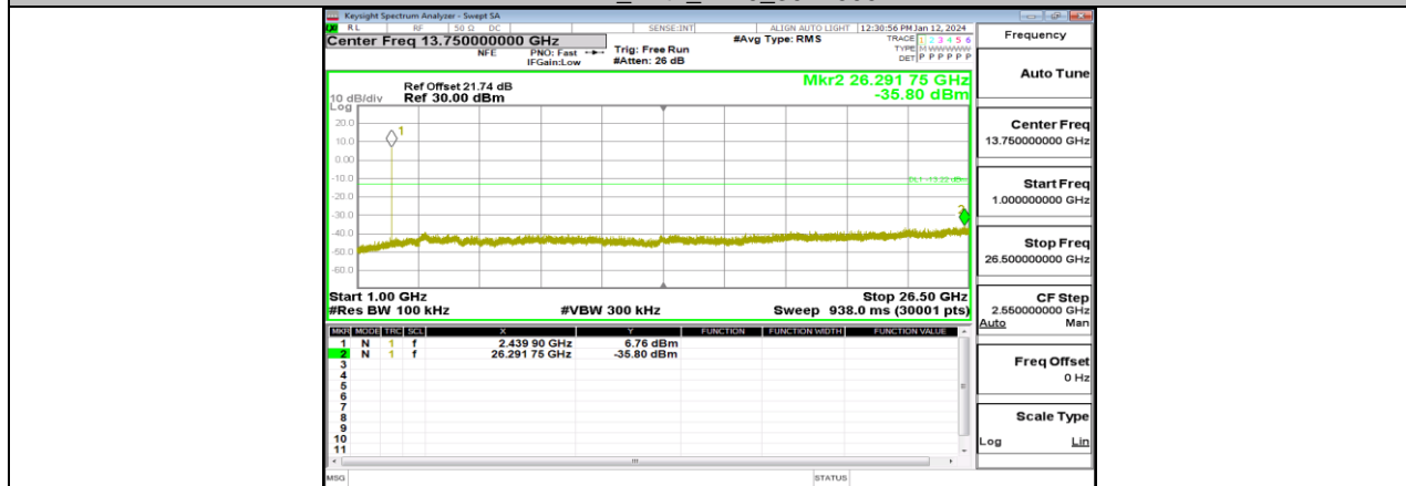
LE 1M_Ant1_2440_1000~26500
