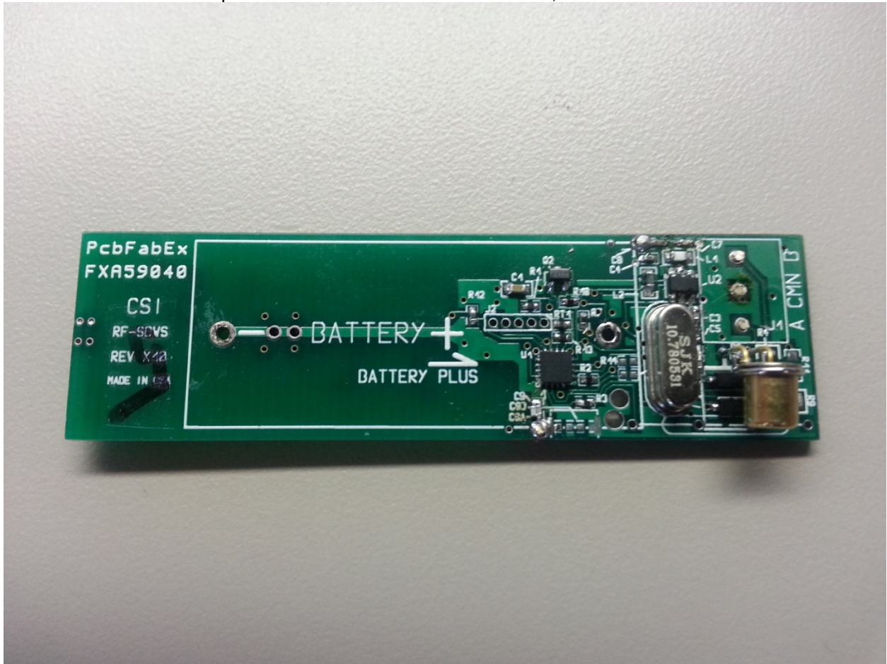
Top Parts Removed Model MSS-RFS-200, MSS-RFS-300
