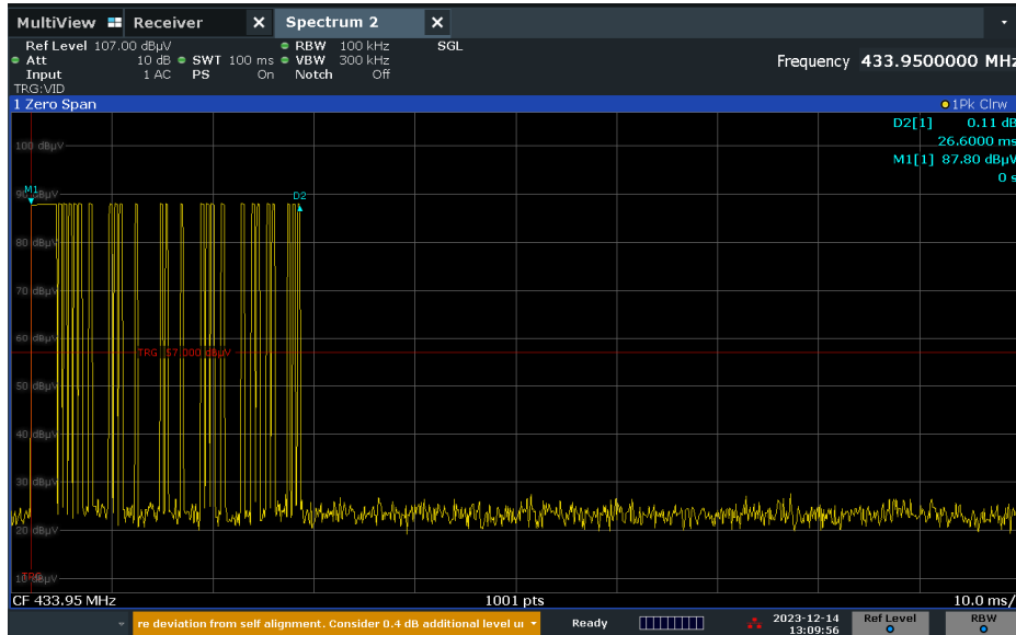
Figure 2-2 – Pulse within 100ms
