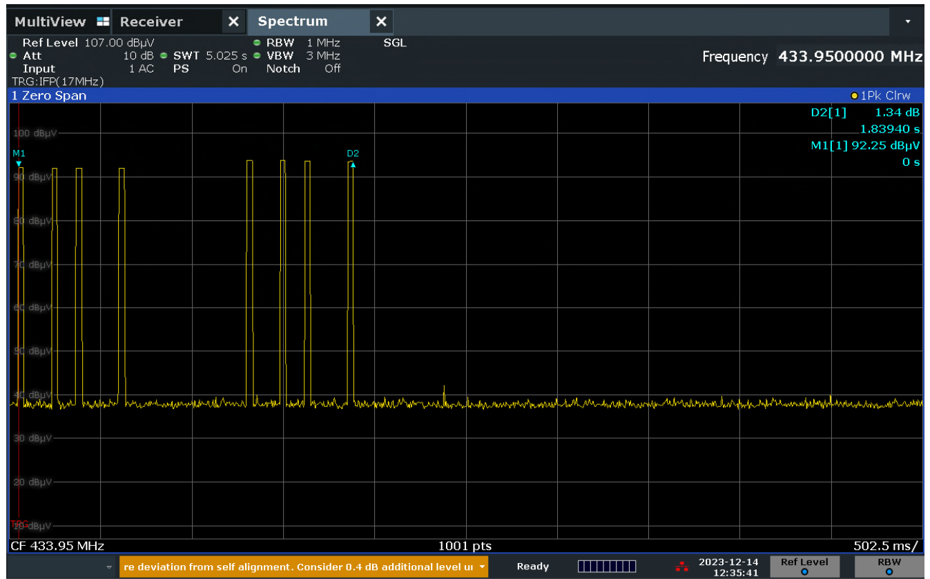
Figure 2-1 – Deactivation Period
