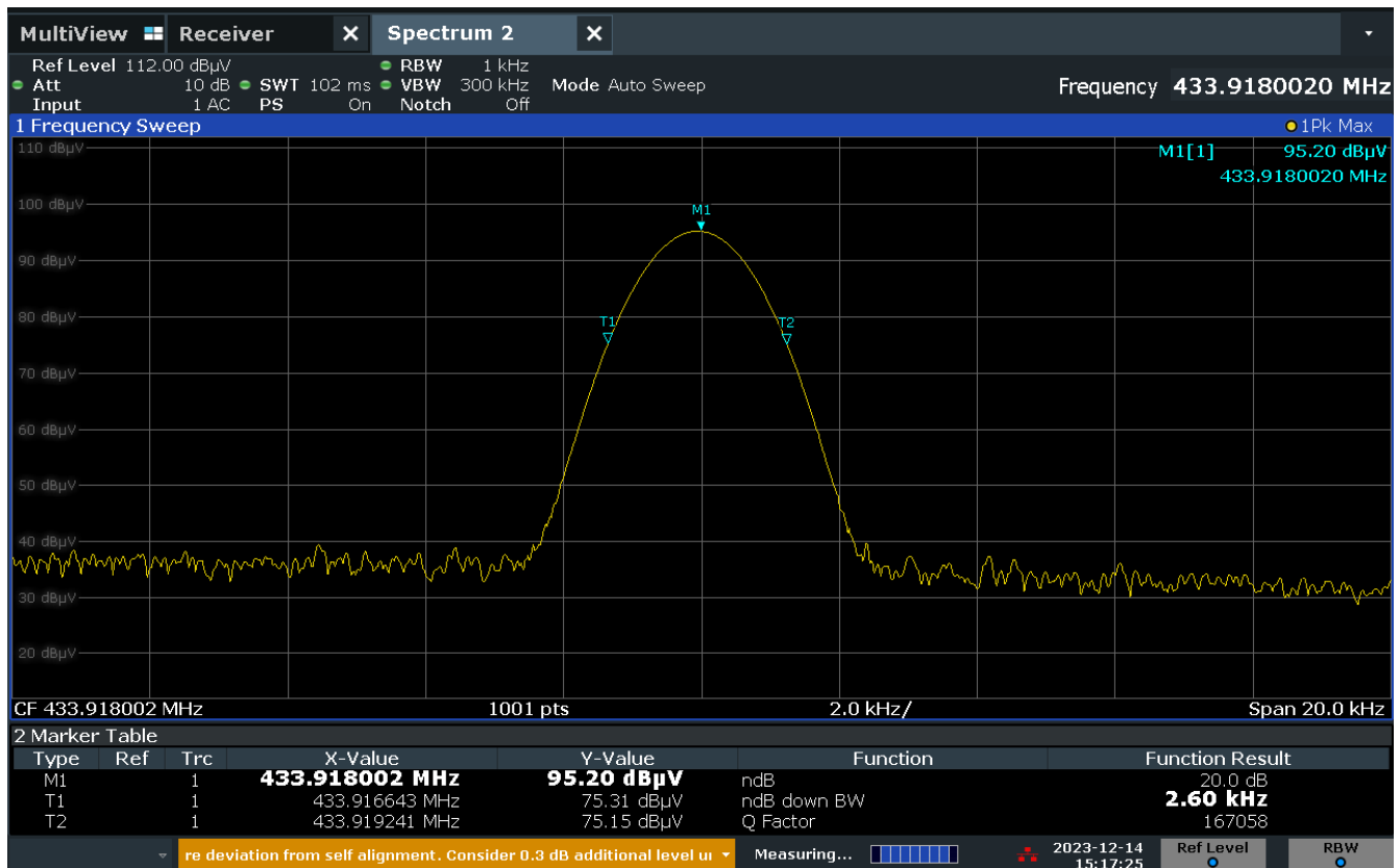
Figure 2-11 – Occupied Bandwidth
