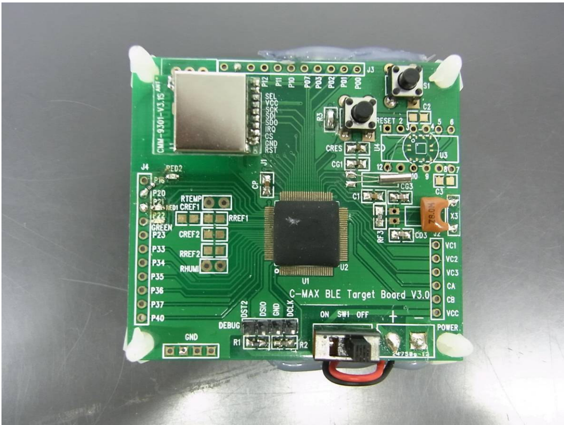
Module with demo board (Top side)
