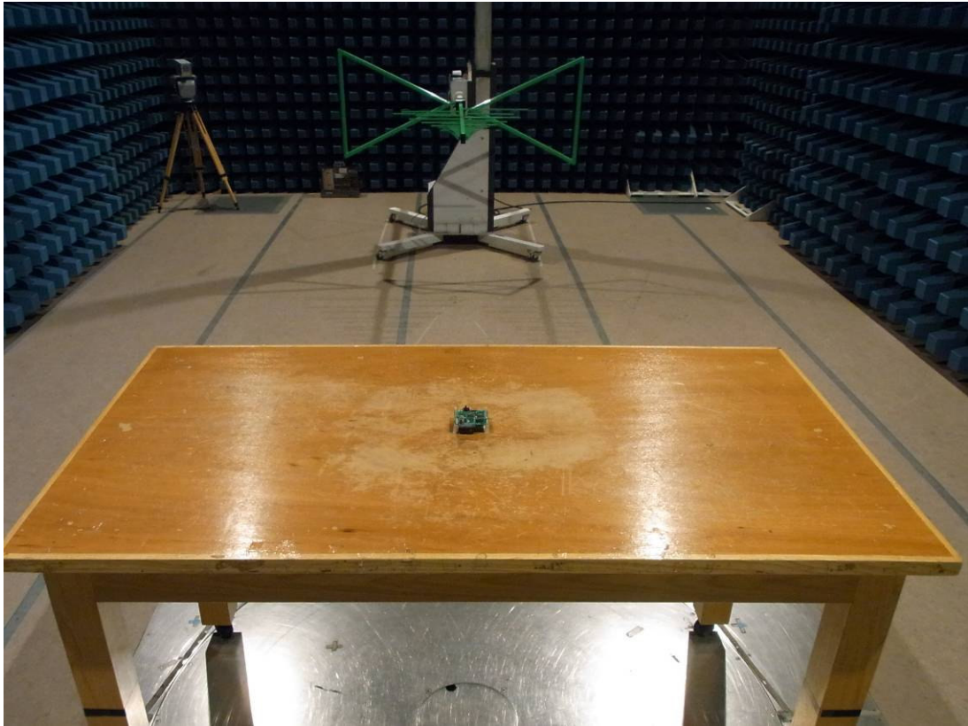
30MHz-1GHz (front view)
