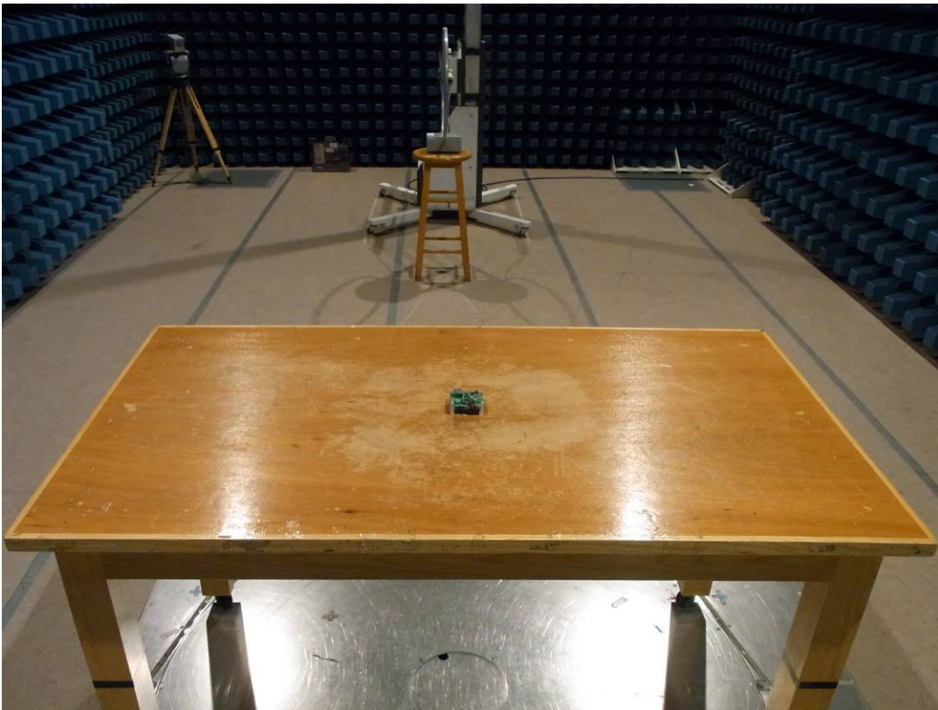
9kHz – 30MHz (back view)
