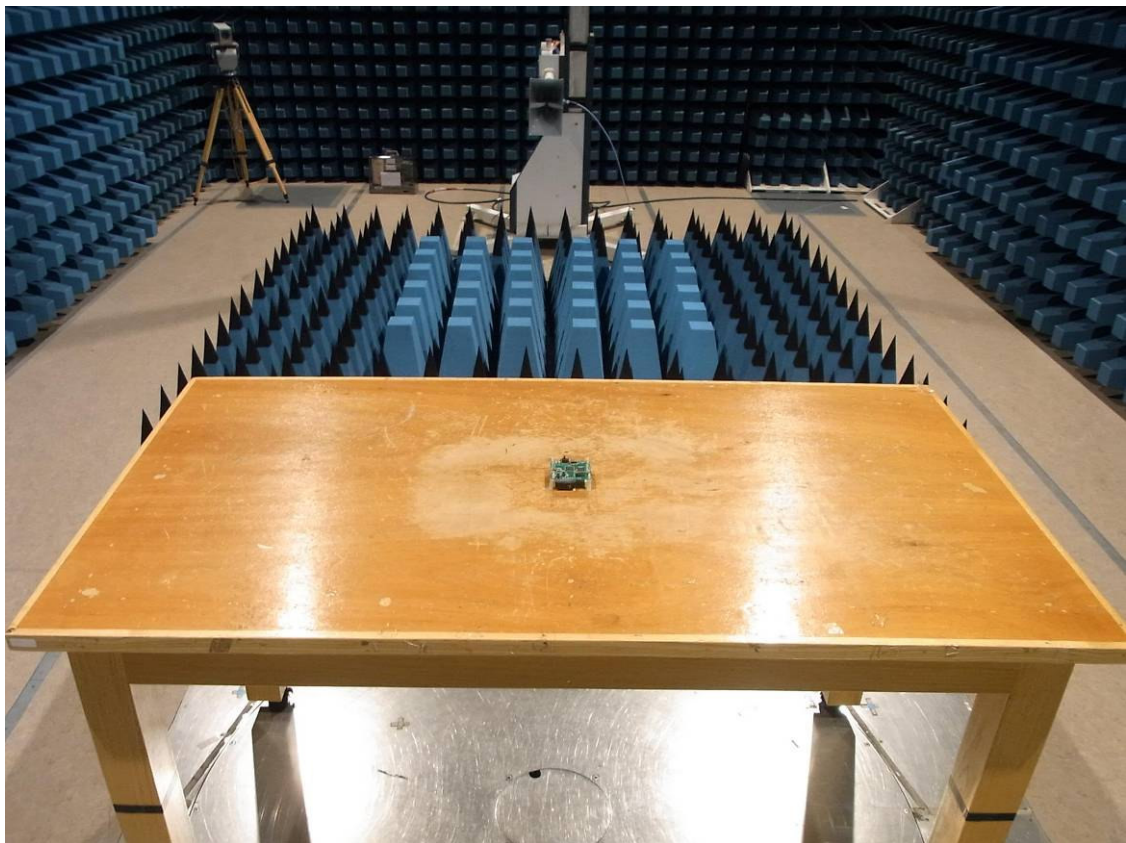
1GHz-25GHz (back view)
