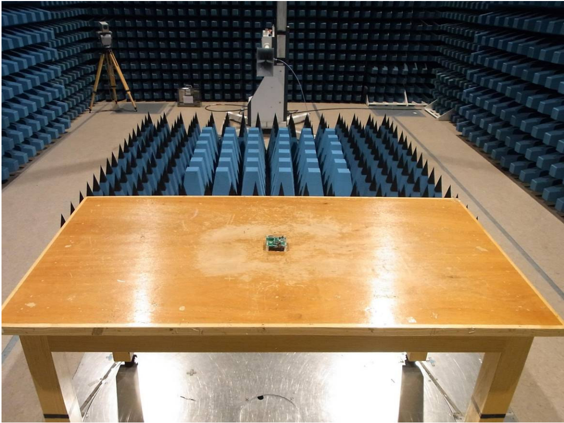
1GHz-25GHz (front view)
