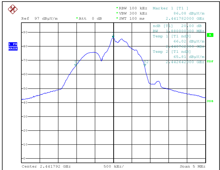
Bandwidth 2 (2442MHz)
