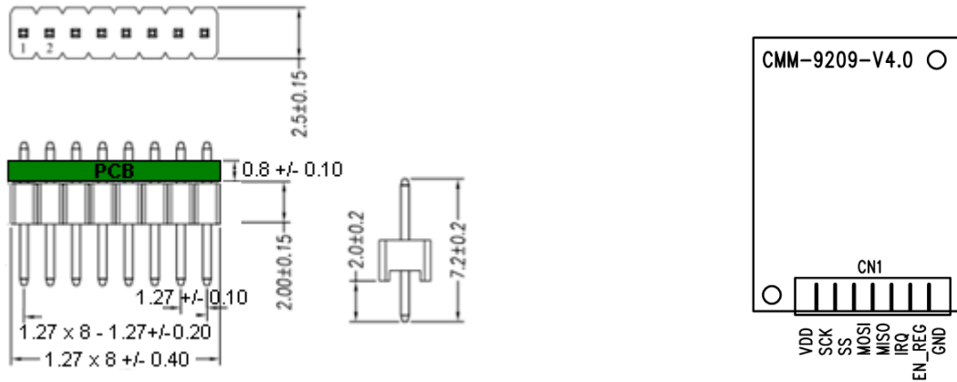
Pin Connection Dimension (applicable only for CMM-9209-V4.0P/4.0X)
