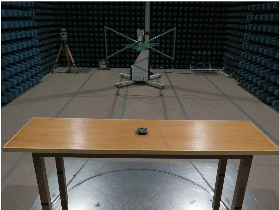
Rear view (30Mz – 1GHz)
