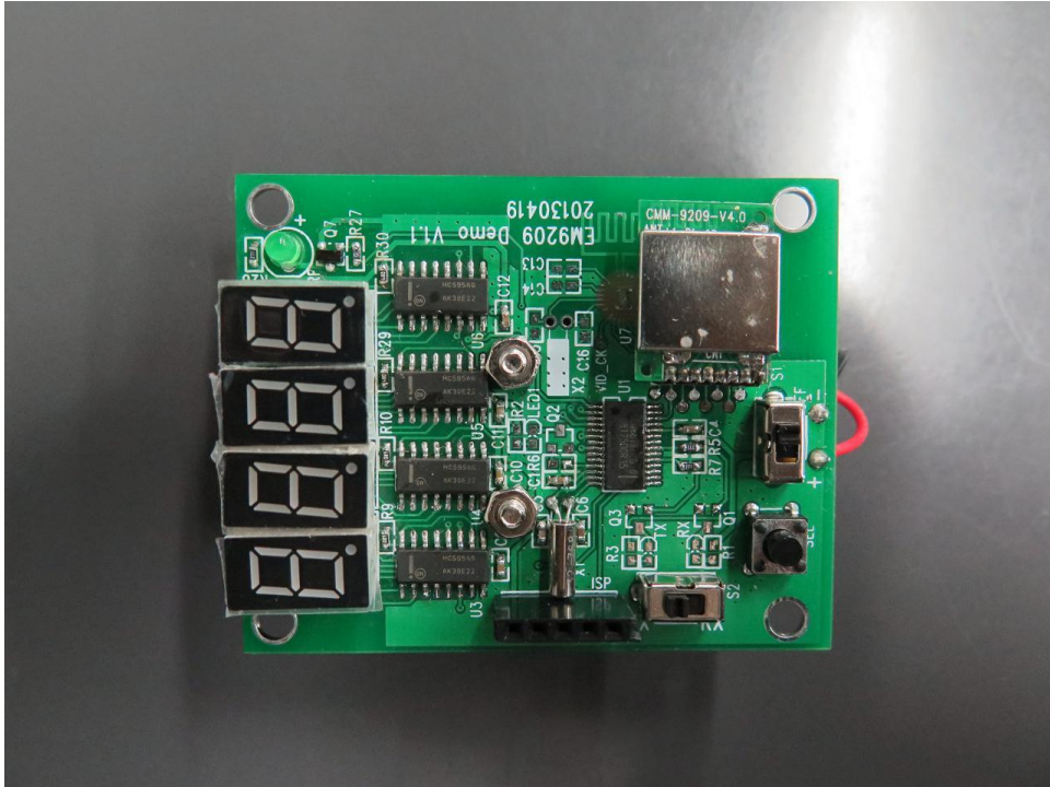
EUT with control board (top view)
