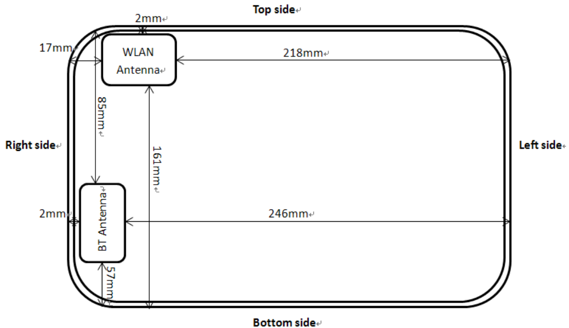
Figure 2: The antenna positions of the DUT
