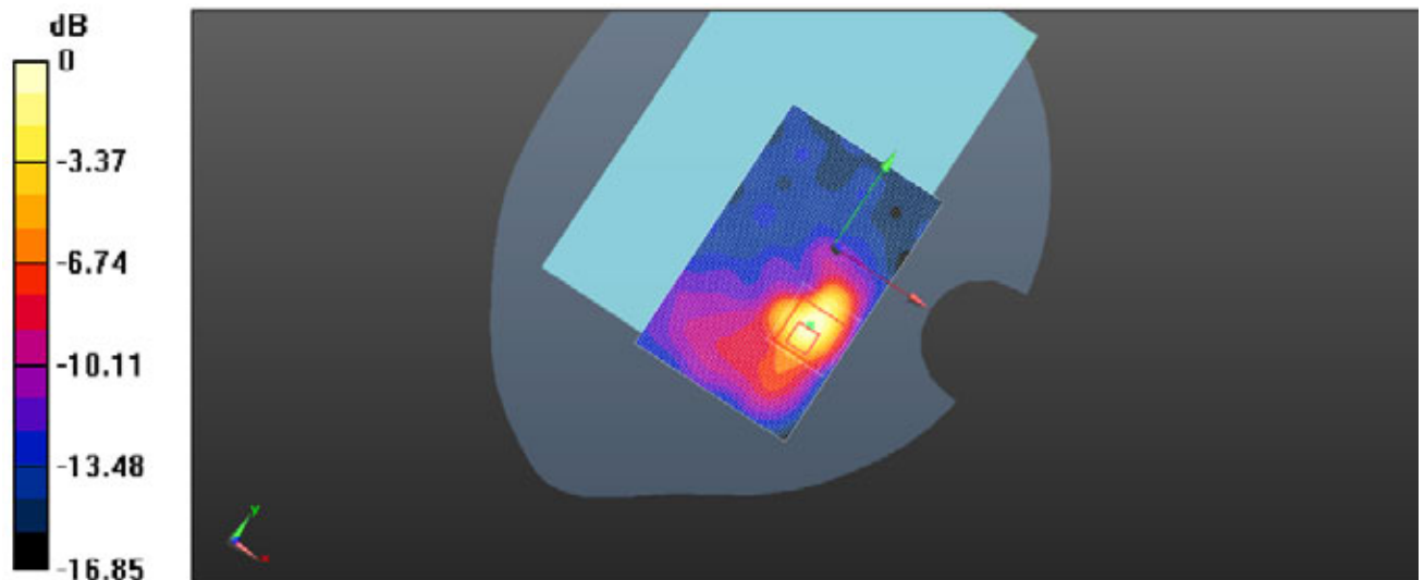
Plot 1: Rear Side (WLAN2450-Middle Channel-Channel 6-2437MHz(1Mbps))
