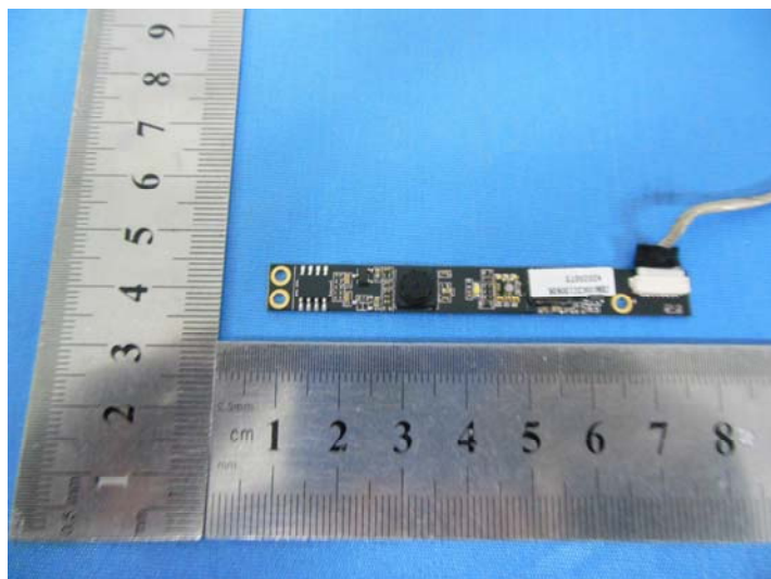
EUT –Second Camera PCB View
