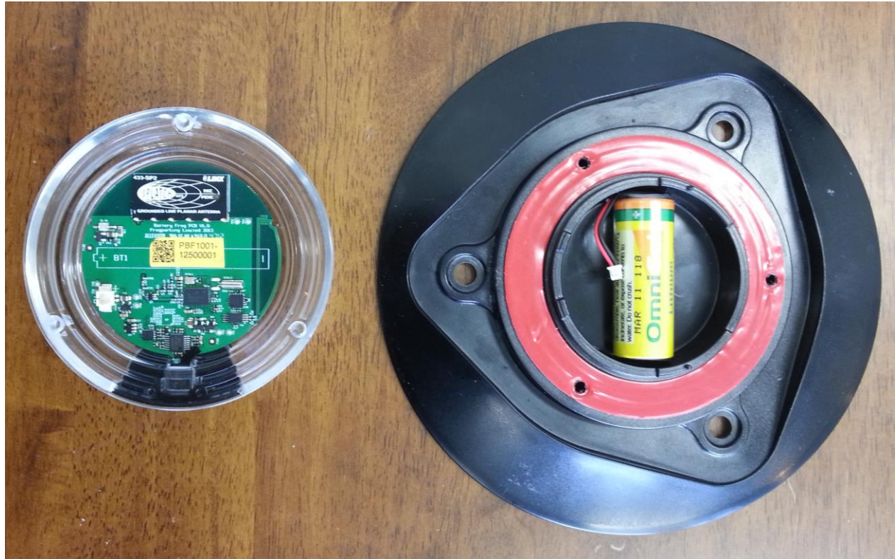
Figure 9 - Frog Main Board and IR Insert Tab inserted, Battery and Tape Seal fitted
