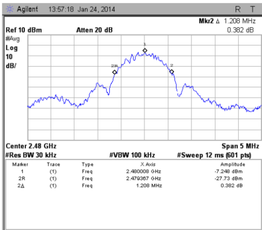
Figure 28: Operation within the Bands - Conducted – Channel 39
