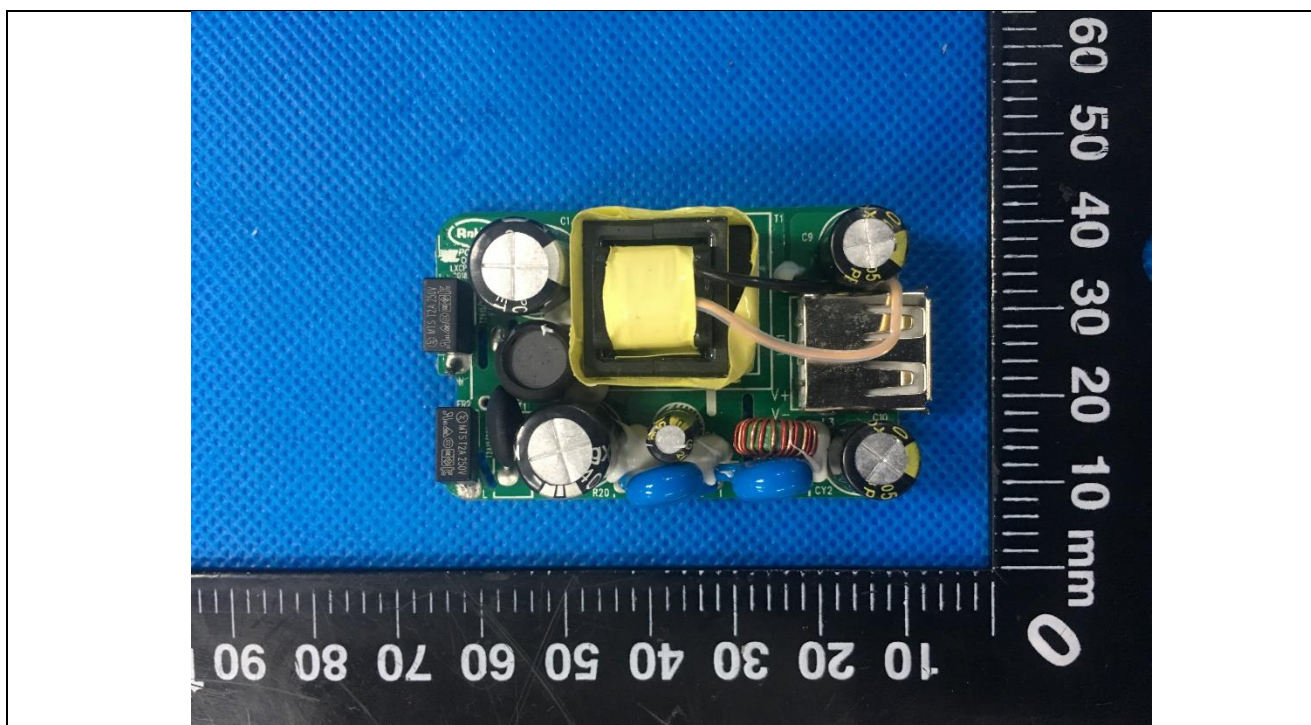
Details of: PCB view 1 of Medical Adapter
