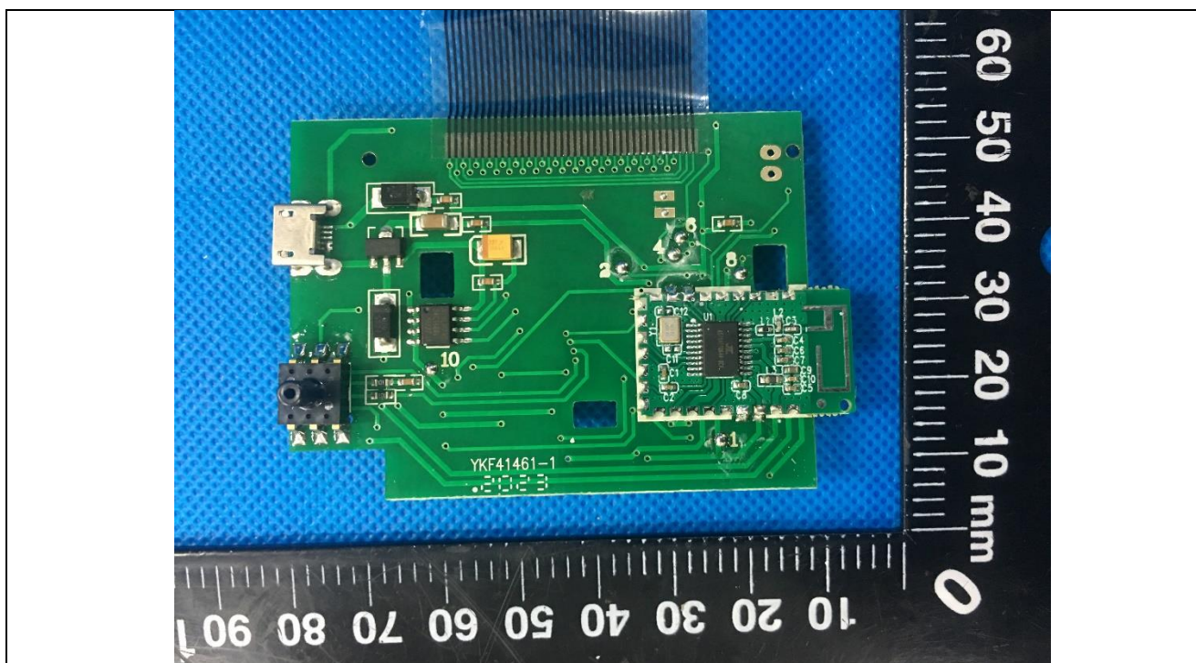
Details of: PCB view 2 of main unit (M/N: MD5990)
