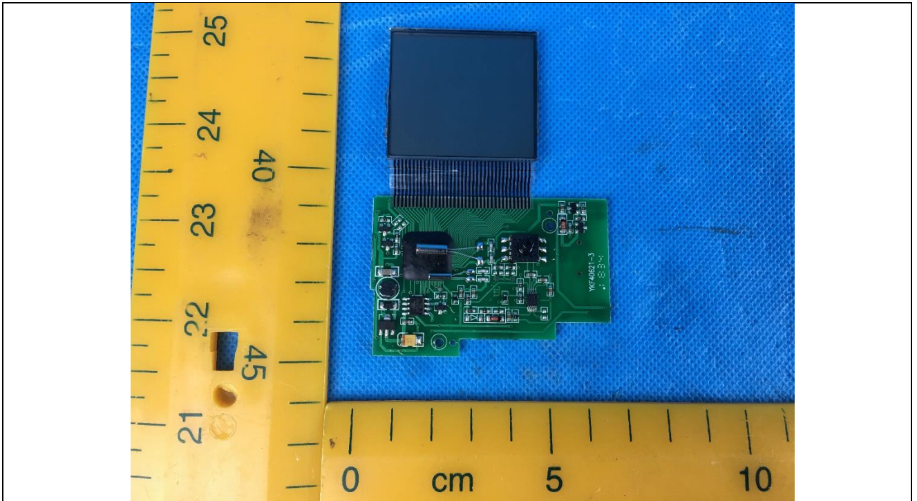
Details of: Digital Automatic Blood Wrist Pressure Monitor PCB view 4
