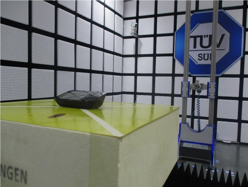
Radiated Emission test 18-25GHz
