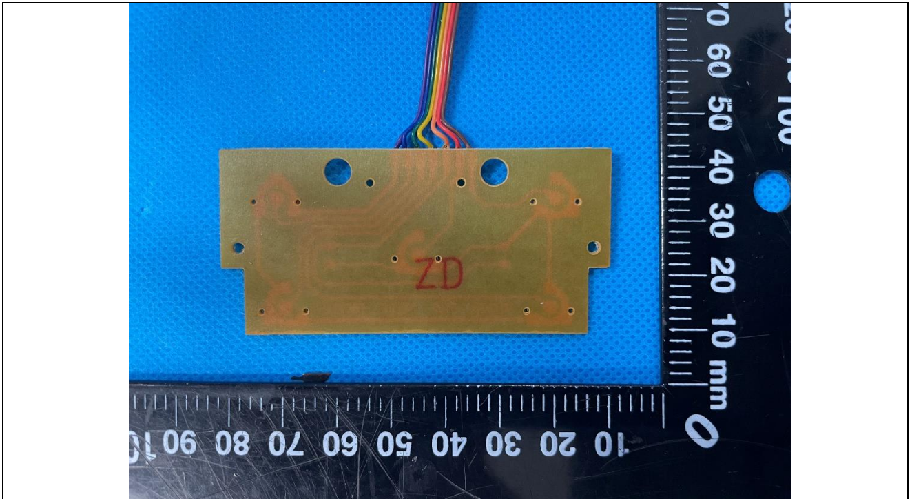
Details of: PCB view 3 of main unit (M/N: MD3610B)
