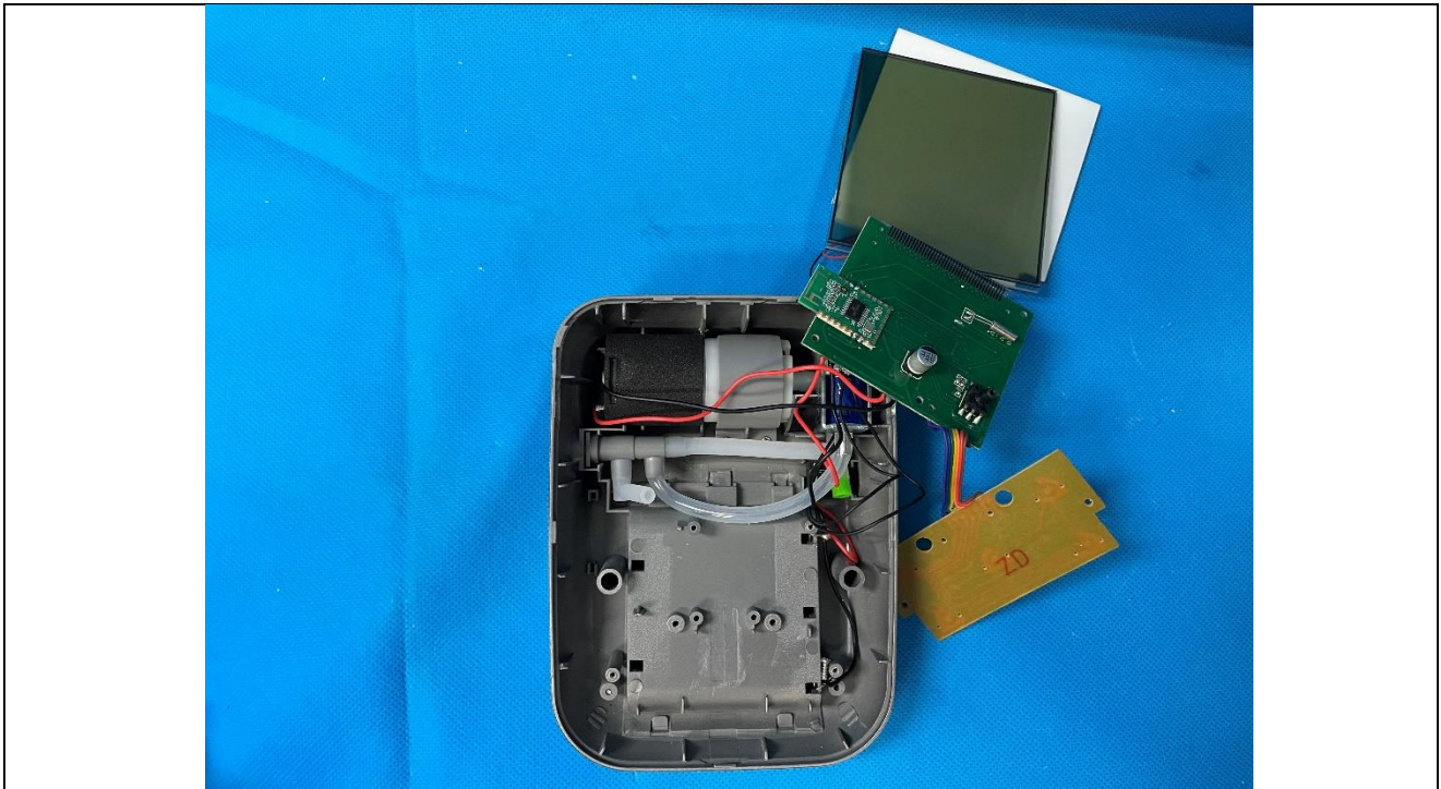
Details of: PCB view 1 of main unit (M/N: MD3610B)
