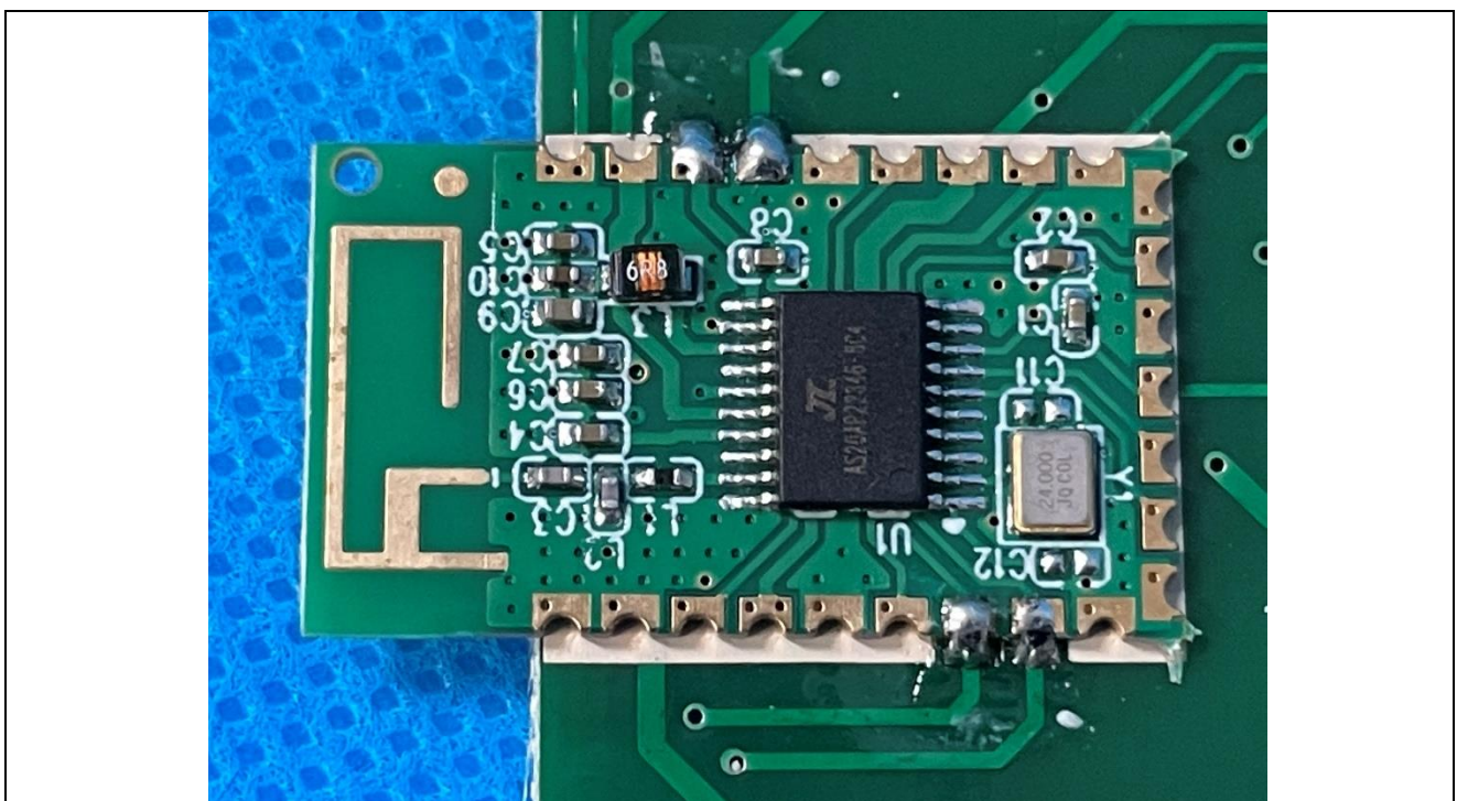
Details of: Bluetooth view of main unit (M/N: MD3610B)
