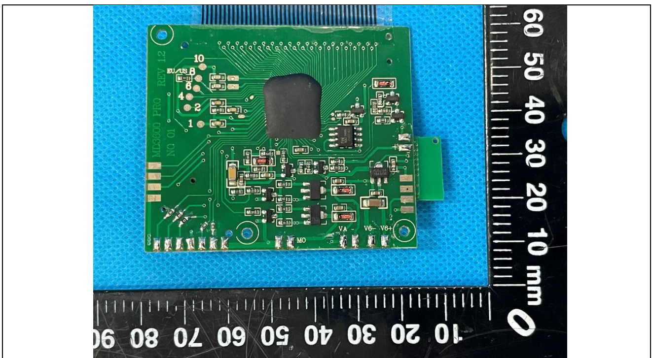
Details of: PCB view 5 of main unit (M/N: MD3610B)
