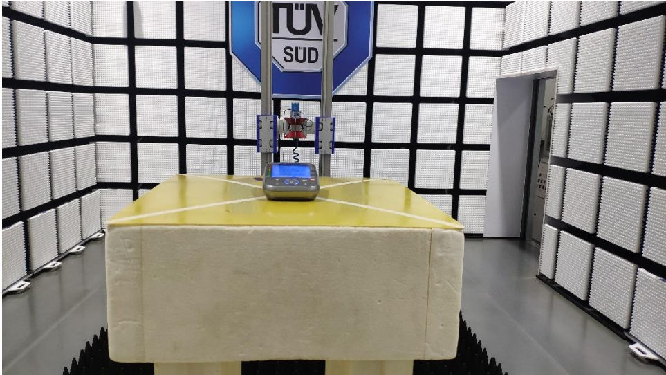
Radiated Emission test 18-25GHz
