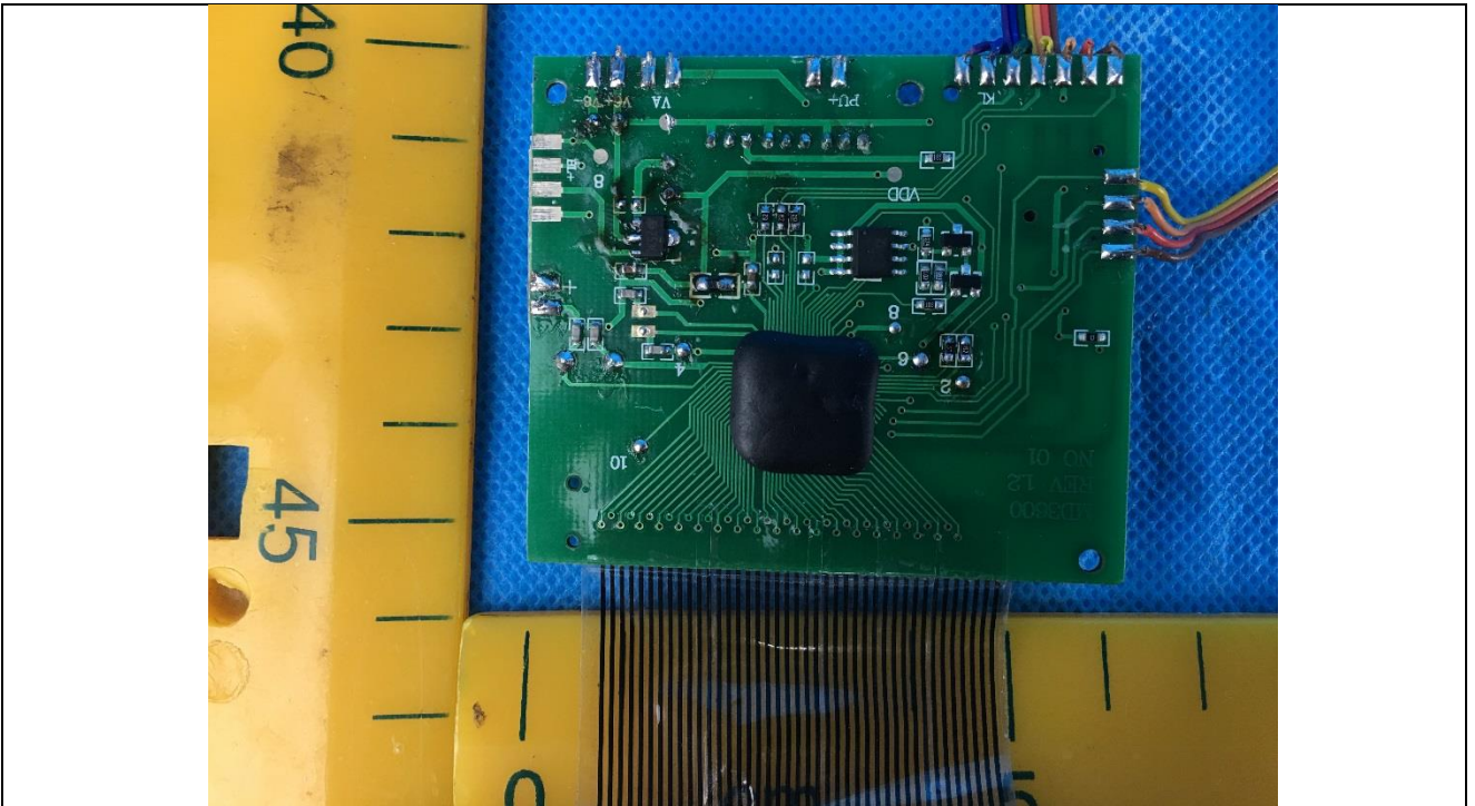
Details of: Digital Automatic Blood Pressure Monitor PCB view 3
