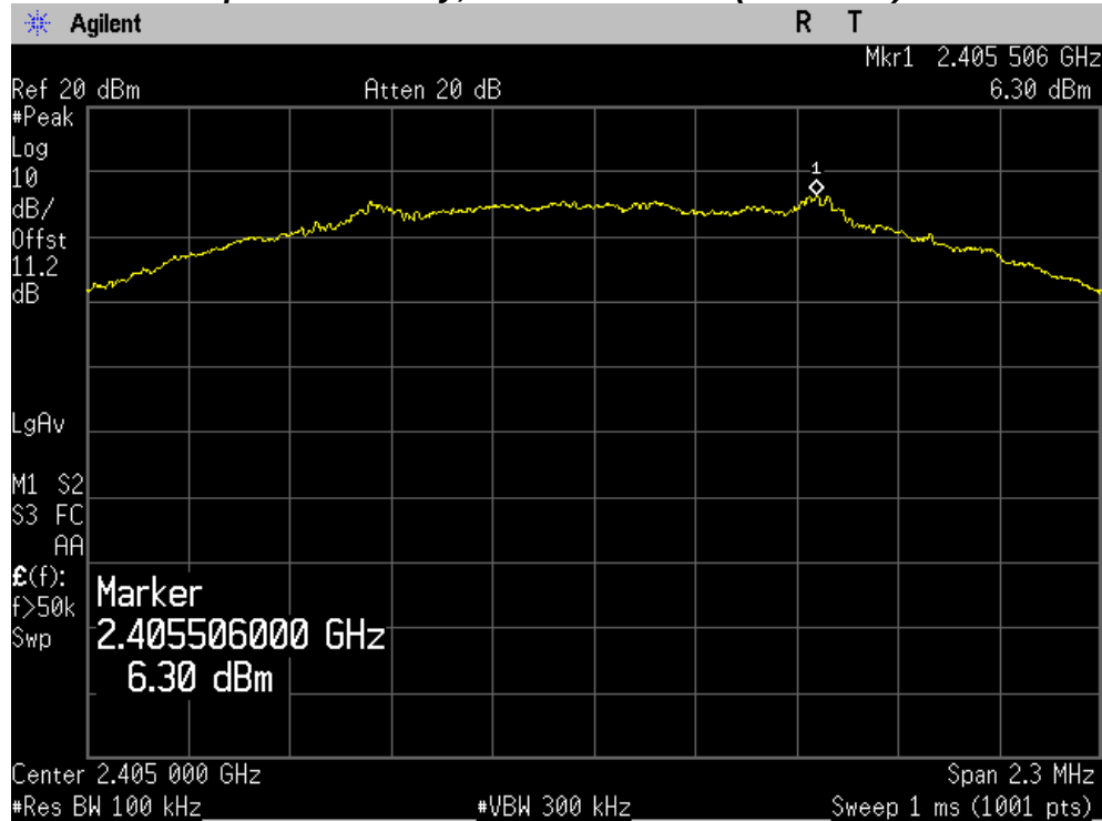
Peak Power Spectral Density, Lowest Channel (2405 MHz)
