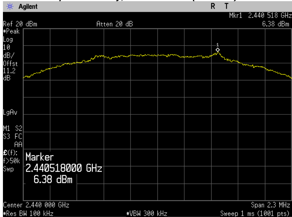
Peak Power Spectral Density, Middle Channel (2440 MHz)
