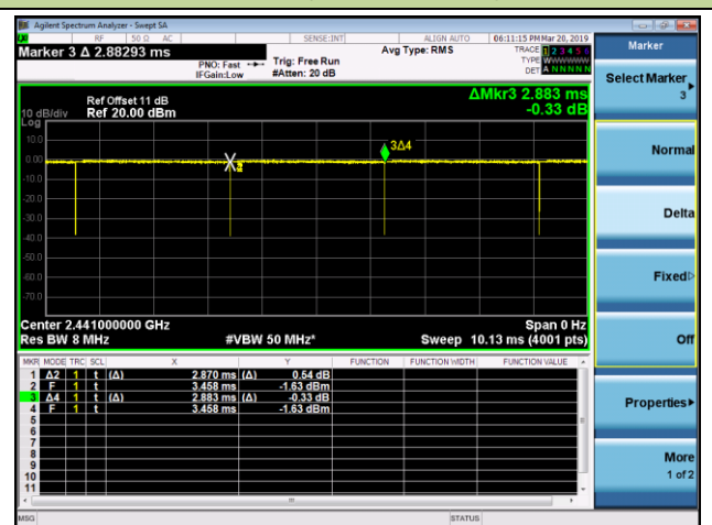
2DH5 (T = 2.870ms)
