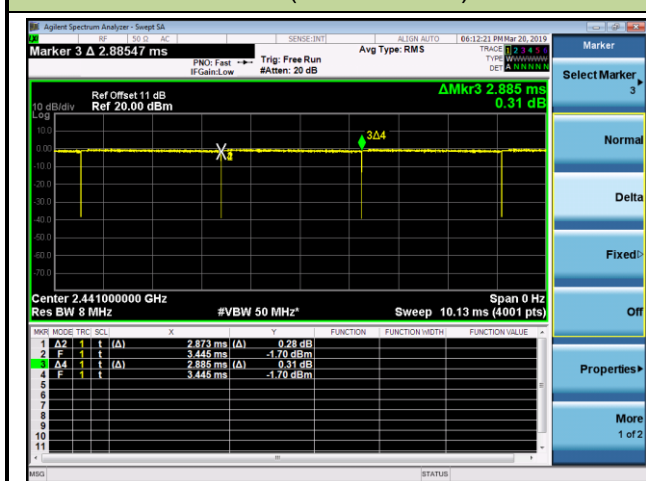
3DH5 (T = 2.873ms)
