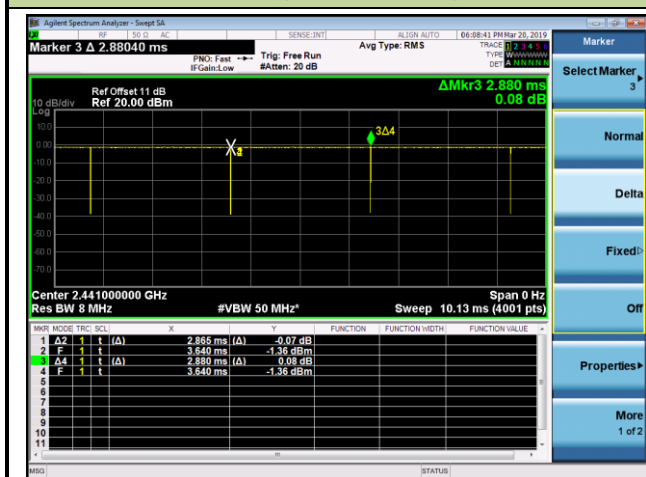
3DH5 (T = 2.873ms)
