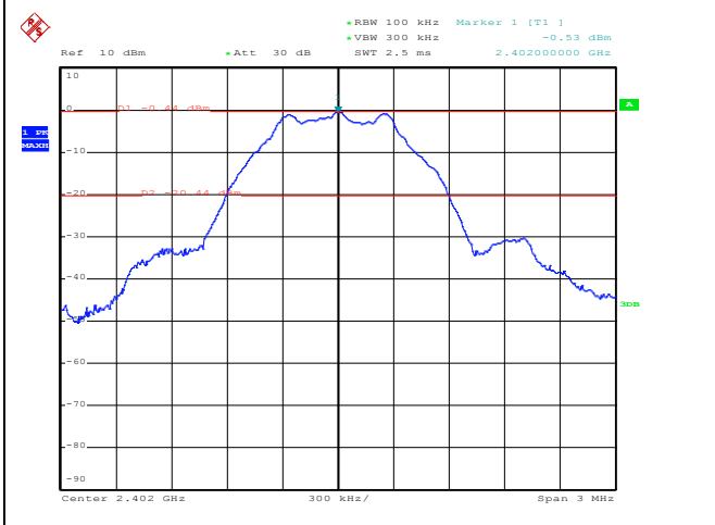
2401 – 2403 MHz
