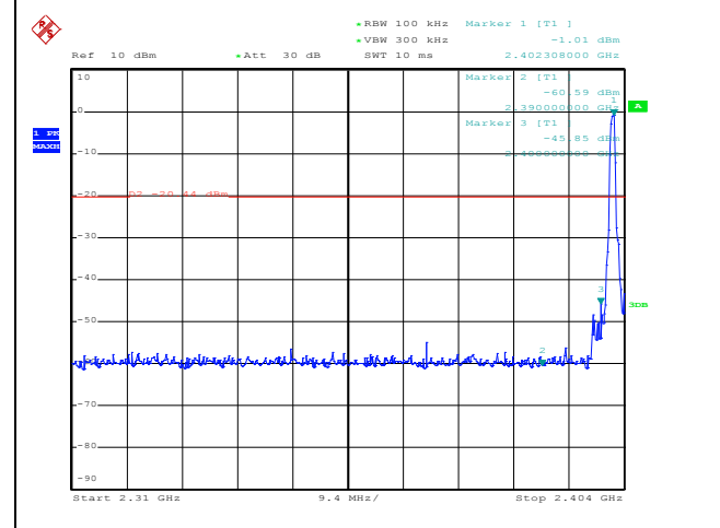
Channel 0 / 2402 MHz
