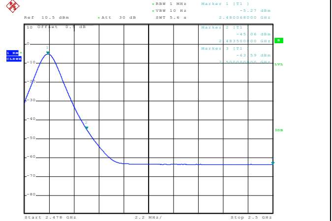
Channel 78 / 2480 MHz –Average
