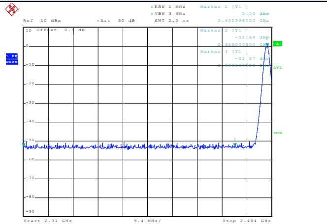
Channel 0 / 2402 MHz – Peak
