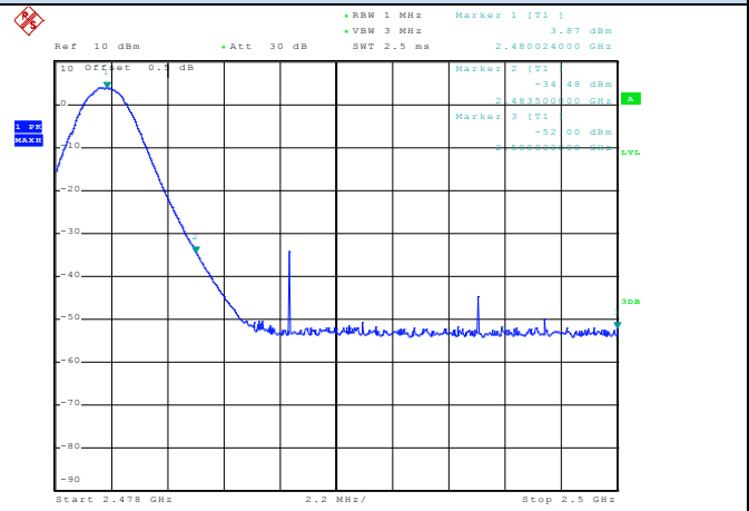
Channel 78 / 2480 MHz – Peak
