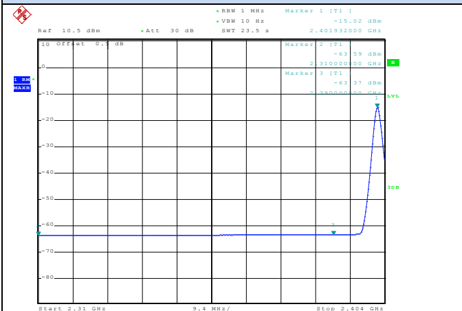
Channel 0 / 2402 MHz –Average
