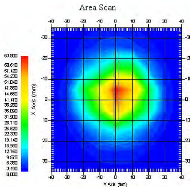
2450 MHz System Validation with Head Tissue
