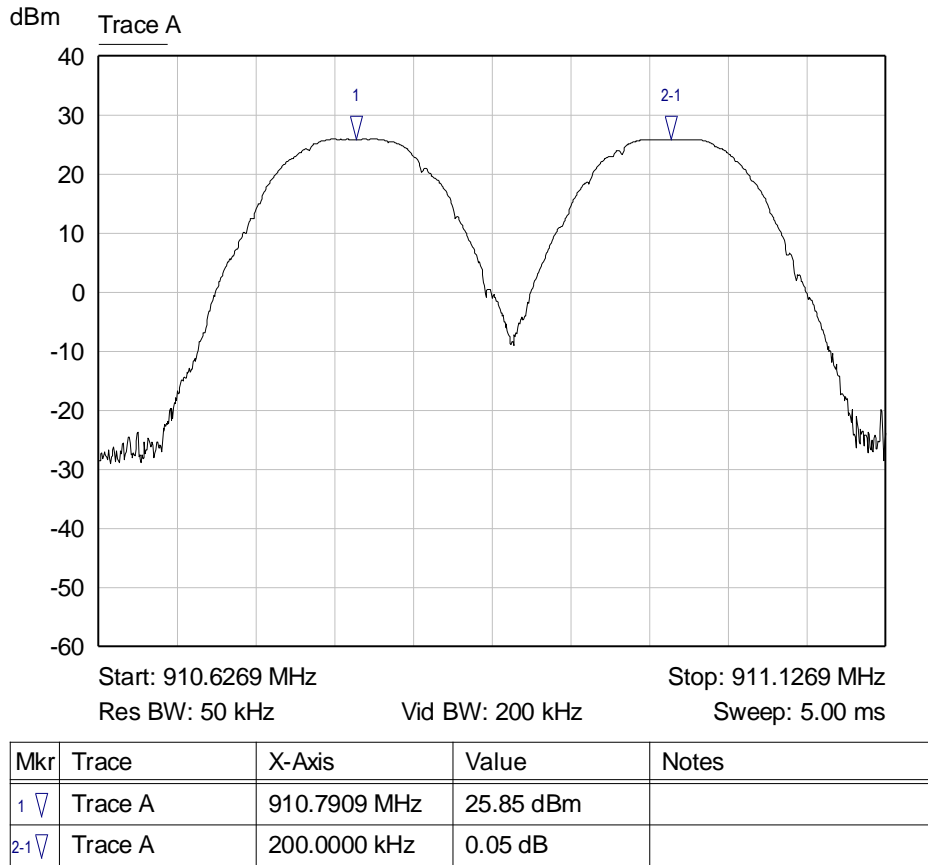
Graph 1: Channel Separation Plot
