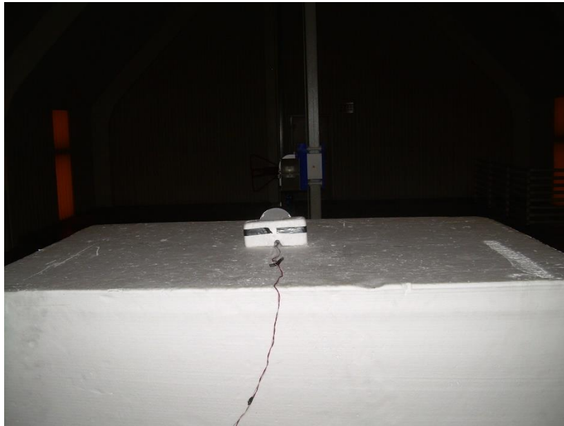
Photograph 4: Back View Radiated Emissions Configuration – Above 1000 MHz
