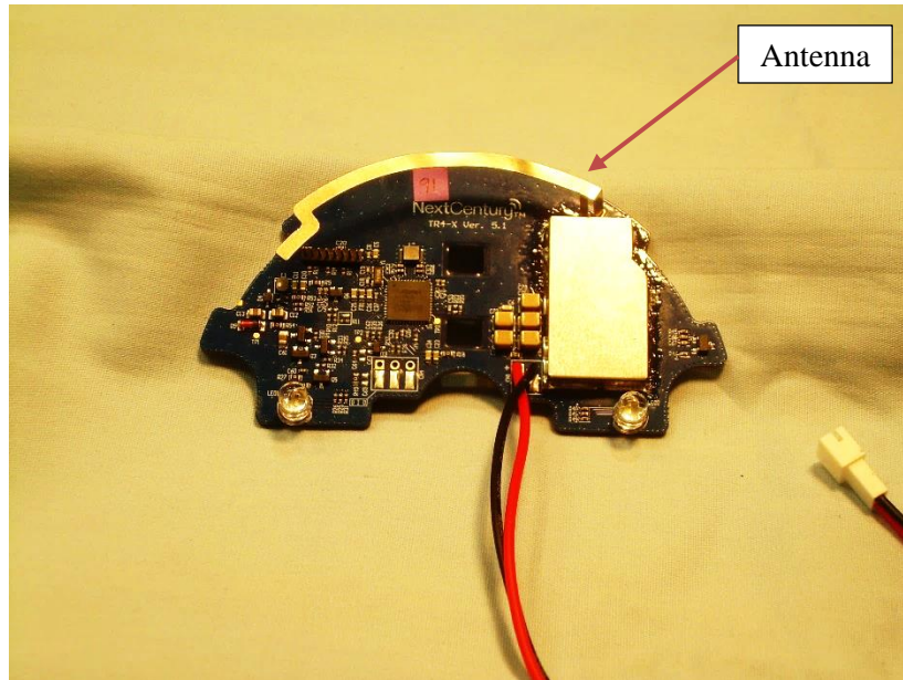
Photograph 13: Front Side of the PCB – RF Shield In Place
