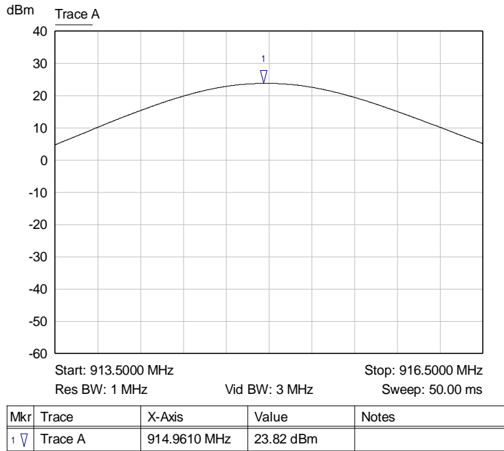
Graph 8: Transmitting at the Middle Channel
