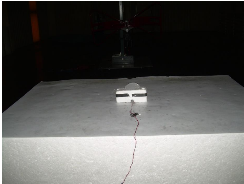
Photograph 2: Back View Radiated Emissions Configuration – 30 to 1000 MHz
