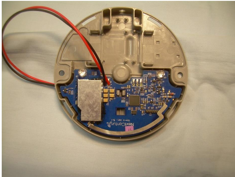
Photograph 12: Cover Removed Showing EUT Without Weather-Proofing
