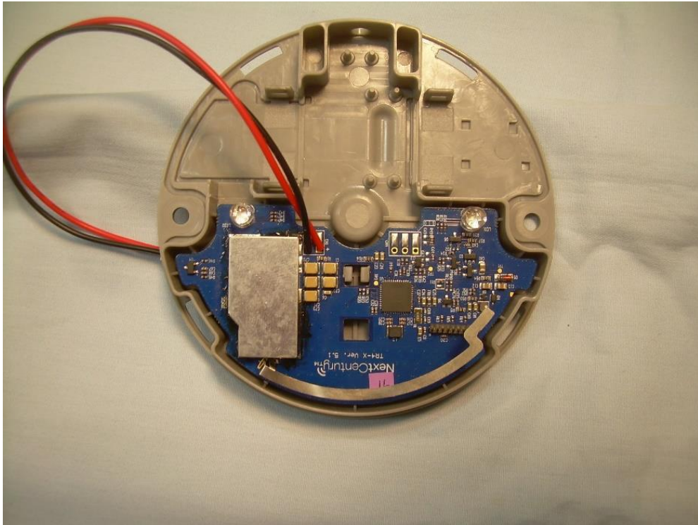
Photograph 7 – PCB Placement View
