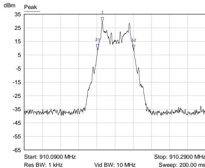
Graph 4: Antenna 0 – Highest Channel 20 dB Bandwidth
