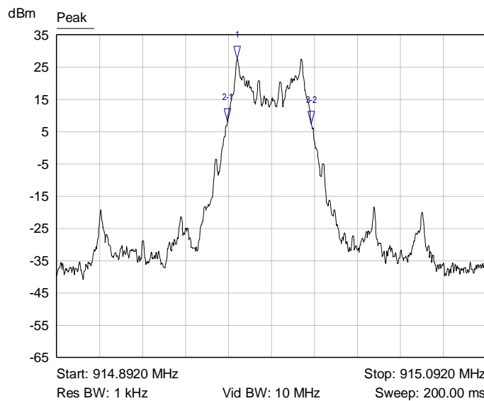
Graph 2: Antenna 0 – Lowest Channel 20 dB Bandwidth
