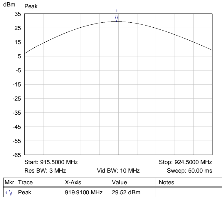
Graph 15: Antenna 1 – Highest Channel Peak Power Plot
