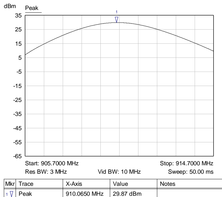
Graph 10: Antenna 0 – Lowest Channel Peak Power Plot
