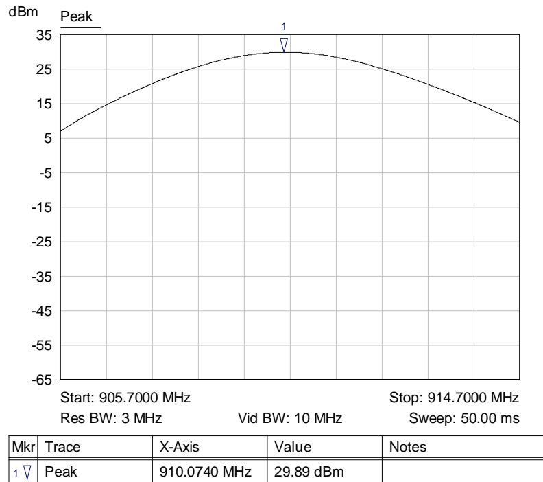
Graph 13: Antenna 1 – Lowest Channel Peak Power Plot
