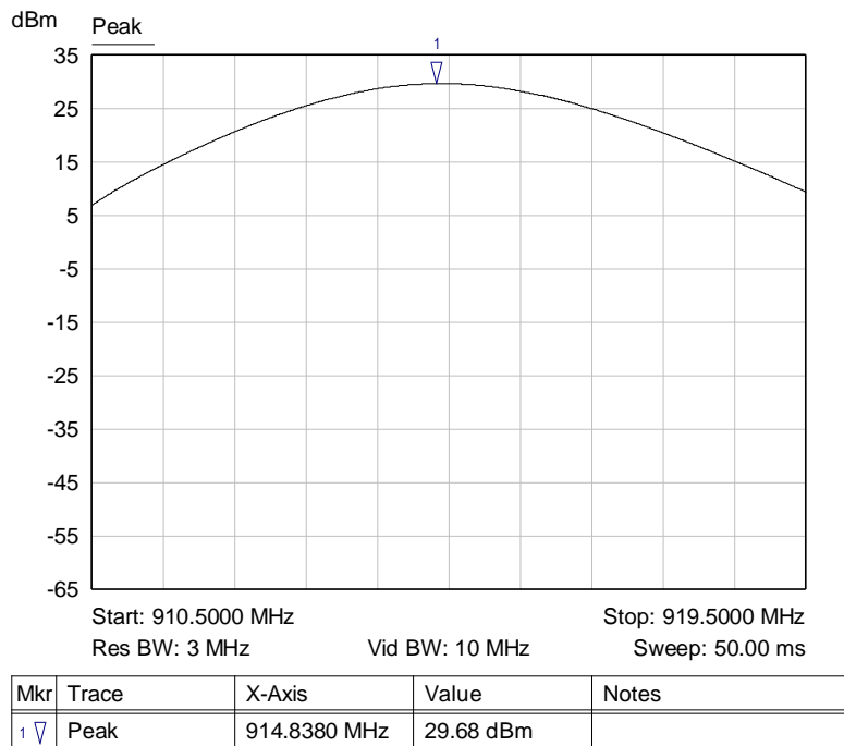
Graph 14: Antenna 1 – Middle Channel Peak Power Plot
