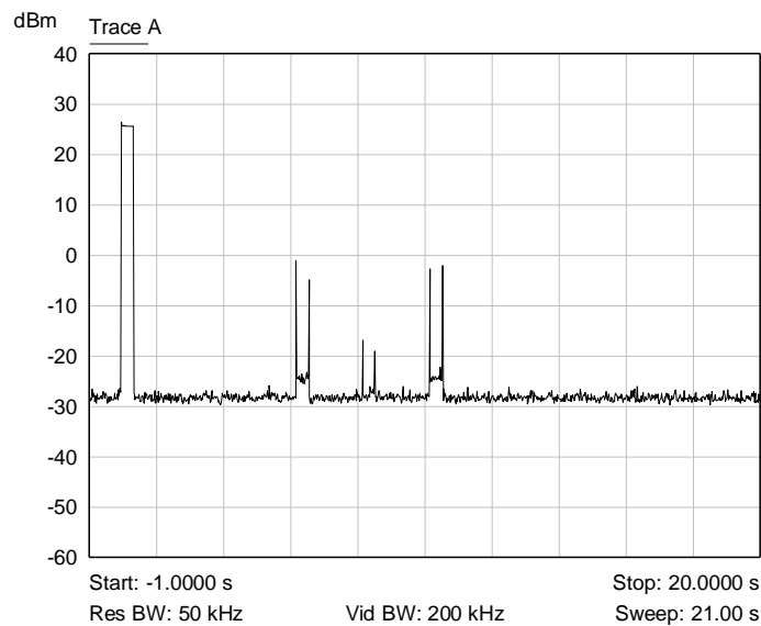
Graph 8: Timing Plot Showing Channel Hits
