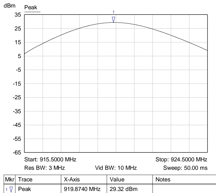
Graph 12: Antenna 0 – Highest Channel Peak Power Plot
