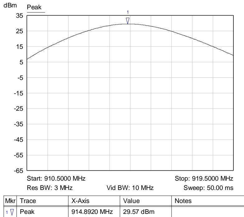
Graph 11: Antenna 0 – Middle Channel Peak Power Plot
