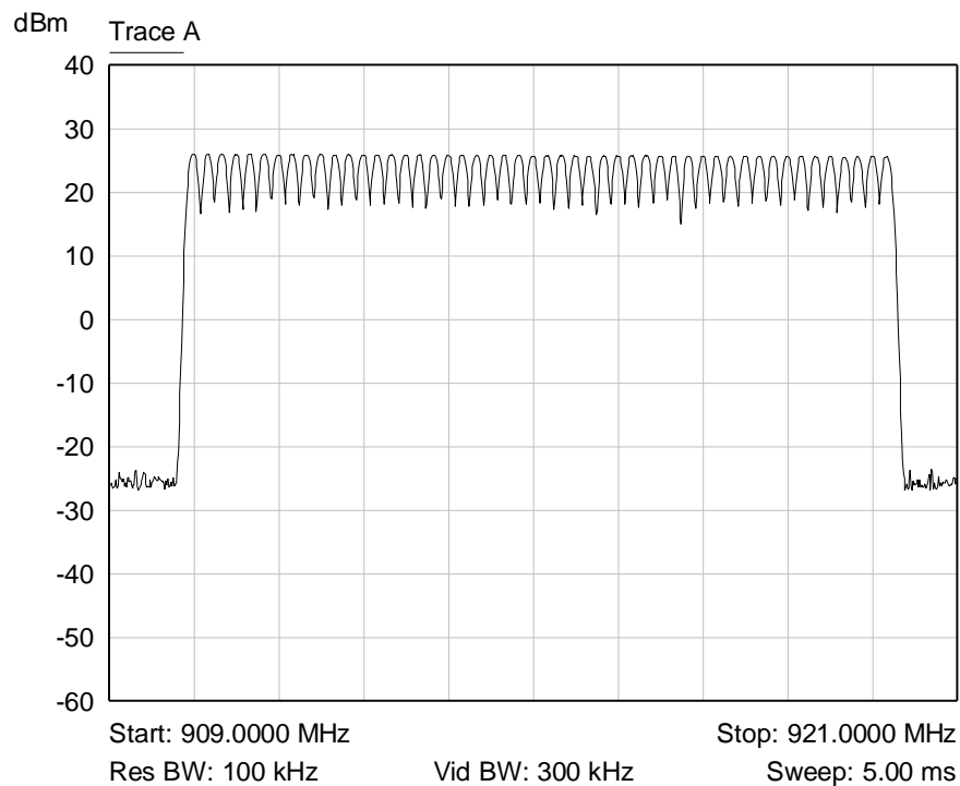
Graph 16: Plot Showing All Channels Operate Within the Authorized Frequency Band
