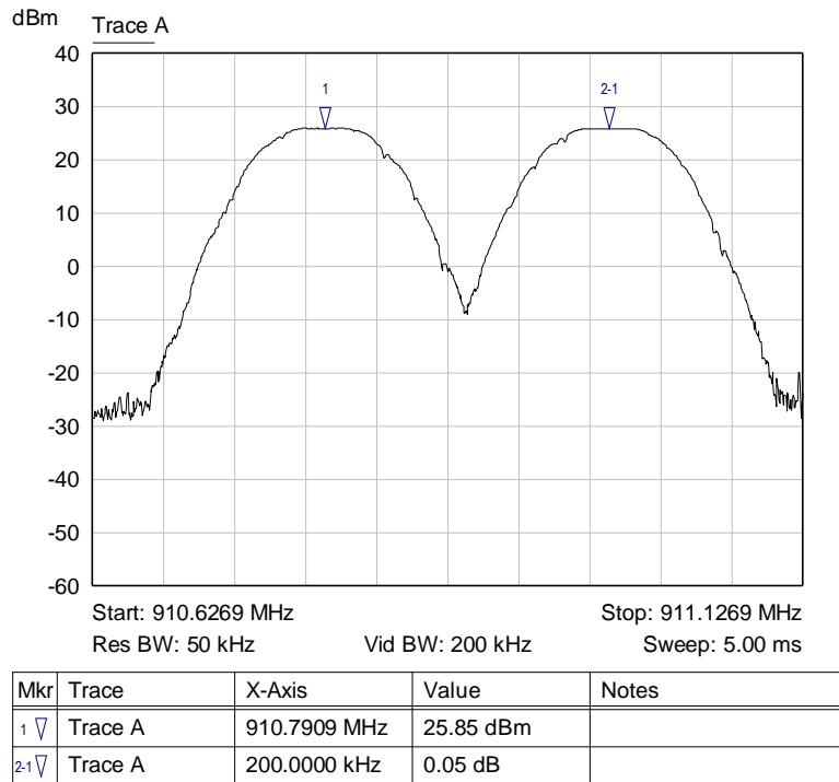
Graph 1: Channel Separation Plot
