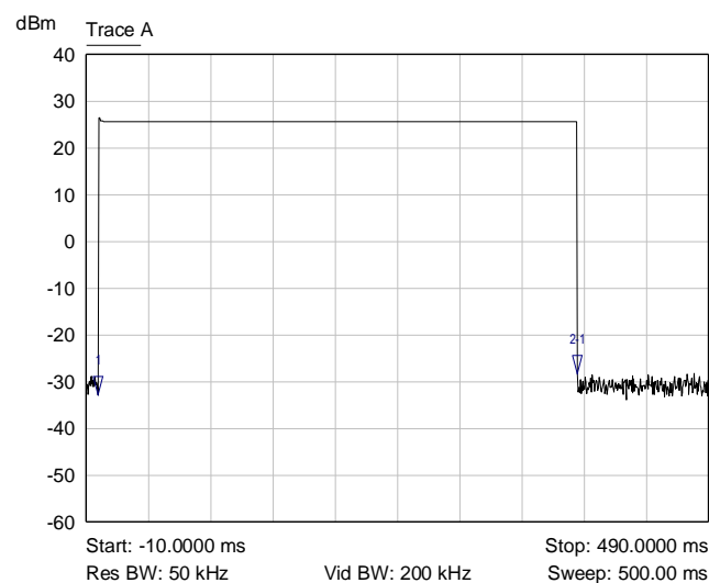
Graph 8: Timing Plot Showing Channel Hits
