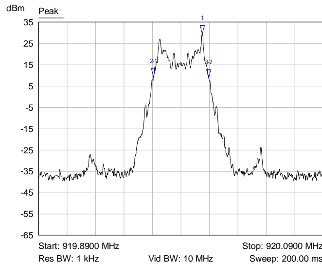
Graph 6: Antenna 1 – Middle Channel 20 dB Bandwidth
