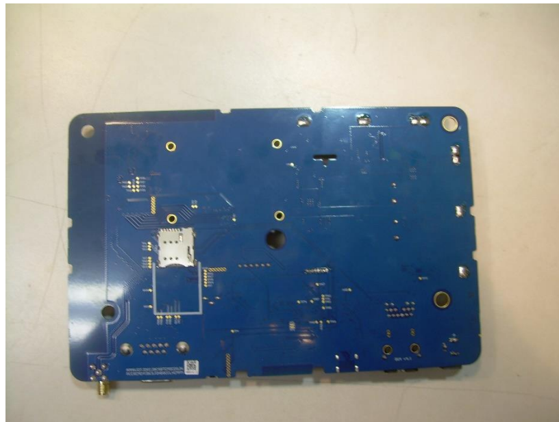
Photograph 14: View of the Back Side of the PCB
