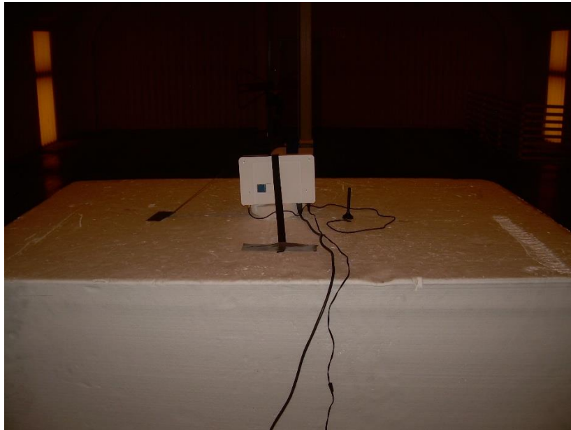
Photograph 4: Back View Radiated Emissions Worst-Case Configuration – Above 1000 MHz
