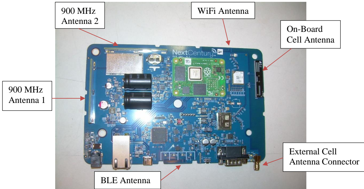
Photograph 13: View of the Front Side of the PCB
