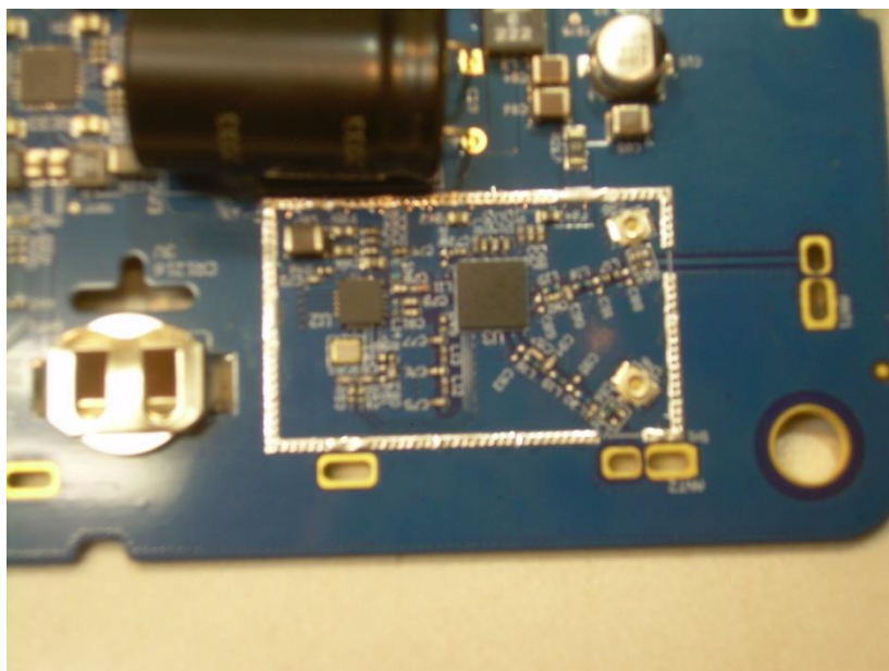
Photograph 15: View of the Circuitry Under the 900 MHz Transceiver RF Shield
