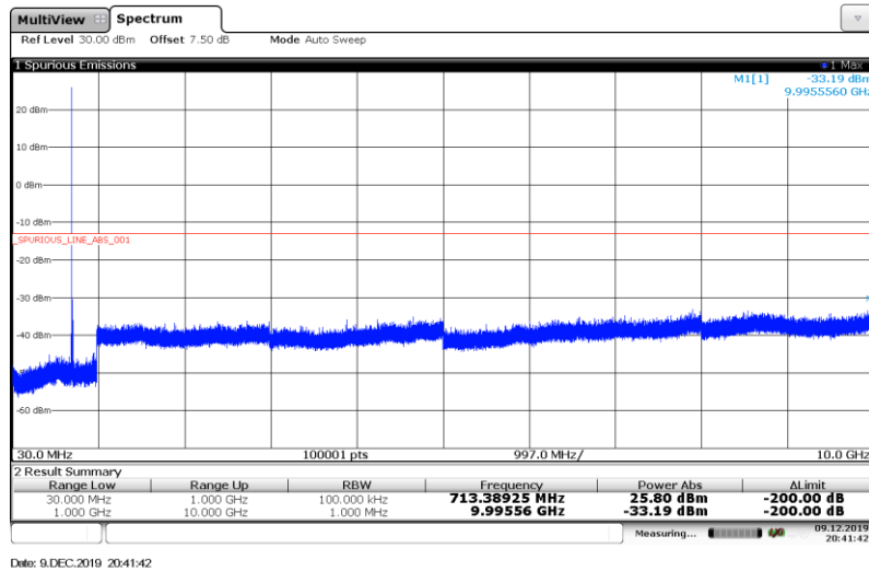
Band12-3MHz-16QAM-23165-1RB#
