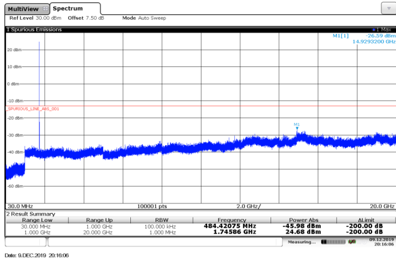
Band4-10MHz-16QAM-20350-1RB#
