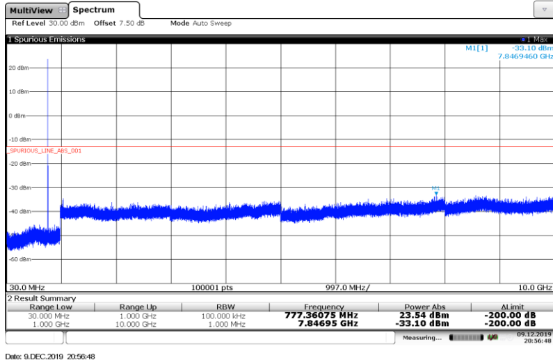
Band13-5MHz-QPSK-23205-1RB#
