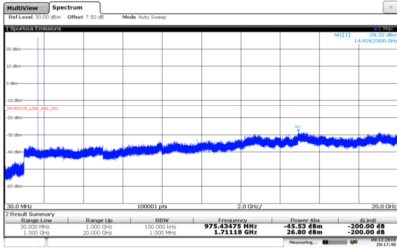
Band4-15MHz-QPSK-20025-1RB#
