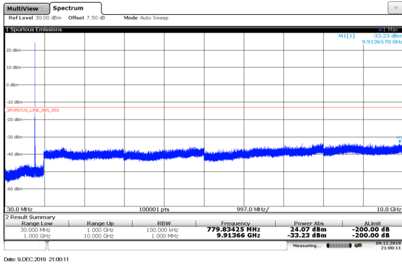
Band13-5MHz-QPSK-23230-1RB#
