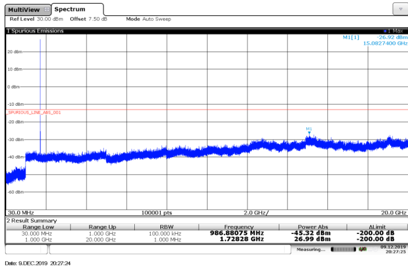
Band4-10MHz-16QAM-20175-1RB#
