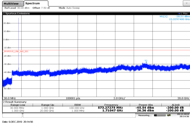
Band4-10MHz-16QAM-20000-1RB#
