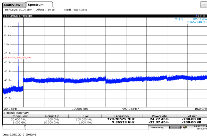
Band13-5MHz-16QAM-23230-1RB#
