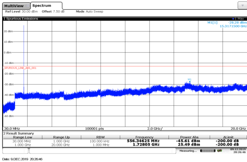
Band4-10MHz-QPSK-20175-1RB#
