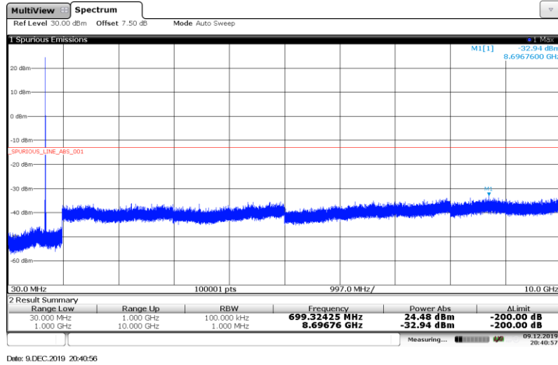
Band12-3MHz-16QAM-23025-1RB#
