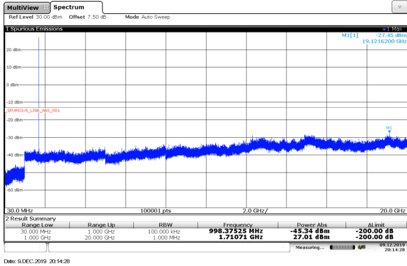
Band4-10MHz-QPSK-20000-1RB#
