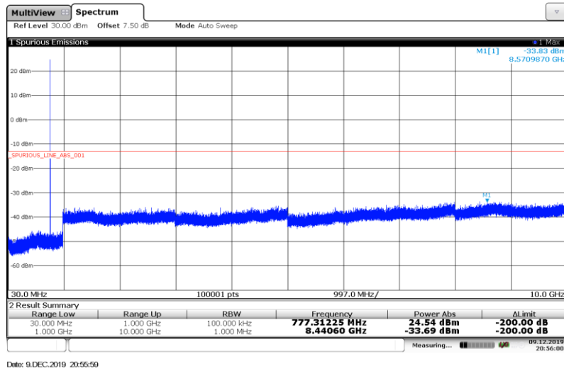
Band13-5MHz-16QAM-23205-1RB#
