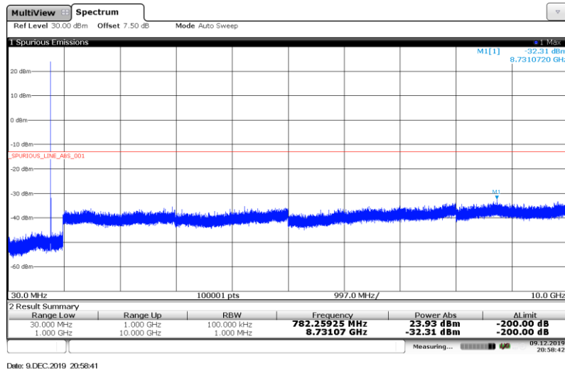
Band13-5MHz-16QAM-23255-1RB#
