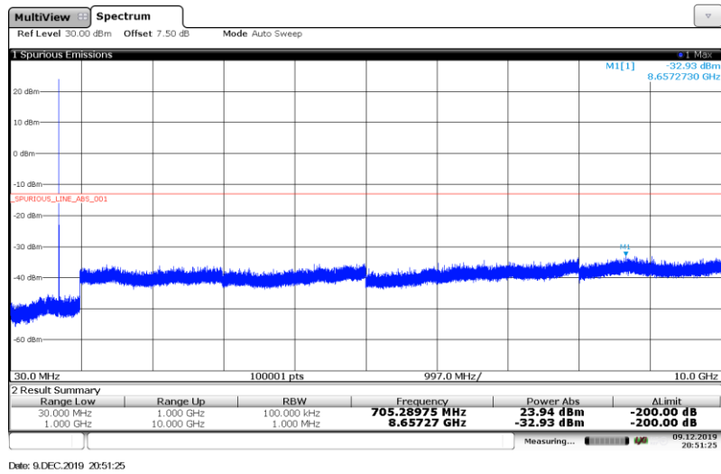
Band12-5MHz-16QAM-23095-1RB#
