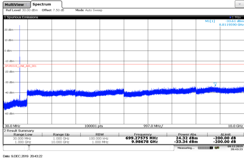
Band12-5MHz-16QAM-23035-1RB#
