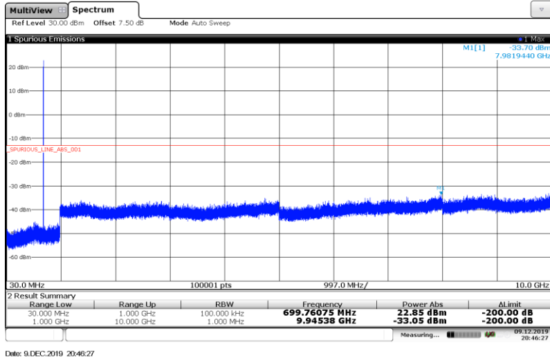
Band12-10MHz-16QAM-23060-1RB#
