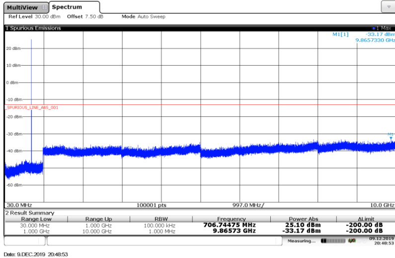
Band12-10MHz-16QAM-23130-1RB#
