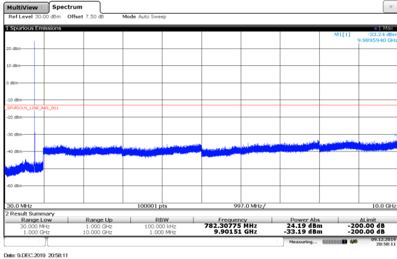
Band13-5MHz-QPSK-23255-1RB#
