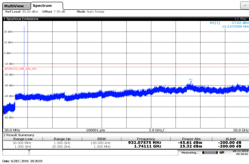
Band4-15MHz-QPSK-20325-1RB#
