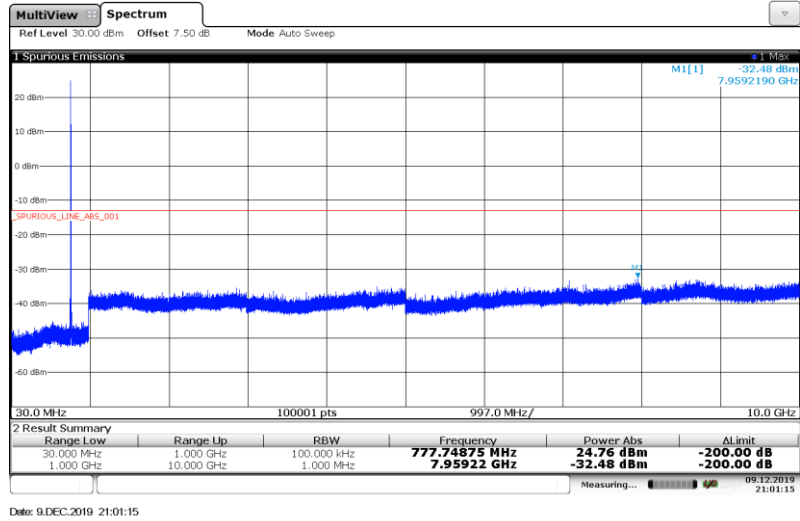
Band13-10MHz-QPSK-23230-1RB#
