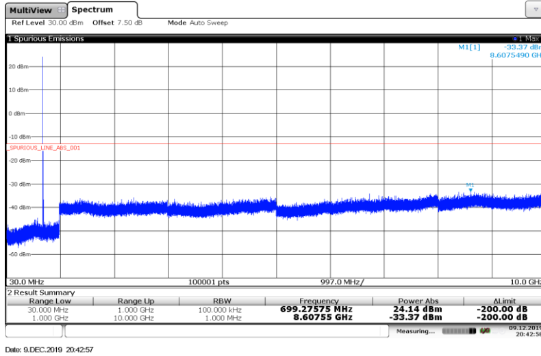
Band12-5MHz-QPSK-23035-1RB#
