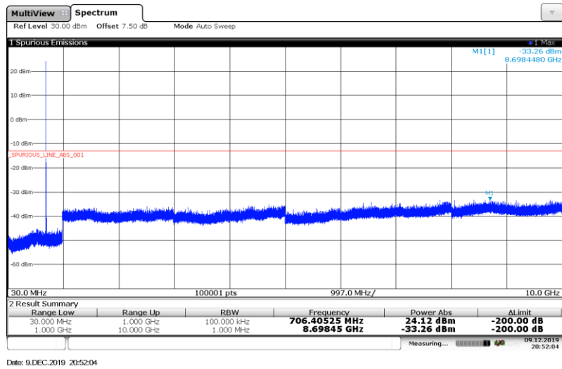
Band12-3MHz-QPSK-23095-1RB#
