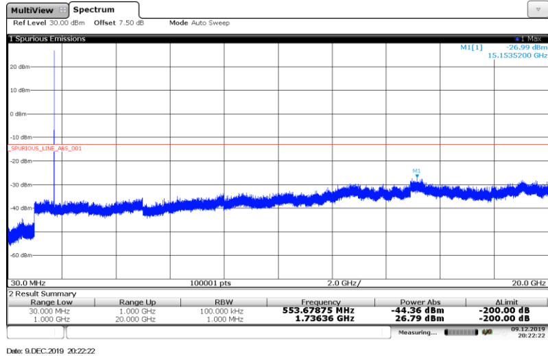
Band4-20MHz-QPSK-20300-1RB#
