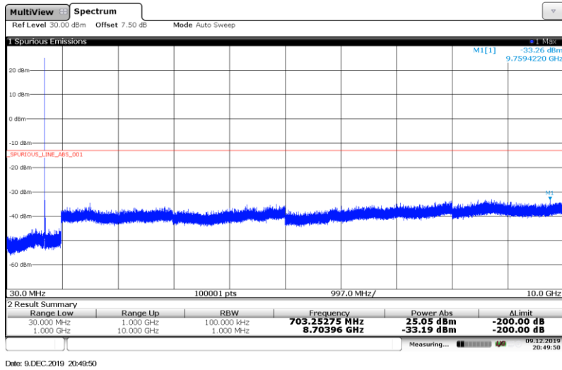
Band12-10MHz-16QAM-23095-1RB#
