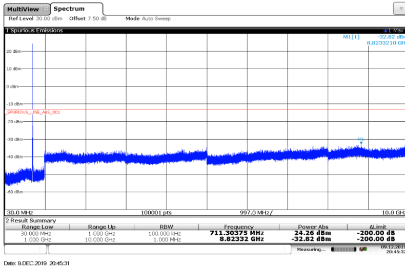
Band12-5MHz-QPSK-23155-1RB#
