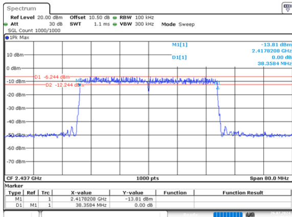
ax40_2437MHz_RU_Full_Chain 0 38.358MHz
