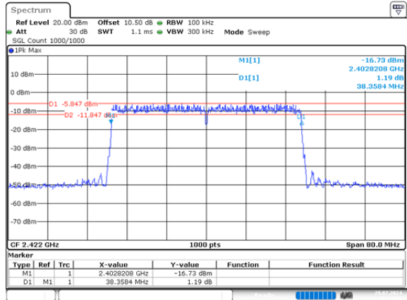
ax40_2422MHz_RU_Full_Chain 1 38.358MHz
