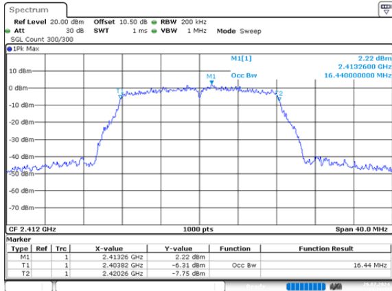
g_2412MHz_Chain 0 16.440MHz
