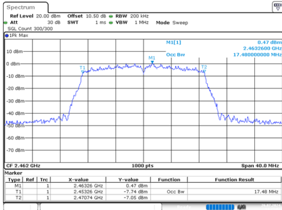
n20_2462MHz_Chain 0 17.480MHz
