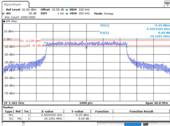
ax20_2462MHz_RU_Full_Chain 0 19.139MHz
