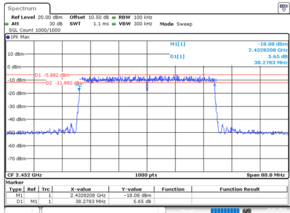
ax40_2452MHz_RU_Full_Chain 1 38.278MHz
