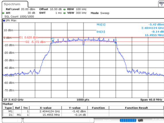
g_2412MHz_Chain 0 15.495MHz
