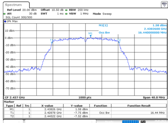
g_2437MHz_Chain 1 16.440MHz
