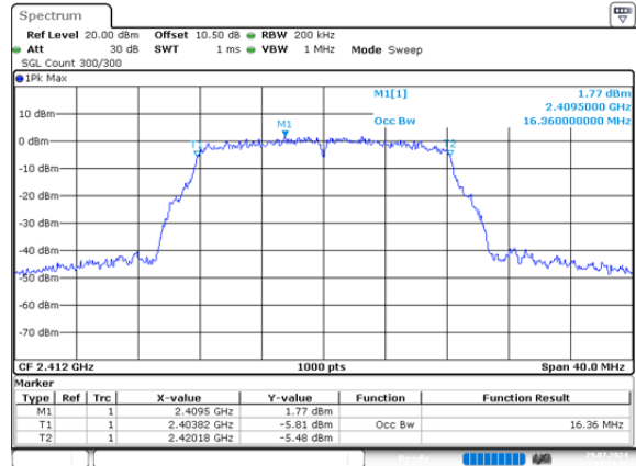
g_2412MHz_Chain 1 16.360MHz
