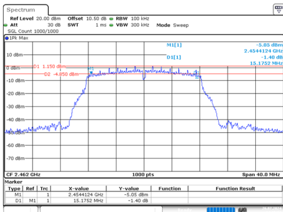
g_2462MHz_Chain 0 15.175MHz
