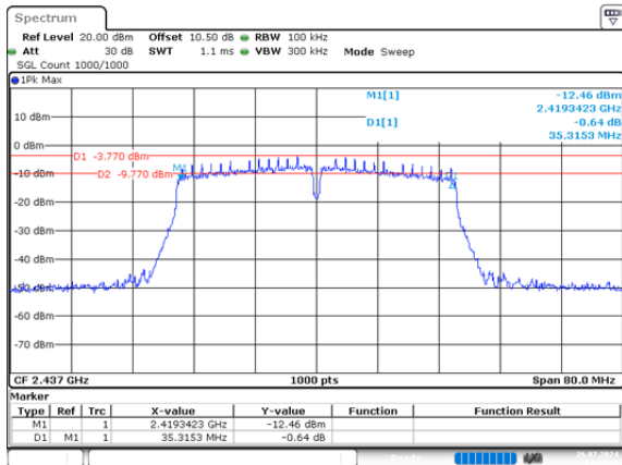
n40_2437MHz_Chain 0 35.315MHz
