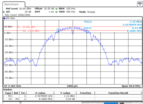
b_2462MHz_Chain 1 8.168MHz
