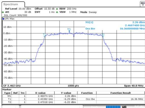
g_2462MHz_Chain 0 16.360MHz
