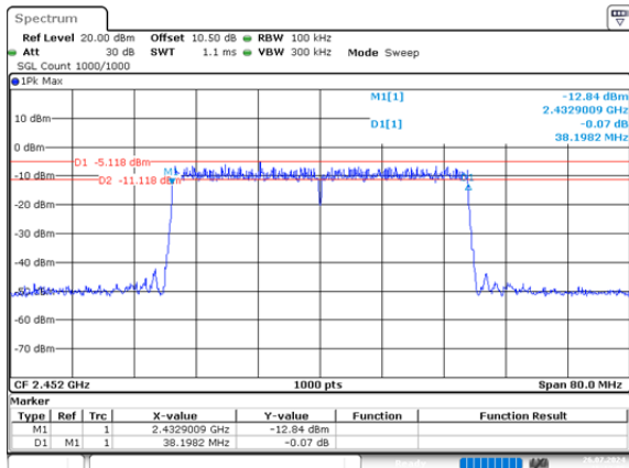
ax40_2452MHz_RU_Full_Chain 0 38.198MHz
