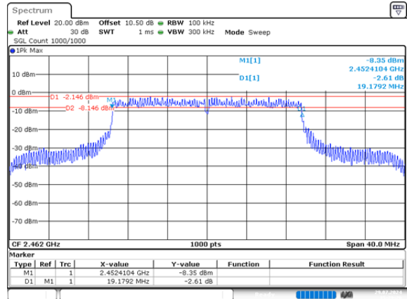
ax20_2462MHz_RU_Full_Chain 1 19.179MHz
