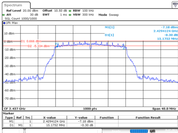
g_2437MHz_Chain 0 15.175MHz
