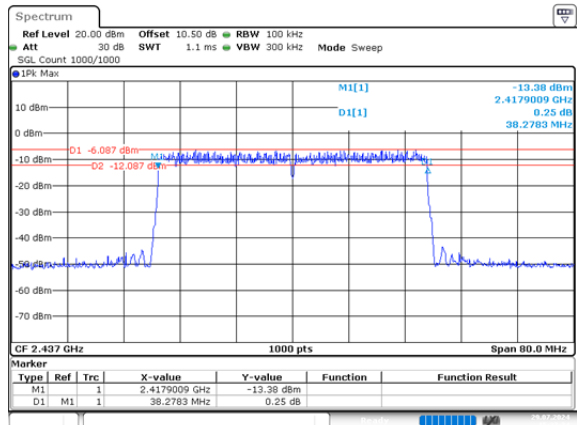
ax40_2437MHz_RU_Full_Chain 1 38.278MHz
