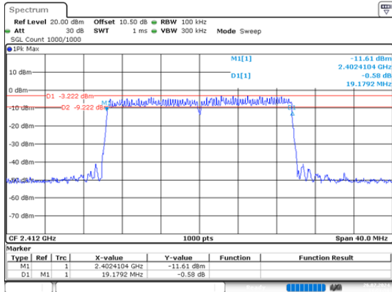
ax20_2412MHz_RU_Full_Chain 0 19.179MHz
