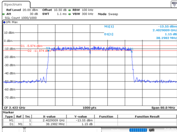
ax40_2422MHz_RU_Full_Chain 0 38.198MHz
