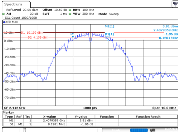
b_2412MHz_Chain 0 8.128MHz
