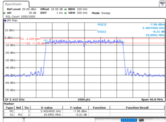
ax20_2412MHz_RU_Full_Chain 1 19.099MHz
