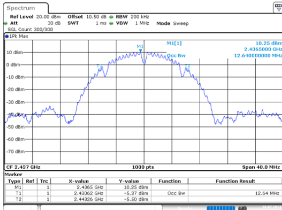
b_2437MHz_Chain 0 12.640MHz
