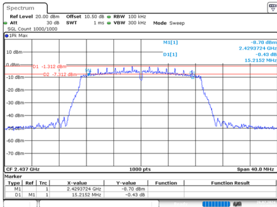
n20_2437MHz_Chain 0 15.215MHz
