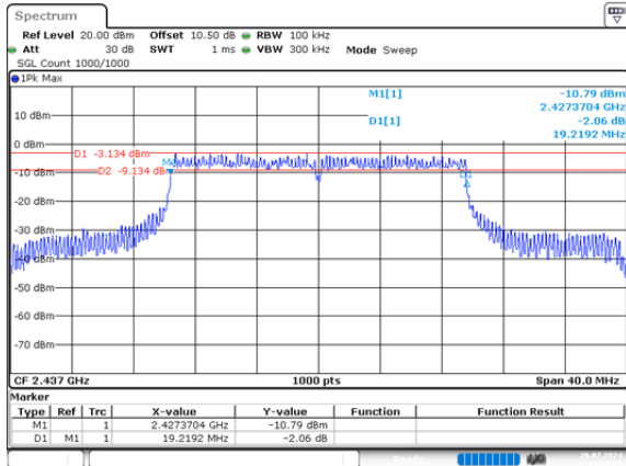
ax20_2437MHz_RU_Full_Chain 0 19.219MHz
