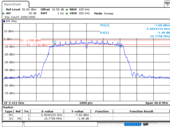
n20_2412MHz_Chain 0 15.776MHz
