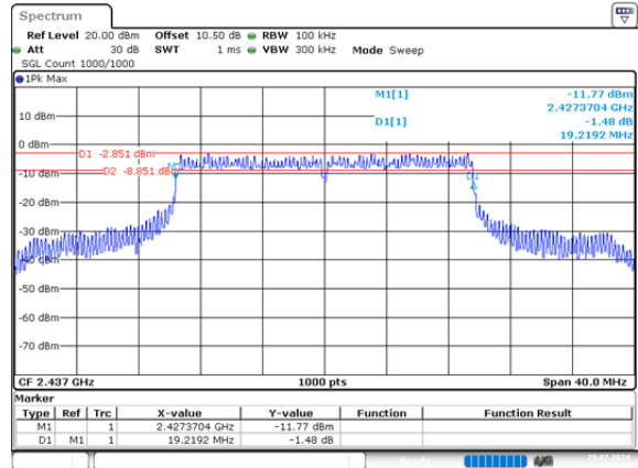
ax20_2437MHz_RU_Full_Chain 1 19.219MHz
