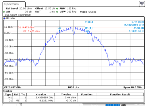
b_2437MHz_Chain 1 8.128MHz
