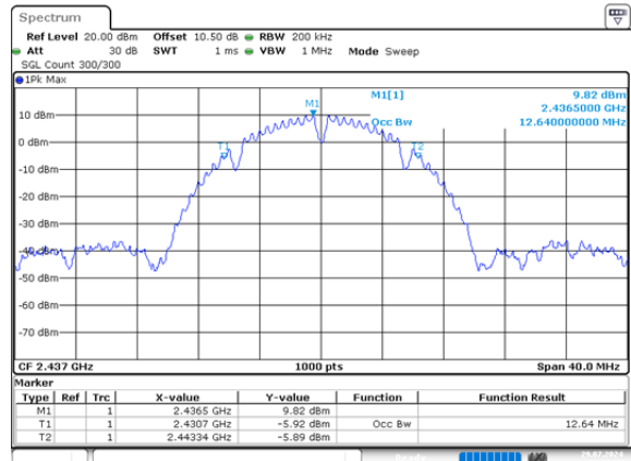
b_2437MHz_Chain 1 12.640MHz
