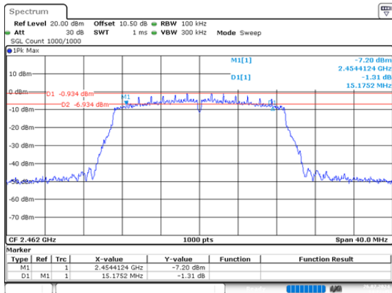
n20_2462MHz_Chain 0 15.175MHz
