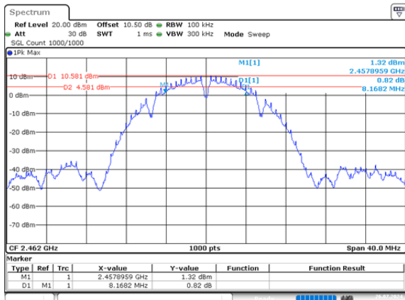
b_2462MHz_Chain 0 8.168MHz
