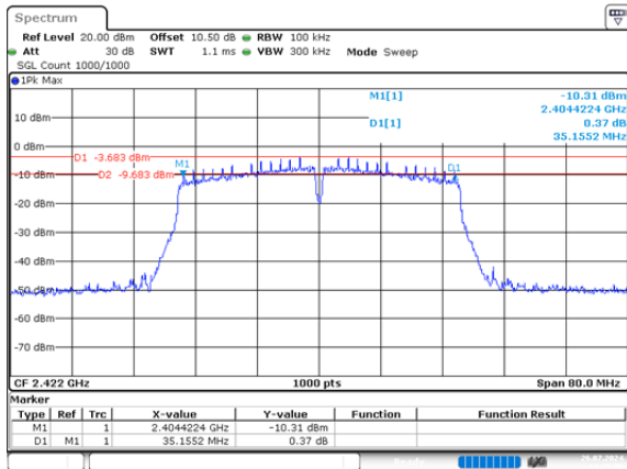
n40_2422MHz_Chain 0 35.155MHz
