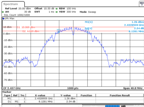
b_2437MHz_Chain 0 8.128MHz
