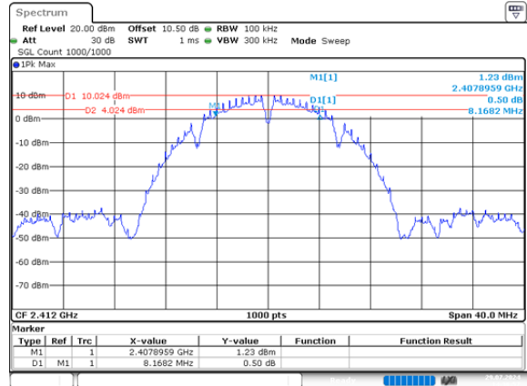
b_2412MHz_Chain 1 8.168MHz
