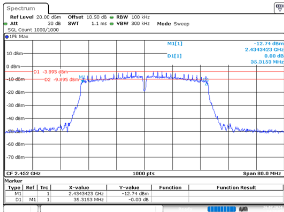
n40_2452MHz_Chain 0 35.315MHz
