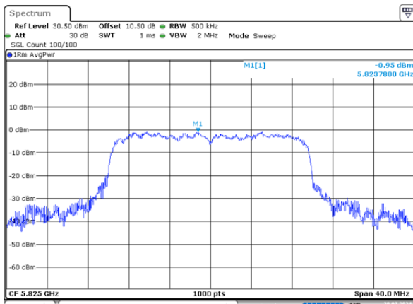
ax20_5825MHz_RU_Full_Chain 0 - 0.95dBm/MHz
