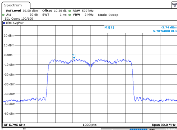
ax40_5795MHz_RU_Full_Chain 0 - 3.74dBm/MHz
