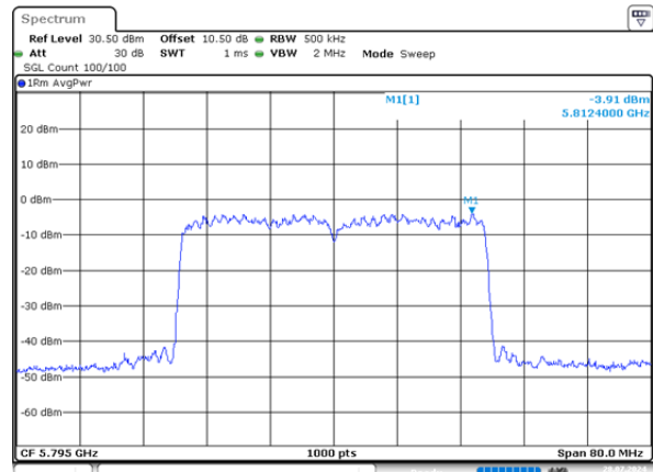
ax40_5795MHz_RU_Full_Chain 1 - 3.91dBm/MHz
