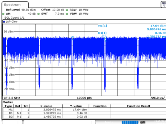
a_5200MHz_Chain 0 1.391ms,1.451ms
