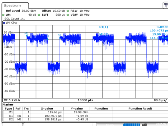
ax20_5200MHz_RU_Full_Chain 0 0.100ms,0.159ms
