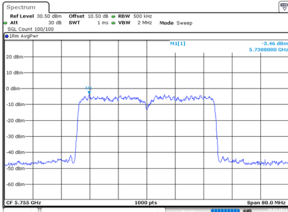
ax40_5755MHz_RU_Full_Chain 0 - 3.46dBm/MHz
