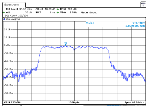
ax20_5825MHz_RU_Full_Chain 1 - 0.37dBm/MHz
