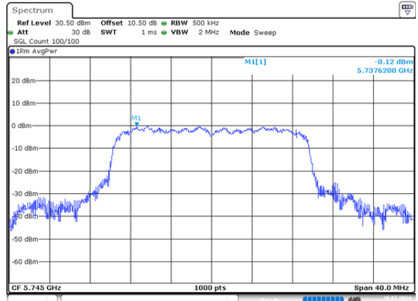
ax20_5745MHz_RU_Full_Chain 1 - 0.12dBm/MHz
