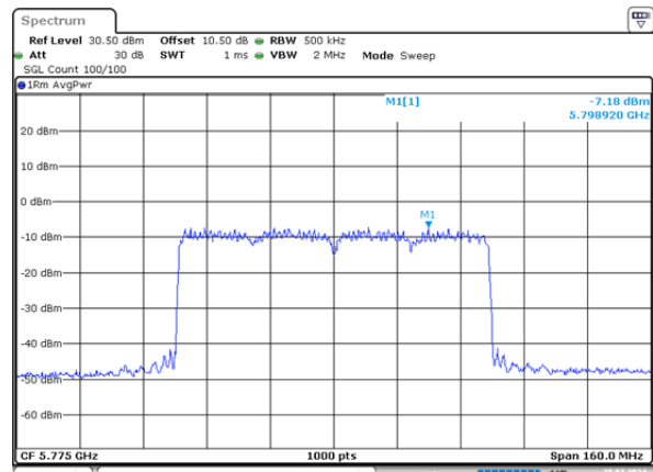
ax80_5775MHz_RU_Full_Chain 1 - 7.18dBm/MHz
