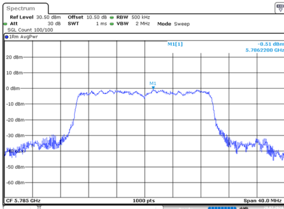
ax20_5785MHz_RU_Full_Chain 0 - 0.51dBm/MHz
