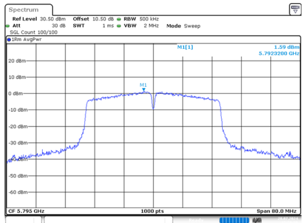
n40_5795MHz_Chain 1 1.59dBm/MHz
