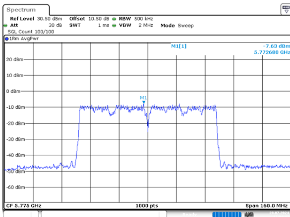
ac80_5775MHz_Chain 0 -7.63dBm/MHz
