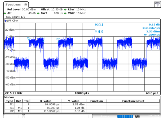
ac80_5210MHz_Chain 0 0.056ms,0.113ms
