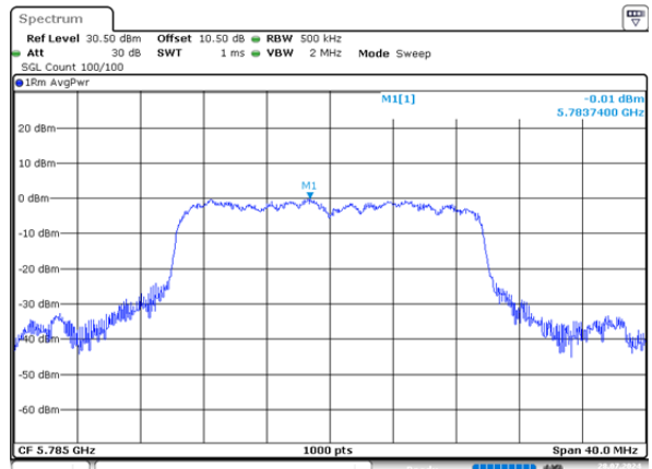
ax20_5785MHz_RU_Full_Chain 1 - 0.01dBm/MHz
