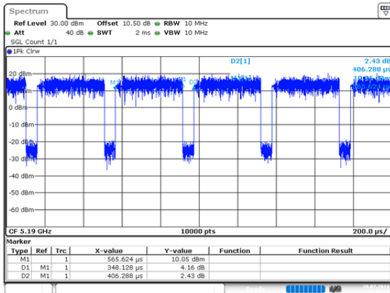
n40_5190MHz_Chain 0 0.348ms,0.406ms
