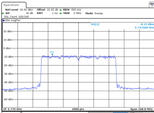
ax80_5775MHz_RU_Full_Chain 0 - 8.12dBm/MHz
