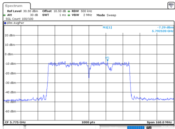
ac80_5775MHz_Chain 1 -7.29dBm/MHz
