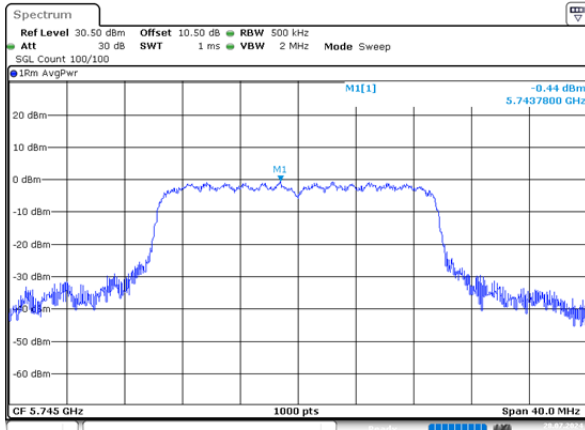
ax20_5745MHz_RU_Full_Chain 0 - 0.44dBm/MHz
