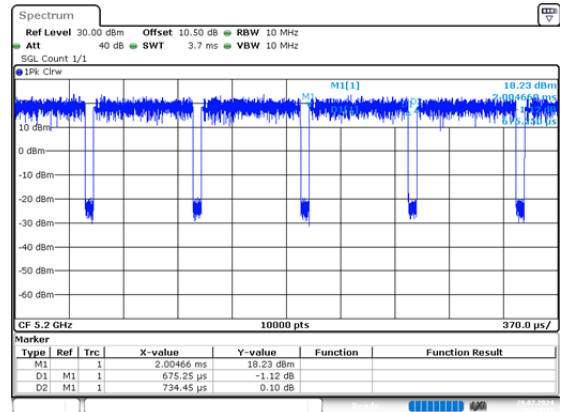
n20_5200MHz_Chain 0 0.675ms,0.734ms
