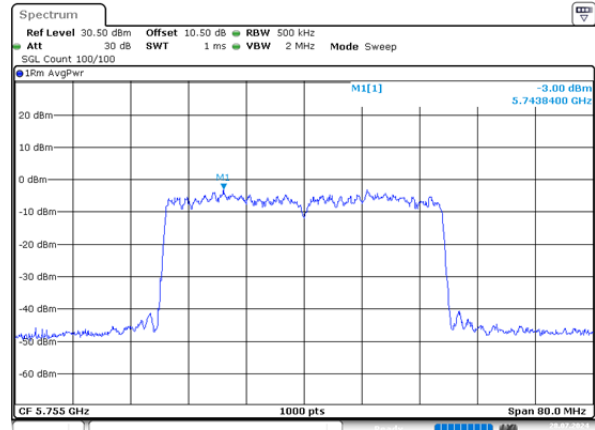
ax40_5755MHz_RU_Full_Chain 1 - 3.00dBm/MHz
