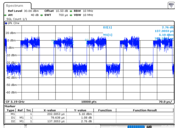
ax40_5190MHz_RU_Full_Chain 0 0.079ms,0.137ms
