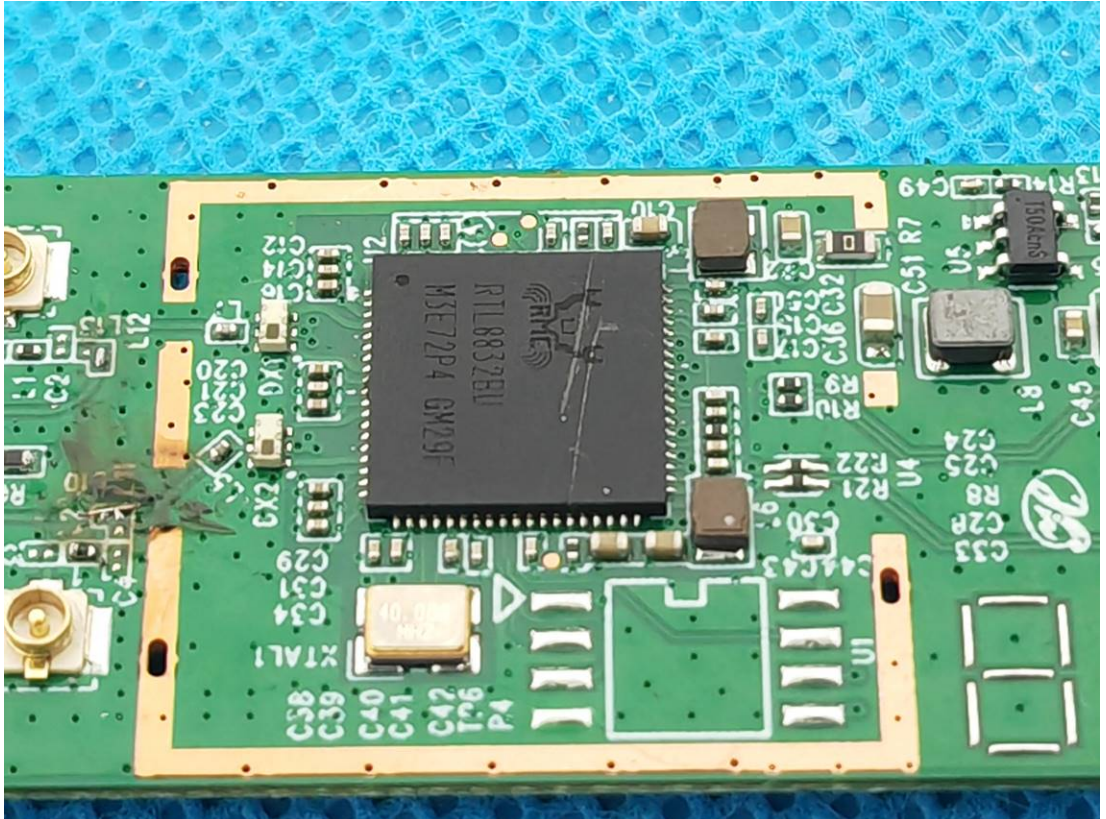
chip
