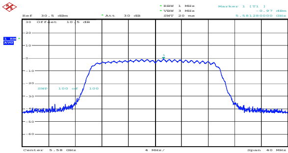
ax20_5580MHz_RU_Full_Chain 0 -0.97dBm/MHz
