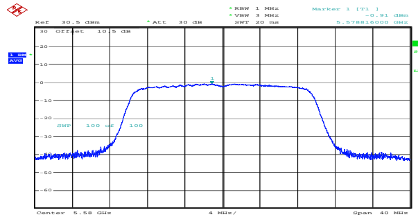
ax20_5580MHz_RU_Full_Chain 1 -0.91dBm/MHz
