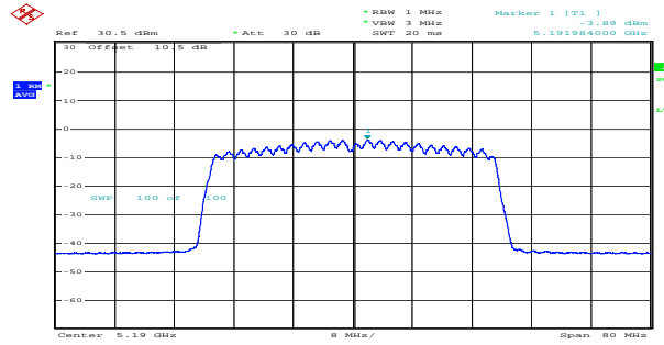
ax40_5190MHz_RU_Full_Chain 1 -3.89dBm/MHz
