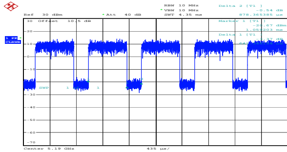
n40_5190MHz_Chain 0 0.641ms,0.878ms
