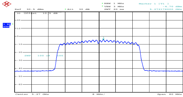
ax40_5270MHz_RU_Full_Chain 0 -4.70dBm/MHz
