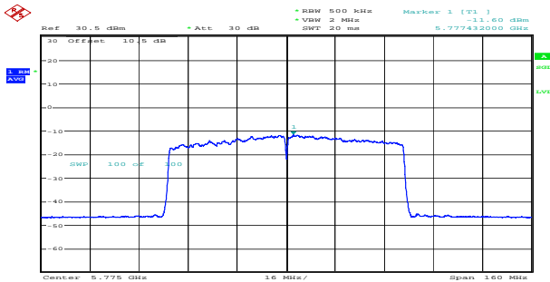
ac80_5775MHz_Chain 0 -11.60dBm/MHz
