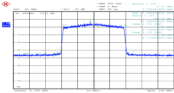
ax40_5755MHz_RU_Full_Chain 0 37.600MHz
