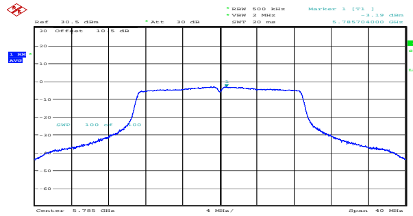
n20_5785MHz_Chain 1 -3.19dBm/MHz
