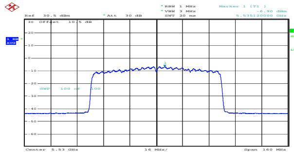
ax80_5530MHz_RU_Full_Chain 1 -6.90dBm/MHz
