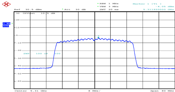
ax40_5310MHz_RU_Full_Chain 0 -4.05dBm/MHz
