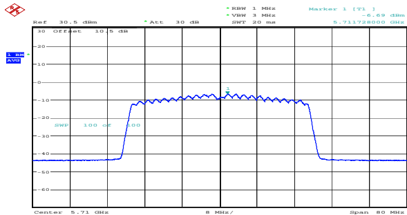
ax40_5710MHz_RU_Full_Chain 0 -6.69dBm/MHz
