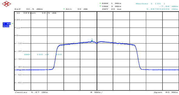
ax40_5670MHz_RU_Full_Chain 0 -7.66dBm/MHz
