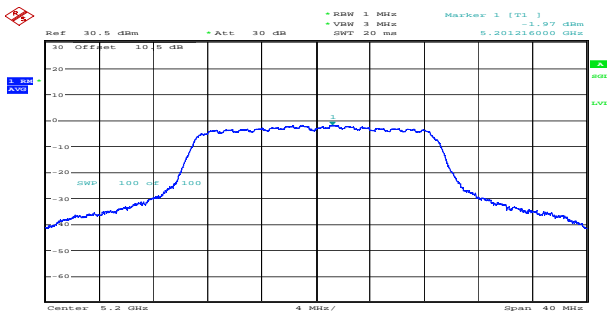
n20_5200MHz_Chain 0 -1.97dBm/MHz
