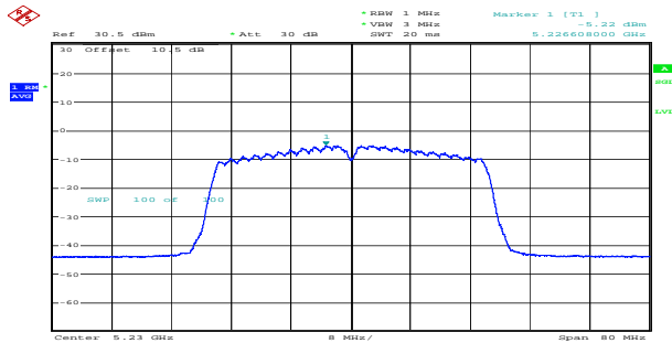
n40_5230MHz_Chain 0 -5.22dBm/MHz
