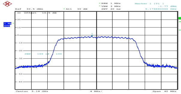
ax20_5180MHz_RU_Full_Chain 1 -1.77dBm/MHz
