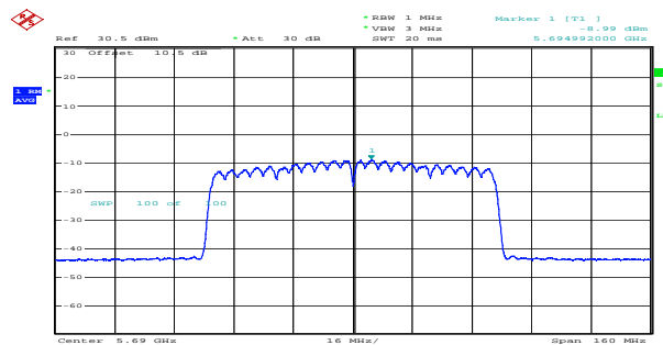
ac80_5690MHz_Chain 1 -8.99dBm/MHz
