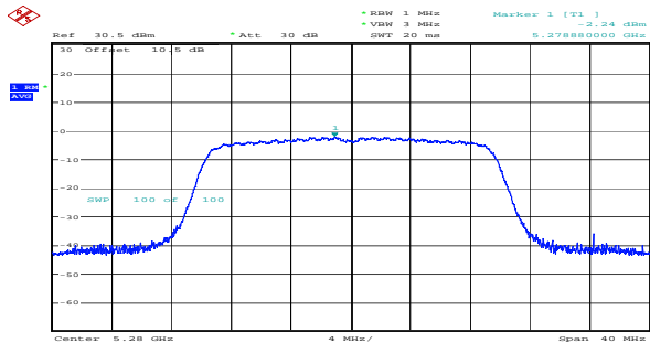
ax20_5280MHz_RU_Full_Chain 0 -2.24dBm/MHz
