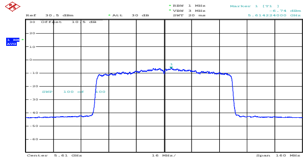
ax80_5610MHz_RU_Full_Chain 1 -6.74dBm/MHz
