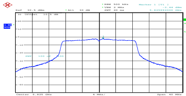
n20_5825MHz_Chain 1 -2.44dBm/MHz
