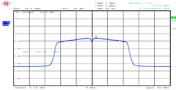
n40_5190MHz_Chain 0 -5.82dBm/MHz
