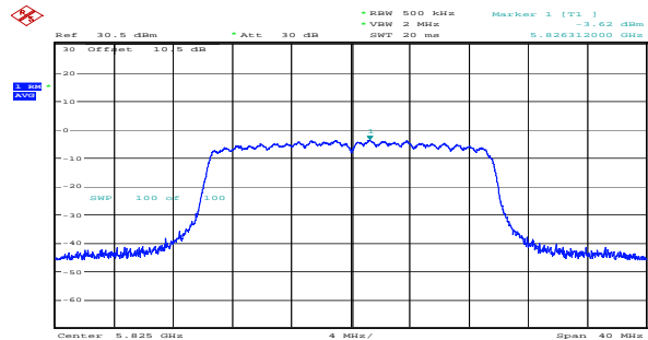
ax20_5825MHz_RU_Full_Chain 1 -3.62dBm/MHz
