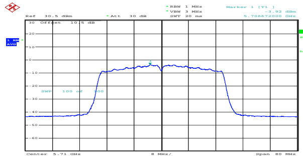
n40_5710MHz_Chain 1 -3.92dBm/MHz
