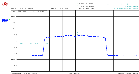
ac80_5690MHz_Chain 0 -9.82dBm/MHz
