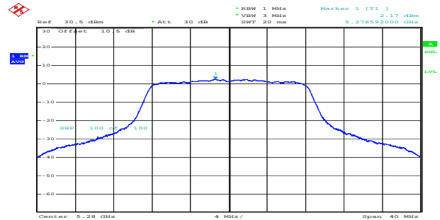
a_5280MHz_Chain 1 2.17dBm/MHz
