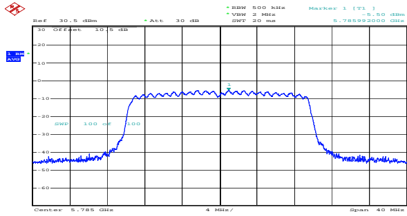
ax20_5785MHz_RU_Full_Chain 0 -5.50dBm/MHz
