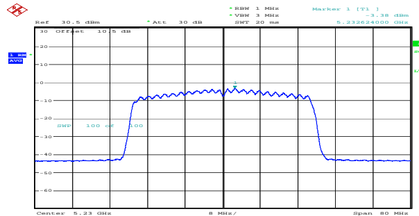
ax40_5230MHz_RU_Full_Chain 1 -3.38dBm/MHz
