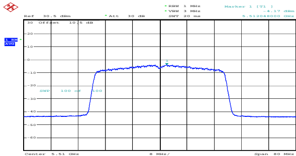
ax40_5510MHz_RU_Full_Chain 0 -4.17dBm/MHz
