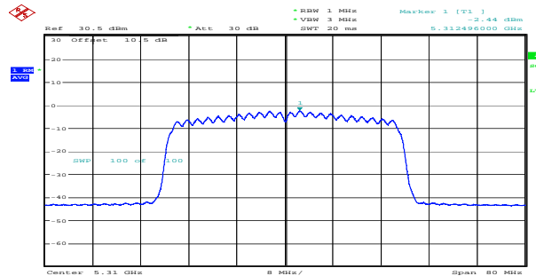
ax40_5310MHz_RU_Full_Chain 1 -2.44dBm/MHz
