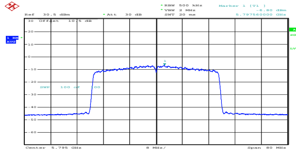
ax40_5795MHz_RU_Full_Chain 1 -6.80dBm/MHz
