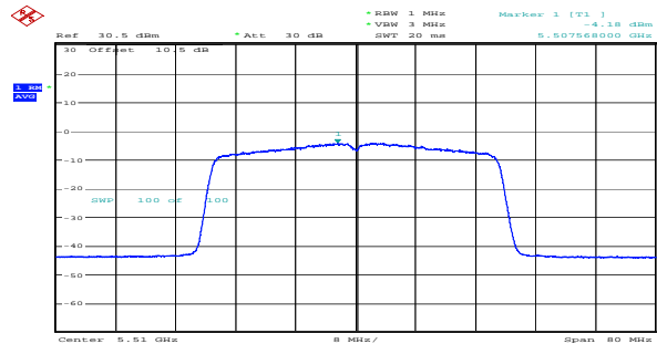
ax40_5510MHz_RU_Full_Chain 1 -4.18dBm/MHz
