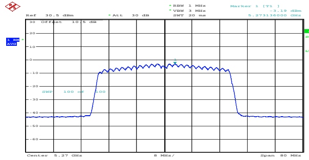
ax40_5270MHz_RU_Full_Chain 1 -3.19dBm/MHz
