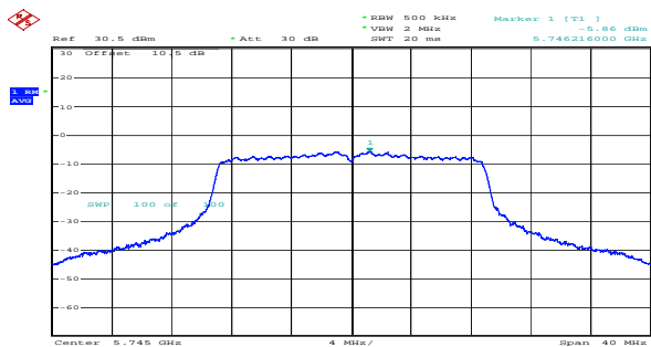
n20_5745MHz_Chain 0 -5.86dBm/MHz
