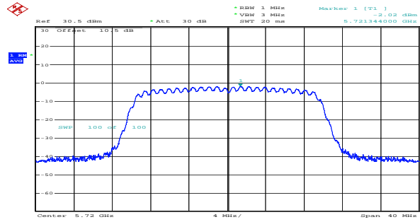
ax20_5720MHz_RU_Full_Chain 1 -2.02dBm/MHz
