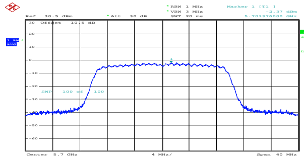
ax20_5700MHz_RU_Full_Chain 1 -2.37dBm/MHz
