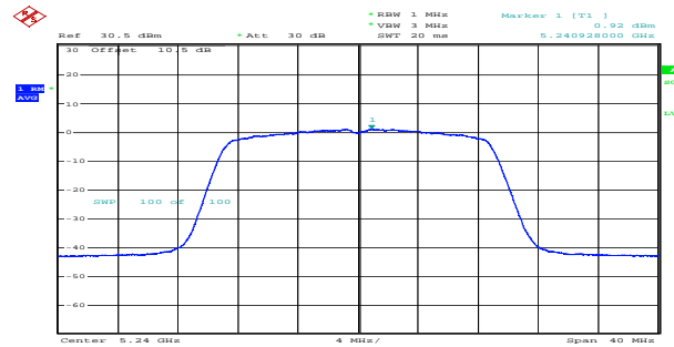
n20_5240MHz_Chain 1 0.92dBm/MHz
