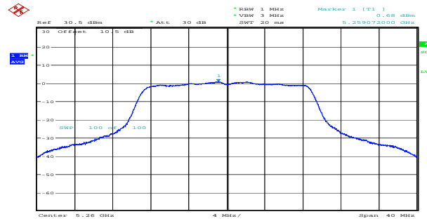
n20_5260MHz_Chain 1 0.68dBm/MHz
