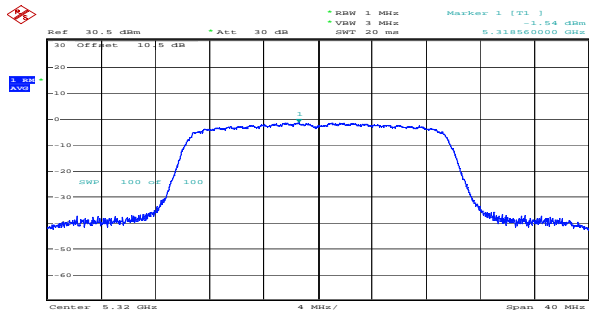
ax20_5320MHz_RU_Full_Chain 0 -1.54dBm/MHz
