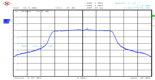
n20_5280MHz_Chain 1 0.72dBm/MHz
