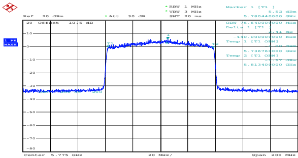
ax80_5775MHz_RU_Full_Chain 0 76.640MHz
