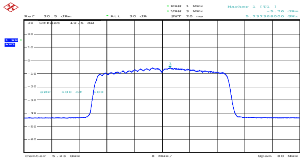
ax40_5230MHz_RU_Full_Chain 0 -5.76dBm/MHz
