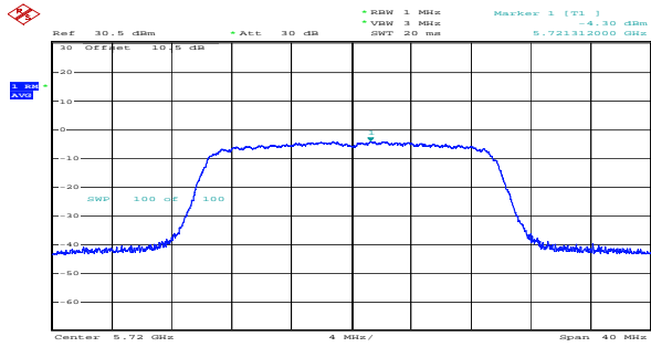
ax20_5720MHz_RU_Full_Chain 0 -4.30dBm/MHz
