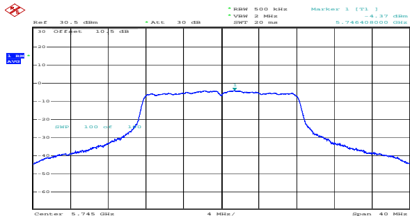
a_5745MHz_Chain 0 -4.37dBm/MHz
