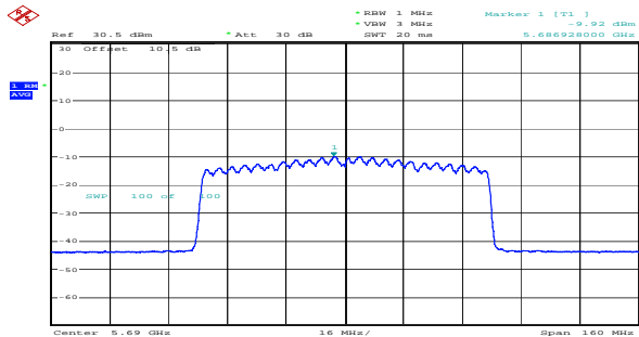
ax80_5690MHz_RU_Full_Chain 0 -9.92dBm/MHz
