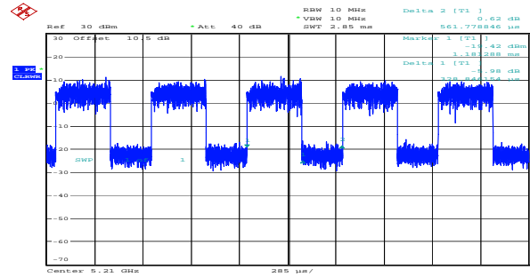
ac80_5210MHz_Chain 0 0.329ms,0.562ms
