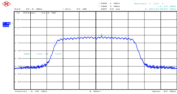
ax20_5260MHz_RU_Full_Chain 0 -2.10dBm/MHz
