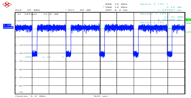
a_5200MHz_Chain 0 1.380ms,1.629ms
