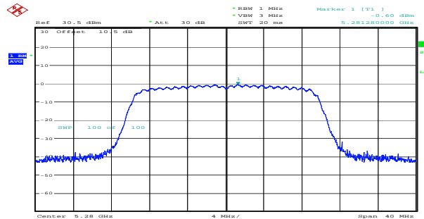
ax20_5280MHz_RU_Full_Chain 1 -0.60dBm/MHz
