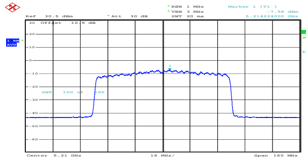
ax80_5210MHz_RU_Full_Chain 1 -7.58dBm/MHz
