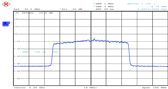
ax80_5290MHz_RU_Full_Chain 0 -8.14dBm/MHz
