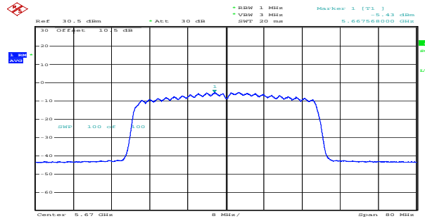
ax40_5670MHz_RU_Full_Chain 1 -5.43dBm/MHz
