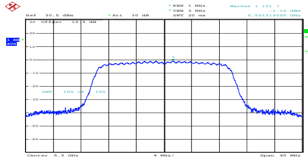
ax20_5500MHz_RU_Full_Chain 1 -1.12dBm/MHz
