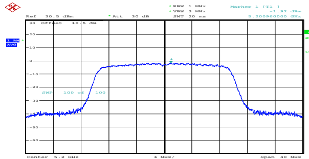
ax20_5200MHz_RU_Full_Chain 1 -1.92dBm/MHz
