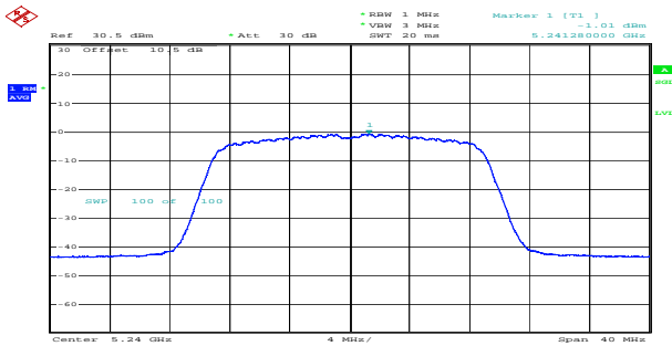
n20_5240MHz_Chain 0 -1.01dBm/MHz
