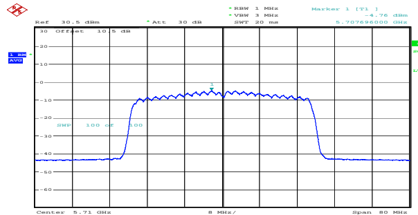
ax40_5710MHz_RU_Full_Chain 1 -4.76dBm/MHz
