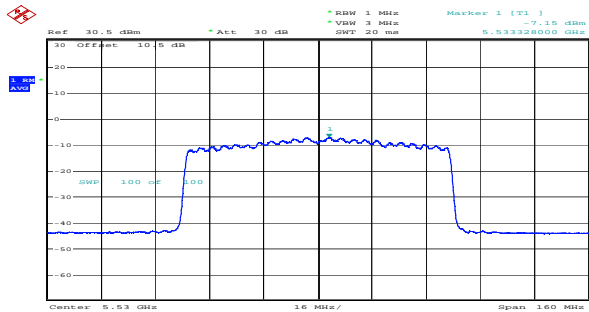
ax80_5530MHz_RU_Full_Chain 0 -7.15dBm/MHz
