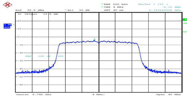
ax20_5745MHz_RU_Full_Chain 1 -5.10dBm/MHz
