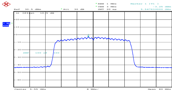
ax40_5550MHz_RU_Full_Chain 0 -3.25dBm/MHz
