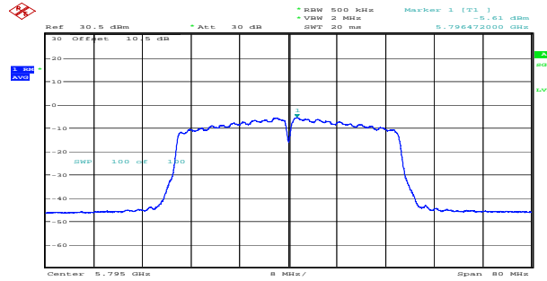
n40_5795MHz_Chain 1 -5.61dBm/MHz
