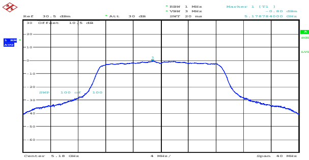
n20_5180MHz_Chain 0 -0.80dBm/MHz
