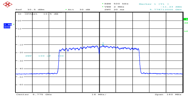
ac80_5775MHz_Chain 1 -11.23dBm/MHz
