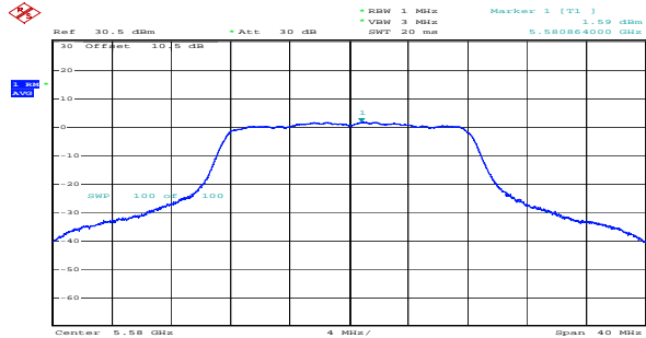
a_5580MHz_Chain 0 1.59dBm/MHz
