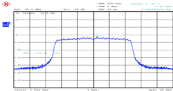
ax20_5825MHz_RU_Full_Chain 0 -3.87dBm/MHz
