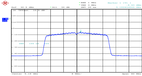
ax40_5190MHz_RU_Full_Chain 0 -6.43dBm/MHz
