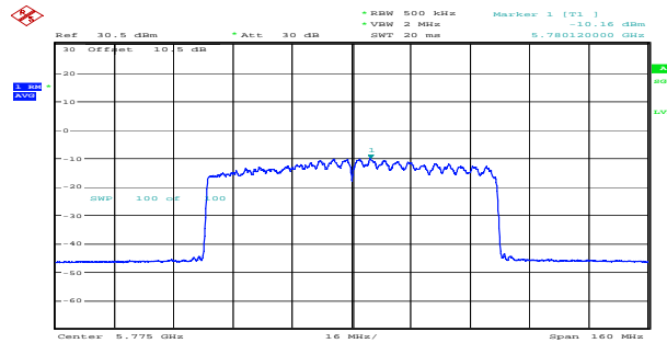
ax80_5775MHz_RU_Full_Chain 1 -10.16dBm/MHz
