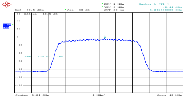
ax20_5240MHz_RU_Full_Chain 0 -2.44dBm/MHz
