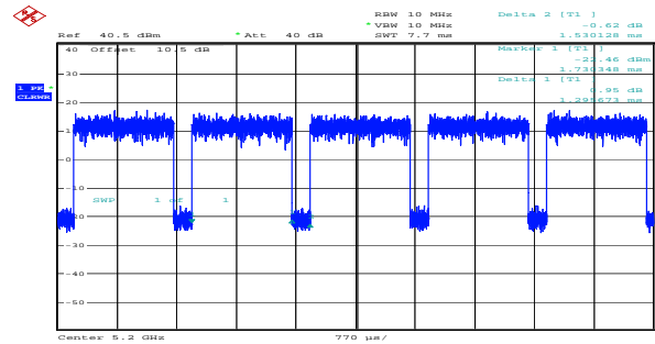
n20_5200MHz_Chain 0 1.296ms,1.530ms
