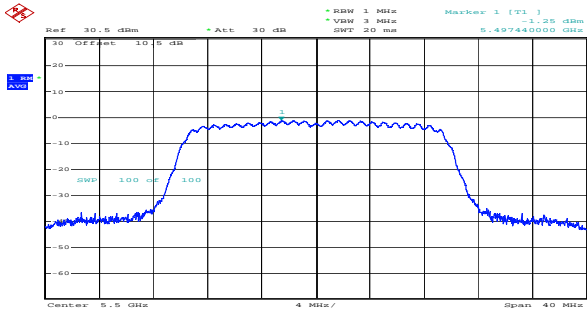
ax20_5500MHz_RU_Full_Chain 0 -1.25dBm/MHz
