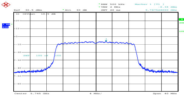
ax20_5745MHz_RU_Full_Chain 0 -6.36dBm/MHz
