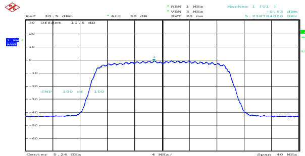
ax20_5240MHz_RU_Full_Chain 1 -0.83dBm/MHz
