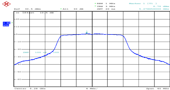
a_5280MHz_Chain 0 0.70dBm/MHz
