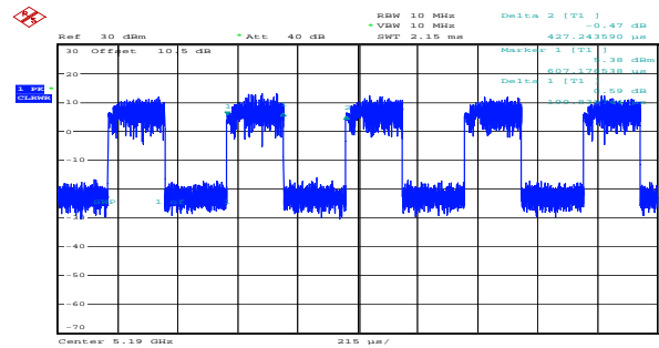
ax40_5190MHz_RU_Full_Chain 0 0.200ms,0.427ms
