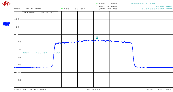
ax80_5610MHz_RU_Full_Chain 0 -6.66dBm/MHz
