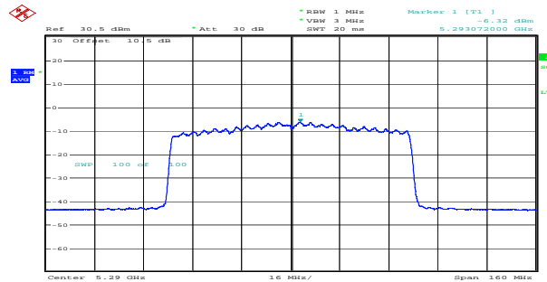
ax80_5290MHz_RU_Full_Chain 1 -6.32dBm/MHz
