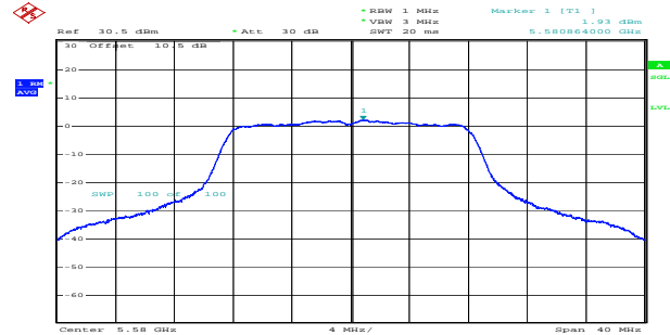
a_5580MHz_Chain 1 1.93dBm/MHz
