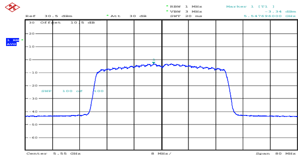
ax40_5550MHz_RU_Full_Chain 1 -3.34dBm/MHz
