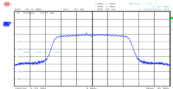
ax20_5320MHz_RU_Full_Chain 1 -0.09dBm/MHz
