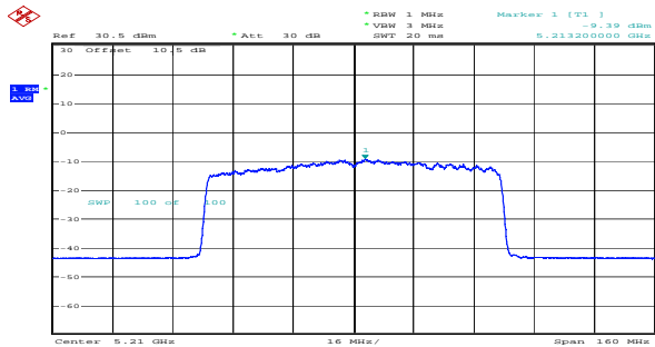
ax80_5210MHz_RU_Full_Chain 0 -9.39dBm/MHz
