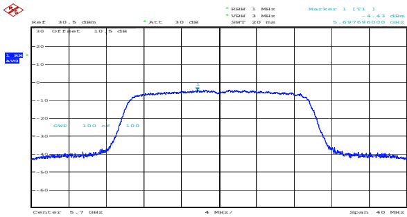
ax20_5700MHz_RU_Full_Chain 0 -4.43dBm/MHz
