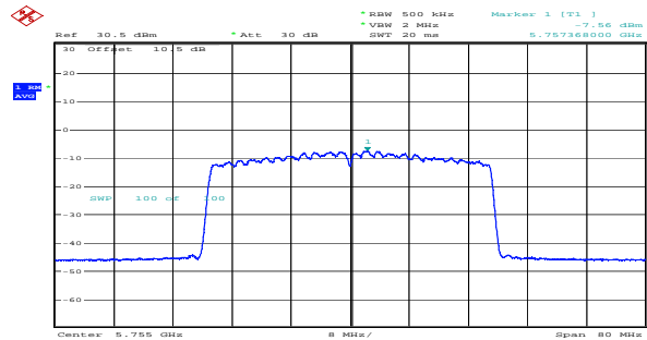
ax40_5755MHz_RU_Full_Chain 1 -7.56dBm/MHz
