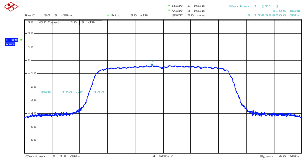
ax20_5180MHz_RU_Full_Chain 0 -4.06dBm/MHz
