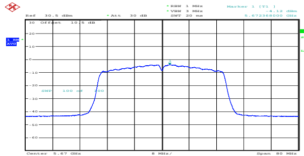
n40_5670MHz_Chain 1 -4.12dBm/MHz
