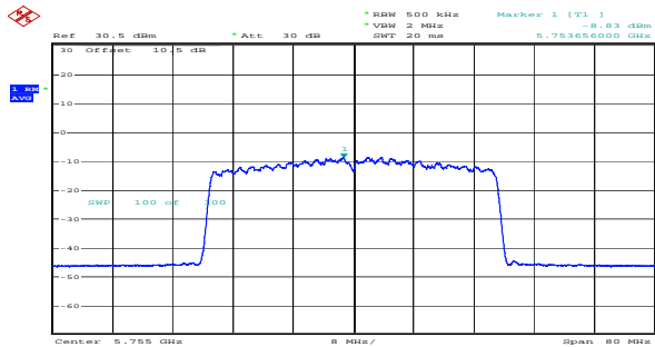
ax40_5755MHz_RU_Full_Chain 0 -8.83dBm/MHz
