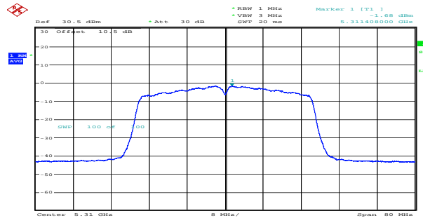
n40_5310MHz_Chain 1 -1.68dBm/MHz
