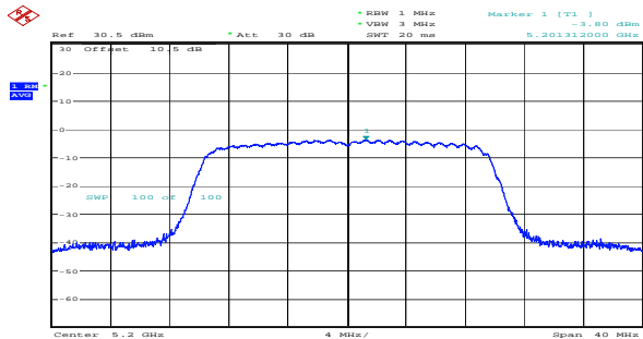
ax20_5200MHz_RU_Full_Chain 0 -3.80dBm/MHz
