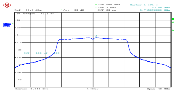
n20_5745MHz_Chain 1 -3.58dBm/MHz
