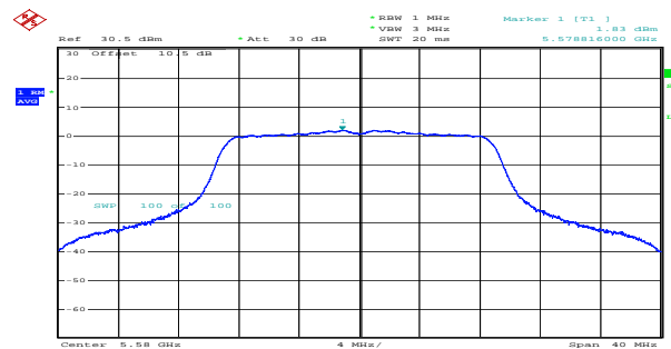
n20_5580MHz_Chain 1 1.83dBm/MHz
