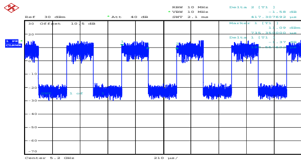
ax20_5200MHz_RU_Full_Chain 0 0.199ms,0.417ms
