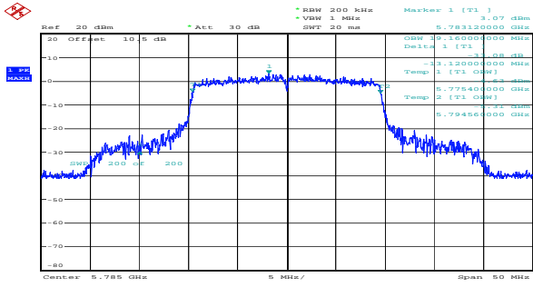
ax20_5785MHz_RU_Full_Chain 0 19.160MHz
