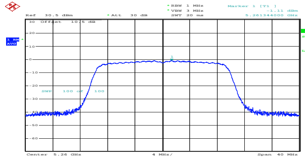
ax20_5260MHz_RU_Full_Chain 1 -1.11dBm/MHz
