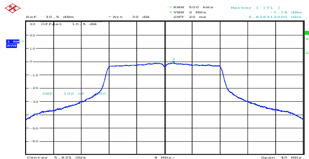
a_5825MHz_Chain 1 -1.14dBm/MHz
