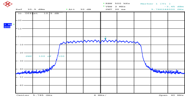
ax20_5785MHz_RU_Full_Chain 1 -3.45dBm/MHz
