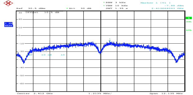
b_2412MHz_Chain 1 -7.89dBm/3kHz
