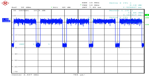
n20_2437MHz_Chain 0 1.286ms,1.530ms
