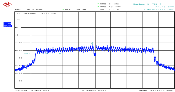
n20_2462MHz_Chain 1 -12.73dBm/3kHz
