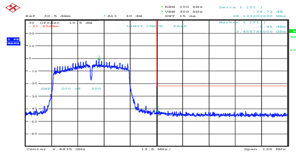
n40_2452MHz_Chain 1 39.72dB
