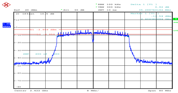
n40_2422MHz_Chain 0 35.300MHz
