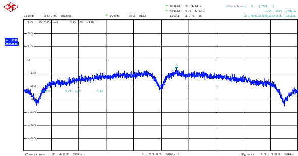
b_2462MHz_Chain 0 -6.90dBm/3kHz
