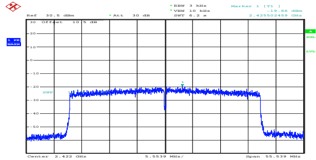
ax40_2422MHz_RU_Full_Chain 1 -19.66dBm/3kHz
