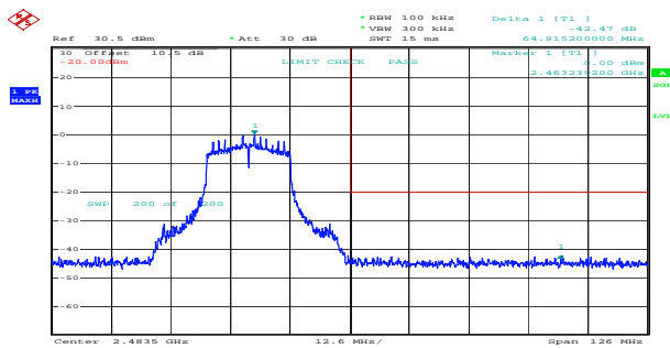
n20_2462MHz_Chain 0 42.47dB
