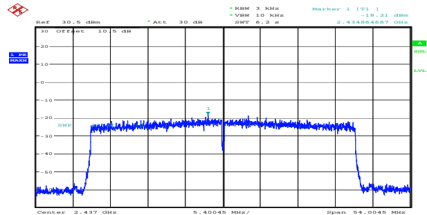
ax40_2437MHz_RU_Full_Chain 1 -18.21dBm/3kHz
