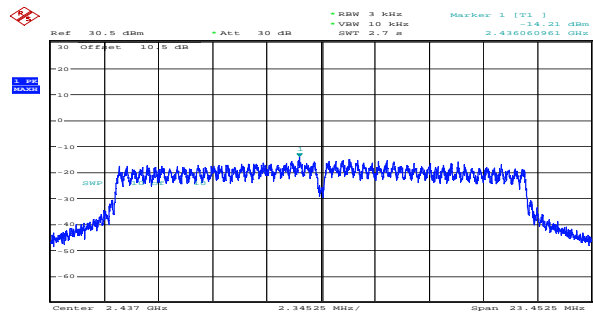
n20_2437MHz_Chain 1 -14.21dBm/3kHz
