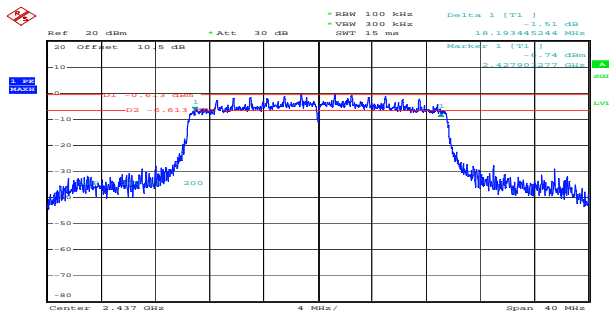
ax20_2437MHz_RU_Full_Chain 0 18.193MHz
