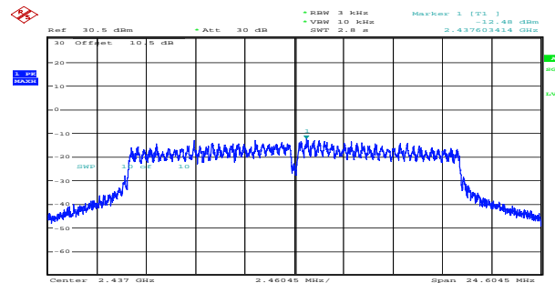
g_2437MHz_Chain 1 -12.48dBm/3kHz
