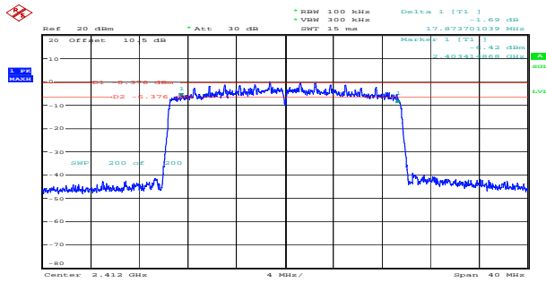
ax20_2412MHz_RU_Full_Chain 0 17.874MHz
