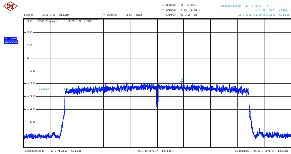
ax40_2422MHz_RU_Full_Chain 0 -19.51dBm/3kHz
