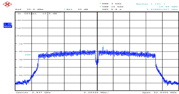
n40_2437MHz_Chain 1 -16.49dBm/3kHz
