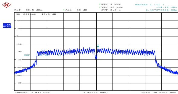
n20_2437MHz_Chain 0 -14.19dBm/3kHz
