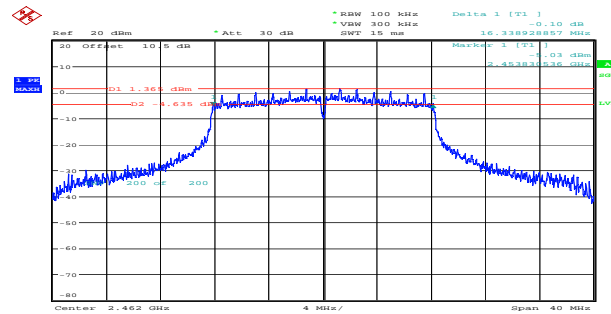
g_2462MHz_Chain 1 16.339MHz
