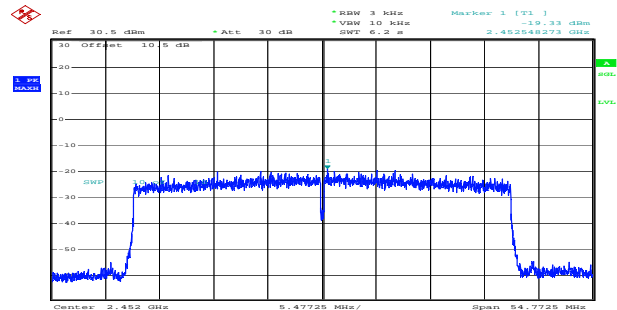
ax40_2452MHz_RU_Full_Chain 1 -19.33dBm/3kHz
