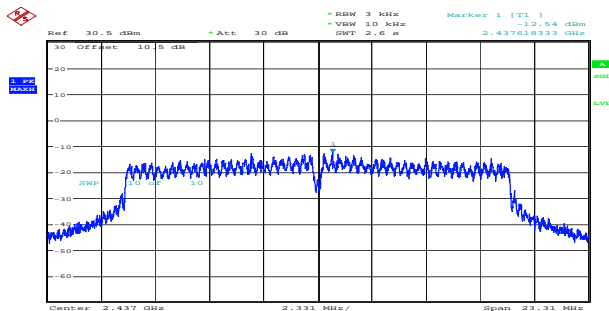
g_2437MHz_Chain 0 -12.54dBm/3kHz
