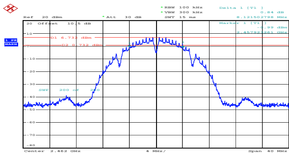
b_2462MHz_Chain 0 8.122MHz
