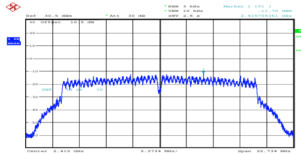
g_2412MHz_Chain 1 -11.70dBm/3kHz
