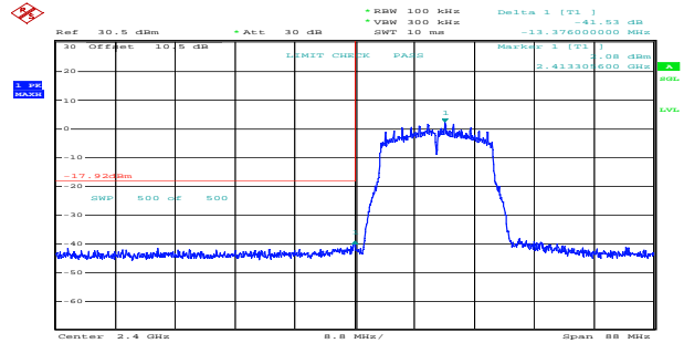
g_2412MHz_Chain 1 41.53dB
