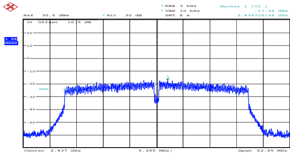
n40_2437MHz_Chain 0 -17.29dBm/3kHz
