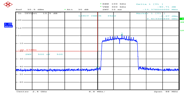
ax20_2412MHz_RU_Full_Chain 1 40.71dB
