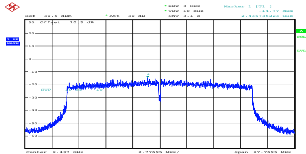
ax20_2437MHz_RU_Full_Chain 1 -14.77dBm/3kHz
