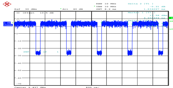
g_2437MHz_Chain 0 1.390ms,1.634ms
