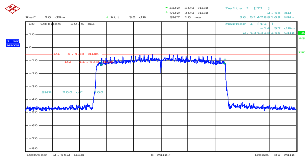
ax40_2452MHz_RU_Full_Chain 1 36.515MHz
