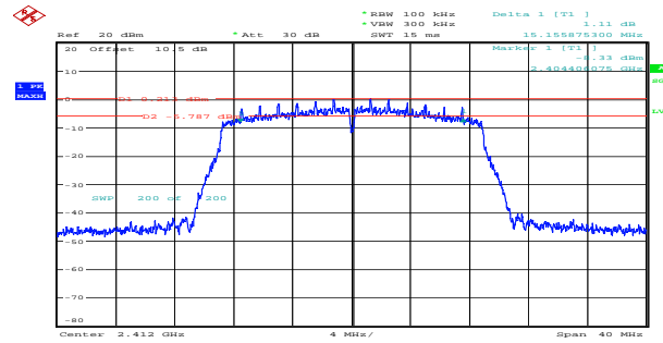
n20_2412MHz_Chain 1 15.156MHz
