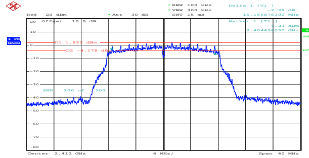
g_2412MHz_Chain 1 15.156MHz
