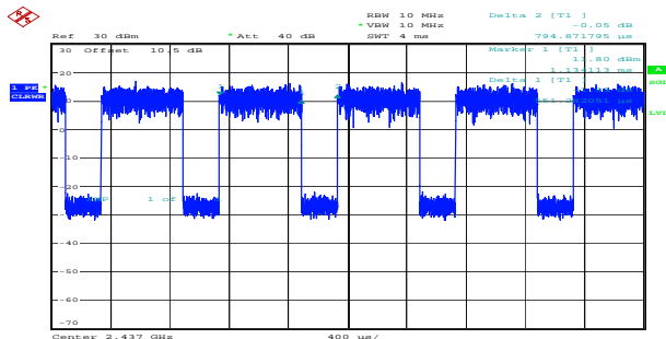
ax20_2437MHz_RU_Full_Chain 0 0.551ms,0.795ms
