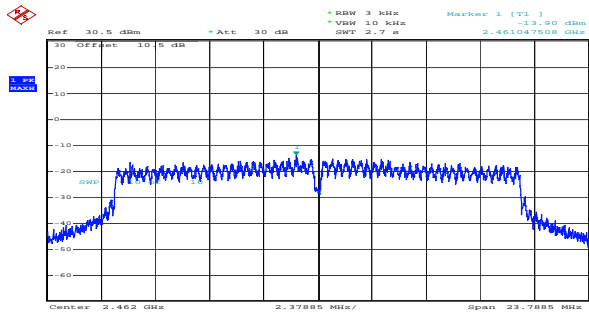
n20_2462MHz_Chain 0 -13.90dBm/3kHz
