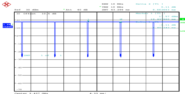
b_2437MHz_Chain 0 8.407ms,8.663ms
