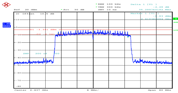
ax40_2437MHz_RU_Full_Chain 0 35.300MHz
