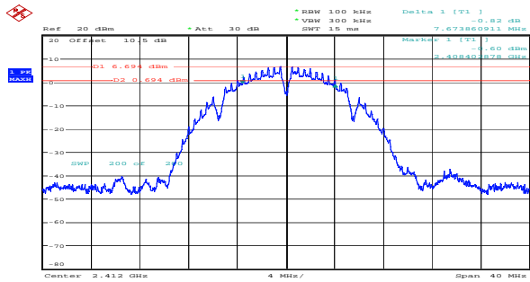
b_2412MHz_Chain 0 7.674MHz
