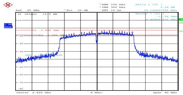
n40_2422MHz_Chain 1 34.149MHz
