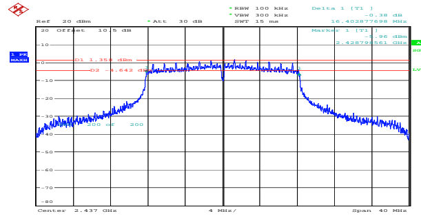
g_2437MHz_Chain 1 16.403MHz
