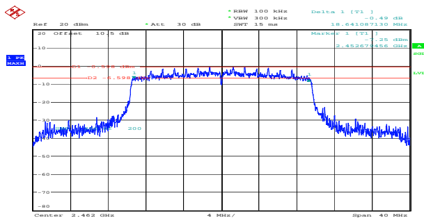
ax20_2462MHz_RU_Full_Chain 0 18.641MHz
