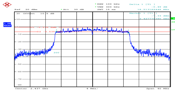
ax20_2437MHz_RU_Full_Chain 1 18.513MHz
