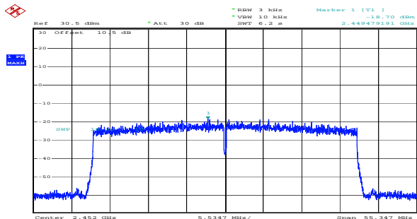
ax40_2452MHz_RU_Full_Chain 0 -18.70dBm/3kHz
