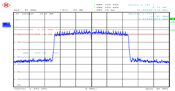
ax40_2452MHz_RU_Full_Chain 0 36.898MHz
