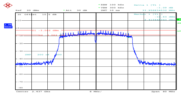
n40_2437MHz_Chain 1 33.957MHz
