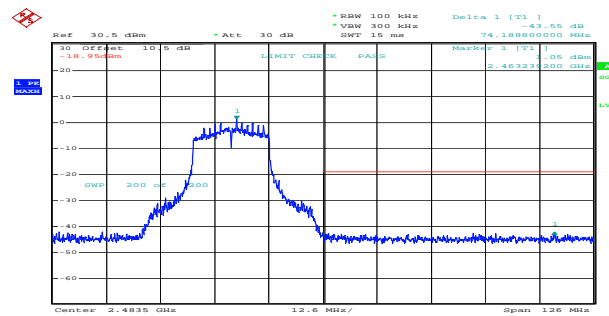
n20_2462MHz_Chain 1 43.55dB
