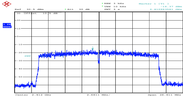
ax20_2412MHz_RU_Full_Chain 0 -16.37dBm/3kHz
