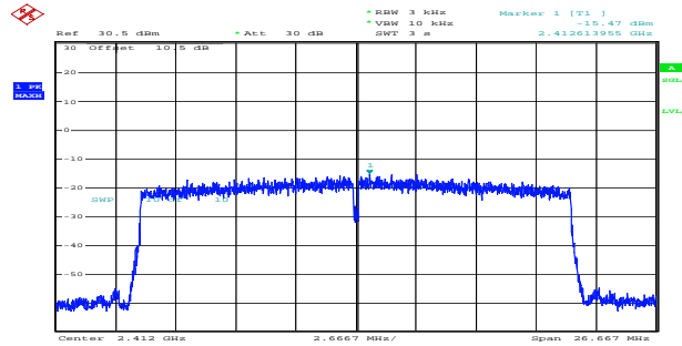
ax20_2412MHz_RU_Full_Chain 1 -15.47dBm/3kHz
