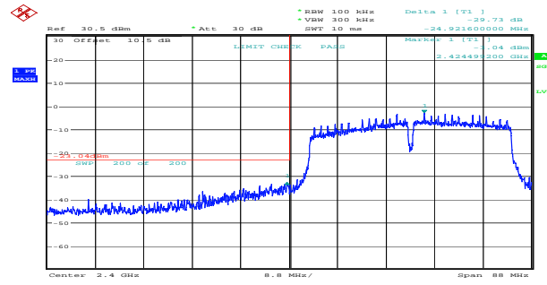
n40_2422MHz_Chain 1 29.73dB
