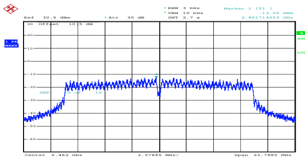
g_2462MHz_Chain 0 -13.05dBm/3kHz
