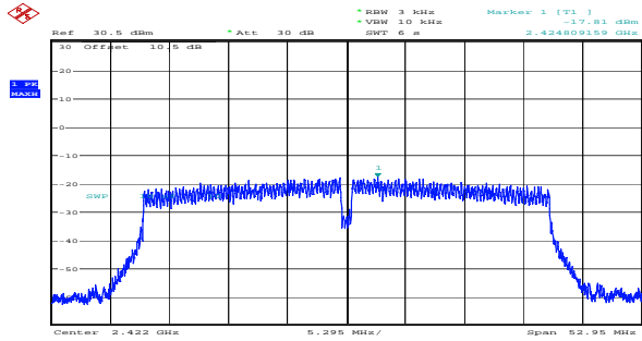
n40_2422MHz_Chain 0 -17.81dBm/3kHz
