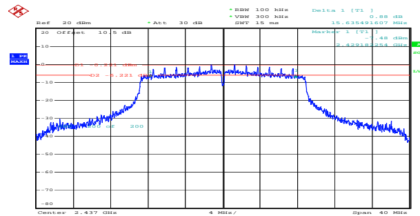
n20_2437MHz_Chain 1 15.635MHz
