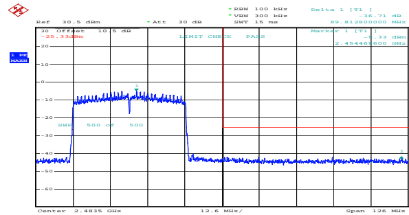
ax40_2452MHz_RU_Full_Chain 1 36.71dB
