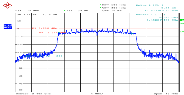
ax20_2462MHz_RU_Full_Chain 1 17.874MHz
