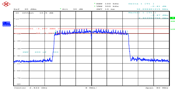
ax40_2422MHz_RU_Full_Chain 0 36.898MHz
