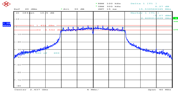
g_2437MHz_Chain 0 15.540MHz
