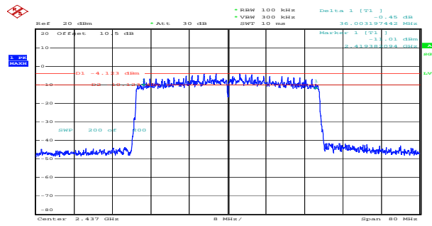
ax40_2437MHz_RU_Full_Chain 1 36.003MHz
