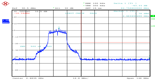
g_2462MHz_Chain 0 43.33dB
