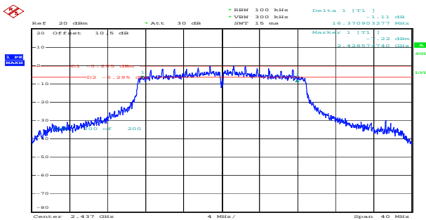
n20_2437MHz_Chain 0 16.371MHz
