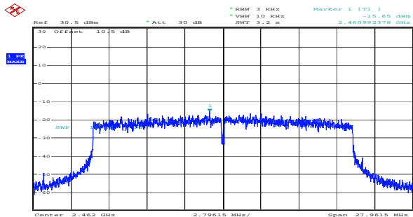
ax20_2462MHz_RU_Full_Chain 0 -15.65dBm/3kHz
