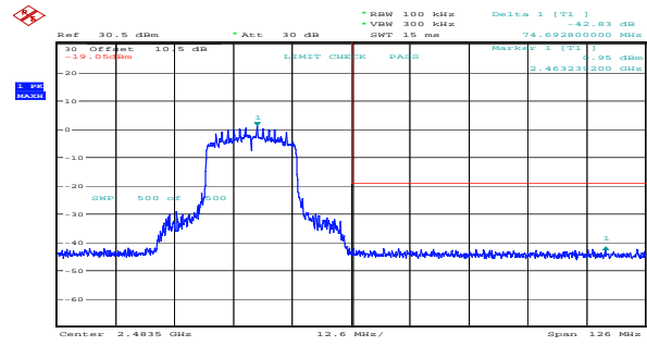
ax20_2462MHz_RU_Full_Chain 1 42.83dB
