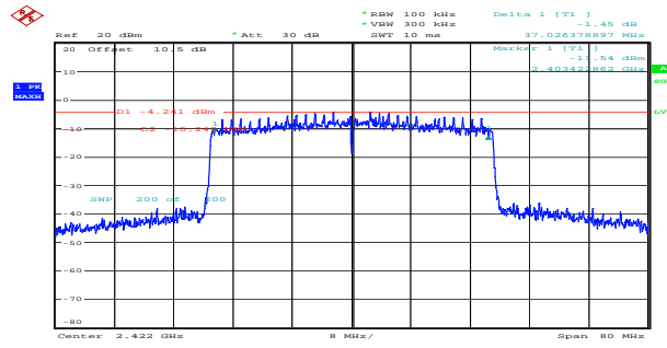
ax40_2422MHz_RU_Full_Chain 1 37.026MHz
