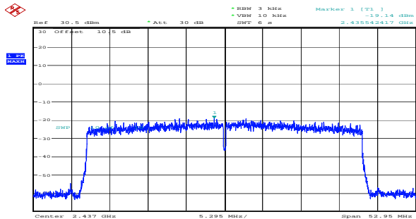
ax40_2437MHz_RU_Full_Chain 0 -19.14dBm/3kHz
