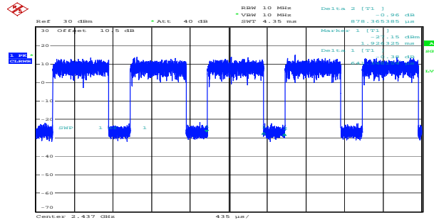
n40_2437MHz_Chain 0 0.641ms,0.878ms
