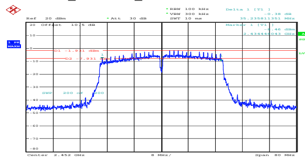
n40_2452MHz_Chain 1 35.236MHz
