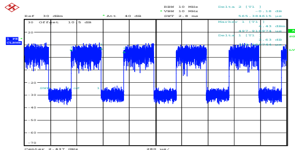
ax40_2437MHz_RU_Full_Chain 0 0.319ms,0.565ms
