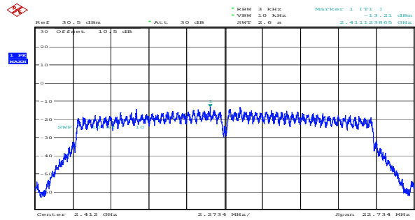
n20_2412MHz_Chain 1 -13.21dBm/3kHz
