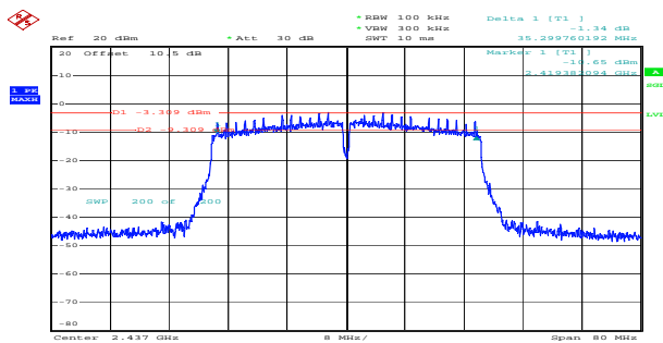
n40_2437MHz_Chain 0 35.300MHz
