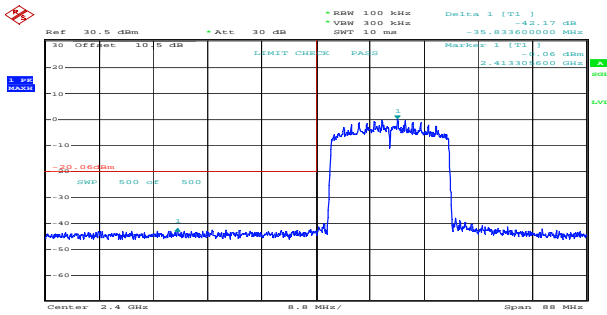
ax20_2412MHz_RU_Full_Chain 0 42.17dB
