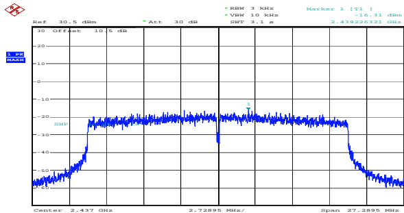
ax20_2437MHz_RU_Full_Chain 0 -16.31dBm/3kHz
