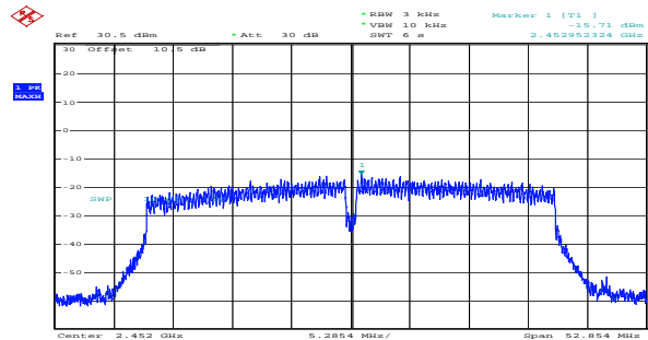
n40_2452MHz_Chain 1 -15.71dBm/3kHz
