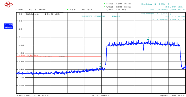
ax40_2422MHz_RU_Full_Chain 1 31.99dB
