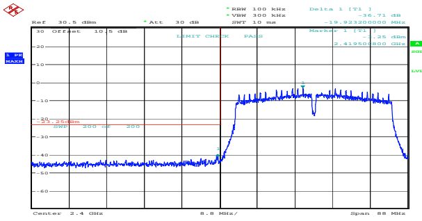
n40_2422MHz_Chain 0 36.71dB
