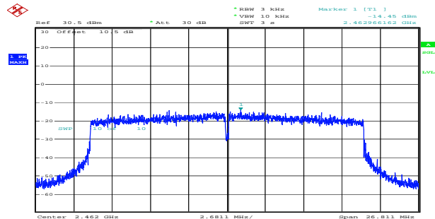
ax20_2462MHz_RU_Full_Chain 1 -14.45dBm/3kHz
