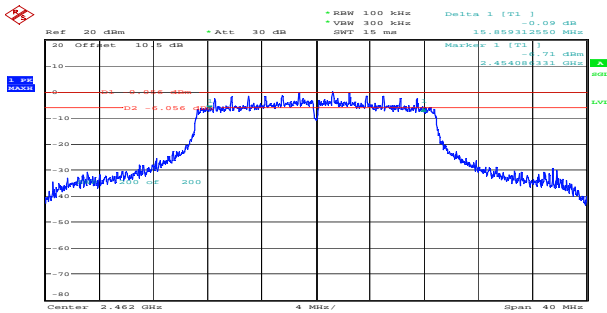
n20_2462MHz_Chain 0 15.859MHz
