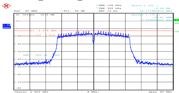
n40_2452MHz_Chain 0 35.172MHz
