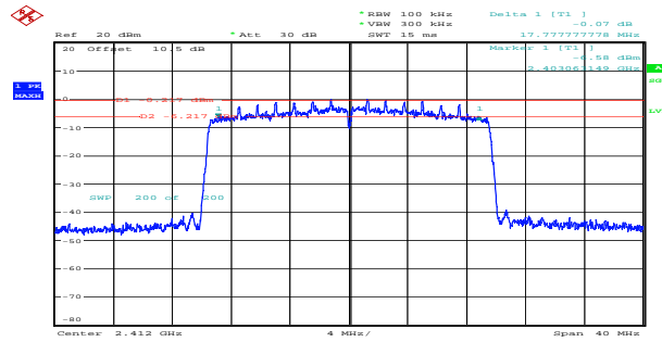
ax20_2412MHz_RU_Full_Chain 1 17.778MHz
