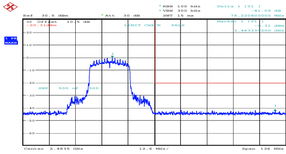
ax20_2462MHz_RU_Full_Chain 0 41.09dB
