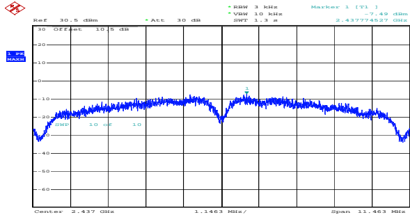
b_2437MHz_Chain 0 -7.49dBm/3kHz
