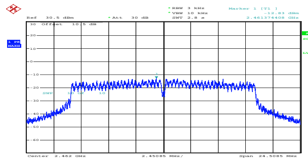
g_2462MHz_Chain 1 -12.83dBm/3kHz
