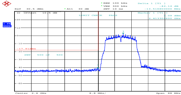
g_2412MHz_Chain 0 42.12dB
