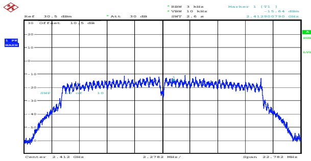
g_2412MHz_Chain 0 -15.64dBm/3kHz
