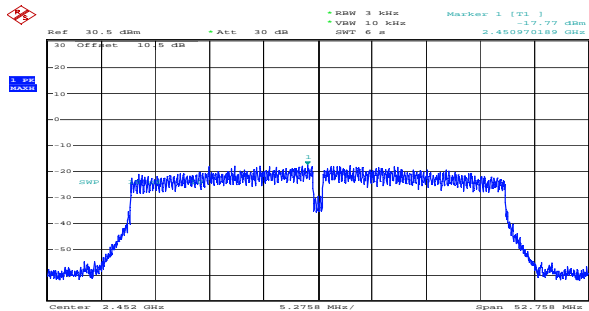
n40_2452MHz_Chain 0 -17.77dBm/3kHz
