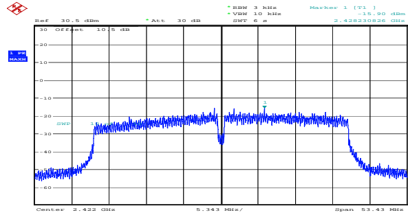
n40_2422MHz_Chain 1 -15.90dBm/3kHz
