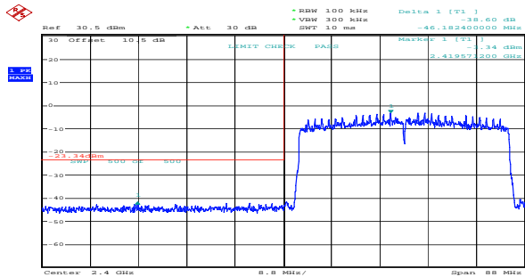
ax40_2422MHz_RU_Full_Chain 0 38.60dB
