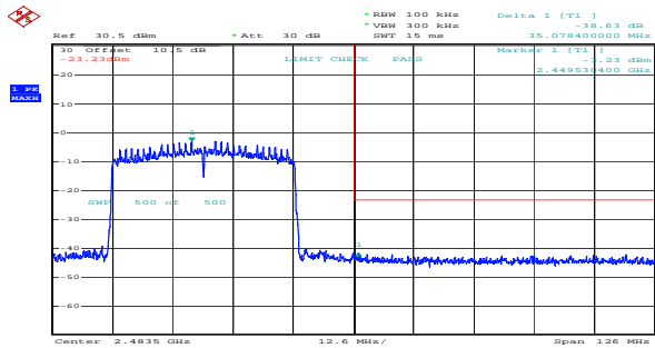
ax40_2452MHz_RU_Full_Chain 0 38.63dB
