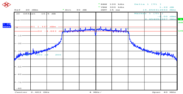
g_2462MHz_Chain 0 15.859MHz
