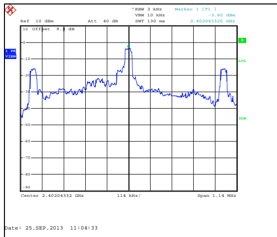
Figure 7.6.2-1: PSD Plot – 2402 MHz
