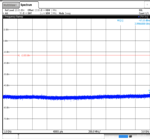
Band17-10MHz-QPSK-23790-1RB#0-1000~3000-PASS
