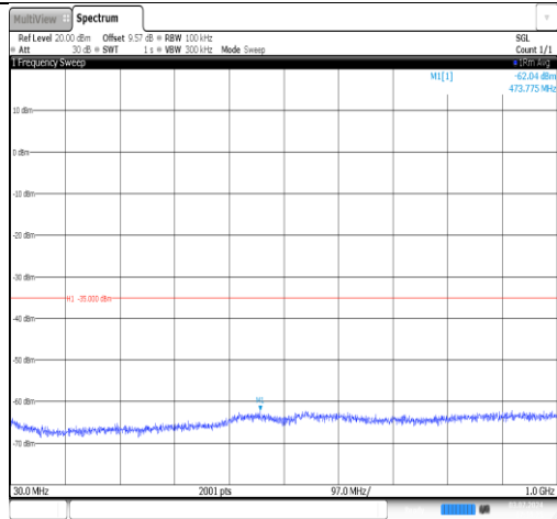
Band7-10MHz-16QAM-21100-1RB#0-20000-PASS
