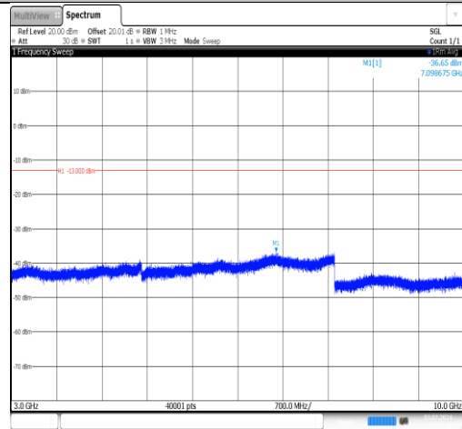
Band17-10MHz-QPSK-23790-1RB#0-3000~10000-PASS
