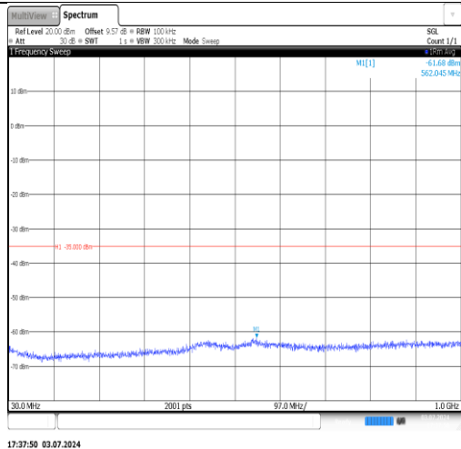
Band7-15MHz-16QAM-21100-1RB#0-20000-PASS
