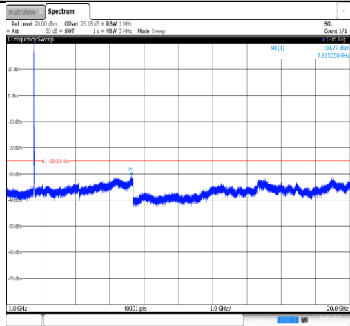
Band7-20MHz-16QAM-20850-1RB#0-1000~20000-PASS
