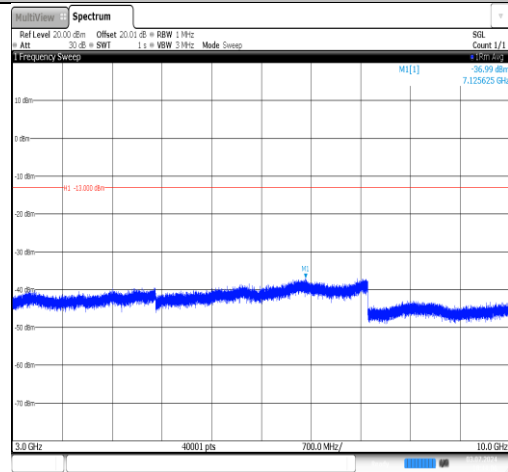
Band17-10MHz-16QAM-23800-1RB#0-3000~10000-PASS
