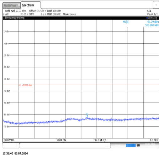
Band7-15MHz-QPSK-20825-1RB#0-20000-PASS
