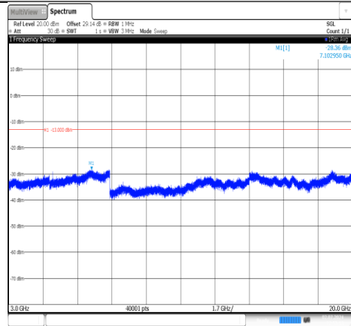
Band4-15MHz-QPSK-20175-1RB#0-3000~20000-PASS
