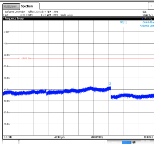
Band5-3MHz-QPSK-20415-1RB#0-3000~10000-PASS
