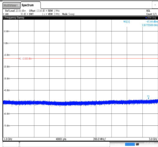
Band5-10MHz-QPSK-20525-1RB#0-1000~3000-PASS
