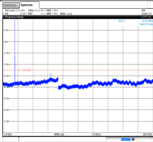
Band7-10MHz-16QAM-20800-1RB#0-1000~20000-PASS
