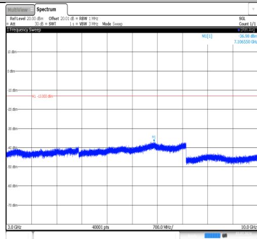
Band5-3MHz-QPSK-20525-1RB#0-3000~10000-PASS
