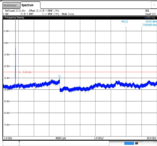
Band7-10MHz-QPSK-21100-1RB#0-1000~20000-PASS
