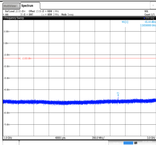
Band5-3MHz-QPSK-20525-1RB#0-1000~3000-PASS
