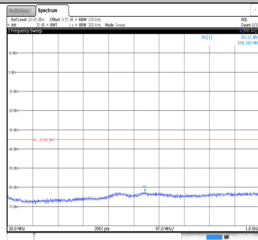
Band7-5MHz-16QAM-20775-1RB#0-30~1000-PASS
