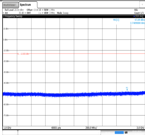
Band5-5MHz-16QAM-20425-1RB#0-1000~3000-PASS
