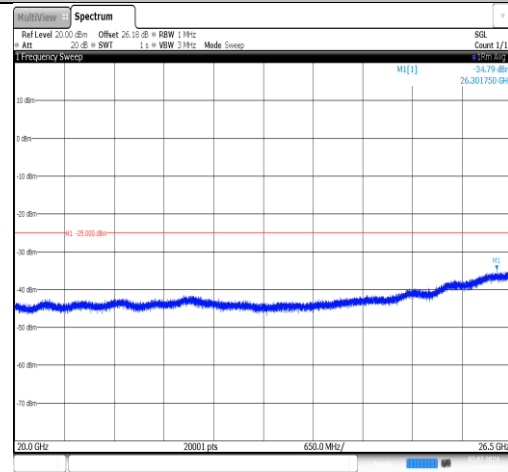
Band7-10MHz-QPSK-21100-1RB#0-20000~26500-PASS
