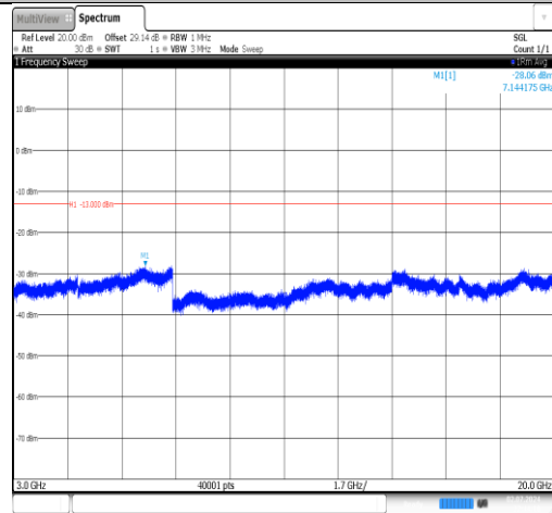
Band4-10MHz-16QAM-20000-1RB#0-3000~20000-PASS
