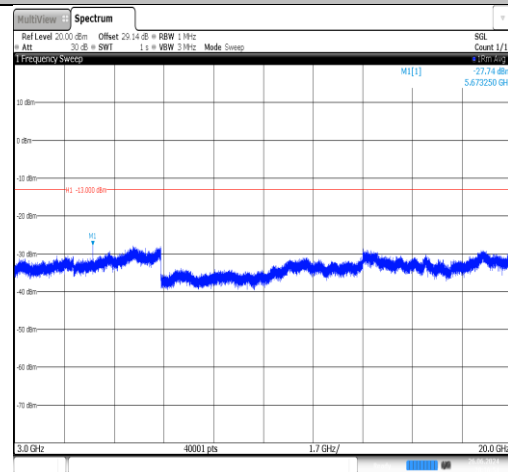
Band2-20MHz-16QAM-19100-1RB#0-3000~20000-PASS
