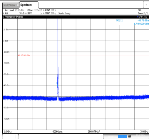
Band4-3MHz-16QAM-20385-1RB#0-1000~3000-PASS
