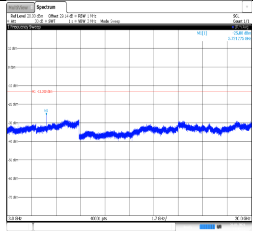
Band2-3MHz-16QAM-19185-1RB#0-3000~20000-PASS
