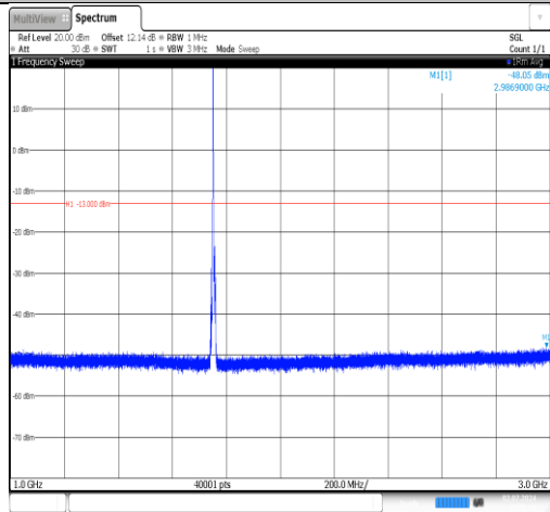
Band4-5MHz-16QAM-20375-1RB#0-1000~3000-PASS
