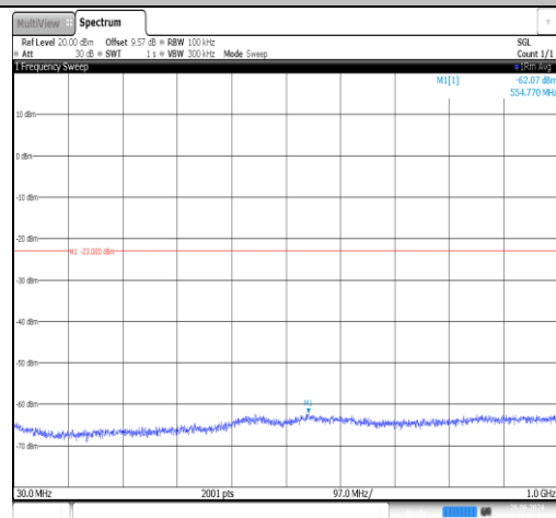
Band2-1.4MHz-16QAM-19193-1RB#0-30~1000-PASS
