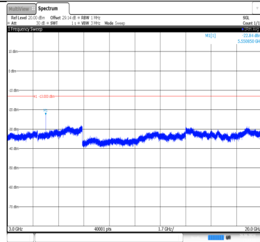
Band2-5MHz-16QAM-18625-1RB#0-3000~20000-PASS
