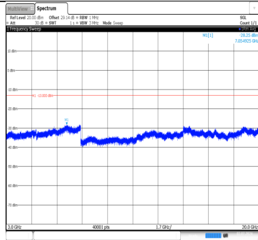
Band4-5MHz-16QAM-20375-1RB#0-3000~20000-PASS
