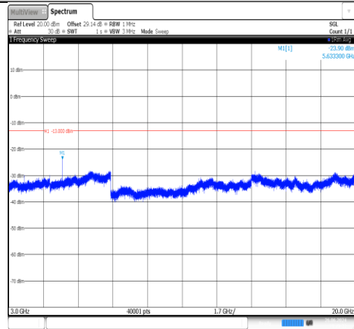
Band2-5MHz-QPSK-18900-1RB#0-3000~20000-PASS
