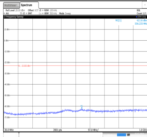
Band4-5MHz-16QAM-20375-1RB#0-30~1000-PASS
