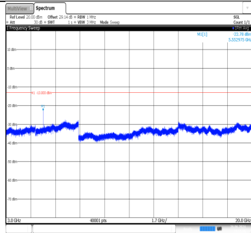
Band2-20MHz-16QAM-18700-1RB#0-3000~20000-PASS
