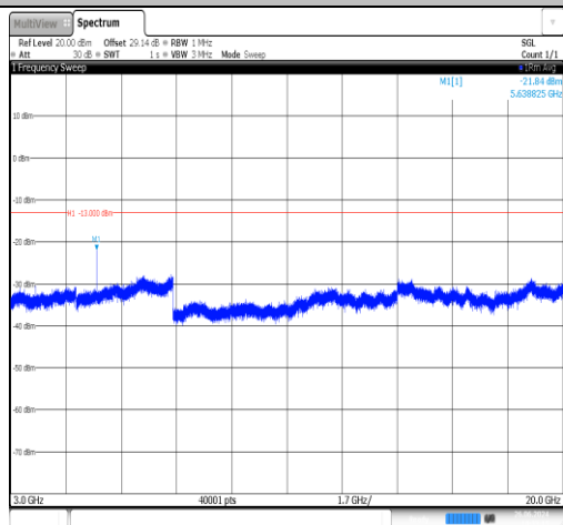
Band2-1.4MHz-16QAM-18900-1RB#0-3000~20000-PASS
