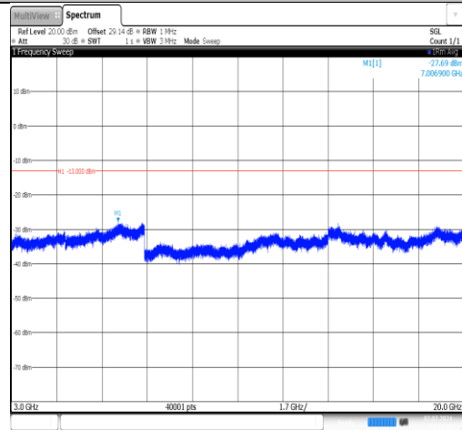
Band4-3MHz-16QAM-20385-1RB#0-3000~20000-PASS
