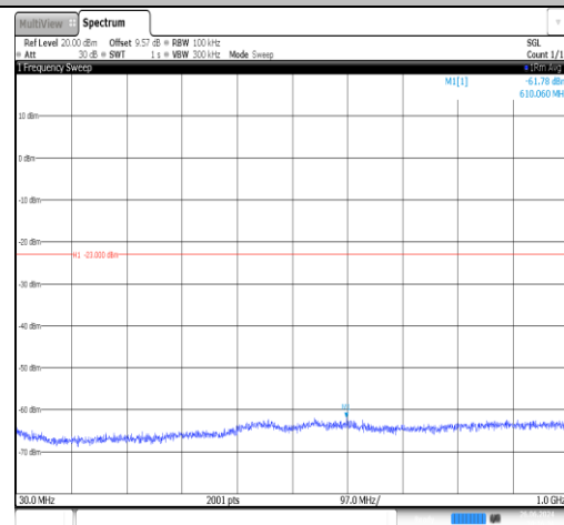
Band2-20MHz-16QAM-19100-1RB#0-30~1000-PASS
