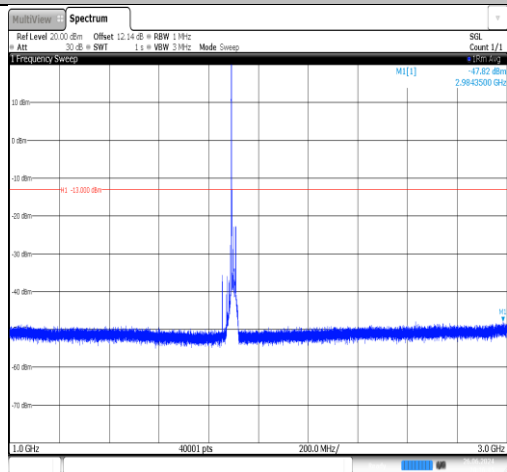
Band2-20MHz-16QAM-19100-1RB#0-1000~3000-PASS
