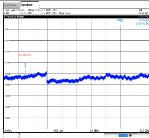
Band2-3MHz-16QAM-18615-1RB#0-3000~20000-PASS
