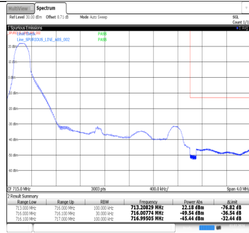
Band12-3MHz-QPSK-23165-1RB#14-PASS
