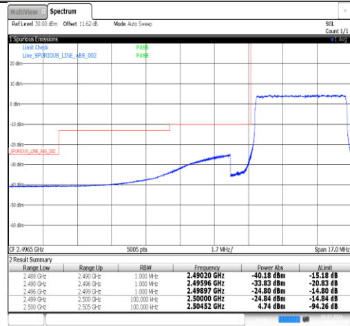
Band7-5MHz-16QAM-20775-25RB#0-PASS
