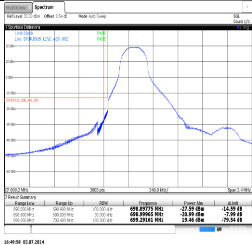
Band12-1.4MHz-16QAM-23017-1RB#5-PASS
