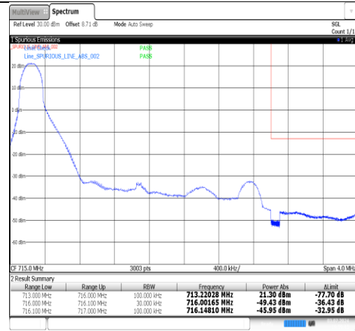
Band12-3MHz-16QAM-23165-1RB#14-PASS
