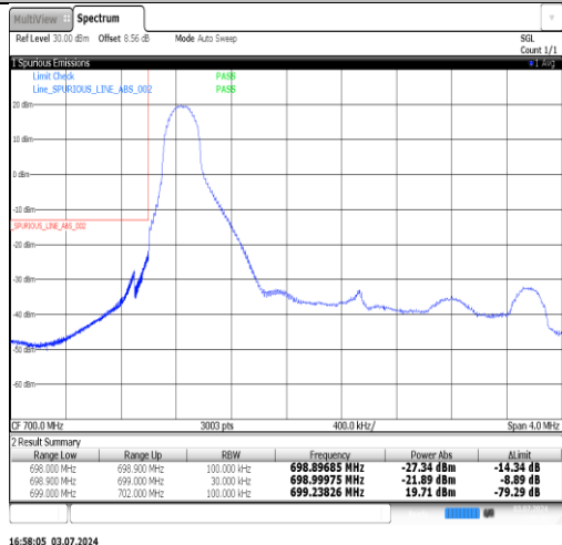
Band12-3MHz-16QAM-23025-1RB#14-PASS
