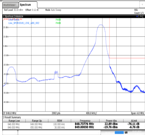
Band5-3MHz-16QAM-20415-15RB#0-PASS
