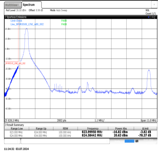
Band5-10MHz-16QAM-20450-1RB#49-PASS
