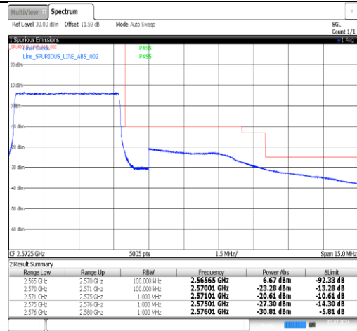
Band7-5MHz-QPSK-21425-1RB#24-Final_1 Integration method
