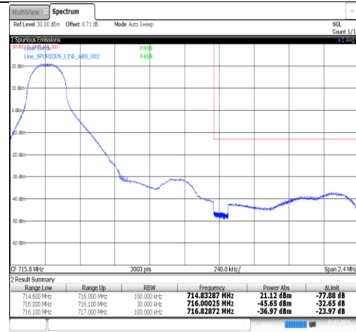
Band12-1.4MHz-16QAM-23173-1RB#5-PASS
