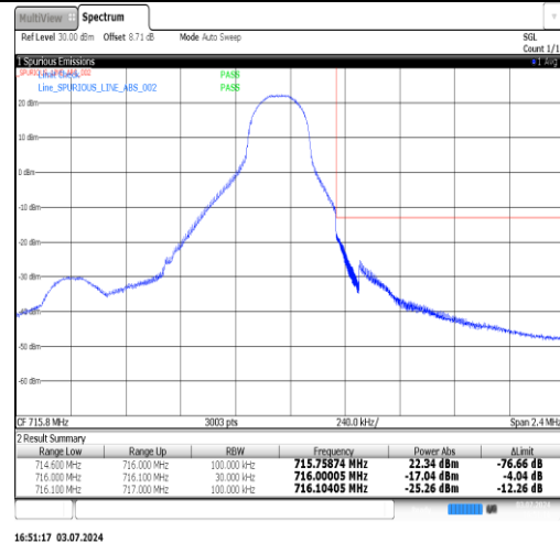
Band12-1.4MHz-16QAM-23017-6RB#0-PASS
