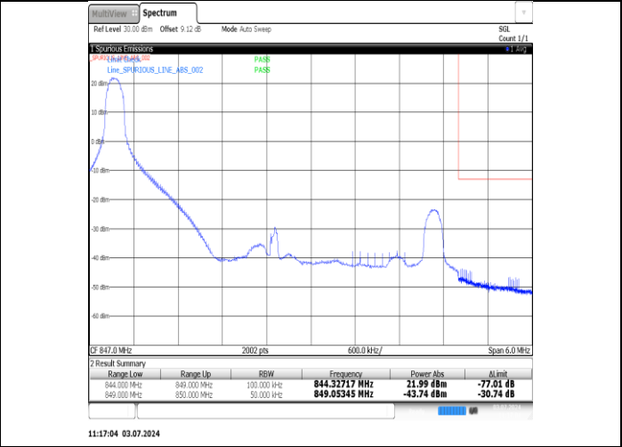
Band5-5MHz-16QAM-20625-1RB#24-PRELIMINARY
