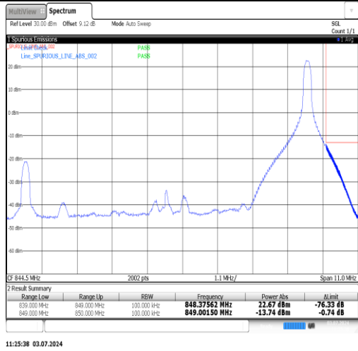
Band5-10MHz-16QAM-20450-50RB#0-PASS
