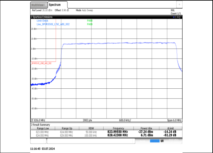
Band5-5MHz-16QAM-20625-1RB#0-PASS
