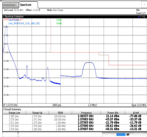
Band7-5MHz-QPSK-21425-1RB#24-PRELIMINARY
