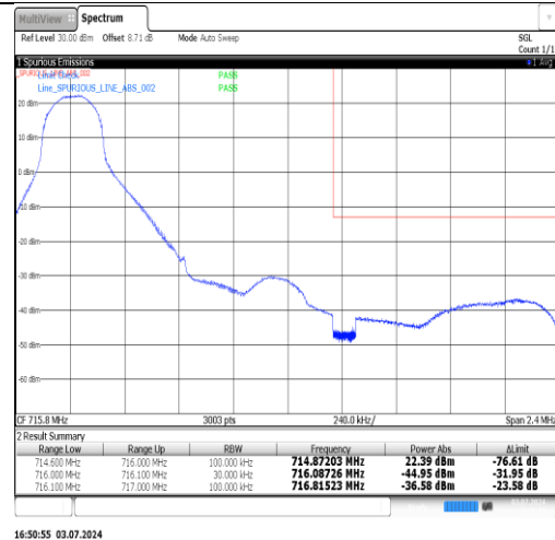
Band12-1.4MHz-QPSK-23173-1RB#5-PASS
