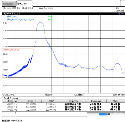
Band12-3MHz-QPSK-23025-1RB#14-PASS
