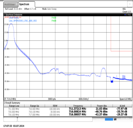
Band12-5MHz-16QAM-23155-1RB#24-PASS
