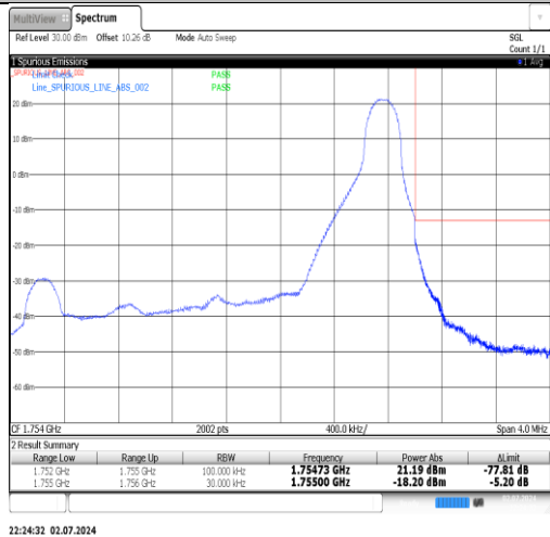
Band4-3MHz-16QAM-19965-15RB#0-PASS
