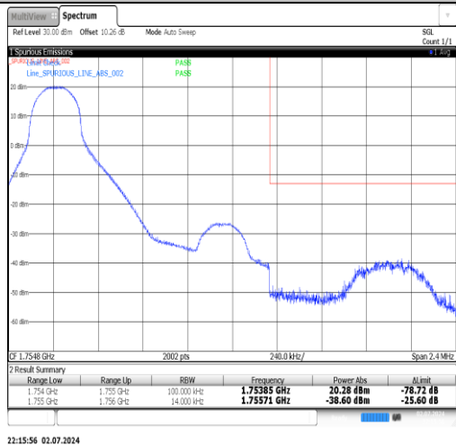
Band4-1.4MHz-16QAM-20393-1RB#5-PASS
