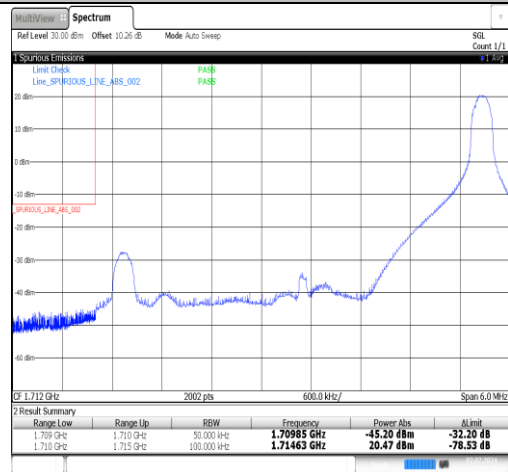
Band4-5MHz-16QAM-20375-25RB#0-PASS
