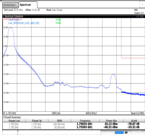
Band4-5MHz-16QAM-20375-1RB#24-PASS
