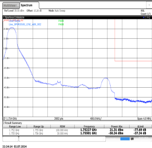
Band4-3MHz-QPSK-20385-1RB#14-PASS
