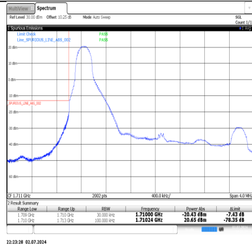
Band4-3MHz-16QAM-19965-1RB#14-PASS
