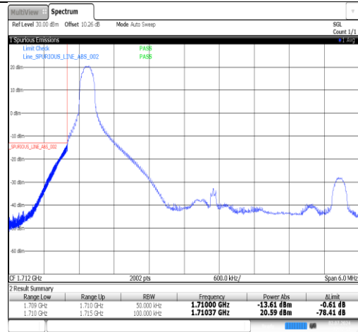
Band4-5MHz-16QAM-19975-1RB#24-PASS
