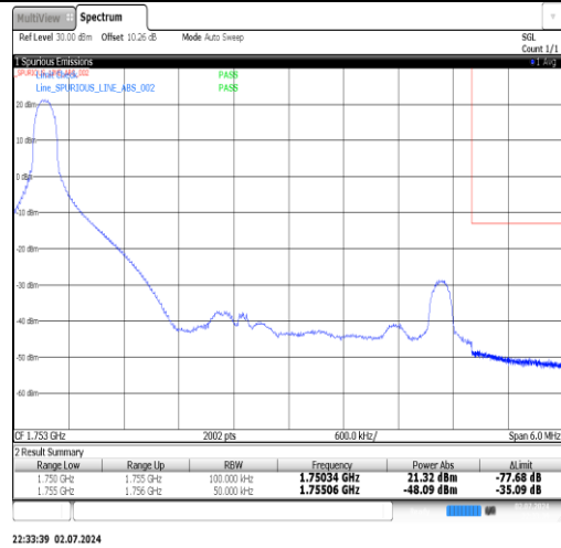
Band4-5MHz-QPSK-20375-1RB#24-PRELIMINARY
