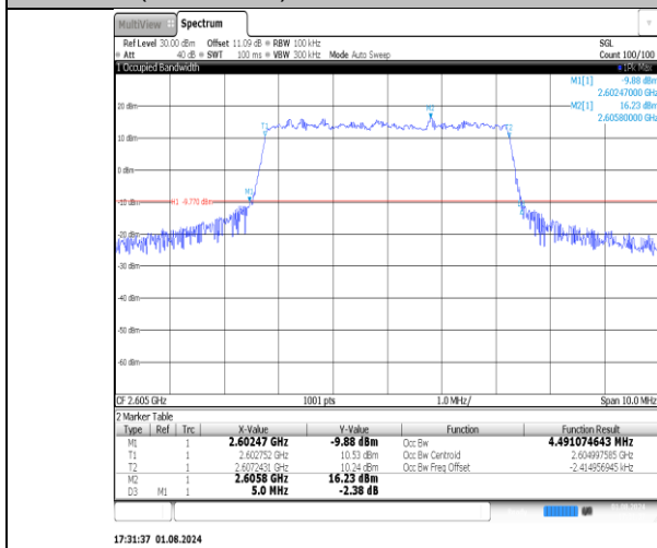
Band41(2560-2650)-5MHz-QPSK-40740-25RB#0-PASS
