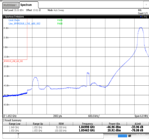
Band2-5MHz-16QAM-19175-25RB#0-PASS
