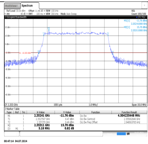
Band40(2350-2360)-10MHz-16QAM-39200-50RB#0-PASS
