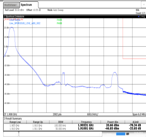
Band2-5MHz-16QAM-19175-1RB#24-PRELIMINARY
