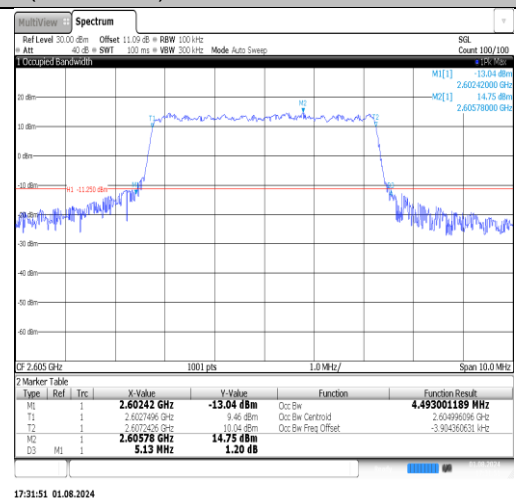
Band41(2560-2650)-5MHz-16QAM-40740-25RB#0-PASS
