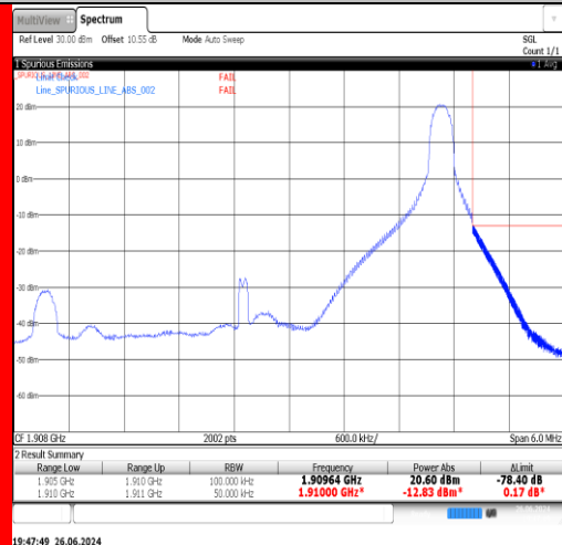
Band2-5MHz-16QAM-19175-1RB#24-PRELIMINARY
