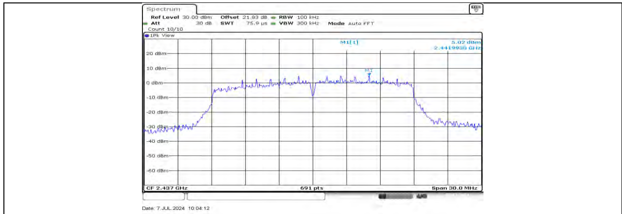
11N20SISO_Ant1_2437_0~Reference
