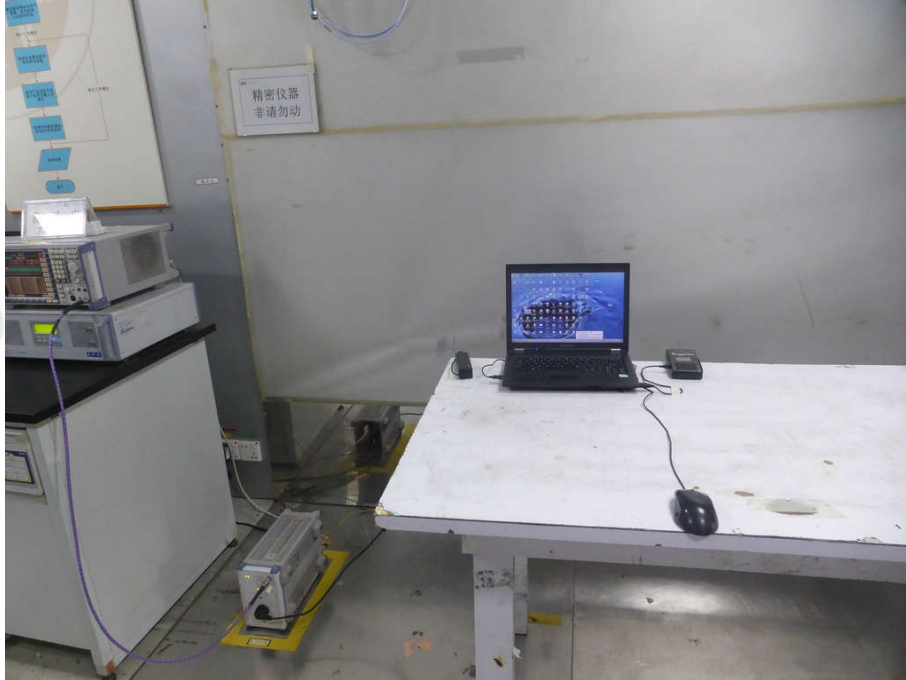
Conducted Emissions
