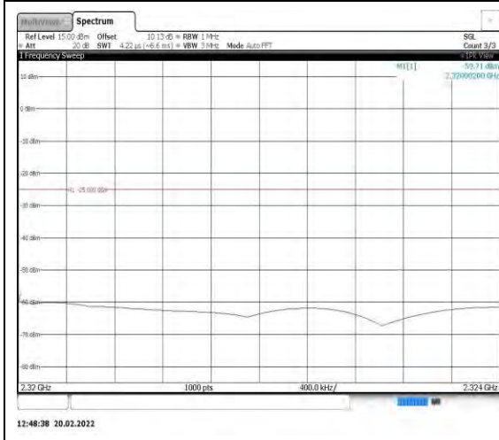
Band40-5MHz-16QAM-38775-1RB#0- Range7:2320~2324MHz
