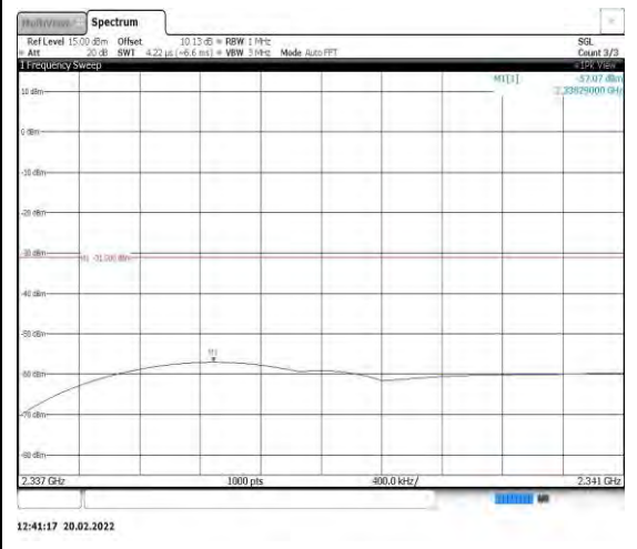
Band40-5MHz-16QAM-38725-1RB#0- Range10:2337~2341MHz
