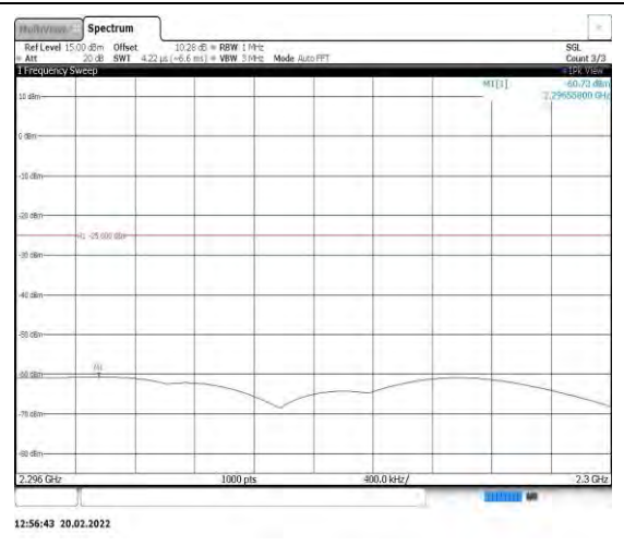
Band40-5MHz-16QAM-39175-1RB#0- Range5:2296~2300MHz
