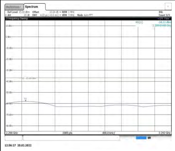
Band40-5MHz-16QAM-39175-1RB#0- Range3:2288~2292MHz
