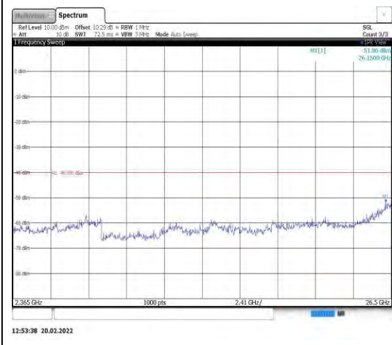
Band40-10MHz-16QAM-38750-1RB#0- Range13:2365~26500MHz
