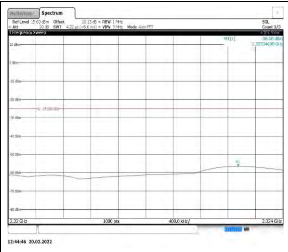
Band40-5MHz-16QAM-38750-1RB#0- Range7:2320~2324MHz
