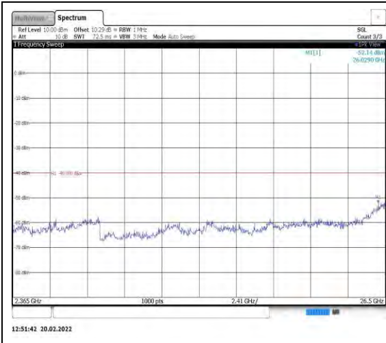
Band40-10MHz-QPSK-38750-1RB#0- Range13:2365~26500MHz
