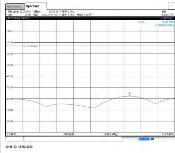
Band40-10MHz-16QAM-39200-1RB#0- Range6:2300~2305MHz
