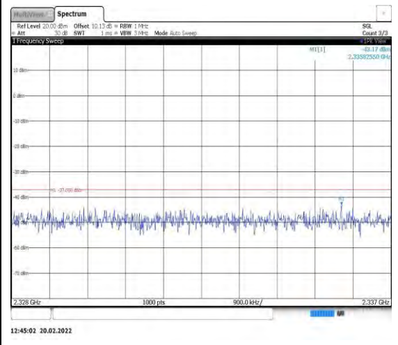
Band40-5MHz-16QAM-38750-1RB#0- Range9:2328~2337MHz
