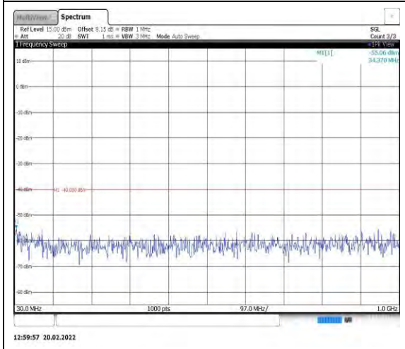
Band40-5MHz-16QAM-39200-1RB#0- Range1:30~1000MHz
