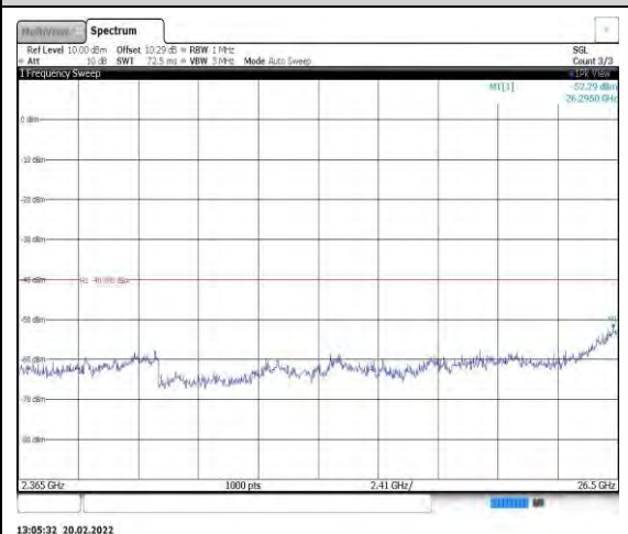
Band40-5MHz-16QAM-39225-1RB#0- Range13:2365~26500MHz
