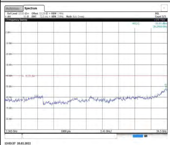
Band40-5MHz-QPSK-39225-1RB#0- Range13:2365~26500MHz
