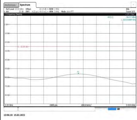
Band40-10MHz-16QAM-39200-1RB#0- Range7:2320~2324MHz
