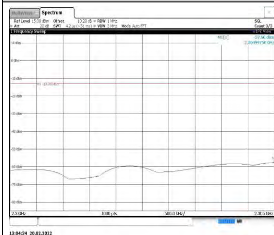
Band40-5MHz-16QAM-39225-1RB#0- Range6:2300~2305MHz
