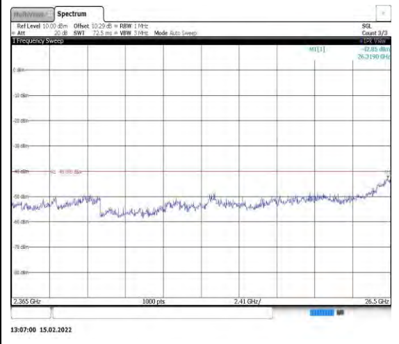
Band40-10MHz-16QAM-39200-1RB#0- Range13:2365~26500MHz
