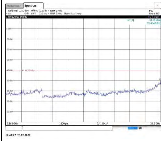
Band40-5MHz-16QAM-38775-1RB#0- Range13:2365~26500MHz
