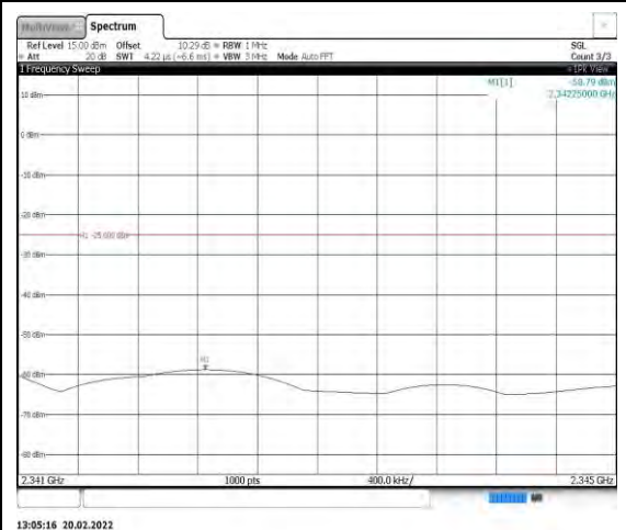
Band40-5MHz-16QAM-39225-1RB#0- Range11:2341~2345MHz
