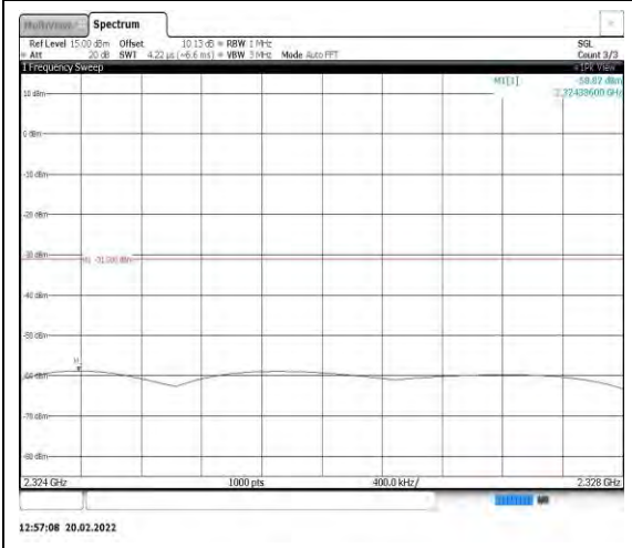
Band40-5MHz-16QAM-39175-1RB#0- Range8:2324~2328MHz
