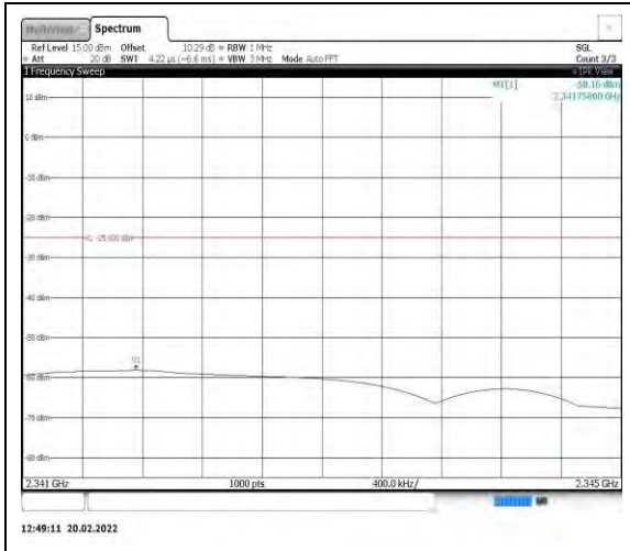
Band40-5MHz-16QAM-38775-1RB#0- Range11:2341~2345MHz
