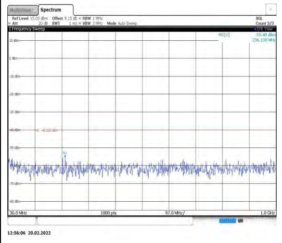
Band40-5MHz-16QAM-39175-1RB#0- Range1:30~1000MHz
