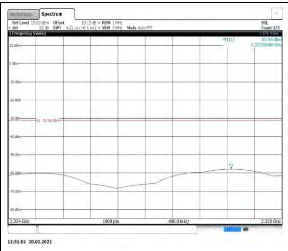
Band40-10MHz-QPSK-38750-1RB#0- Range8:2324~2328MHz
