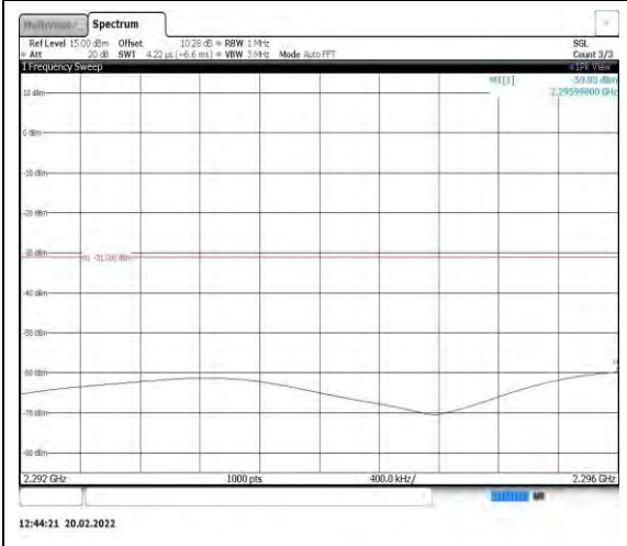
Band40-5MHz-16QAM-38750-1RB#0- Range4:2292~2296MHz
