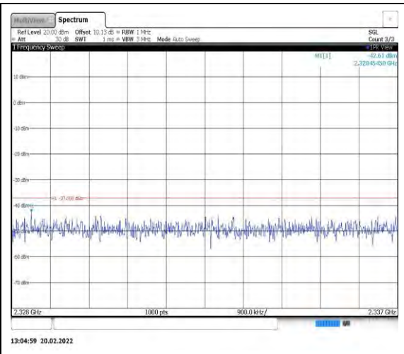
Band40-5MHz-16QAM-39225-1RB#0- Range9:2328~2337MHz
