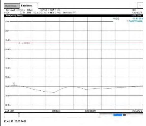
Band40-5MHz-16QAM-38725-1RB#0- Range12:2360~2365MHz
