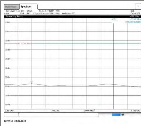
Band40-5MHz-16QAM-38775-1RB#0- Range12:2360~2365MHz
