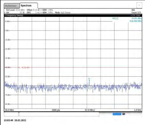
Band40-5MHz-16QAM-39225-1RB#0- Range1:30~1000MHz
