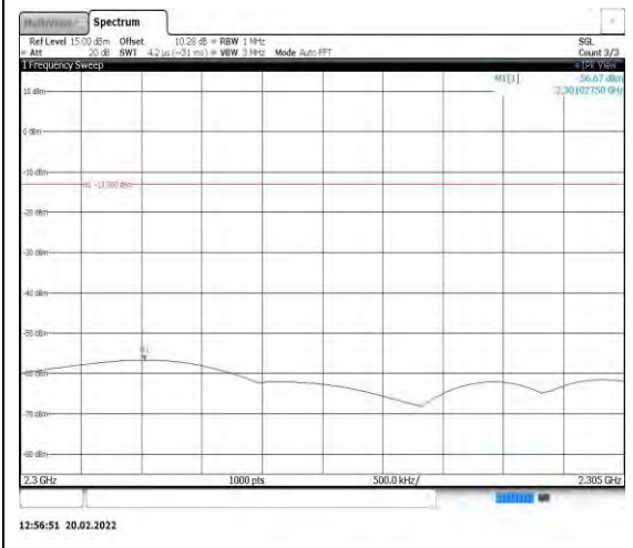
Band40-5MHz-16QAM-39175-1RB#0- Range6:2300~2305MHz
