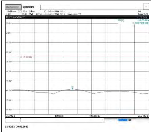
Band40-5MHz-16QAM-38725-1RB#0- Range7:2320~2324MHz
