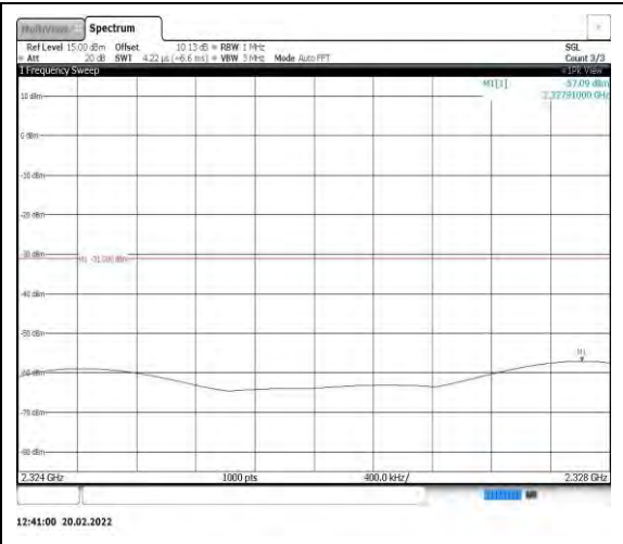
Band40-5MHz-16QAM-38725-1RB#0- Range8:2324~2328MHz
