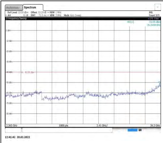
Band40-5MHz-16QAM-38725-1RB#0- Range13:2365~26500MHz
