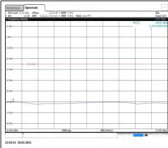
Band40-10MHz-16QAM-38750-1RB#0- Range11:2341~2345MHz
