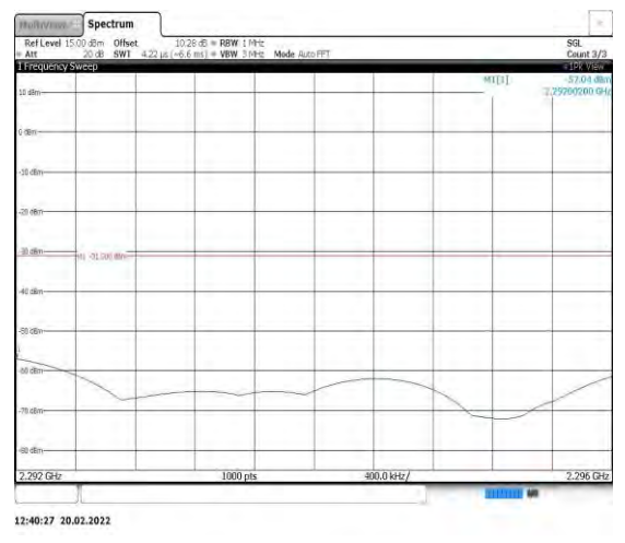
Band40-5MHz-16QAM-38725-1RB#0- Range4:2292~2296MHz
