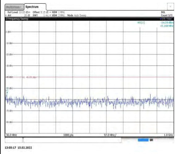
Band40-10MHz-16QAM-39200-1RB#0- Range1:30~1000MHz
