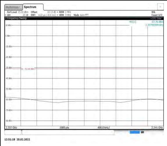
Band40-10MHz-QPSK-38750-1RB#0- Range10:2337~2341MHz
