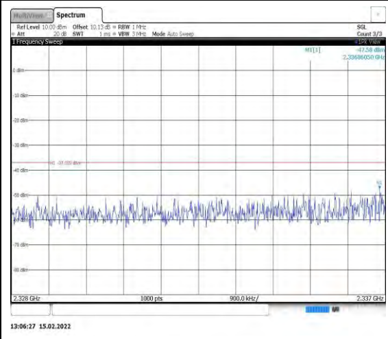
Band40-10MHz-16QAM-39200-1RB#0- Range9:2328~2337MHz
