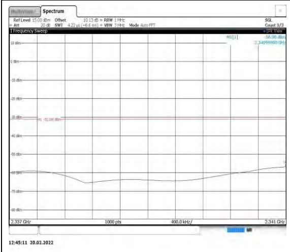
Band40-5MHz-16QAM-38750-1RB#0- Range10:2337~2341MHz
