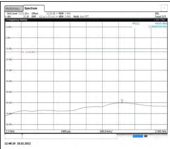
Band40-5MHz-16QAM-38775-1RB#0- Range6:2300~2305MHz
