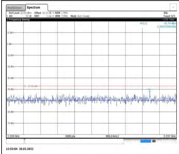
Band40-10MHz-16QAM-38750-1RB#0- Range9:2328~2337MHz
