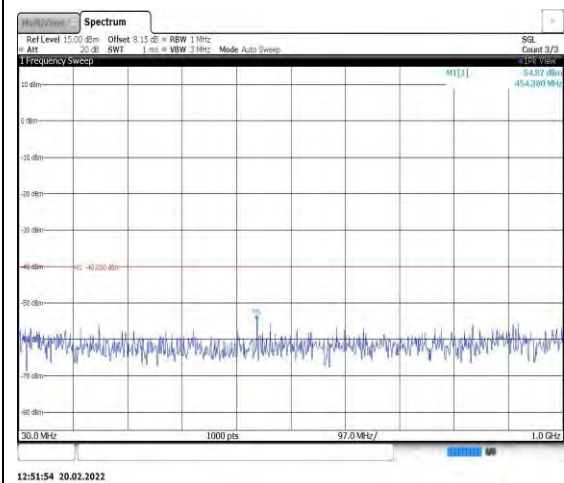
Band40-10MHz-16QAM-38750-1RB#0- Range1:30~1000MHz
