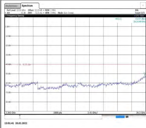
Band40-5MHz-16QAM-39200-1RB#0- Range13:2365~26500MHz
