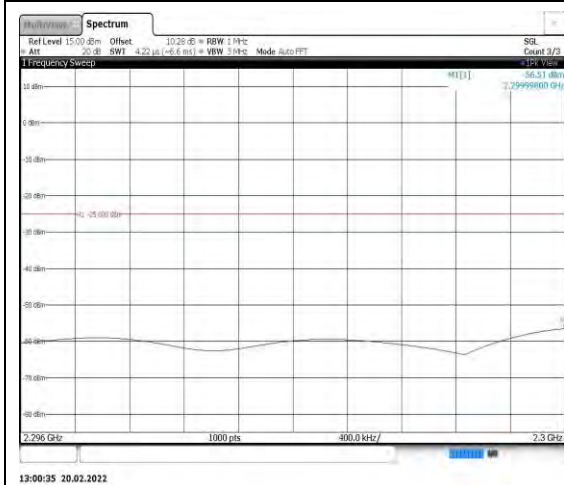
Band40-5MHz-16QAM-39200-1RB#0- Range5:2296~2300MHz
