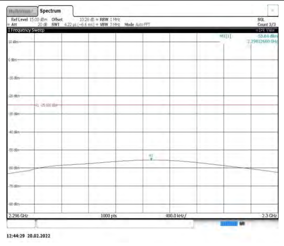
Band40-5MHz-16QAM-38750-1RB#0- Range5:2296~2300MHz
