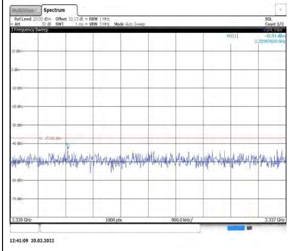
Band40-5MHz-16QAM-38725-1RB#0- Range9:2328~2337MHz
