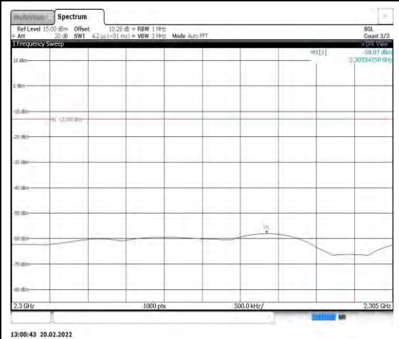
Band40-5MHz-16QAM-39200-1RB#0- Range6:2300~2305MHz
