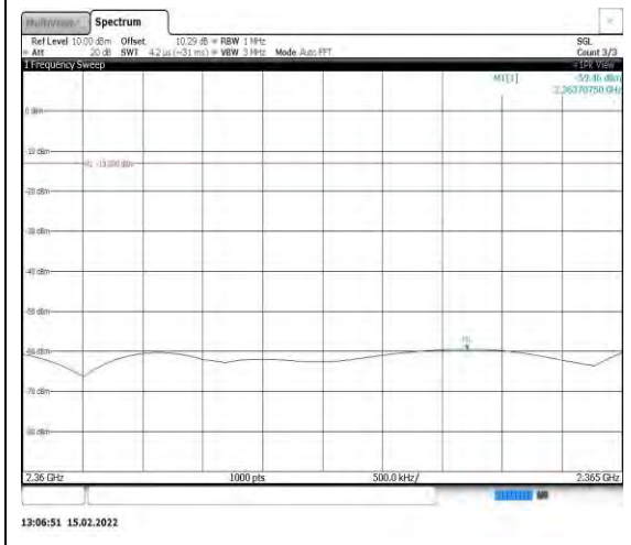
Band40-10MHz-16QAM-39200-1RB#0- Range12:2360~2365MHz
