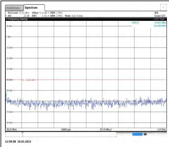
Band40-5MHz-16QAM-38725-1RB#0- Range1:30~1000MHz
