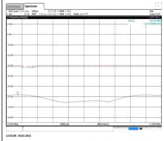
Band40-10MHz-16QAM-38750-1RB#0- Range8:2324~2328MHz
