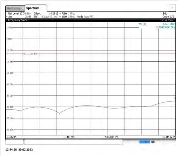
Band40-5MHz-16QAM-38750-1RB#0- Range6:2300~2305MHz
