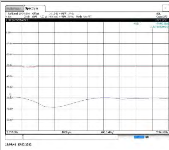
Band40-10MHz-QPSK-39200-1RB#0- Range10:2337~2341MHz
