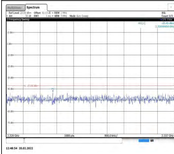
Band40-5MHz-16QAM-38775-1RB#0- Range9:2328~2337MHz
