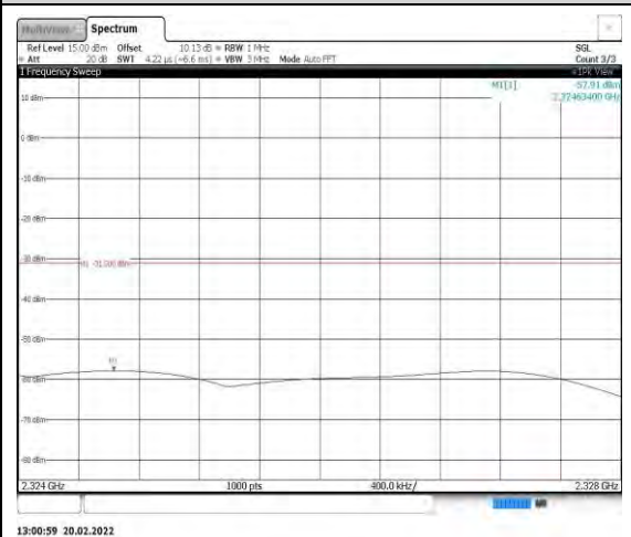
Band40-5MHz-16QAM-39200-1RB#0- Range8:2324~2328MHz
