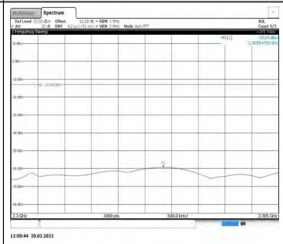
Band40-10MHz-QPSK-38750-1RB#0- Range6:2300~2305MHz
