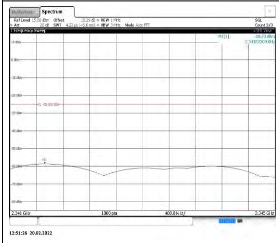
Band40-10MHz-QPSK-38750-1RB#0- Range11:2341~2345MHz
