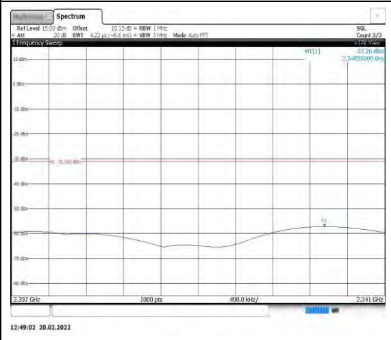
Band40-5MHz-16QAM-38775-1RB#0- Range10:2337~2341MHz
