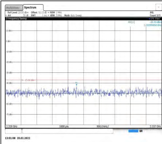
Band40-5MHz-16QAM-39200-1RB#0- Range9:2328~2337MHz
