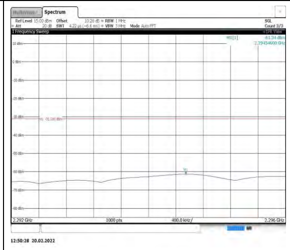
Band40-10MHz-QPSK-38750-1RB#0- Range4:2292~2296MHz
