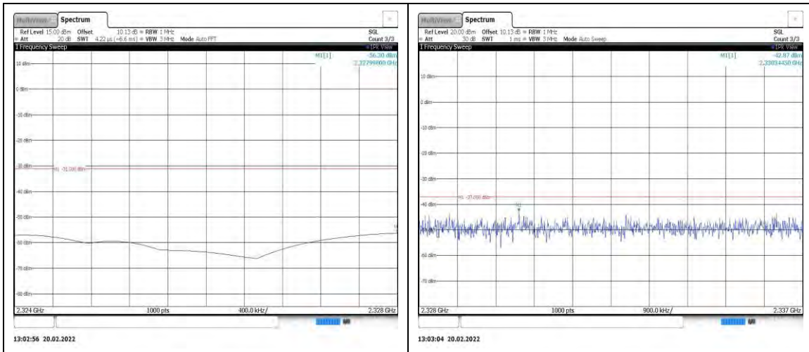
Band40-5MHz-QPSK-39225-1RB#0- Range8:2324~2328MHz
