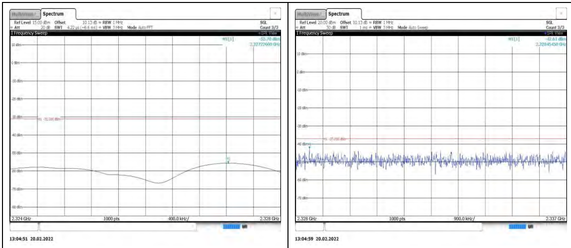
Band40-5MHz-16QAM-39225-1RB#0- Range8:2324~2328MHz
