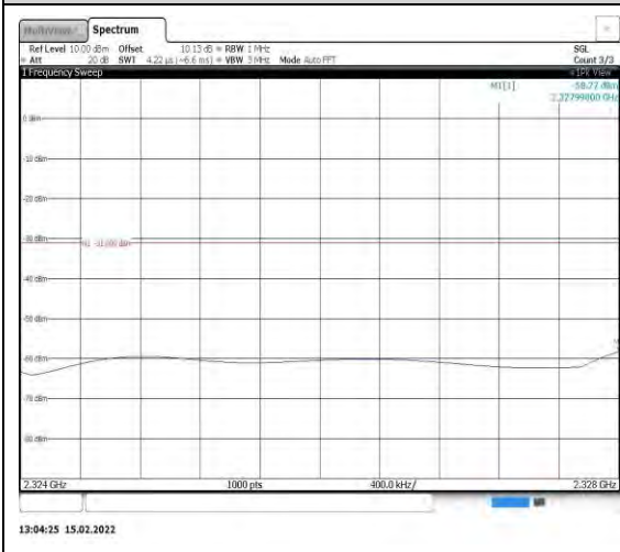
Band40-10MHz-QPSK-39200-1RB#0- Range8:2324~2328MHz
