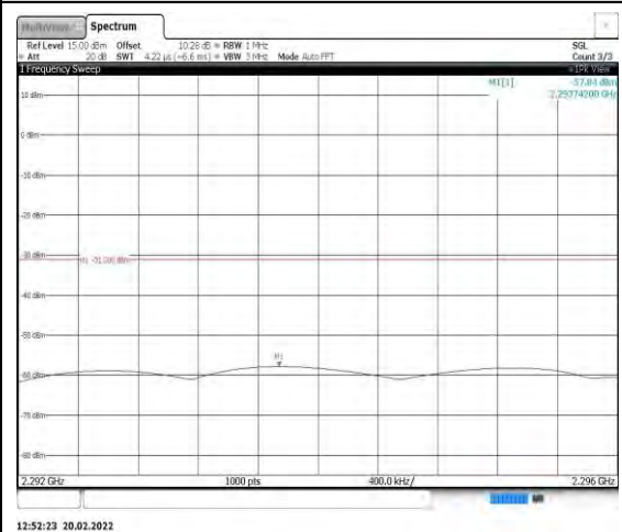
Band40-10MHz-16QAM-38750-1RB#0- Range4:2292~2296MHz
