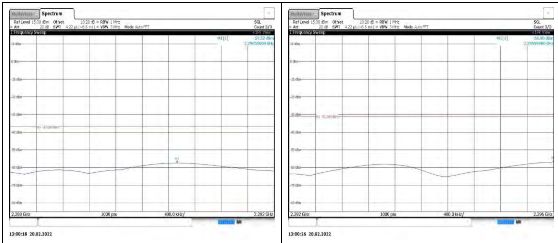
Band40-5MHz-16QAM-39200-1RB#0- Range3:2288~2292MHz
