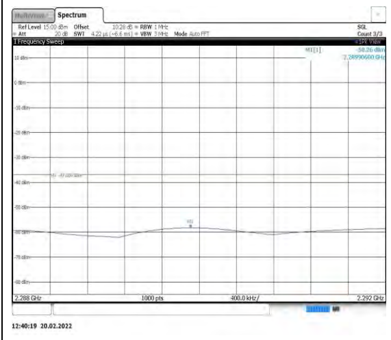
Band40-5MHz-16QAM-38725-1RB#0- Range3:2288~2292MHz
