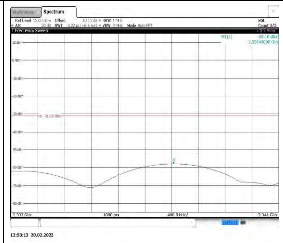
Band40-10MHz-16QAM-38750-1RB#0- Range10:2337~2341MHz
