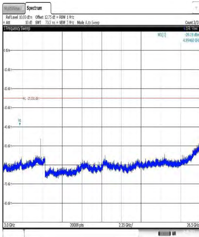
Band41-20MHz-16QAM-39750-1RB#0-Range3:3000~26500MHz
