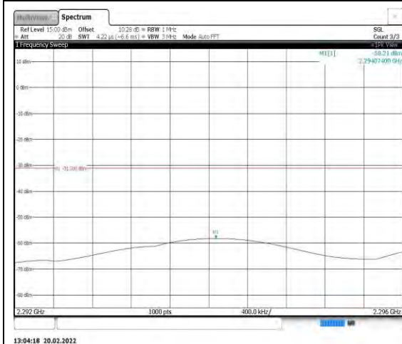
Band40-5MHz-16QAM-39225-1RB#0- Range4:2292~2296MHz
