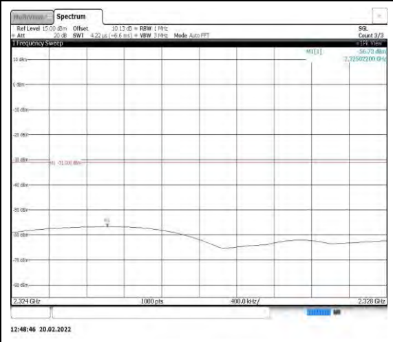
Band40-5MHz-16QAM-38775-1RB#0- Range8:2324~2328MHz
