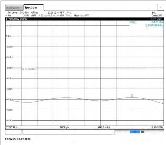
Band40-5MHz-16QAM-39175-1RB#0- Range4:2292~2296MHz
