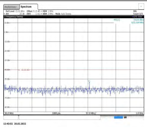
Band40-5MHz-16QAM-38750-1RB#0- Range1:30~1000MHz
