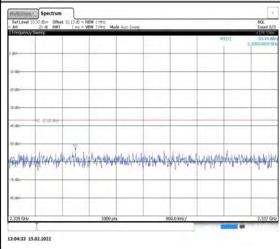
Band40-10MHz-QPSK-39200-1RB#0- Range9:2328~2337MHz
