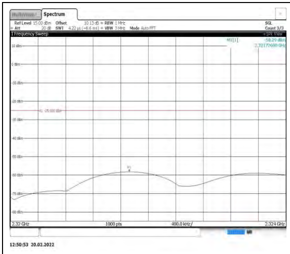
Band40-10MHz-QPSK-38750-1RB#0- Range7:2320~2324MHz
