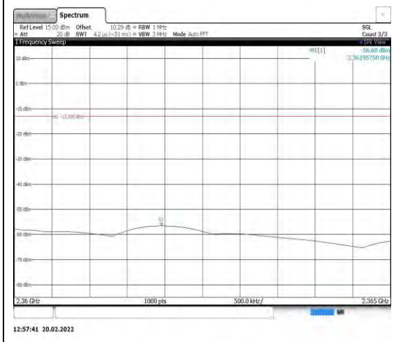
Band40-5MHz-16QAM-39175-1RB#0- Range12:2360~2365MHz
