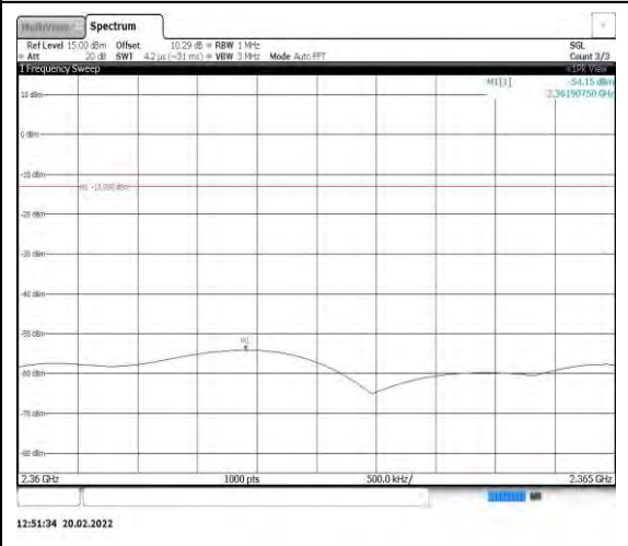
Band40-10MHz-QPSK-38750-1RB#0- Range12:2360~2365MHz
