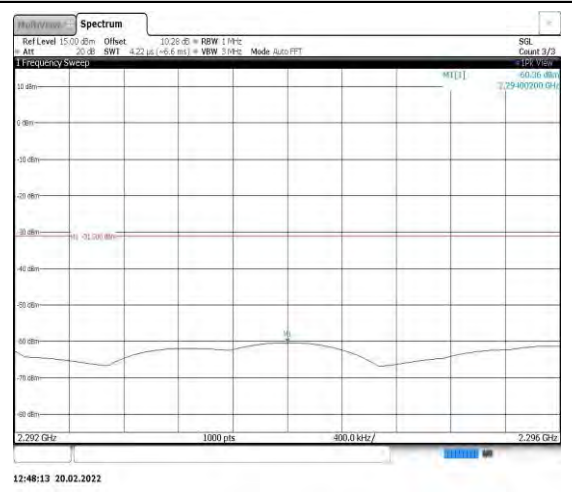
Band40-5MHz-16QAM-38775-1RB#0- Range4:2292~2296MHz
