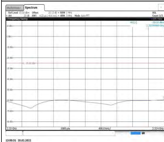
Band40-5MHz-16QAM-39200-1RB#0- Range7:2320~2324MHz
