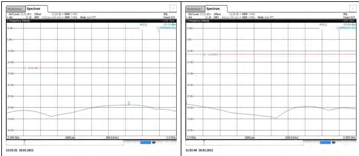
Band40-10MHz-16QAM-38750-1RB#0- Range5:2296~2300MHz
