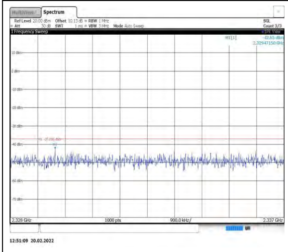
Band40-10MHz-QPSK-38750-1RB#0- Range9:2328~2337MHz
