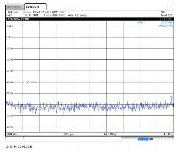
Band40-5MHz-16QAM-38775-1RB#0- Range1:30~1000MHz
