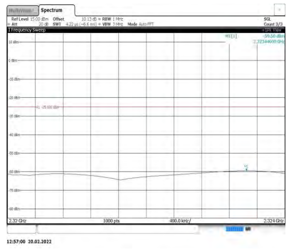
Band40-5MHz-16QAM-39175-1RB#0- Range7:2320~2324MHz
