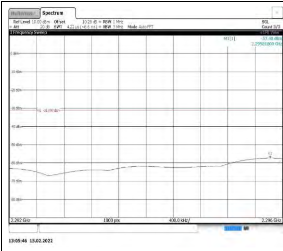
Band40-10MHz-16QAM-39200-1RB#0- Range4:2292~2296MHz
