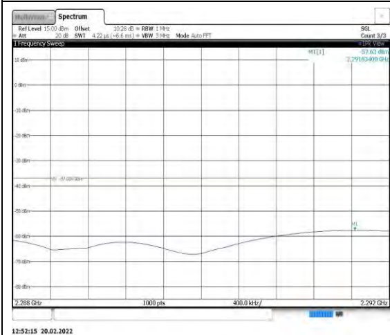
Band40-10MHz-16QAM-38750-1RB#0- Range3:2288~2292MHz
