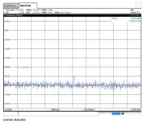
Band40-5MHz-16QAM-38775-1RB#0- Range2:1000~2288MHz
