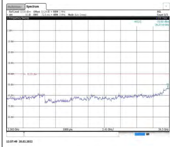
Band40-5MHz-16QAM-39175-1RB#0- Range13:2365~26500MHz
