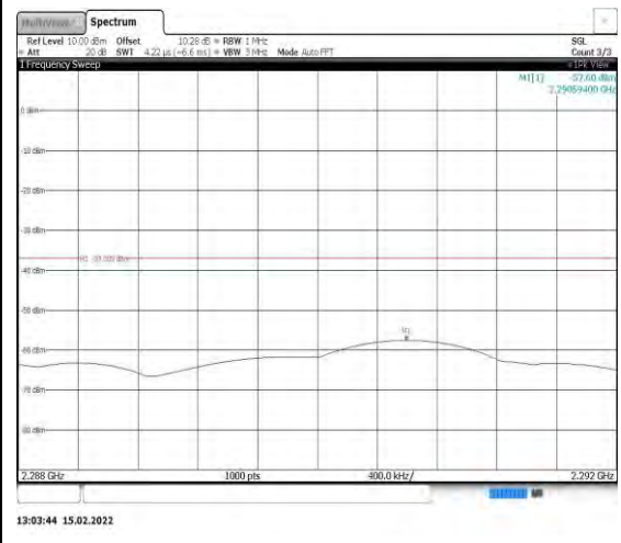
Band40-10MHz-QPSK-39200-1RB#0- Range3:2288~2292MHz
