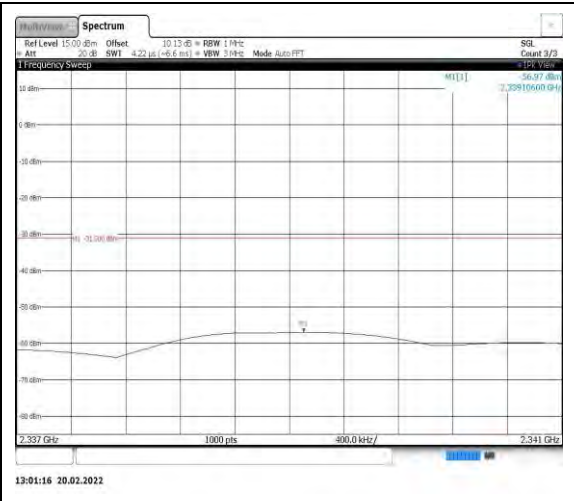
Band40-5MHz-16QAM-39200-1RB#0- Range10:2337~2341MHz
