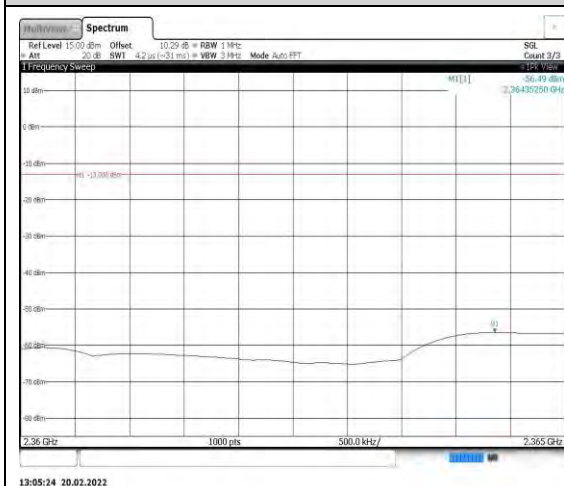
Band40-5MHz-16QAM-39225-1RB#0- Range12:2360~2365MHz
