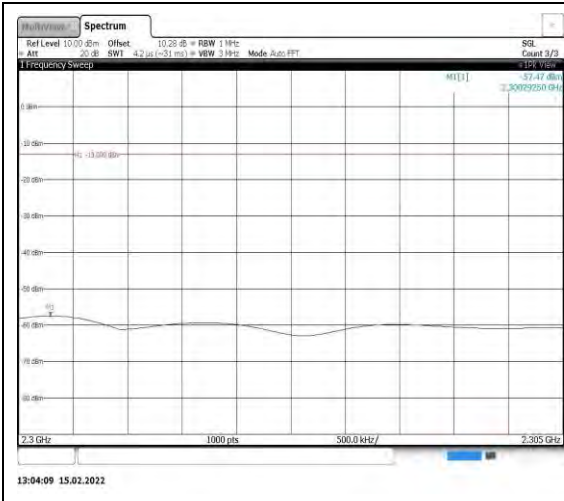
Band40-10MHz-QPSK-39200-1RB#0- Range6:2300~2305MHz
