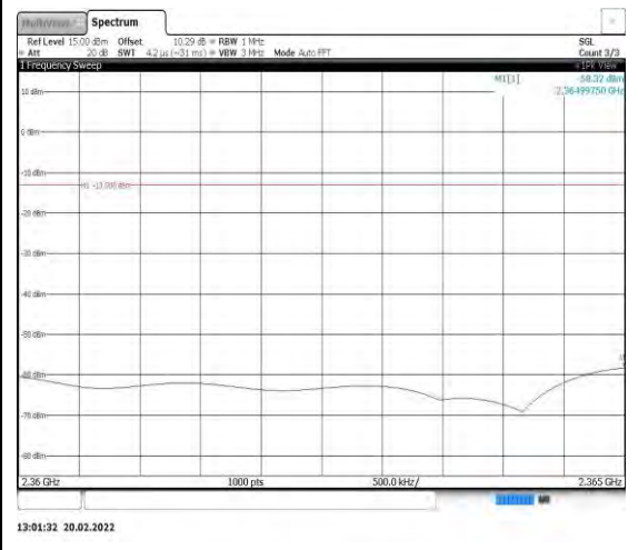
Band40-5MHz-16QAM-39200-1RB#0- Range12:2360~2365MHz
