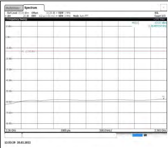
Band40-10MHz-16QAM-38750-1RB#0- Range12:2360~2365MHz
