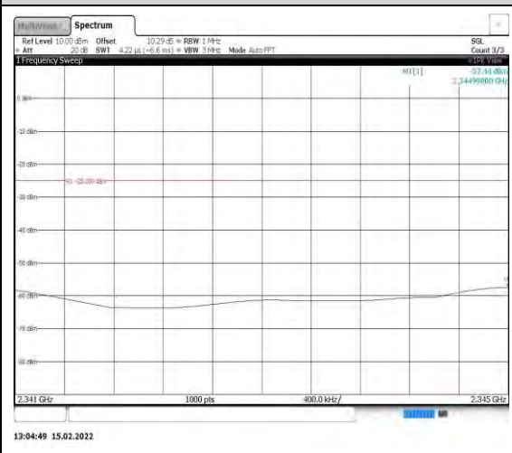
Band40-10MHz-QPSK-39200-1RB#0- Range11:2341~2345MHz
