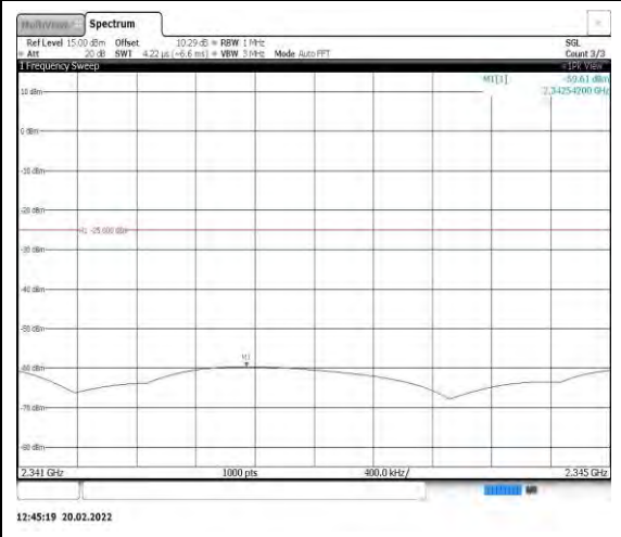
Band40-5MHz-16QAM-38750-1RB#0- Range11:2341~2345MHz
