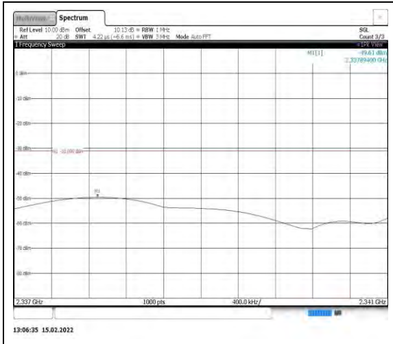
Band40-10MHz-16QAM-39200-1RB#0- Range10:2337~2341MHz
