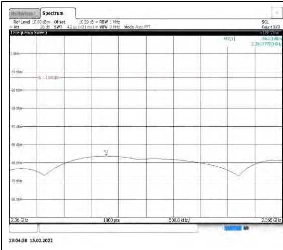
Band40-10MHz-QPSK-39200-1RB#0- Range12:2360~2365MHz
