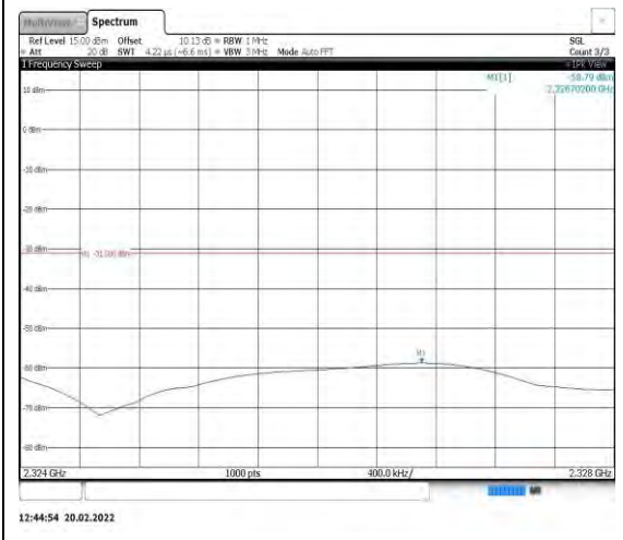
Band40-5MHz-16QAM-38750-1RB#0- Range8:2324~2328MHz
