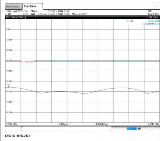
Band40-10MHz-QPSK-39200-1RB#0- Range4:2292~2296MHz
