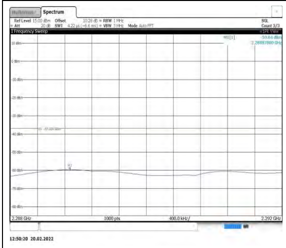
Band40-10MHz-QPSK-38750-1RB#0- Range3:2288~2292MHz
