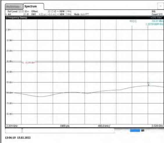
Band40-10MHz-16QAM-39200-1RB#0- Range8:2324~2328MHz
