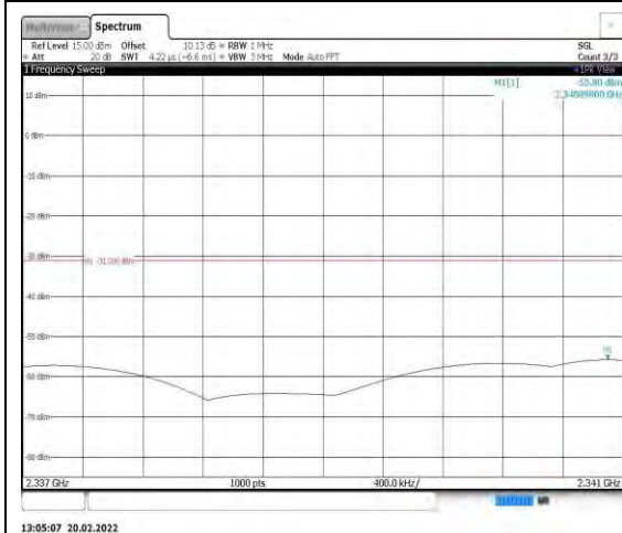
Band40-5MHz-16QAM-39225-1RB#0- Range10:2337~2341MHz
