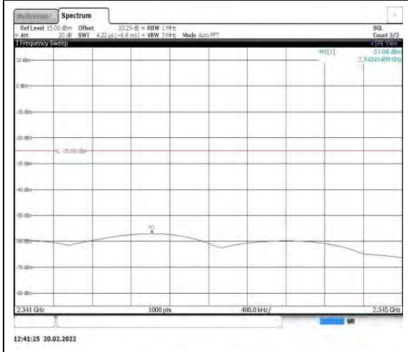
Band40-5MHz-16QAM-38725-1RB#0- Range11:2341~2345MHz
