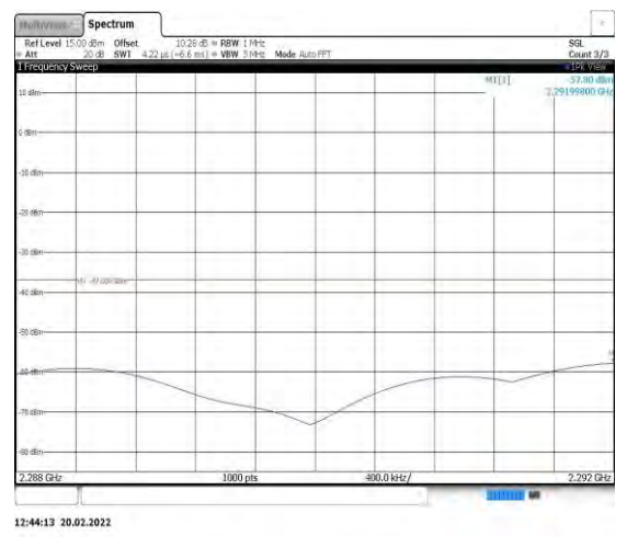
Band40-5MHz-16QAM-38750-1RB#0- Range3:2288~2292MHz
