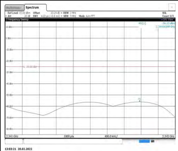
Band40-5MHz-QPSK-39225-1RB#0- Range11:2341~2345MHz
