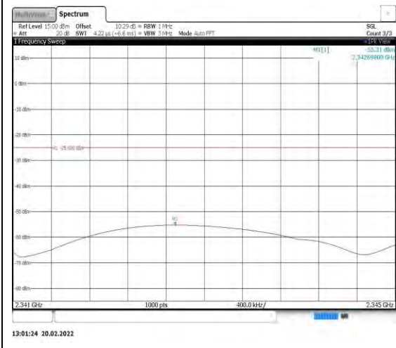
Band40-5MHz-16QAM-39200-1RB#0- Range11:2341~2345MHz
