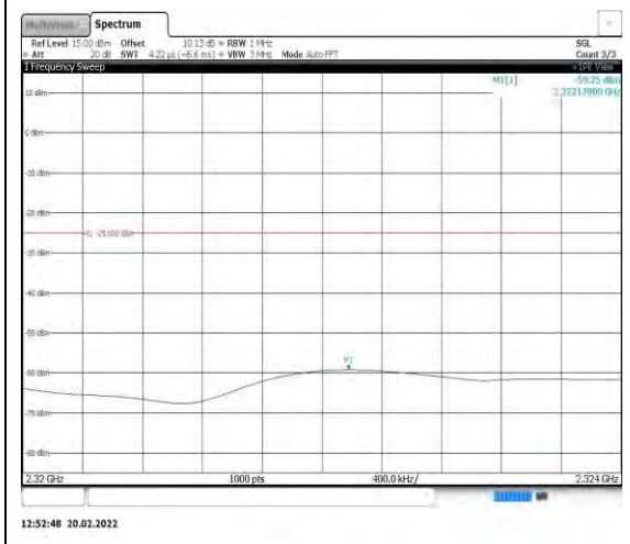
Band40-10MHz-16QAM-38750-1RB#0- Range7:2320~2324MHz
