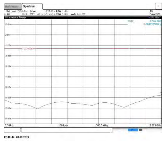
Band40-5MHz-16QAM-38725-1RB#0- Range6:2300~2305MHz
