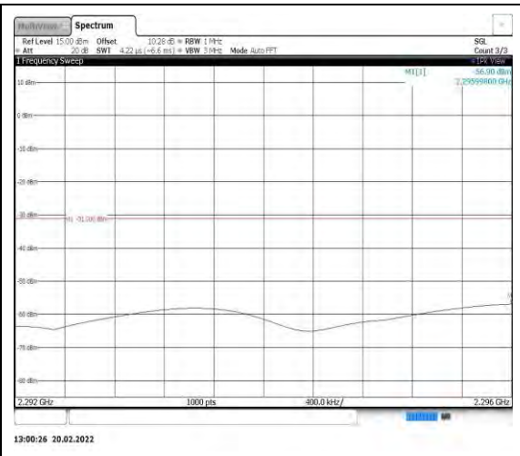
Band40-5MHz-16QAM-39200-1RB#0- Range4:2292~2296MHz
