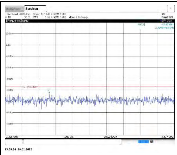
Band40-5MHz-QPSK-39225-1RB#0- Range9:2328~2337MHz
