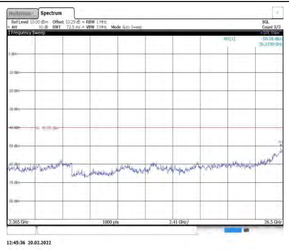
Band40-5MHz-16QAM-38750-1RB#0- Range13:2365~26500MHz
