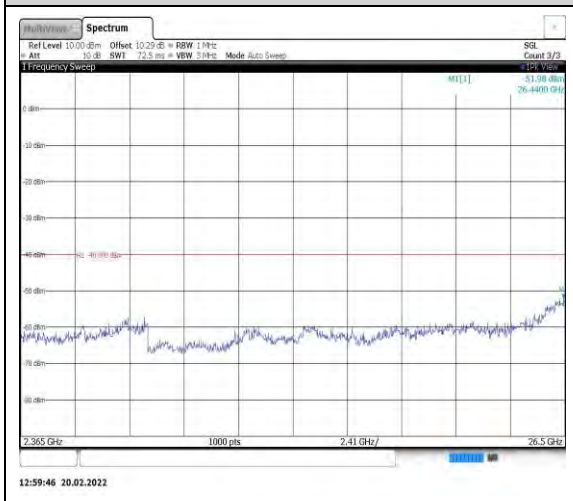
Band40-5MHz-QPSK-39200-1RB#0- Range13:2365~26500MHz
