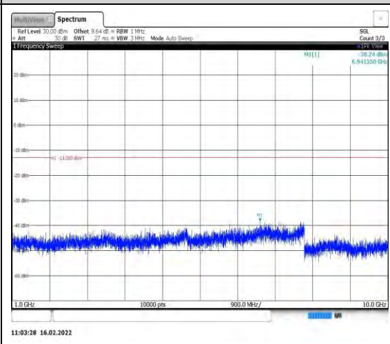
Band26-10MHz-16QAM-26840-1RB#0- Range2:1000~10000MHz
