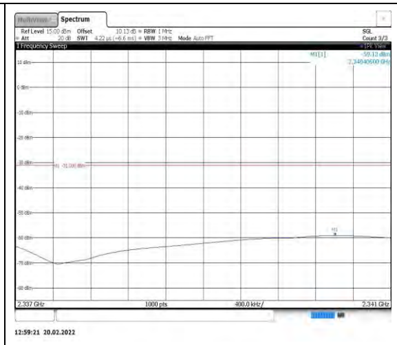
Band40-5MHz-QPSK-39200-1RB#0- Range10:2337~2341MHz
