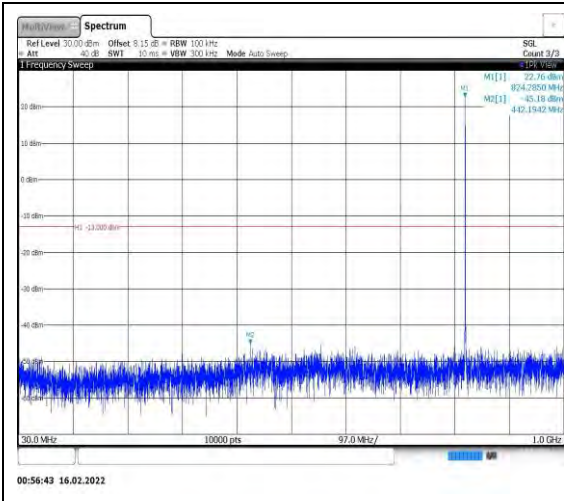
Band26-1.4MHz-QPSK-26797-1RB#0- Range1:30~1000MHz
