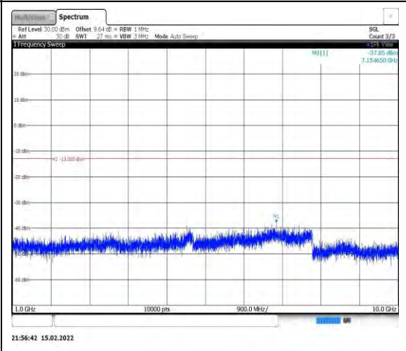
Band26-5MHz-16QAM-26765-1RB#0- Range2:1000~10000MHz
