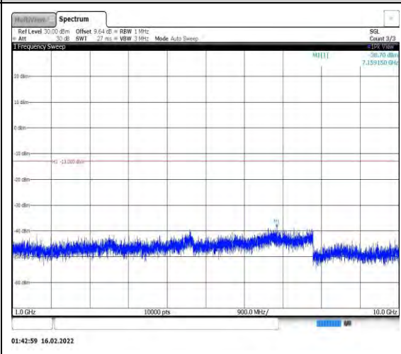
Band26-5MHz-QPSK-26915-1RB#0- Range2:1000~10000MHz
