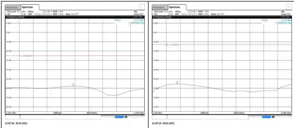
Band40-5MHz-QPSK-38775-1RB#0- Range11:2341~2345MHz
