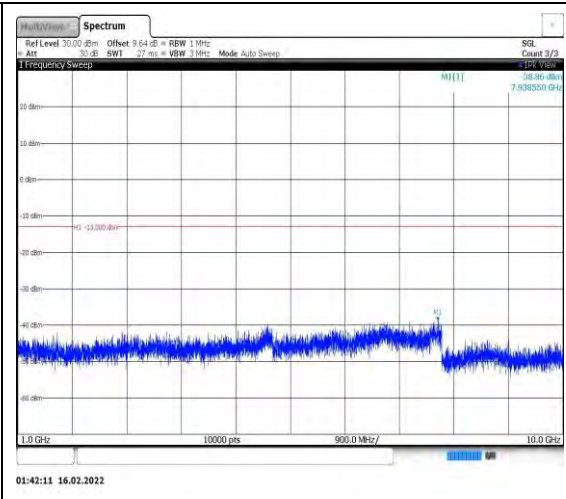
Band26-5MHz-QPSK-26815-1RB#0- Range2:1000~10000MHz
