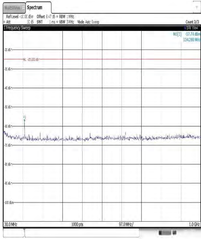
Band38-20MHz-QPSK-38000-1RB#0-Range1:30~1000MHz
