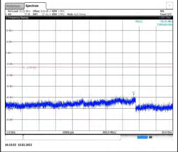
Band26-1.4MHz-QPSK-26783-1RB#0- Range2:1000~10000MHz
