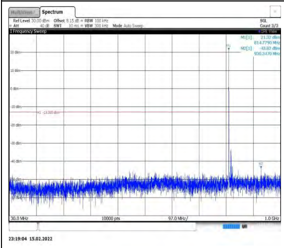
Band26-15MHz-QPSK-26765-1RB#0- Range1:30~1000MHz
