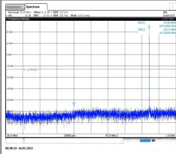
Band26-1.4MHz-QPSK-27033-1RB#0- Range1:30~1000MHz
