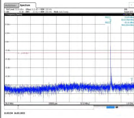
Band26-10MHz-QPSK-26840-1RB#0- Range1:30~1000MHz
