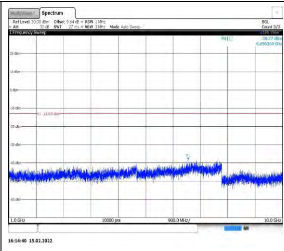
Band26-1.4MHz-16QAM-26697-1RB#0- Range2:1000~10000MHz
