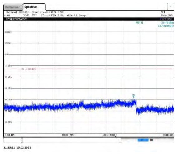
Band26-5MHz-QPSK-26740-1RB#0- Range2:1000~10000MHz
