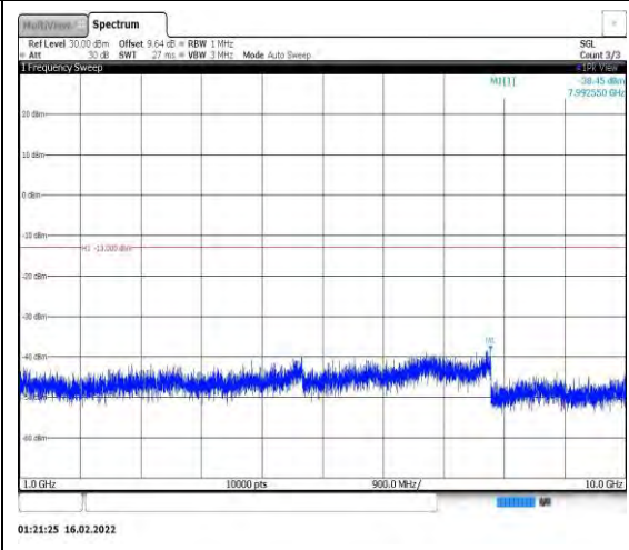
Band26-3MHz-16QAM-27025-1RB#0- Range2:1000~10000MHz
