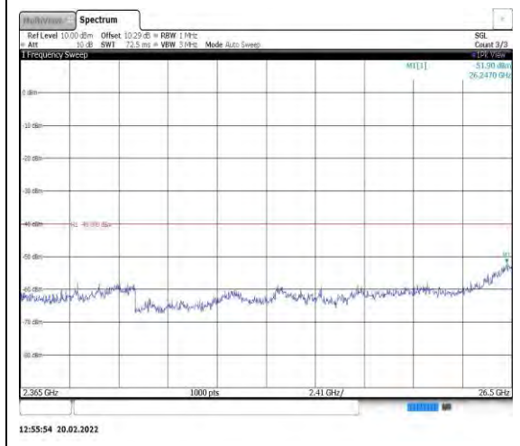
Band40-5MHz-QPSK-39175-1RB#0- Range13:2365~26500MHz
