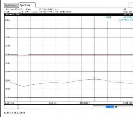
Band40-5MHz-QPSK-39175-1RB#0- Range8:2324~2328MHz
