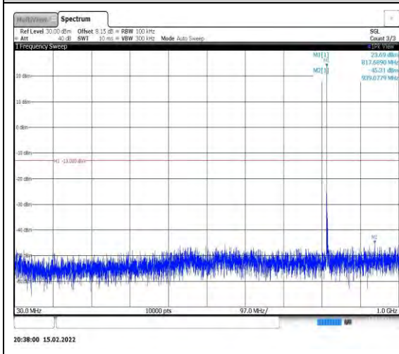
Band26-3MHz-16QAM-26740-1RB#0- Range1:30~1000MHz
