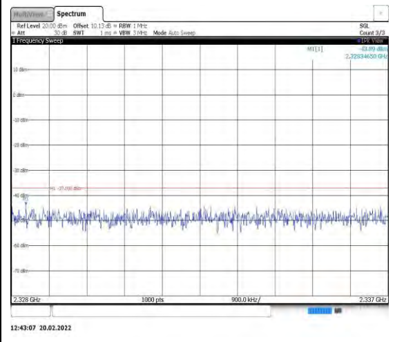
Band40-5MHz-QPSK-38750-1RB#0- Range9:2328~2337MHz
