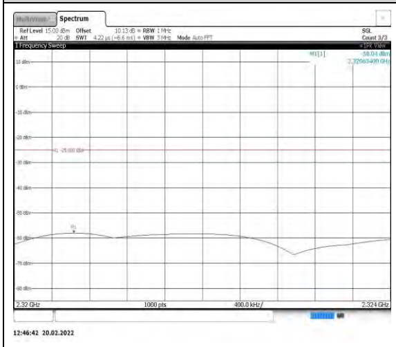
Band40-5MHz-QPSK-38775-1RB#0- Range7:2320~2324MHz
