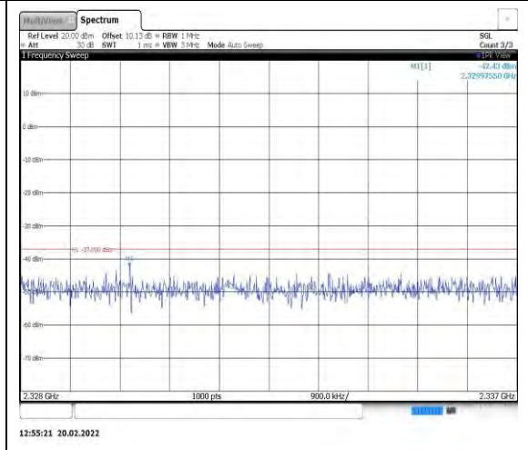
Band40-5MHz-QPSK-39175-1RB#0- Range9:2328~2337MHz
