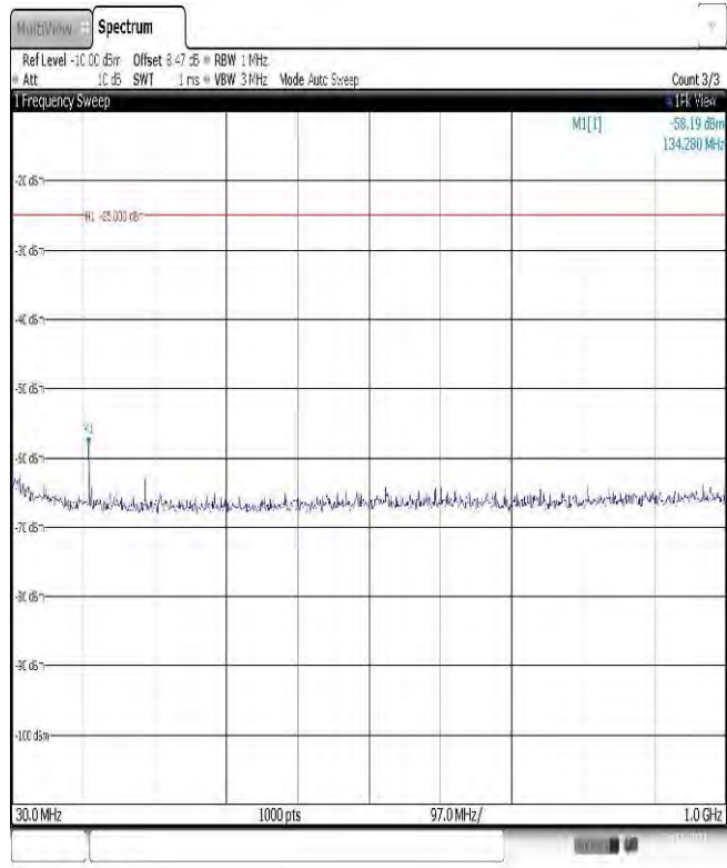
Band38-10MHz-QPSK-38000-1RB#0-Range1:30~1000MHz
