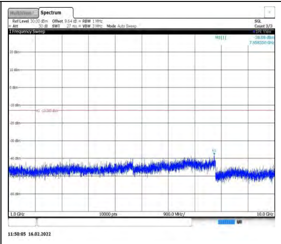
Band26-15MHz-QPSK-26865-1RB#0- Range2:1000~10000MHz
