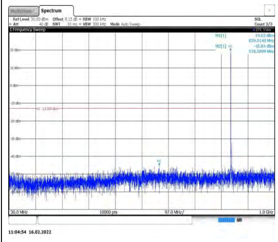
Band26-10MHz-16QAM-26990-1RB#0- Range1:30~1000MHz
