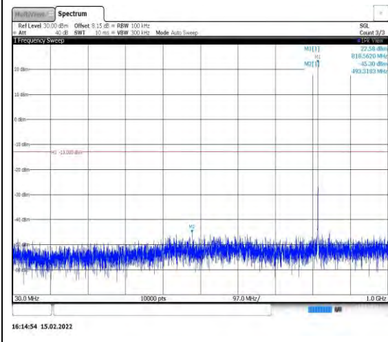
Band26-1.4MHz-QPSK-26740-1RB#0- Range1:30~1000MHz
