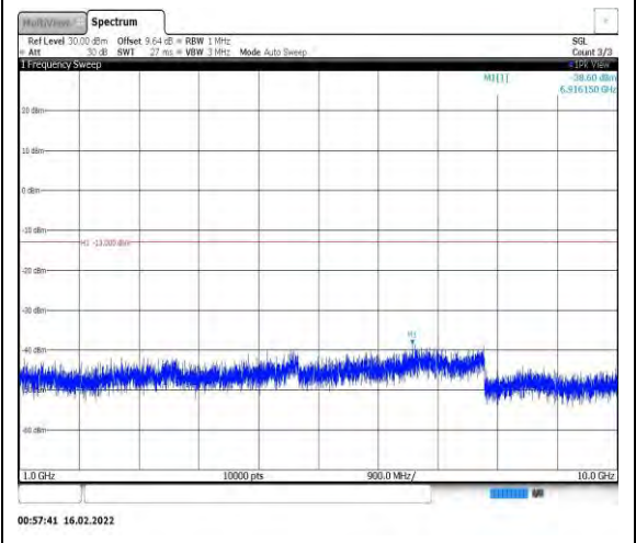
Band26-1.4MHz-QPSK-26915-1RB#0- Range2:1000~10000MHz
