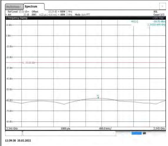
Band40-5MHz-QPSK-38725-1RB#0- Range11:2341~2345MHz
