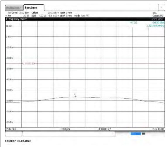
Band40-5MHz-QPSK-38725-1RB#0- Range7:2320~2324MHz
