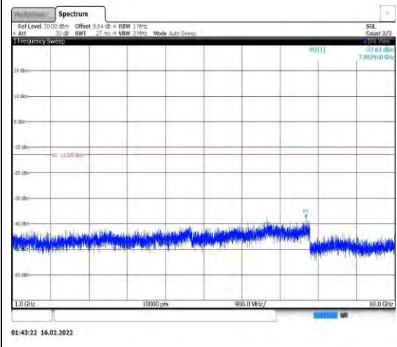
Band26-5MHz-16QAM-26915-1RB#0- Range2:1000~10000MHz
