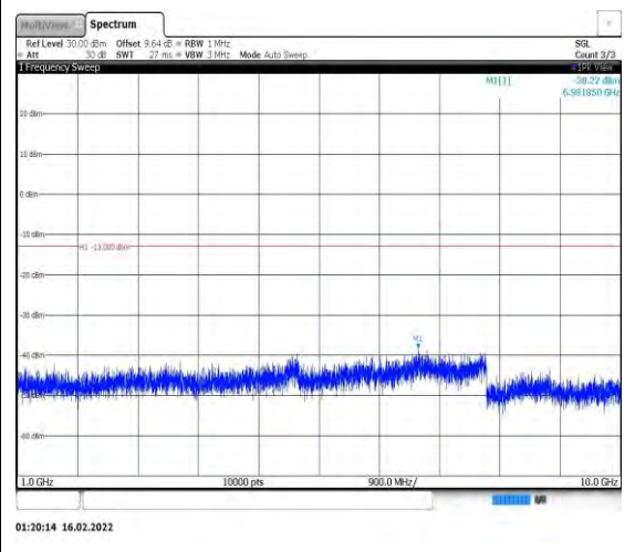
Band26-3MHz-QPSK-26915-1RB#0- Range2:1000~10000MHz
