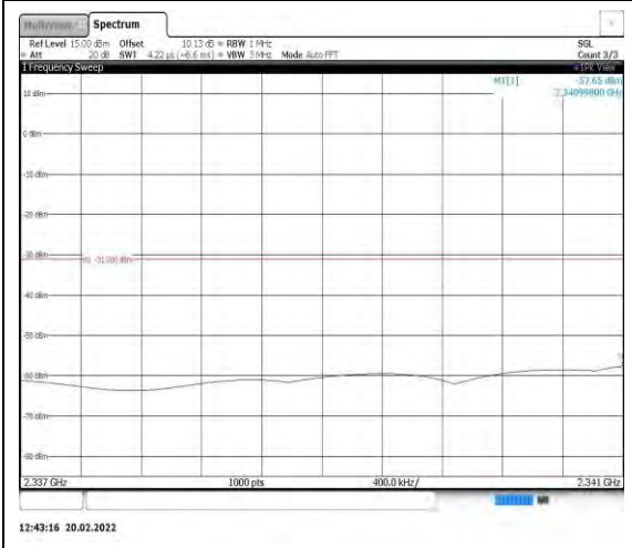
Band40-5MHz-QPSK-38750-1RB#0- Range10:2337~2341MHz
