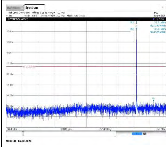
Band26-3MHz-16QAM-26775-1RB#0- Range1:30~1000MHz
