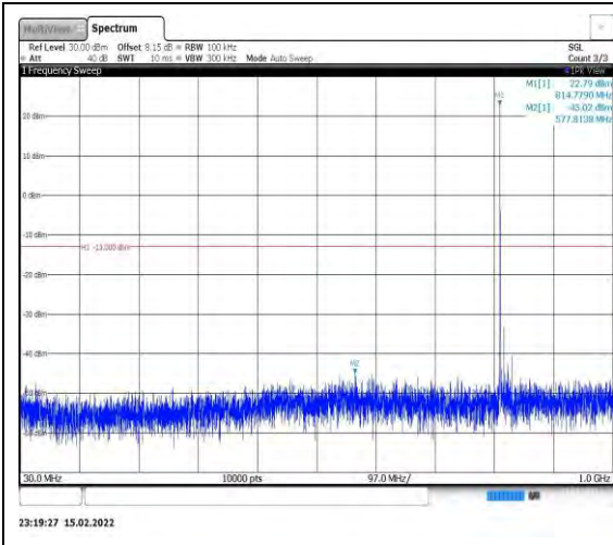
Band26-15MHz-16QAM-26765-1RB#0- Range1:30~1000MHz
