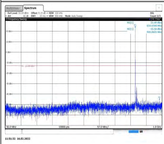
Band26-15MHz-QPSK-26965-1RB#0- Range1:30~1000MHz
