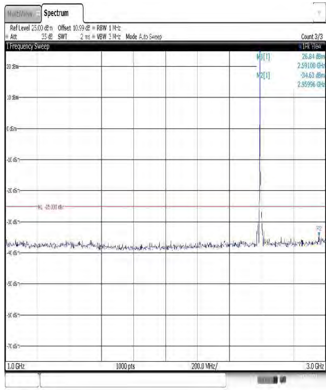
Band38-10MHz-16QAM-38000-1RB#0-Range2:1000~3000MHz
