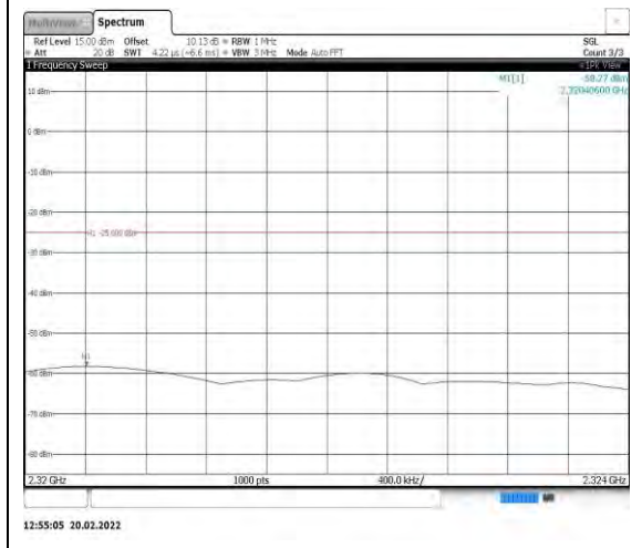
Band40-5MHz-QPSK-39175-1RB#0- Range7:2320~2324MHz
