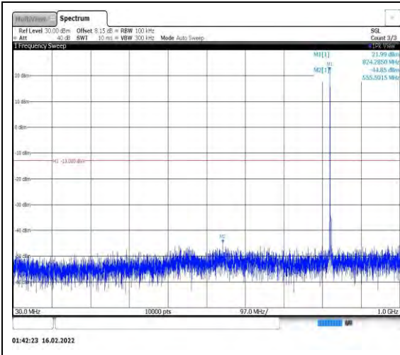
Band26-5MHz-16QAM-26815-1RB#0- Range1:30~1000MHz
