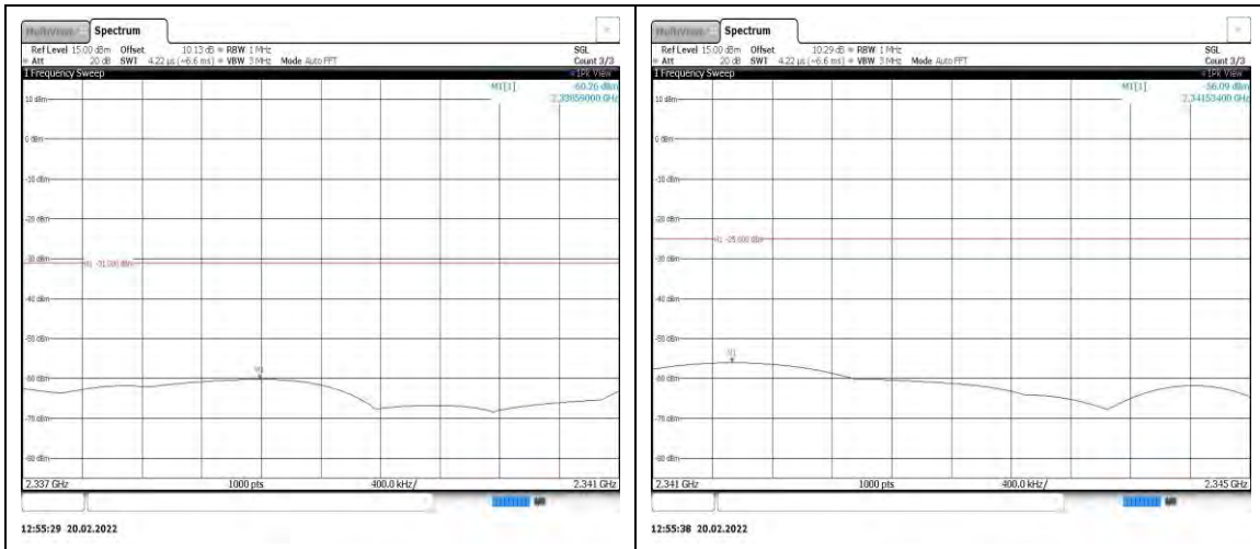
Band40-5MHz-QPSK-39175-1RB#0- Range10:2337~2341MHz
