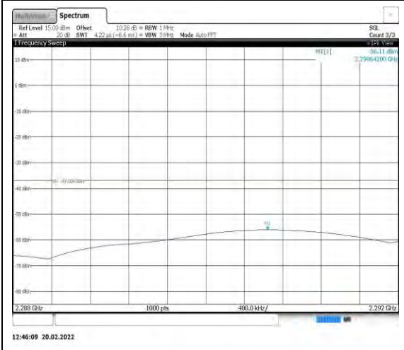
Band40-5MHz-QPSK-38775-1RB#0- Range3:2288~2292MHz
