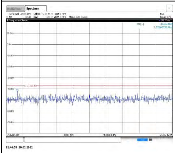
Band40-5MHz-QPSK-38775-1RB#0- Range9:2328~2337MHz
