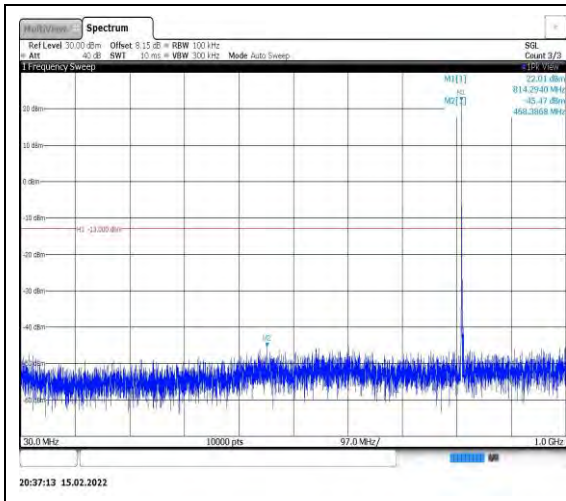
Band26-3MHz-16QAM-26705-1RB#0- Range1:30~1000MHz
