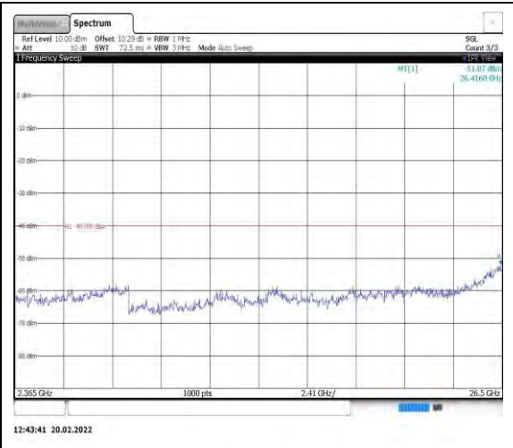
Band40-5MHz-QPSK-38750-1RB#0- Range13:2365~26500MHz
