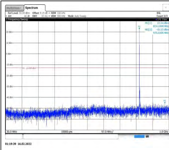
Band26-3MHz-16QAM-26805-1RB#0- Range1:30~1000MHz
