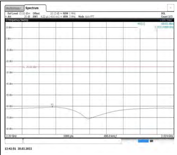
Band40-5MHz-QPSK-38750-1RB#0- Range7:2320~2324MHz
