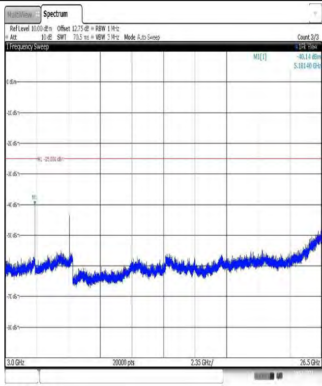
Band38-10MHz-QPSK-38000-1RB#0-Range3:3000~26500MHz
