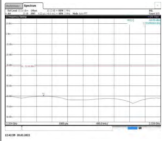
Band40-5MHz-QPSK-38750-1RB#0- Range8:2324~2328MHz
