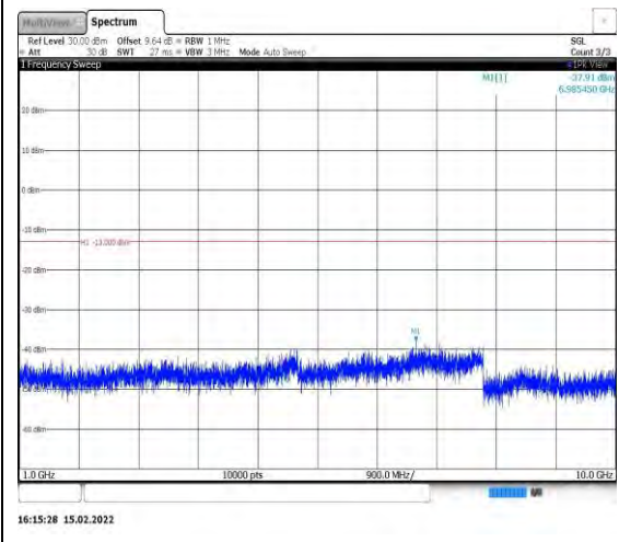
Band26-1.4MHz-16QAM-26740-1RB#0- Range2:1000~10000MHz
