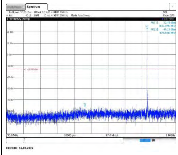
Band26-3MHz-QPSK-26915-1RB#0- Range1:30~1000MHz
