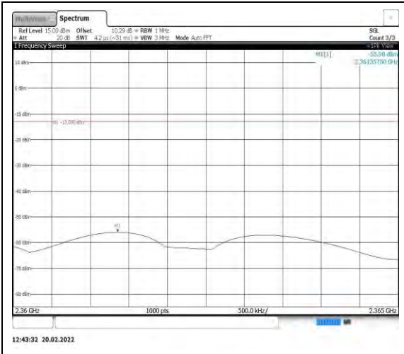
Band40-5MHz-QPSK-38750-1RB#0- Range12:2360~2365MHz
