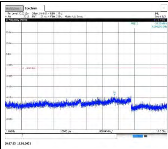
Band26-3MHz-16QAM-26705-1RB#0- Range2:1000~10000MHz
