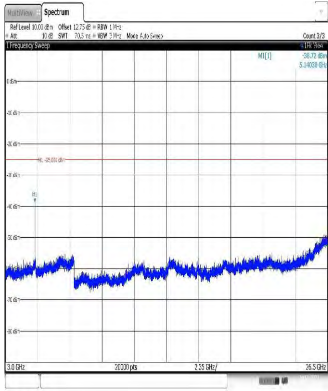
Band38-10MHz-16QAM-37800-1RB#0-Range3:3000~26500MHz
