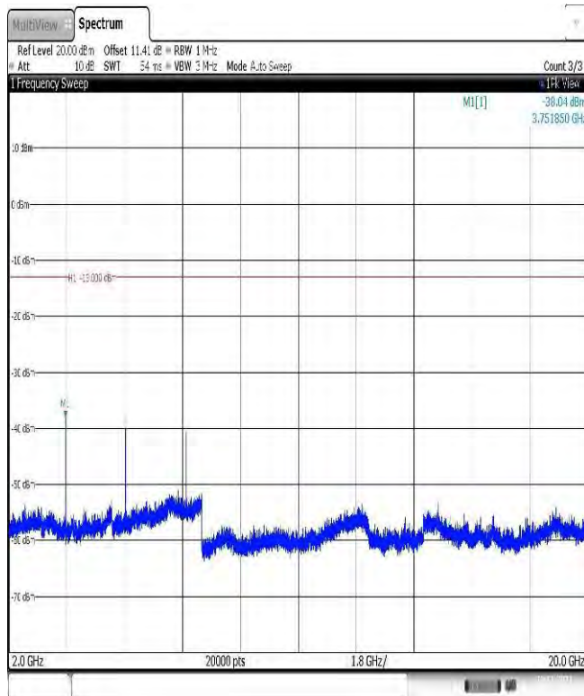
Band25-15MHz-QPSK-26365-1RB#0-Range3:2000~20000MHz
