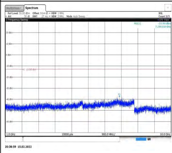
Band26-3MHz-16QAM-26775-1RB#0- Range2:1000~10000MHz
