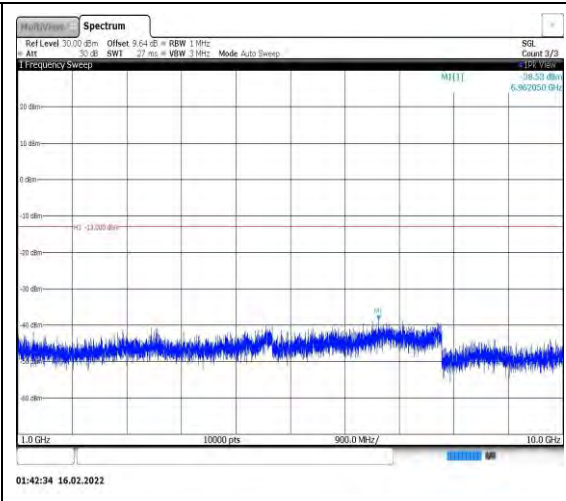
Band26-5MHz-16QAM-26815-1RB#0- Range2:1000~10000MHz
