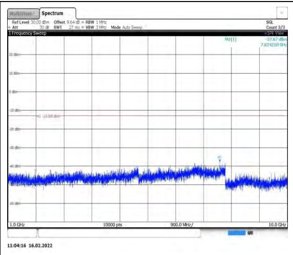
Band26-10MHz-16QAM-26915-1RB#0- Range2:1000~10000MHz
