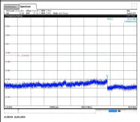
Band26-15MHz-QPSK-26915-1RB#0- Range2:1000~10000MHz
