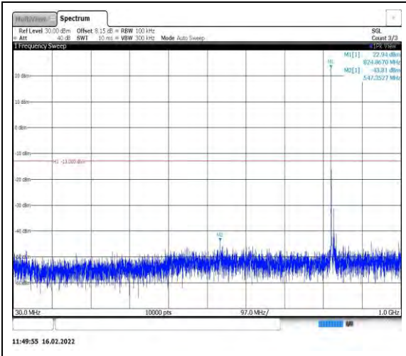
Band26-15MHz-QPSK-26865-1RB#0- Range1:30~1000MHz
