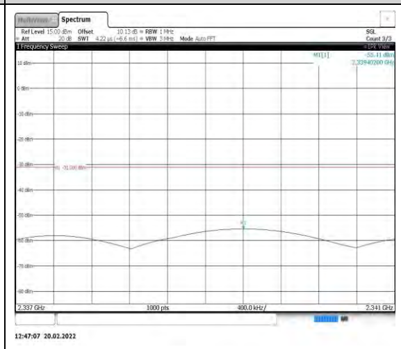
Band40-5MHz-QPSK-38775-1RB#0- Range10:2337~2341MHz
