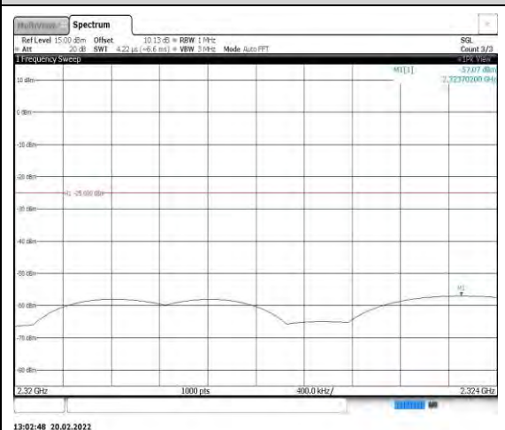
Band40-5MHz-QPSK-39225-1RB#0- Range7:2320~2324MHz
