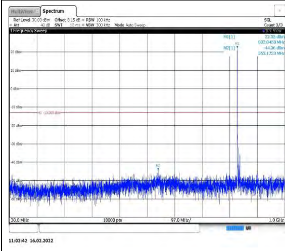
Band26-10MHz-QPSK-26915-1RB#0- Range1:30~1000MHz
