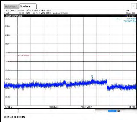
Band26-3MHz-16QAM-26805-1RB#0- Range2:1000~10000MHz
