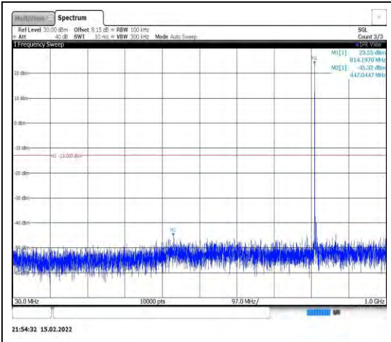
Band26-5MHz-QPSK-26715-1RB#0- Range1:30~1000MHz
