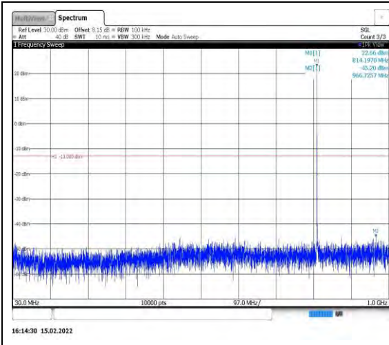
Band26-1.4MHz-16QAM-26697-1RB#0- Range1:30~1000MHz
