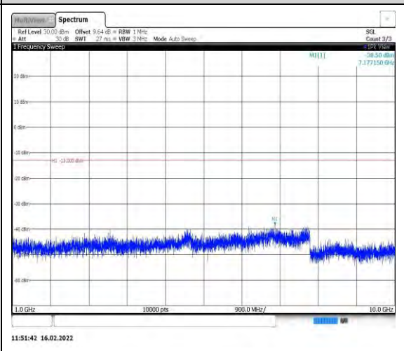
Band26-15MHz-QPSK-26965-1RB#0- Range2:1000~10000MHz
