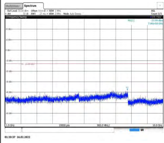
Band26-3MHz-16QAM-26915-1RB#0- Range2:1000~10000MHz
