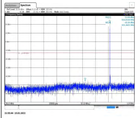
Band26-5MHz-16QAM-26740-1RB#0- Range1:30~1000MHz
