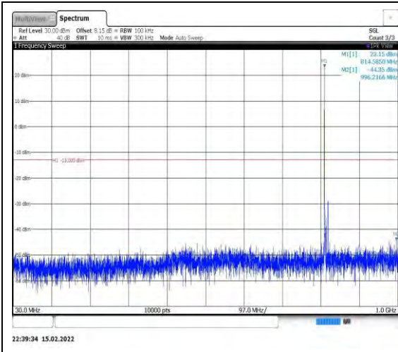
Band26-10MHz-QPSK-26740-1RB#0- Range1:30~1000MHz
