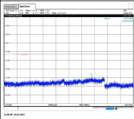
Band26-10MHz-16QAM-26740-1RB#0- Range2:1000~10000MHz
