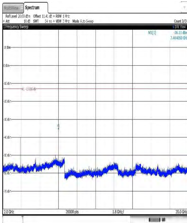
Band25-20MHz-16QAM-26140-1RB#0-Range3:2000~20000MHz
