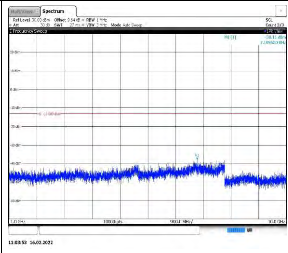
Band26-10MHz-QPSK-26915-1RB#0- Range2:1000~10000MHz
