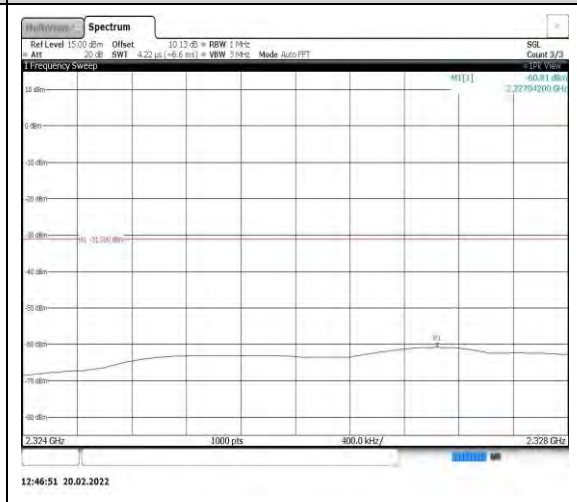
Band40-5MHz-QPSK-38775-1RB#0- Range8:2324~2328MHz
