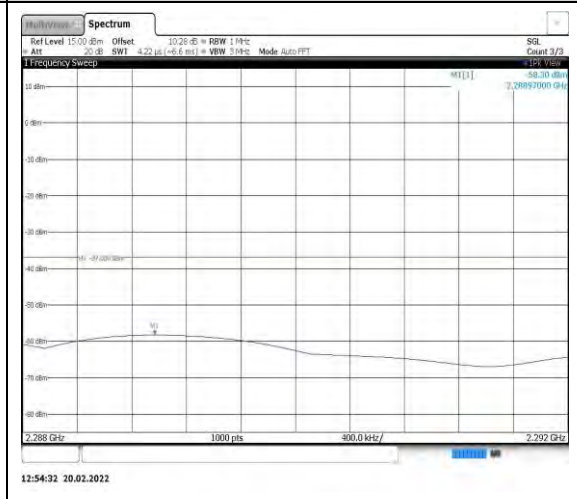
Band40-5MHz-QPSK-39175-1RB#0- Range3:2288~2292MHz
