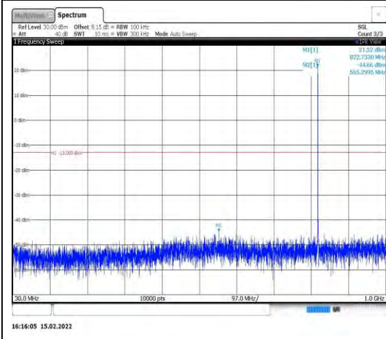
Band26-1.4MHz-16QAM-26783-1RB#0- Range1:30~1000MHz
