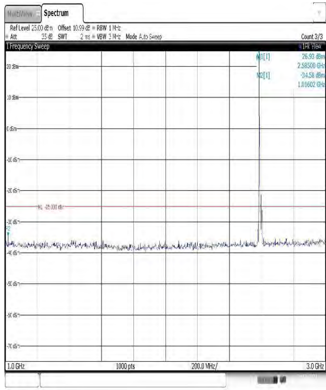
Band38-20MHz-16QAM-38000-1RB#0-Range2:1000~3000MHz
