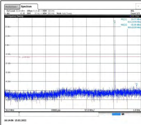
Band26-1.4MHz-QPSK-26697-1RB#0- Range1:30~1000MHz
