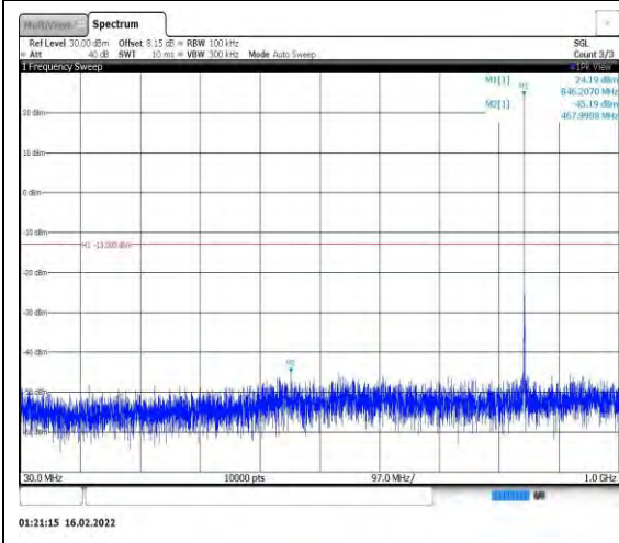
Band26-3MHz-16QAM-27025-1RB#0- Range1:30~1000MHz
