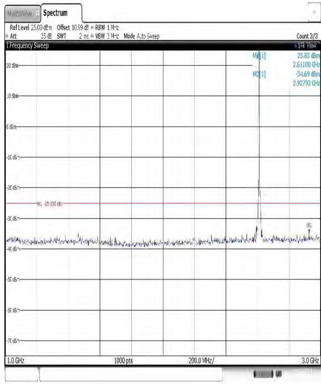
Band38-10MHz-QPSK-38200-1RB#0-Range2:1000~3000MHz
