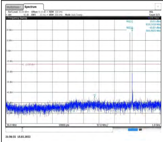
Band26-5MHz-16QAM-26765-1RB#0- Range1:30~1000MHz
