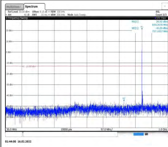
Band26-5MHz-16QAM-27015-1RB#0- Range1:30~1000MHz
