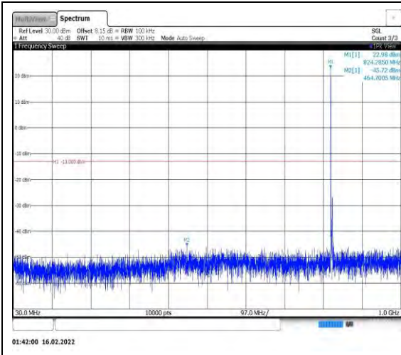
Band26-5MHz-QPSK-26815-1RB#0- Range1:30~1000MHz
