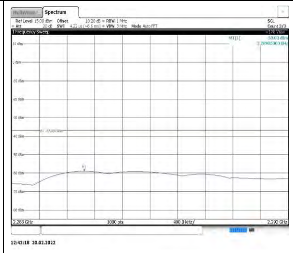
Band40-5MHz-QPSK-38750-1RB#0- Range3:2288~2292MHz
