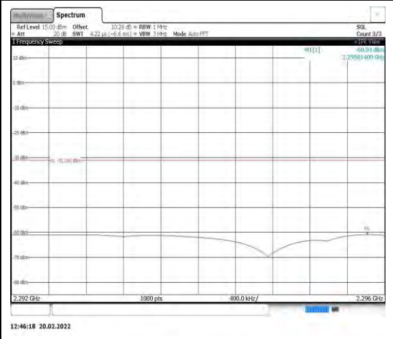
Band40-5MHz-QPSK-38775-1RB#0- Range4:2292~2296MHz
