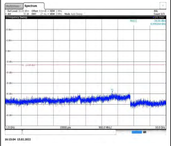
Band26-1.4MHz-QPSK-26740-1RB#0- Range2:1000~10000MHz
