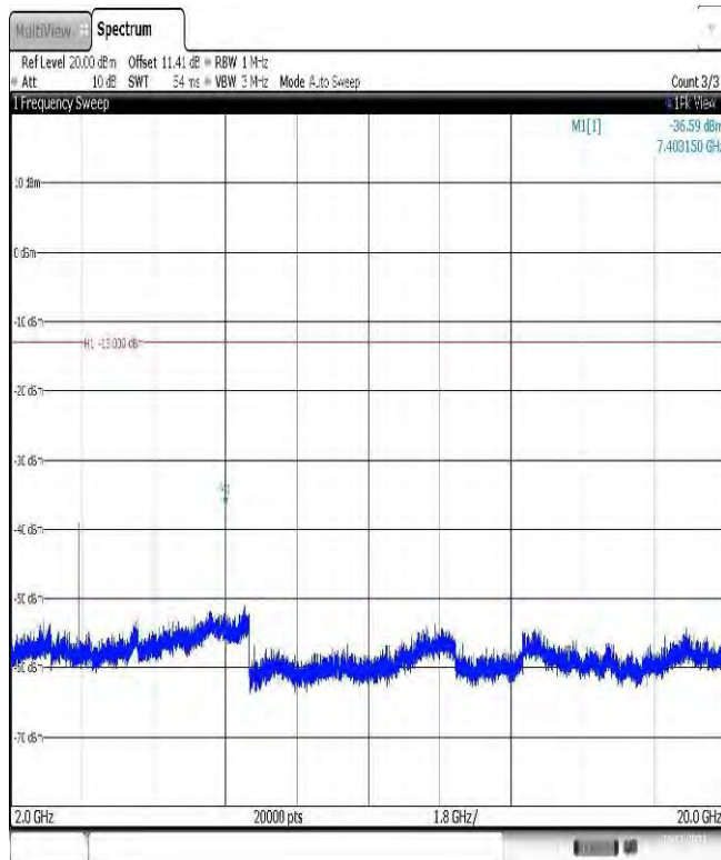
Band25-15MHz-16QAM-26115-1RB#0-Range3:2000~20000MHz
