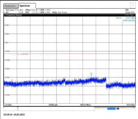
Band26-15MHz-QPSK-26765-1RB#0- Range2:1000~10000MHz
