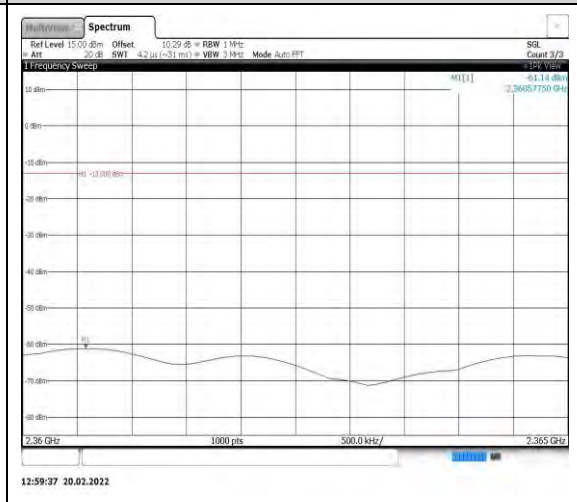
Band40-5MHz-QPSK-39200-1RB#0- Range12:2360~2365MHz
