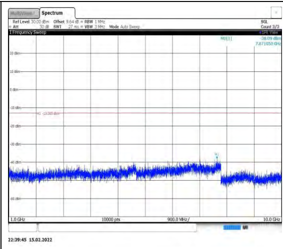
Band26-10MHz-QPSK-26740-1RB#0- Range2:1000~10000MHz
