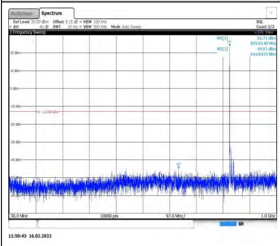
Band26-15MHz-QPSK-26915-1RB#0- Range1:30~1000MHz
