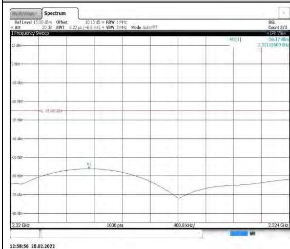
Band40-5MHz-QPSK-39200-1RB#0- Range7:2320~2324MHz
