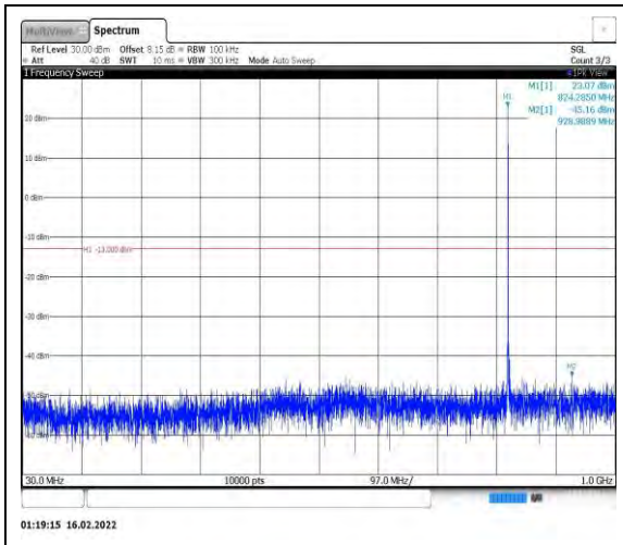
Band26-3MHz-QPSK-26805-1RB#0- Range1:30~1000MHz
