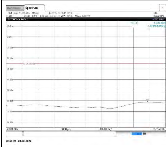
Band40-5MHz-QPSK-39200-1RB#0- Range11:2341~2345MHz
