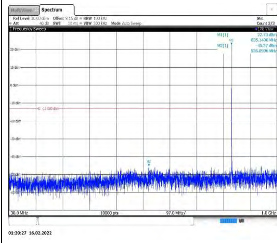
Band26-3MHz-16QAM-26915-1RB#0- Range1:30~1000MHz
