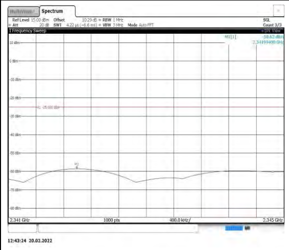
Band40-5MHz-QPSK-38750-1RB#0- Range11:2341~2345MHz
