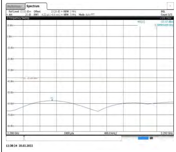
Band40-5MHz-QPSK-38725-1RB#0- Range3:2288~2292MHz
