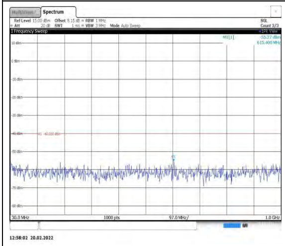
Band40-5MHz-QPSK-39200-1RB#0- Range1:30~1000MHz
