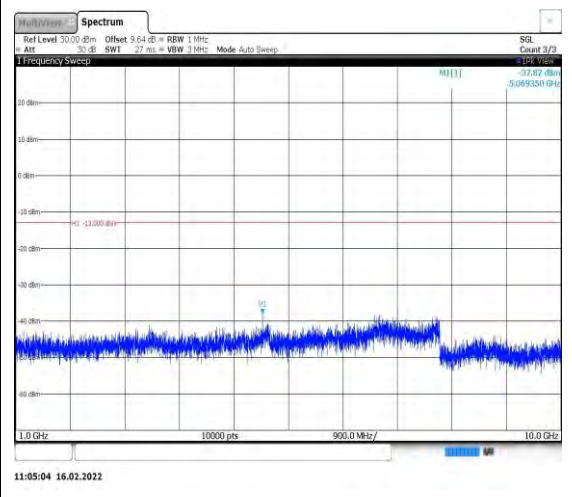
Band26-10MHz-16QAM-26990-1RB#0- Range2:1000~10000MHz
