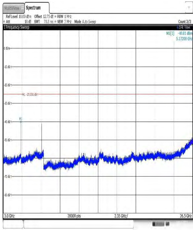
Band38-20MHz-QPSK-38000-1RB#0-Range3:3000~26500MHz
