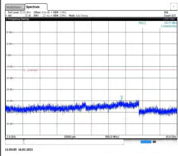
Band26-10MHz-QPSK-26840-1RB#0- Range2:1000~10000MHz
