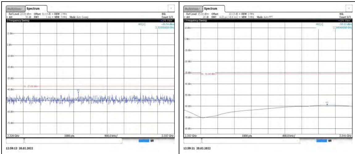
Band40-5MHz-QPSK-39200-1RB#0- Range9:2328~2337MHz
