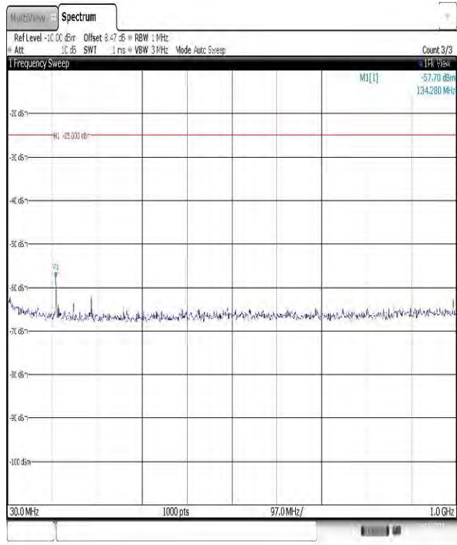
Band38-15MHz-QPSK-38000-1RB#0-Range1:30~1000MHz
