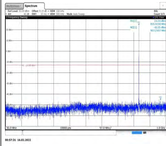
Band26-1.4MHz-QPSK-26915-1RB#0- Range1:30~1000MHz
