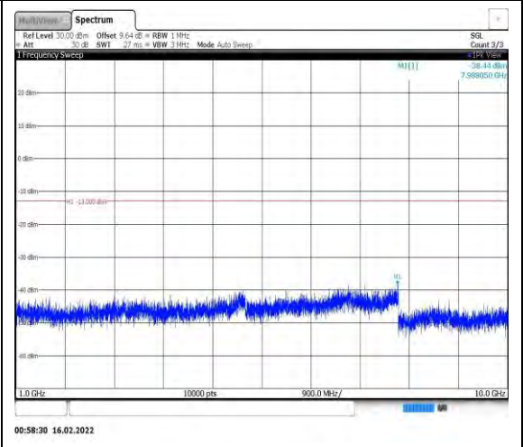
Band26-1.4MHz-QPSK-27033-1RB#0- Range2:1000~10000MHz
