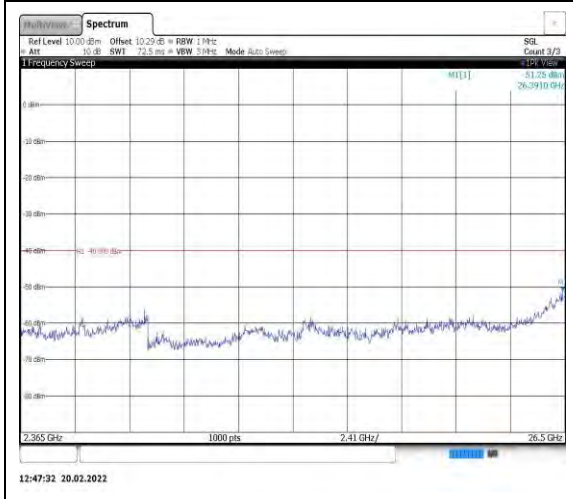
Band40-5MHz-QPSK-38775-1RB#0- Range13:2365~26500MHz
