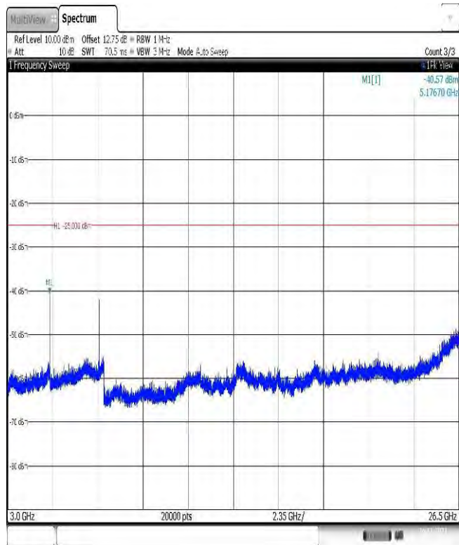
Band38-15MHz-QPSK-38000-1RB#0-Range3:3000~26500MHz
