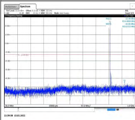
Band26-10MHz-16QAM-26740-1RB#0- Range1:30~1000MHz
