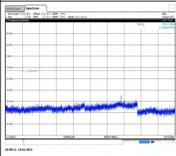
Band26-3MHz-16QAM-26740-1RB#0- Range2:1000~10000MHz
