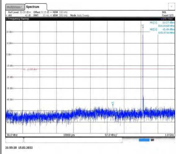
Band26-5MHz-QPSK-26740-1RB#0- Range1:30~1000MHz
