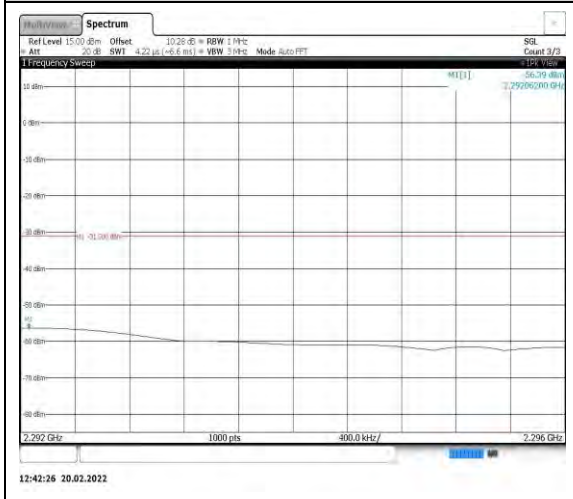
Band40-5MHz-QPSK-38750-1RB#0- Range4:2292~2296MHz
