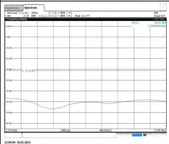
Band40-5MHz-QPSK-39200-1RB#0- Range8:2324~2328MHz
