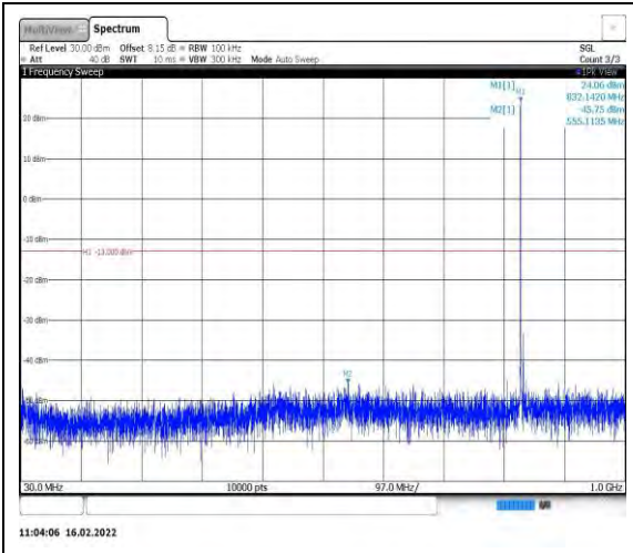
Band26-10MHz-16QAM-26915-1RB#0- Range1:30~1000MHz
