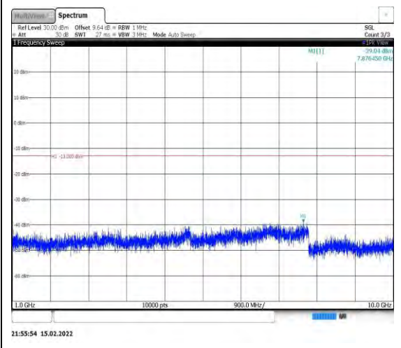
Band26-5MHz-16QAM-26740-1RB#0- Range2:1000~10000MHz
