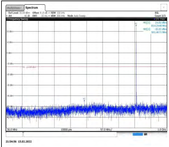
Band26-5MHz-16QAM-26715-1RB#0- Range1:30~1000MHz
