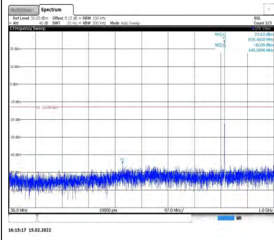
Band26-1.4MHz-16QAM-26740-1RB#0- Range1:30~1000MHz
