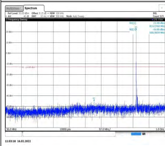
Band26-10MHz-16QAM-26840-1RB#0- Range1:30~1000MHz
