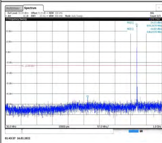
Band26-5MHz-QPSK-27015-1RB#0- Range1:30~1000MHz
