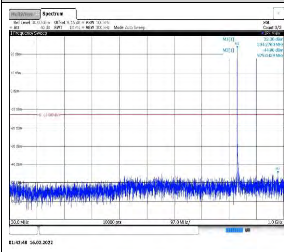
Band26-5MHz-QPSK-26915-1RB#0- Range1:30~1000MHz
