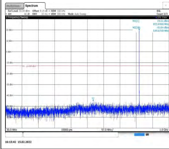
Band26-1.4MHz-QPSK-26783-1RB#0- Range1:30~1000MHz
