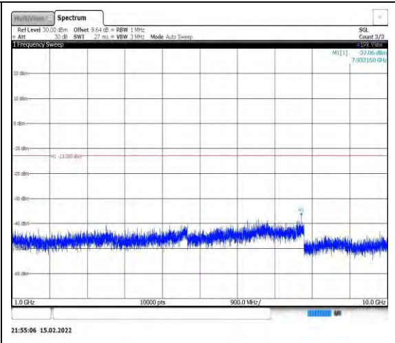
Band26-5MHz-16QAM-26715-1RB#0- Range2:1000~10000MHz
