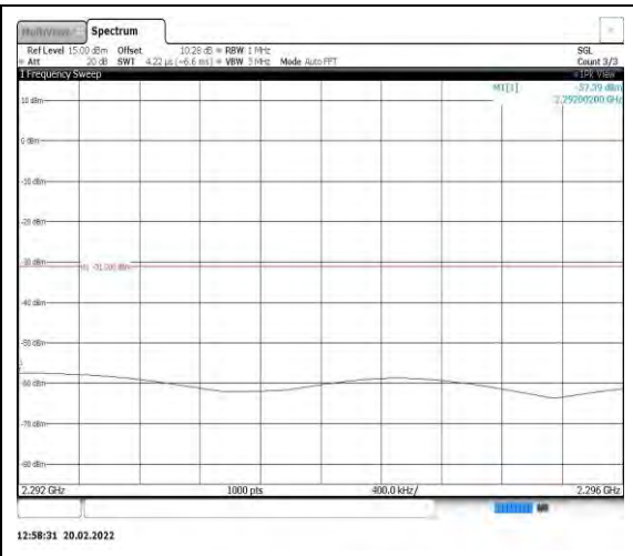
Band40-5MHz-QPSK-39200-1RB#0- Range4:2292~2296MHz
