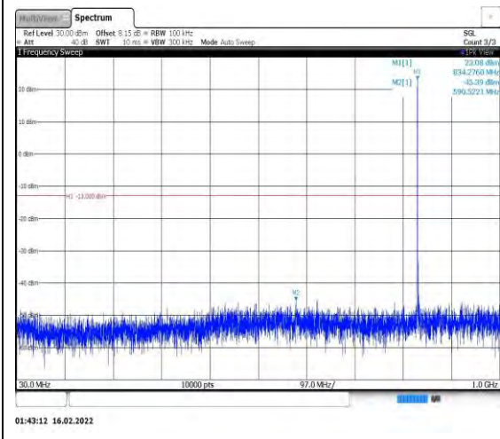
Band26-5MHz-16QAM-26915-1RB#0- Range1:30~1000MHz
