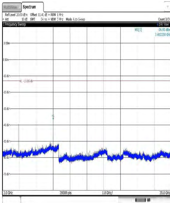
Band25-10MHz-16QAM-26090-1RB#0-Range3:2000~20000MHz
