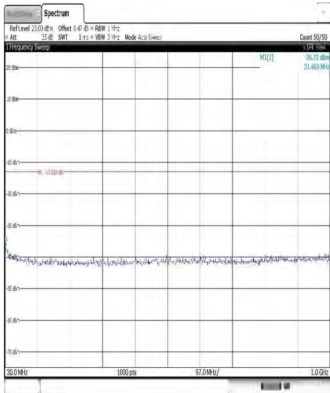
Band25-5MHz-16QAM-26665-1RB#0-Range1:30~1000MHz
