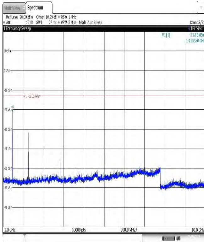
Band17-10MHz-16QAM-23800-1RB#0-Range2: 1000~10000MHz
