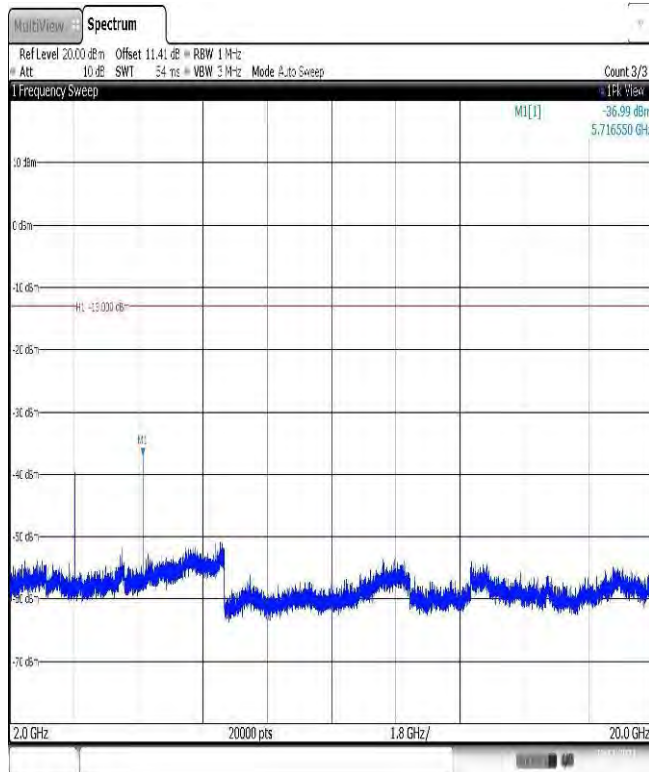
Band25-10MHz-16QAM-26640-1RB#0-Range3:2000~20000MHz
