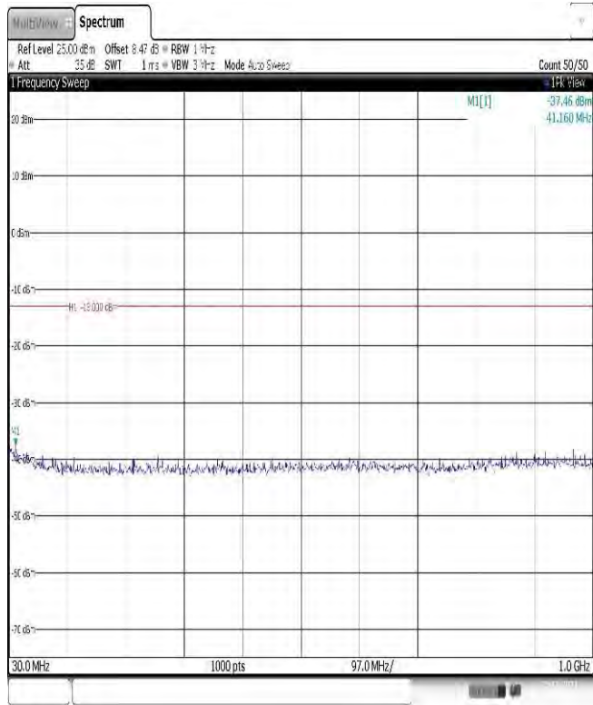
Band25-3MHz-QPSK-26365-1RB#0-Range1:30~1000MHz
