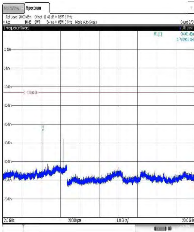
Band25-5MHz-16QAM-26665-1RB#0-Range3:2000~20000MHz
