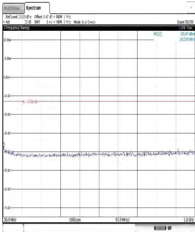
Band25-5MHz-16QAM-26065-1RB#0-Range1:30~1000MHz
