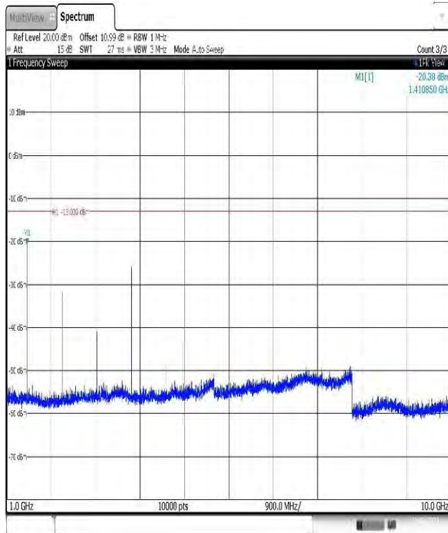
Band17-10MHz-16QAM-23790-1RB#0-Range2: 1000~10000MHz
