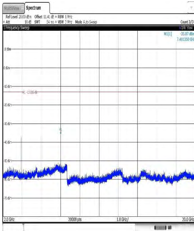
Band25-1.4MHz-16QAM-26047-1RB#0-Range3:2000~20000MHz
