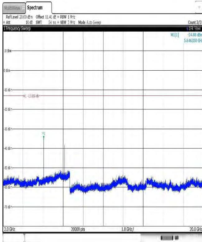
Band25-1.4MHz-QPSK-26365-1RB#0-Range3:2000~20000MHz
